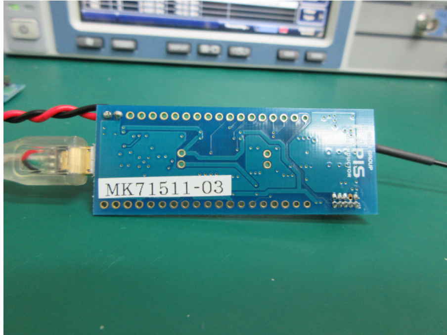
Photograph 9: Set-up for Conducted testing (View 3)
