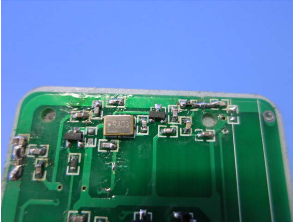
Transmitter Unit Oscillator comp side
