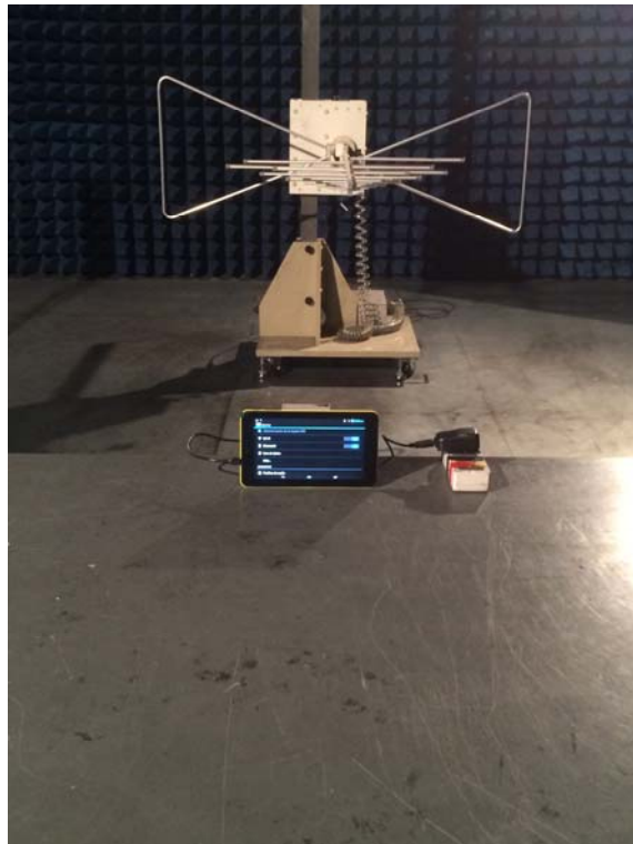
WIFI,BT, 2G, 3G communicating mode
