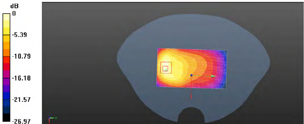
Plot 6: Body Rear Side (WCDMA Band V RMC Middle Channel)
