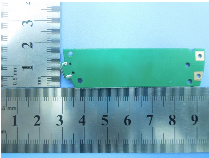
Photo 10 Appearance of PCB (Charger)
