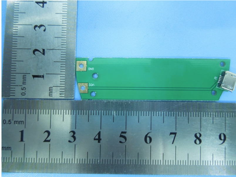
Photo 11 Appearance of PCB (Charger)
