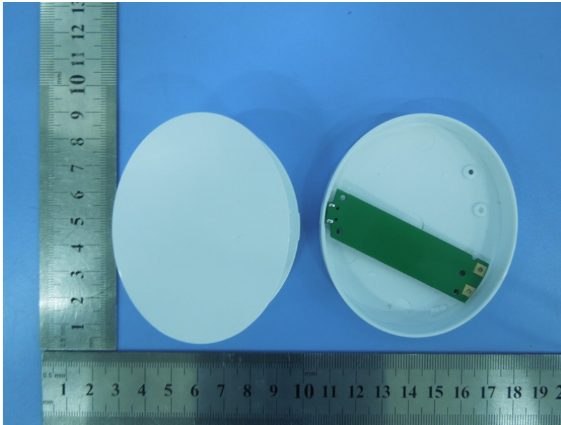
Photo 9 Internal of Charger
