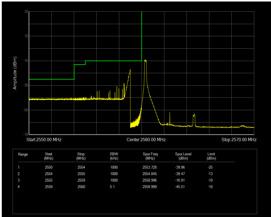
Band41 QAM16 BW=5MHz Channel=40315 RB Size=1 Position=#Max
