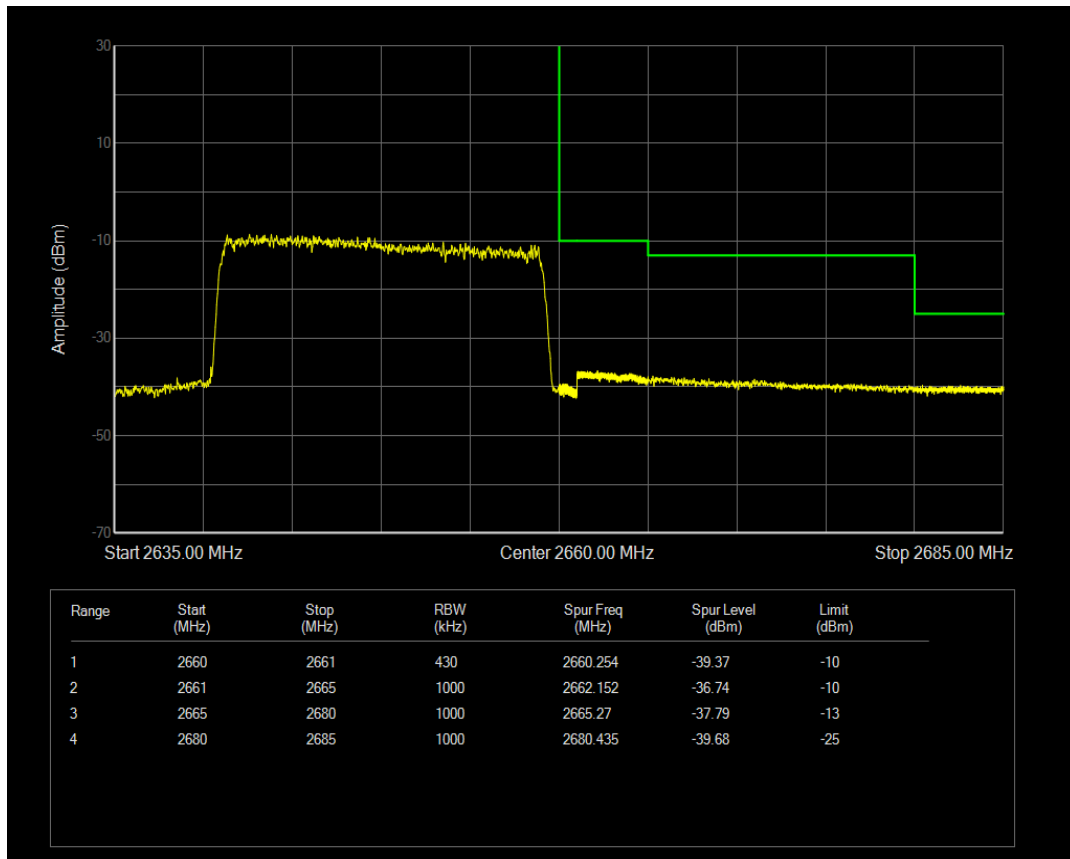
Band41 QPSK BW=20MHz Channel=41190 RB Size=1 Position=#Max
