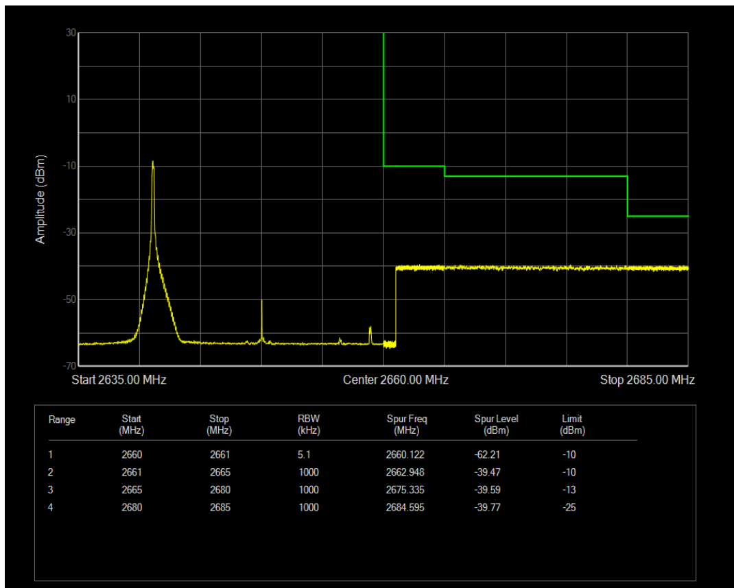
Band41 QAM16 BW=20MHz Channel=41190 RB Size=100 Position=#0
