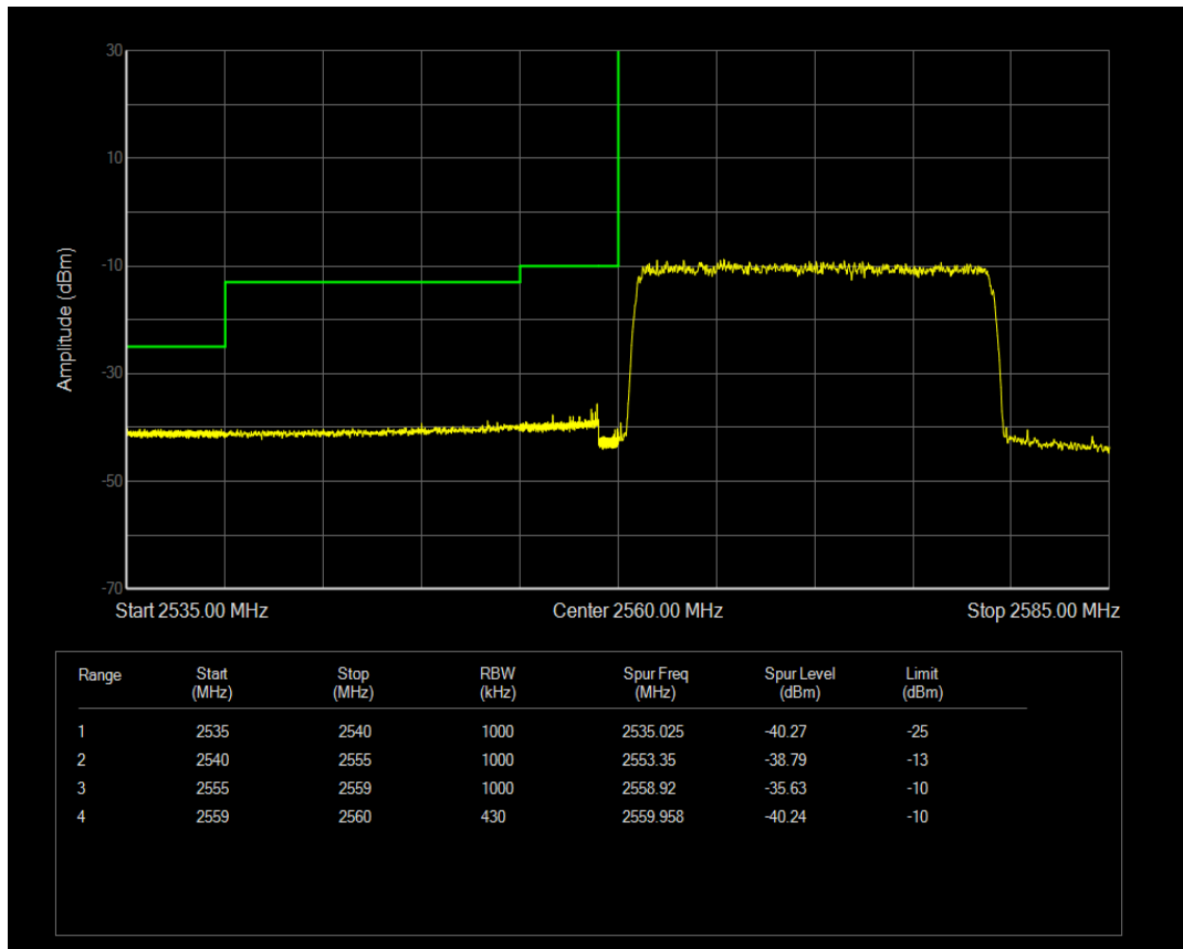
Band41 QPSK BW=20MHz Channel=40390 RB Size=1 Position=#Max
