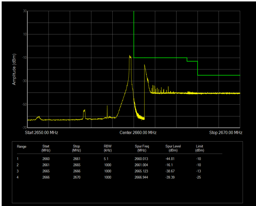
Band41 QAM16 BW=5MHz Channel=41265 RB Size=1 Position=#0
