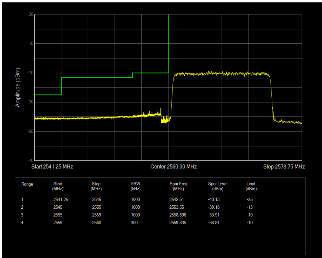
Band41 QAM16 BW=15MHz Channel=40365 RB Size=1 Position=#0
