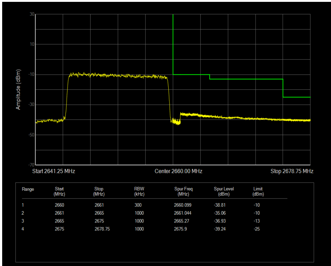
Band41 QAM16 BW=15MHz Channel=41215 RB Size=1 Position=#Max
