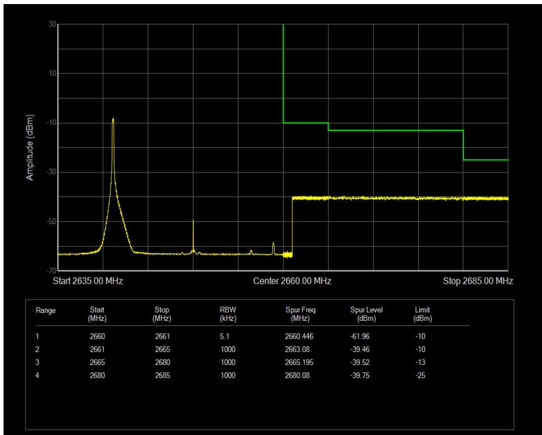
Band41 QPSK BW=20MHz Channel=41190 RB Size=100 Position=#0
