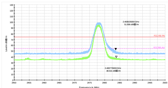
2478MHz-Channel 27 Peak+ Average
