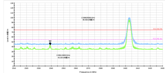
2403MHz-Channel 2 Peak+ Average
