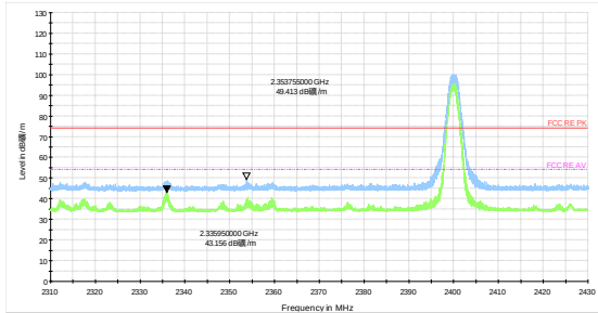
2400MHz-Channel 1 Peak+ Average
