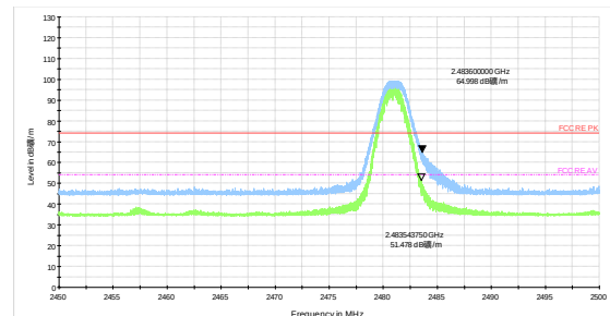
2481MHz-Channel 28 Peak+ Average
