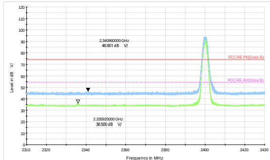
2400MHz-Channel 1 Peak+ Average
