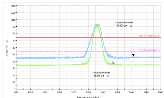
2478MHz-Channel 27 Peak+ Average
