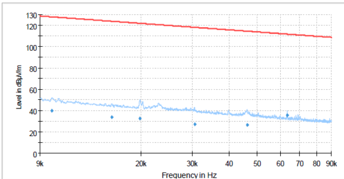
Radiates Emission from 9KHz to 90KHz
