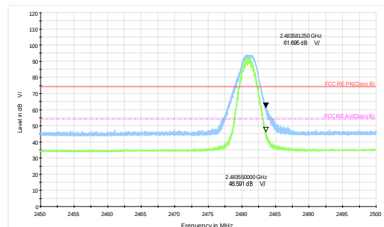
2481MHz-Channel 28 Peak+ Average
