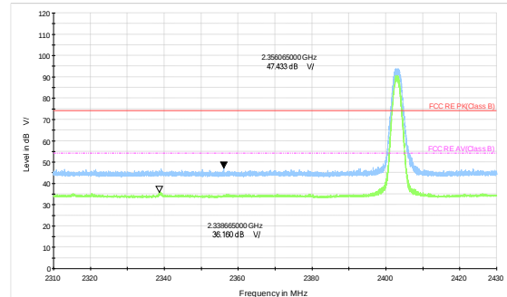
2403MHz-Channel 2 Peak+ Average
