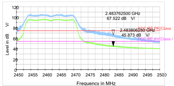
802.11g-Channel 11 Peak+ Average
