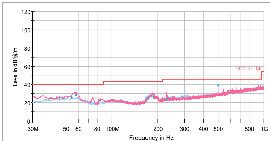
Radiates Emission from 30MHz to 1GHz
