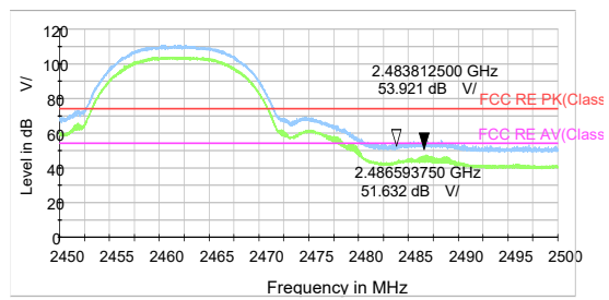
802.11b-Channel 11 Peak+ Average
