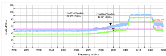
802.11n HT20 -Channel 1 Peak+ Average
