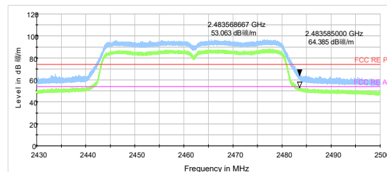
802.11n HT40 -Channel 9 Peak+ Average
