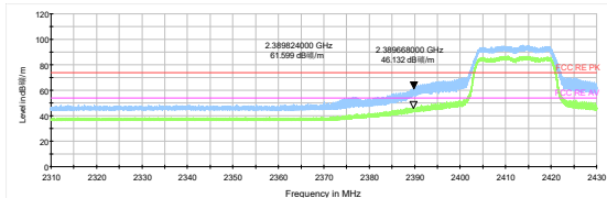
802.11g-Channel 1 Peak+ Average
