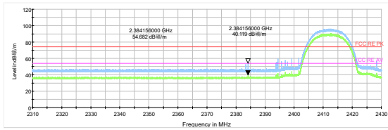
802.11b-Channel 1 Peak+ Average
