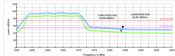
802.11g-Channel 11 Peak+ Average
