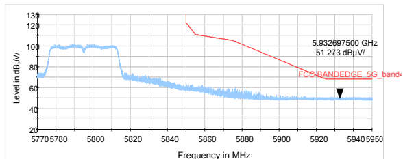
802.11n HT40-Channel 159: Peak
