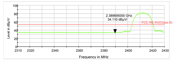
802.11b-Channel 1 Average
