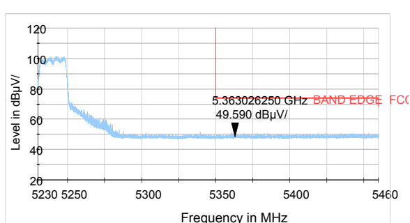
802.11n HT20-Channel 48: Peak
