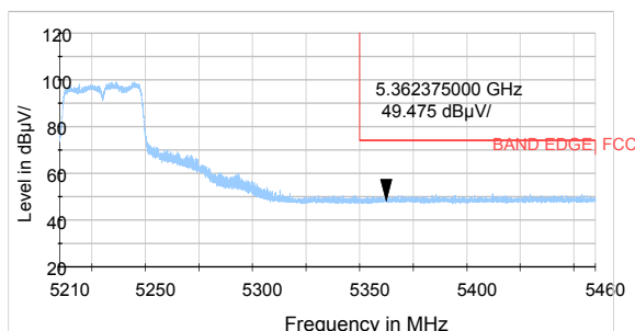
802.11n HT40-Channel 46: Peak
