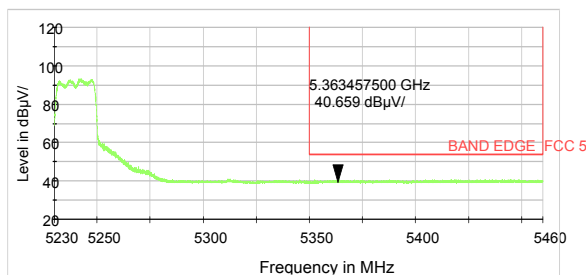
802.11n HT40-Channel 46: Peak
