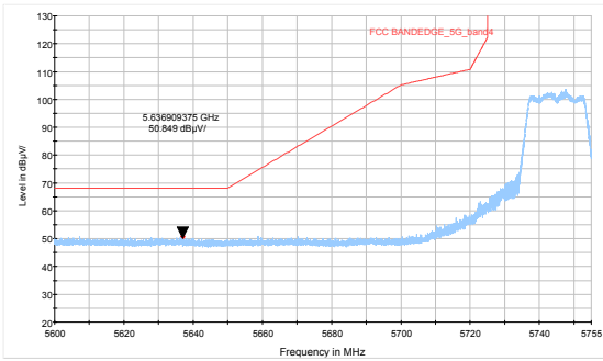
802.11a-Channel 149: Peak
