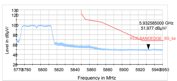
802.11n HT40-Channel 159: Peak
