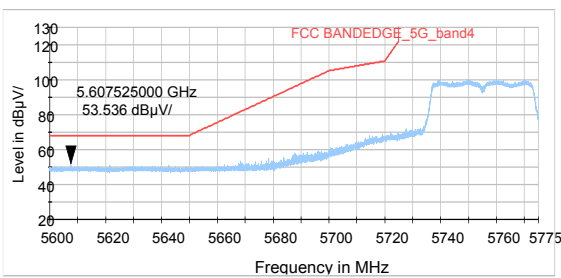
802.11ac VHT80- Channel 155: Peak
