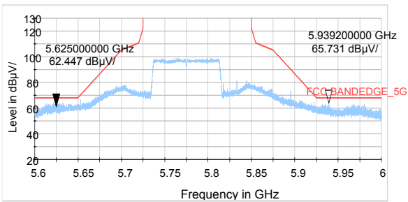
802.11ac VHT80- Channel 155: Peak
