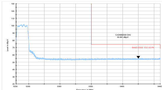
802.11a-Channel 48: Peak
