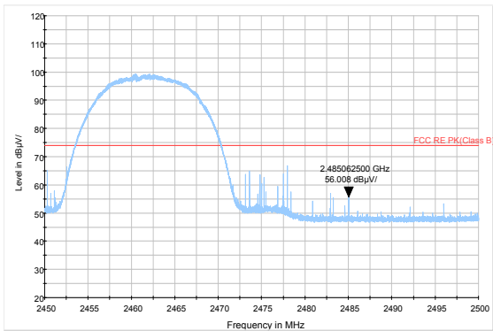
802.11b-Channel 11 Peak
