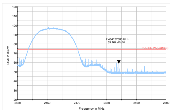
802.11b-Channel 11 Peak
