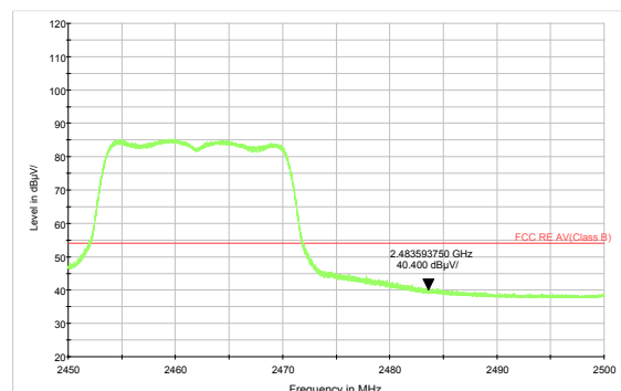
802.11g-Channel 11 Average
