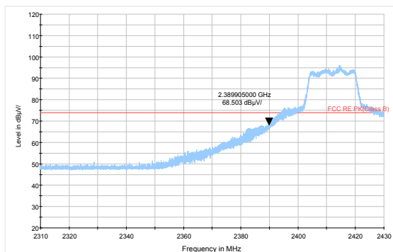
802.11g-Channel 1 Peak
