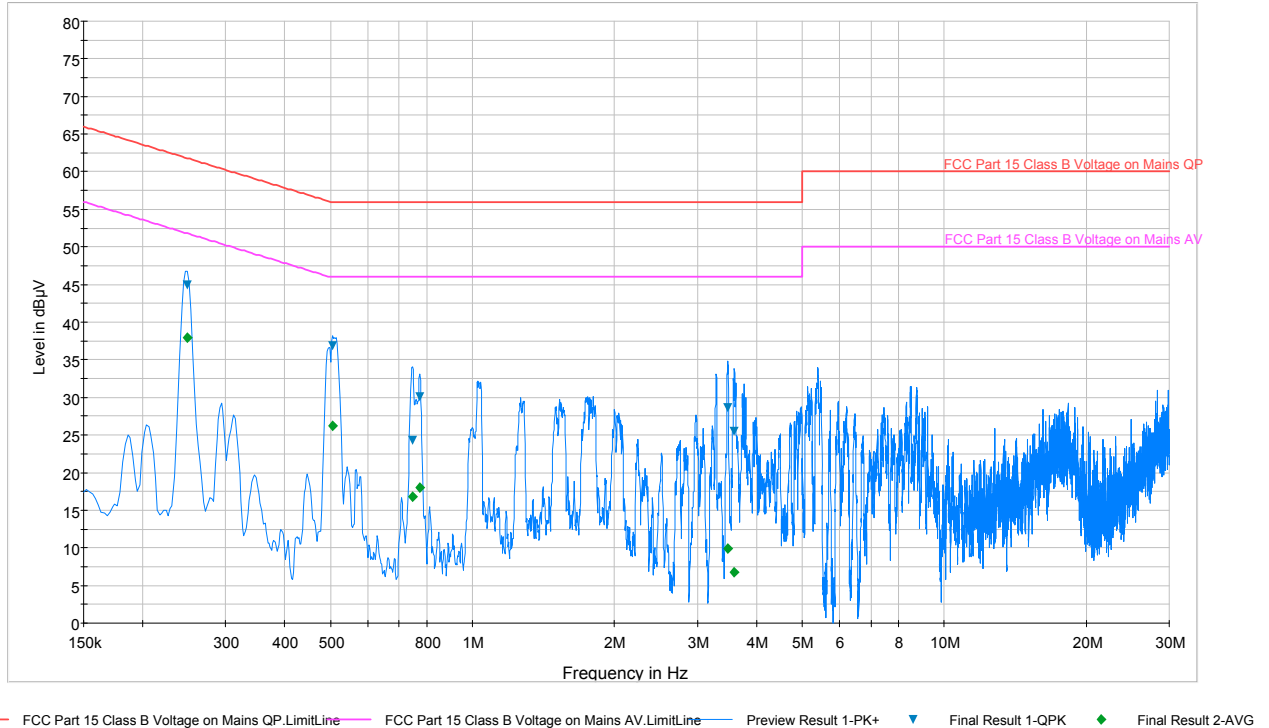
Plot 6-3. Line-Conducted Test Plot (N)
