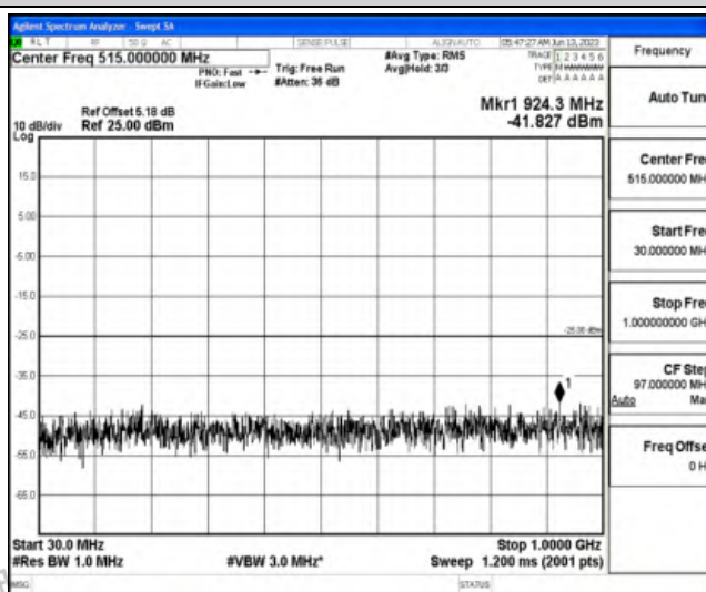
Band38-5MHz-QPSK-38225-1RB#0-Range3:30~1000MHz
