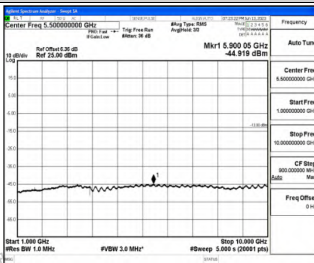
Band26-1.4MHz-16QAM-26740-1RB#0-Range4:1000~10000MHz
