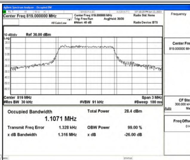
Band26-1.4MHz-16QAM-26740-6RB#0
