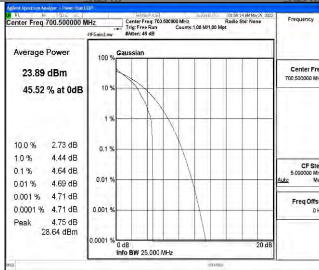
Band12-3MHz-QPSK-23025-15RB#0
