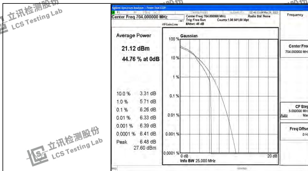
Band12-10MHz-16QAM-23060-50RB#0
