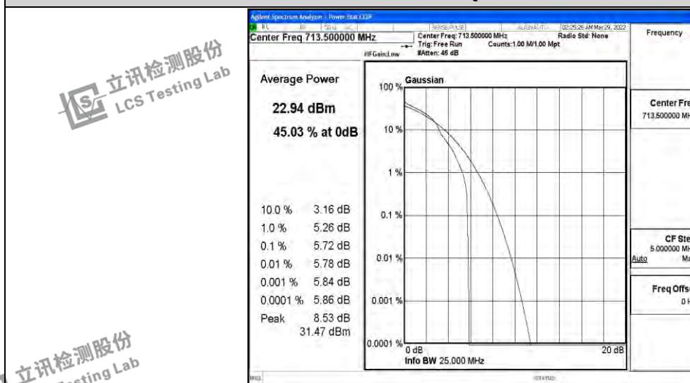
Band12-5MHz-16QAM-23155-1RB#0
