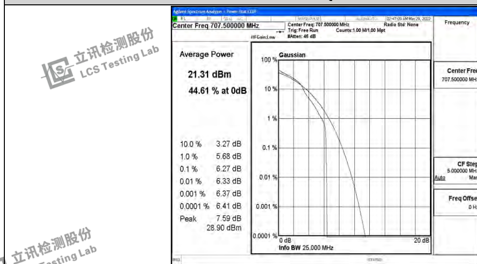
Band12-10MHz-16QAM-23095-1RB#0
