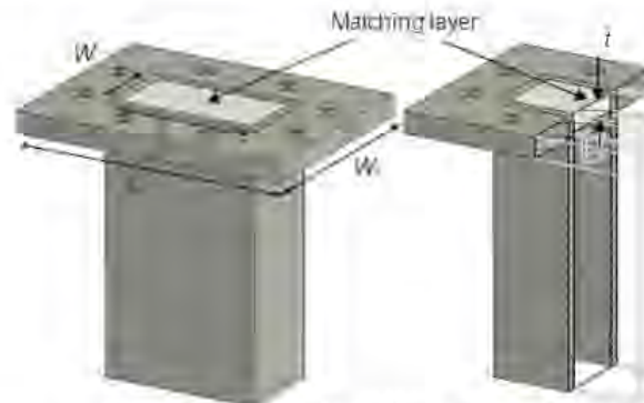
Figure 1: Validation Waveguide Dimensions
