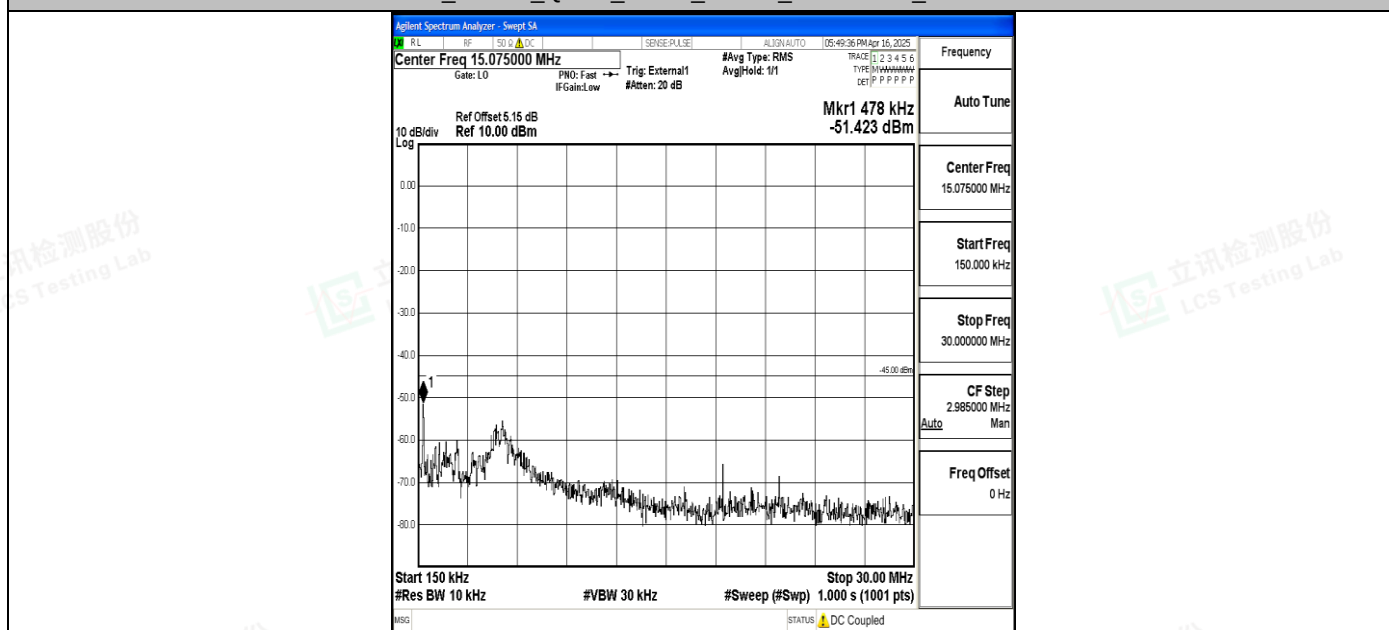
Band41_20MHz_QPSK_40620_1RB#0_0.15~30_0.15~30
