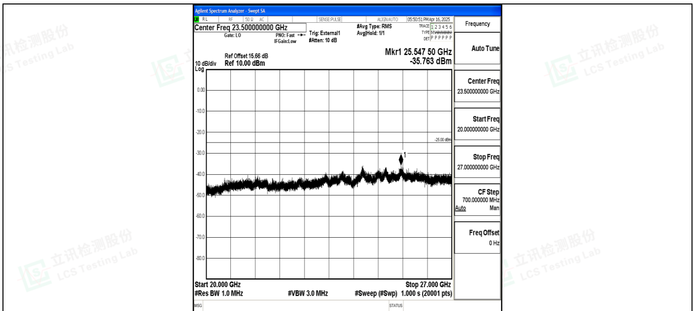
Band41_20MHz_QPSK_40620_1RB#0_20000~27000_20000~27000
