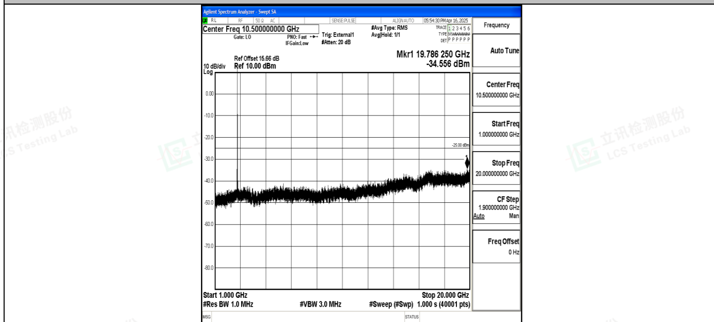
Band41_20MHz_QPSK_41490_1RB#0_1000~20000_1000~20000
