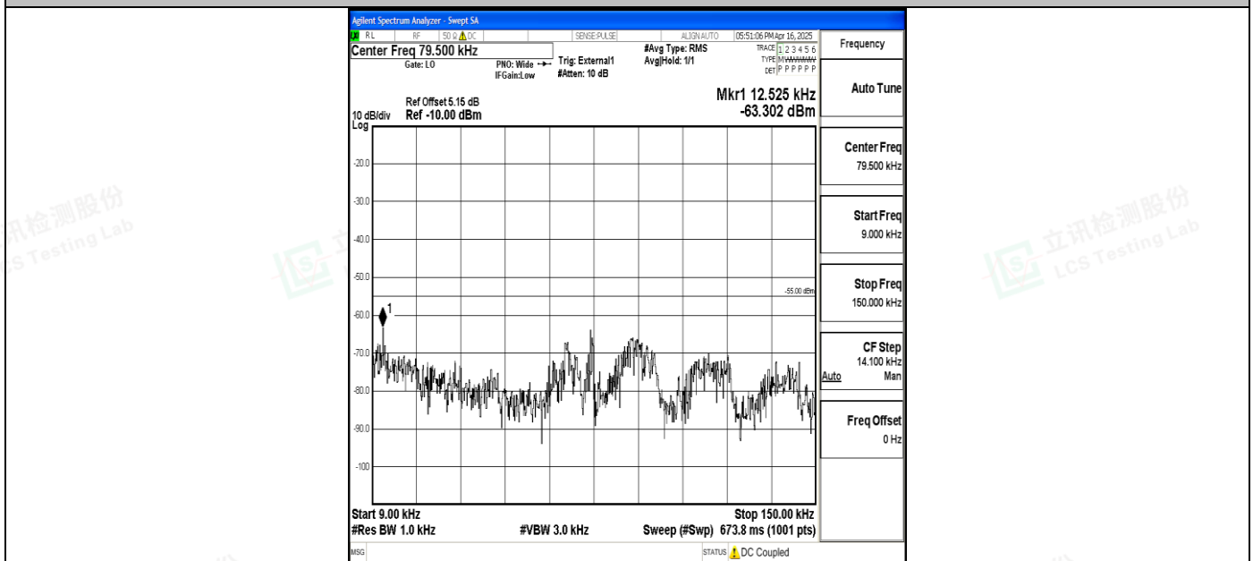
Band41_20MHz_16QAM_40620_1RB#0_0.009~0.15_0.009~0.15
