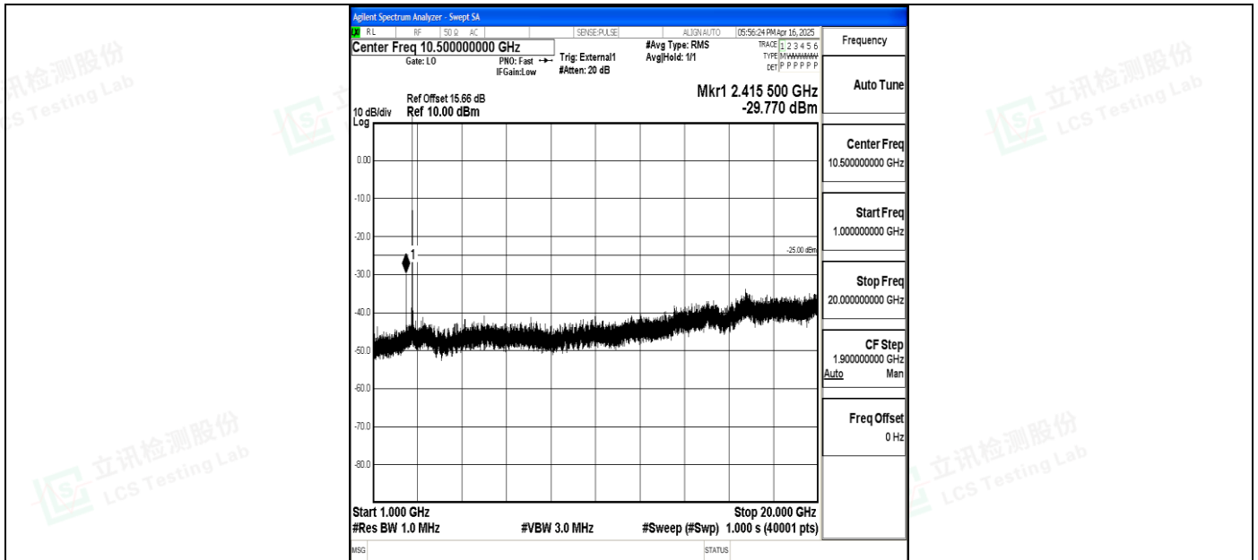
Band41_20MHz_16QAM_41490_1RB#0_1000~20000_1000~20000
