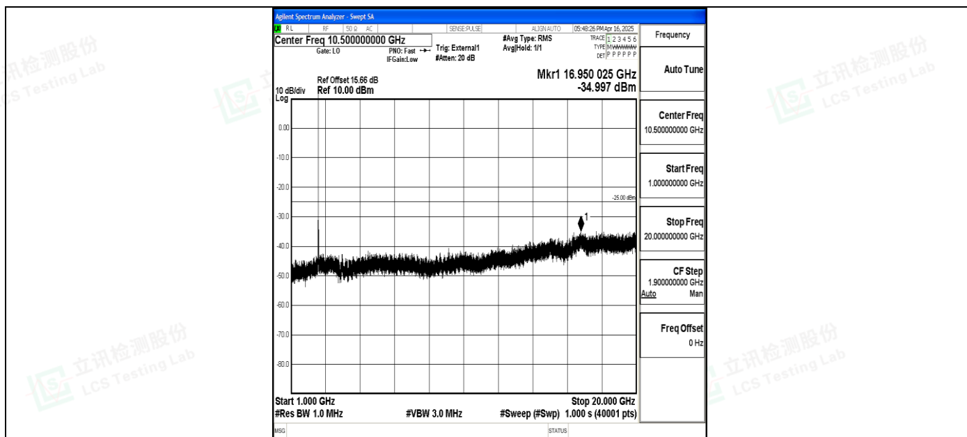
Band41_20MHz_16QAM_39750_1RB#0_1000~20000_1000~20000
