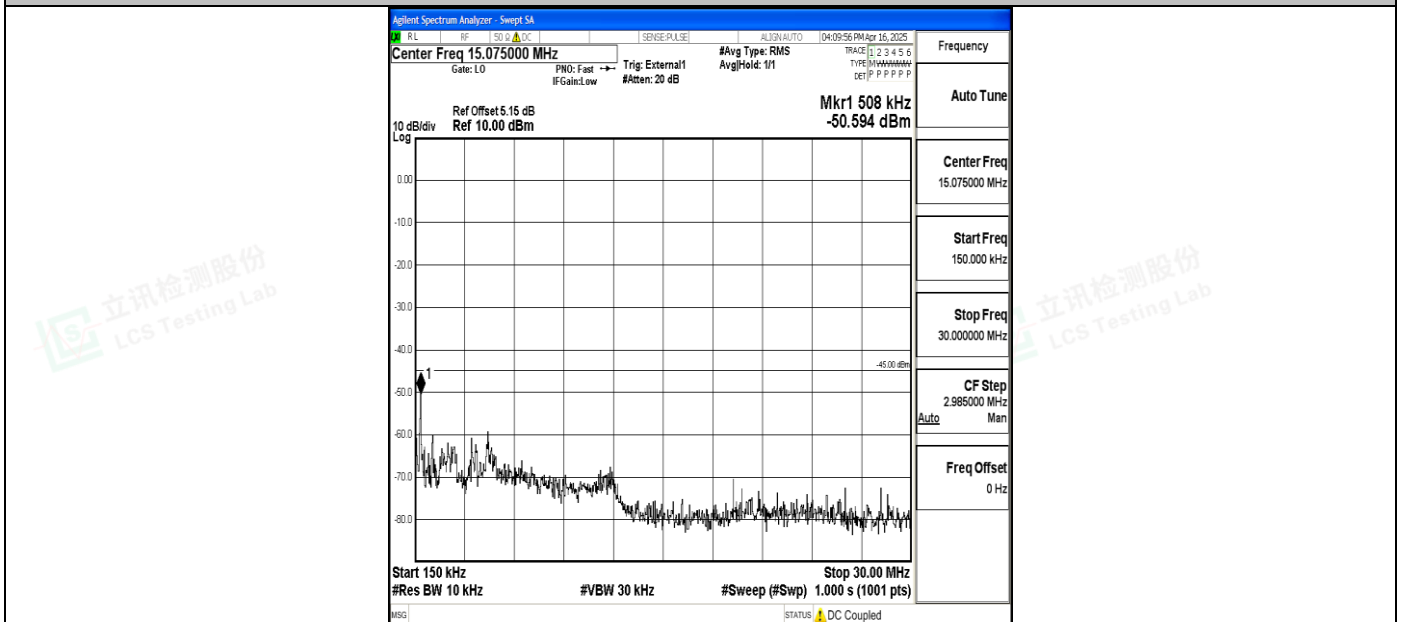
Band41_5MHz_QPSK_39675_1RB#0_0.15~30_0.15~30
