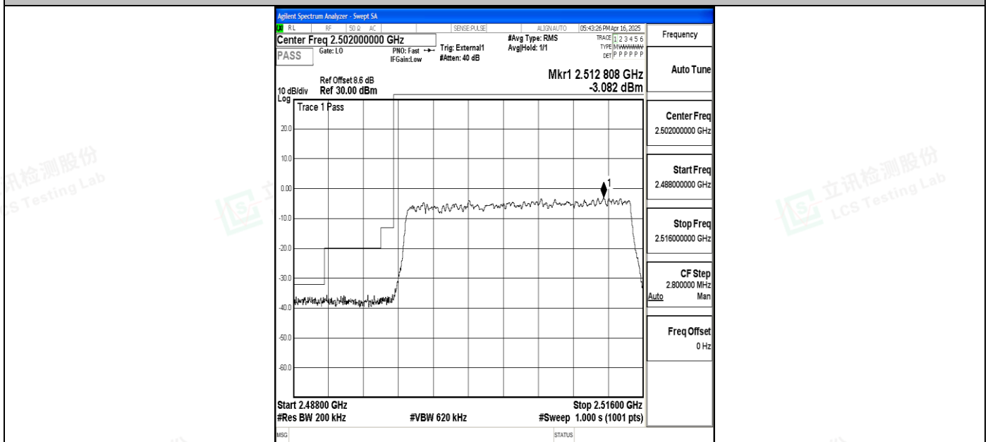
Band41_20MHz_QPSK_39750_100RB#0
