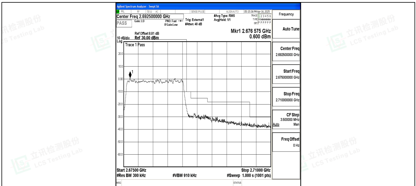
Band41_15MHz_16QAM_41515_75RB#0
