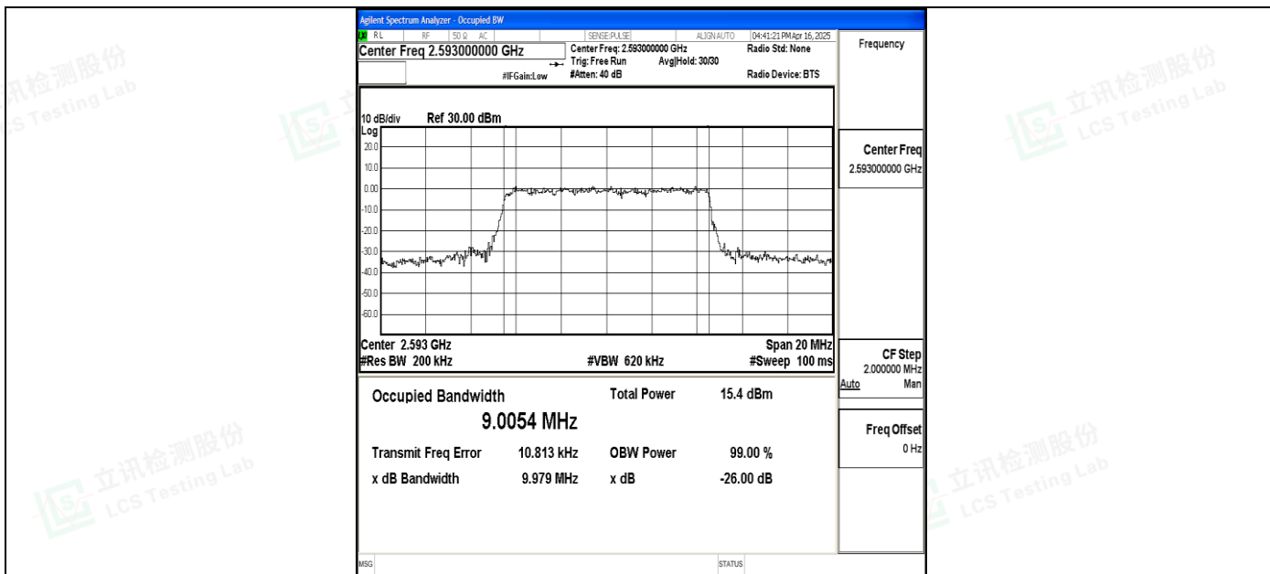
Band41-10MHz-QPSK-40620-50RB#0-PASS
