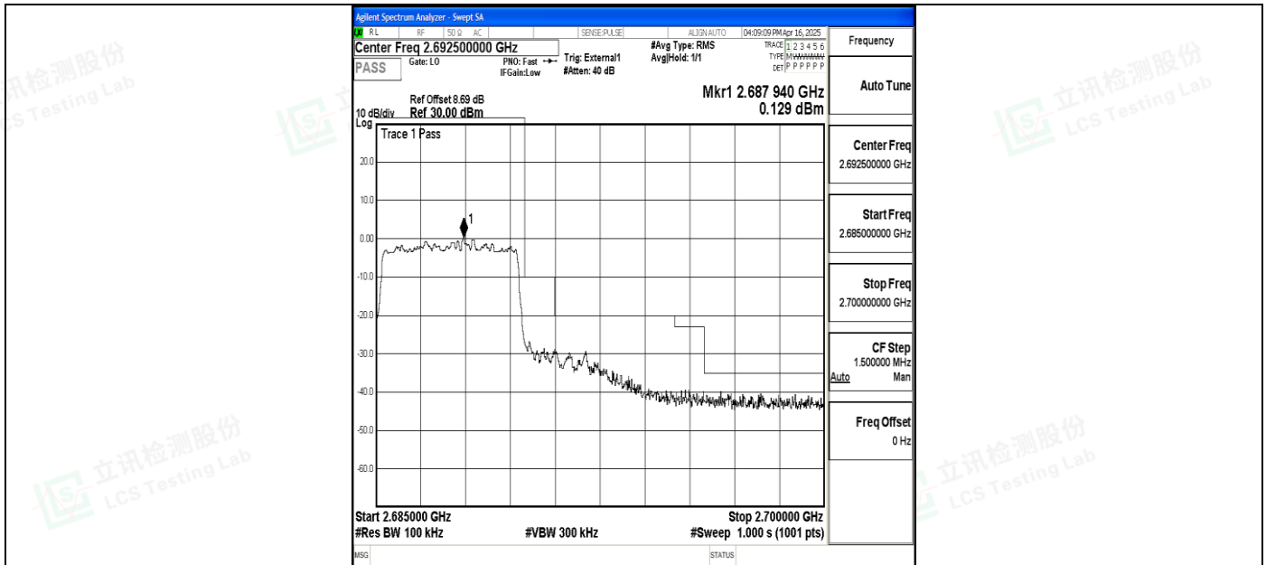
Band41_5MHz_16QAM_41565_25RB#0
