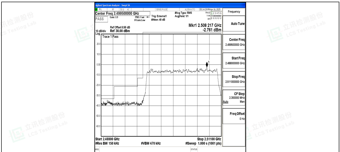
Band41_15MHz_16QAM_39725_75RB#0
