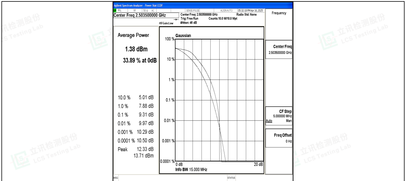
Band41-15MHz-QPSK-39725-75RB#0-PASS
