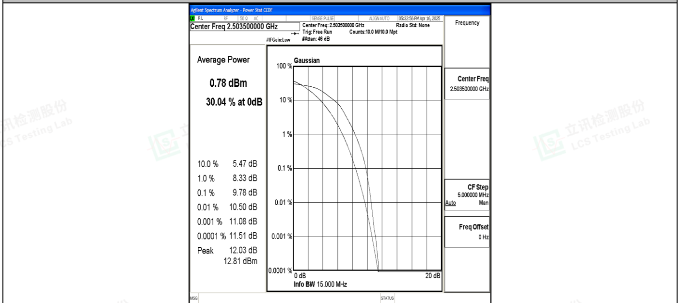
Band41-15MHz-16QAM-39725-75RB#0-PASS
