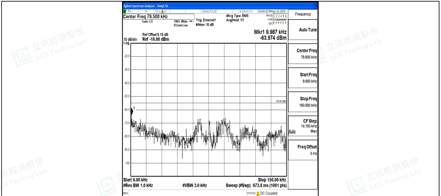
Band41_5MHz_QPSK_39675_1RB#0_0.009~0.15_0.009~0.15
