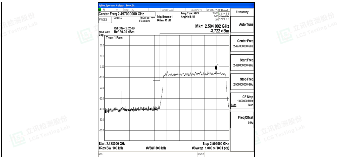
Band41_10MHz_16QAM_39700_50RB#0
