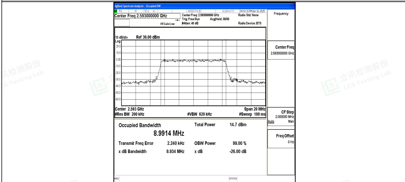
Band41-10MHz-16QAM-40620-50RB#0-PASS
