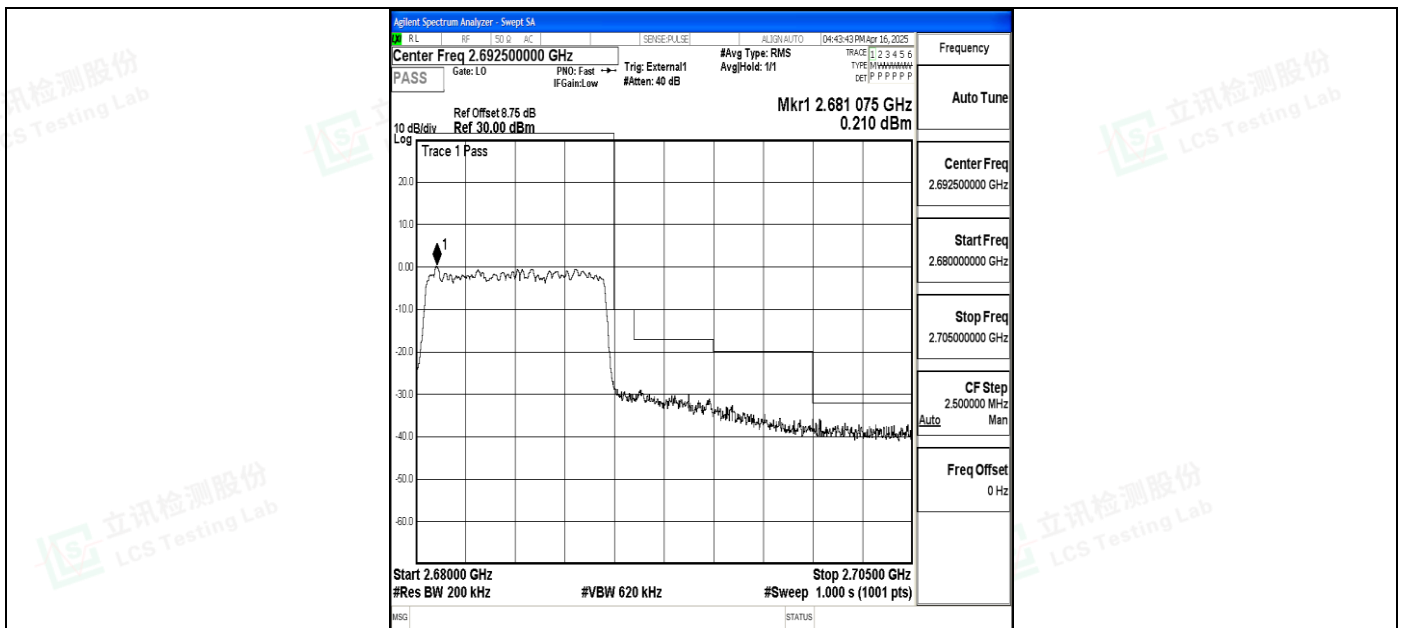
Band41_10MHz_16QAM_41540_50RB#0
