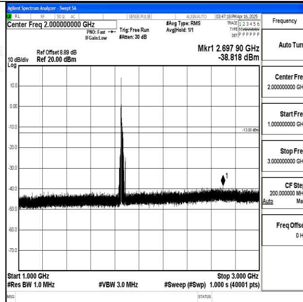
Band25_20MHz_16QAM_26140_1RB#0_1000~3000_1000~3000
