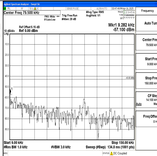
Band25_20MHz_QPSK_26365_1RB#0_0.009~0.15_0.009~0.15
