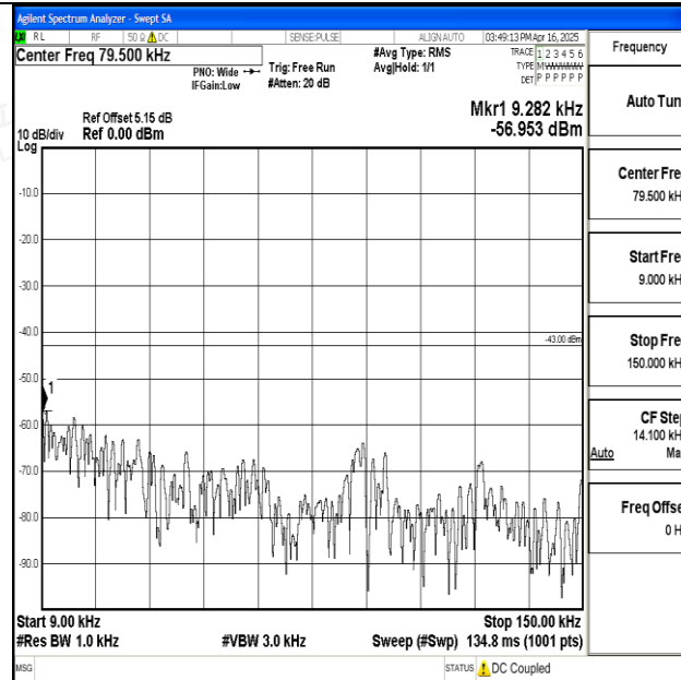
Band25_20MHz_QPSK_26590_1RB#0_0.009~0.15_0.009~0.15
