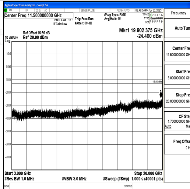
Band25_20MHz_QPSK_26365_1RB#0_3000~20000_3000~20000
