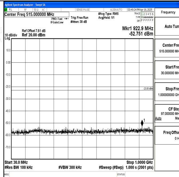
Band25_20MHz_QPSK_26590_1RB#0_30~1000_30~1000
