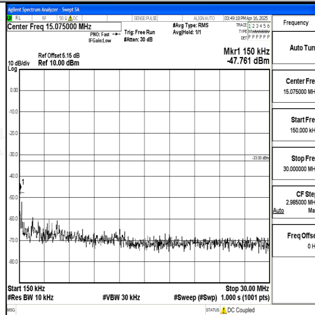
Band25_20MHz_QPSK_26590_1RB#0_0.15~30_0.15~30
