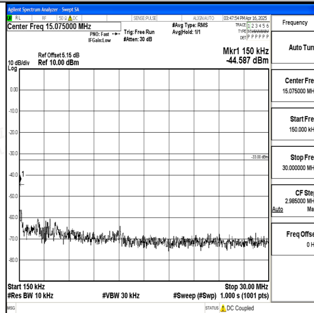
Band25_20MHz_QPSK_26365_1RB#0_0.15~30_0.15~30
