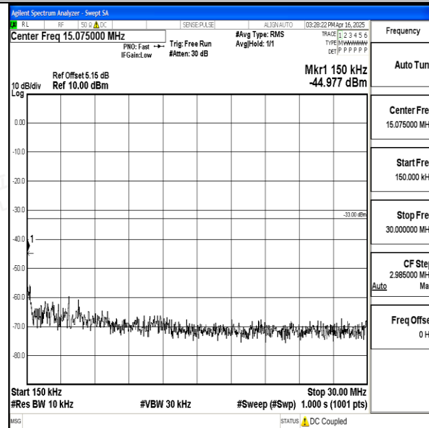
Band25_15MHz_QPSK_26365_1RB#0_0.15~30_0.15~30
