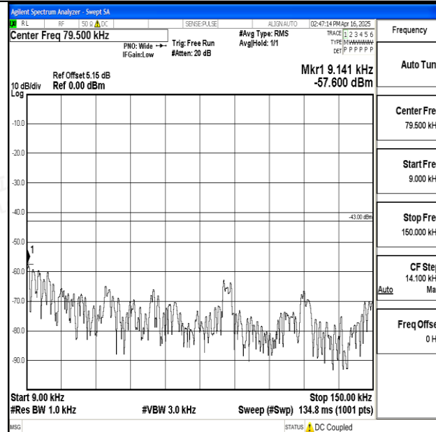
Band25_5MHz_16QAM_26665_1RB#0_0.009~0.15_0.009~0.15
