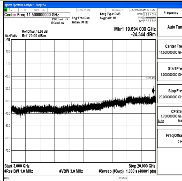
Band25_15MHz_QPSK_26615_1RB#0_3000~20000_3000~20000
