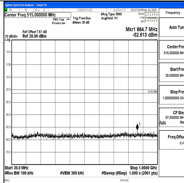
Band25_15MHz_QPSK_26115_1RB#0_30~1000_30~1000
