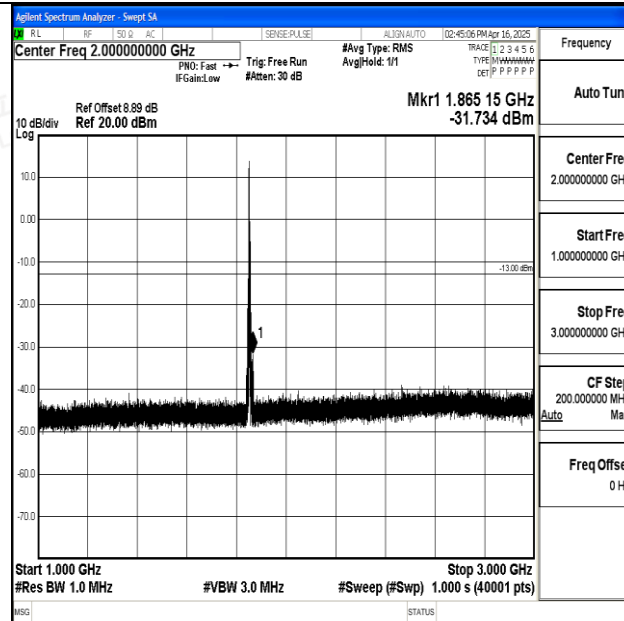
Band25_5MHz_16QAM_26065_1RB#0_1000~3000_1000~3000
