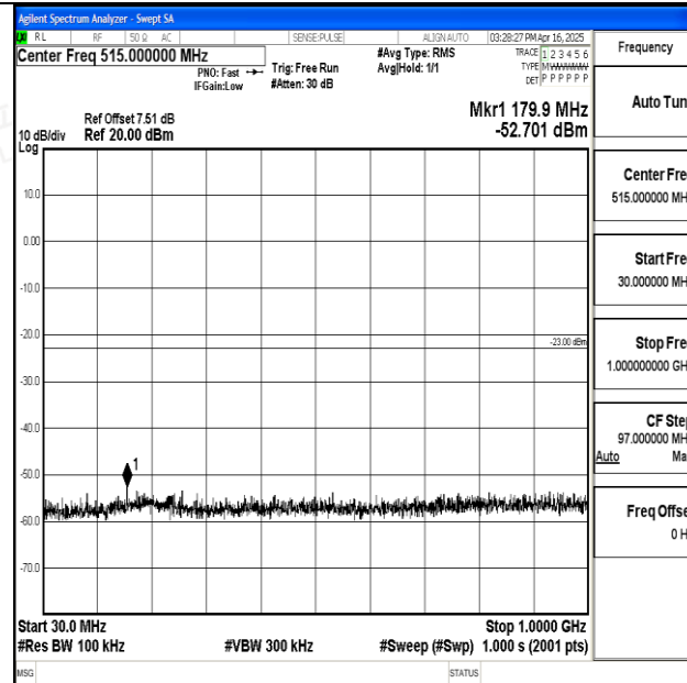
Band25_15MHz_QPSK_26365_1RB#0_30~1000_30~1000
