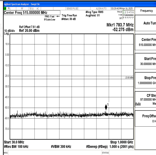
Band25_15MHz_QPSK_26615_1RB#0_30~1000_30~1000
