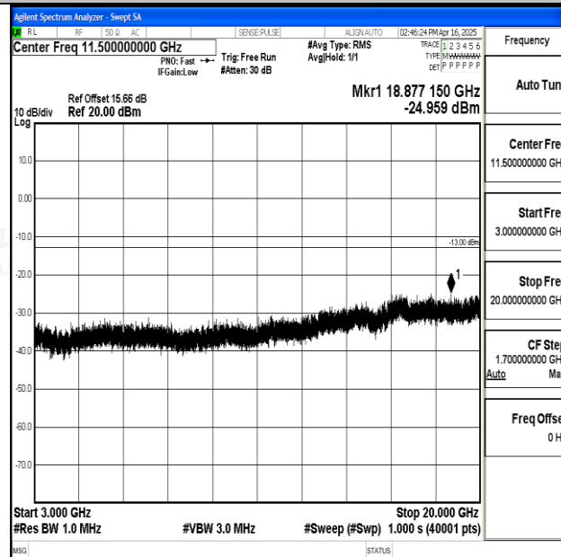
Band25_5MHz_16QAM_26365_1RB#0_3000~20000_3000~20000
