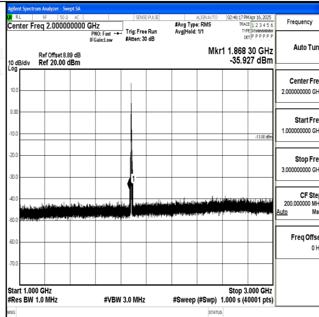
Band25_5MHz_16QAM_26365_1RB#0_1000~3000_1000~3000
