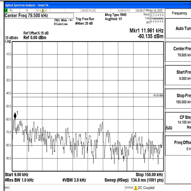
Band25_15MHz_QPSK_26365_1RB#0_0.009~0.15_0.009~0.15
