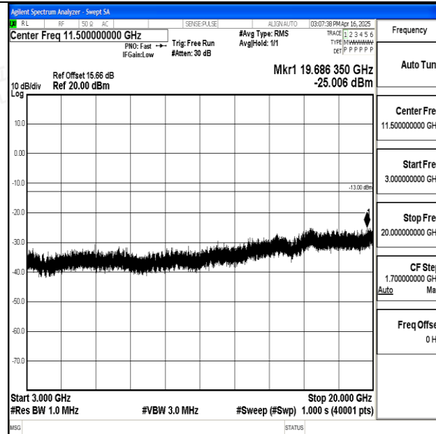
Band25_10MHz_QPSK_26640_1RB#0_3000~20000_3000~20000
