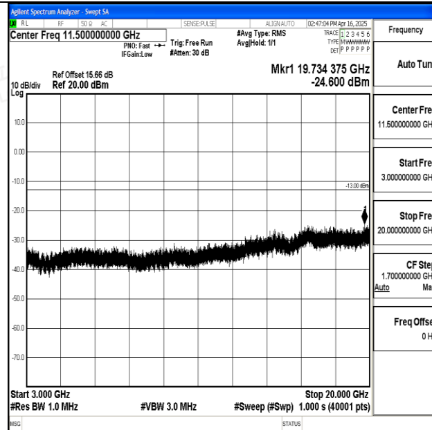
Band25_5MHz_QPSK_26665_1RB#0_3000~20000_3000~20000
