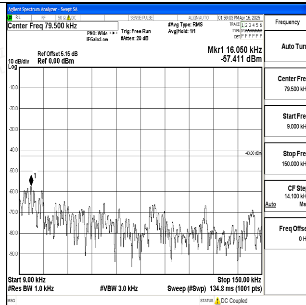
Band25_1.4MHz_QPSK_26365_1RB#0_0.009~0.15_0.009~0.15
