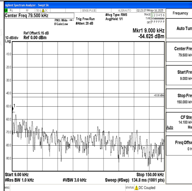
Band25_3MHz_QPSK_26365_1RB#0_0.009~0.15_0.009~0.15
