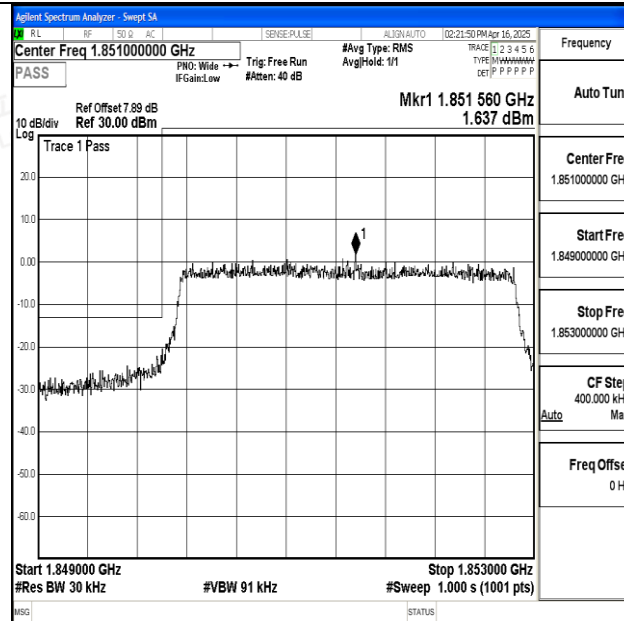
Band25_3MHz_QPSK_26055_15RB#0
