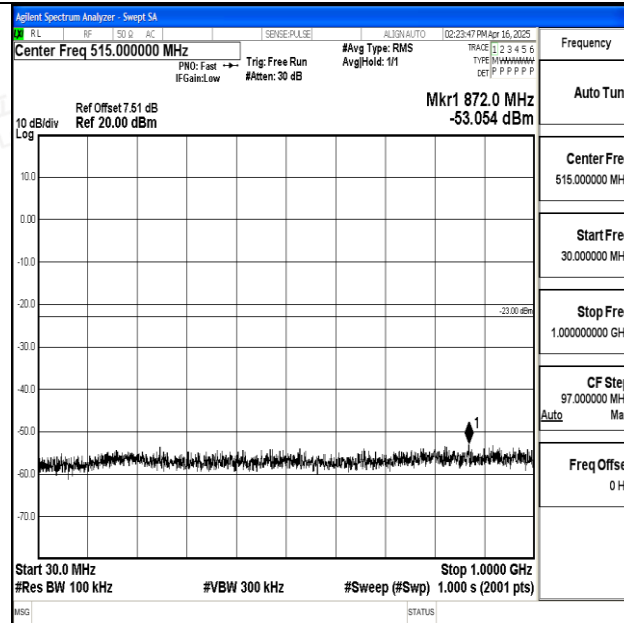
Band25_3MHz_QPSK_26365_1RB#0_30~1000_30~1000
