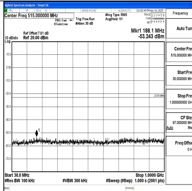
Band25_1.4MHz_QPSK_26683_1RB#0_30~1000_30~1000
