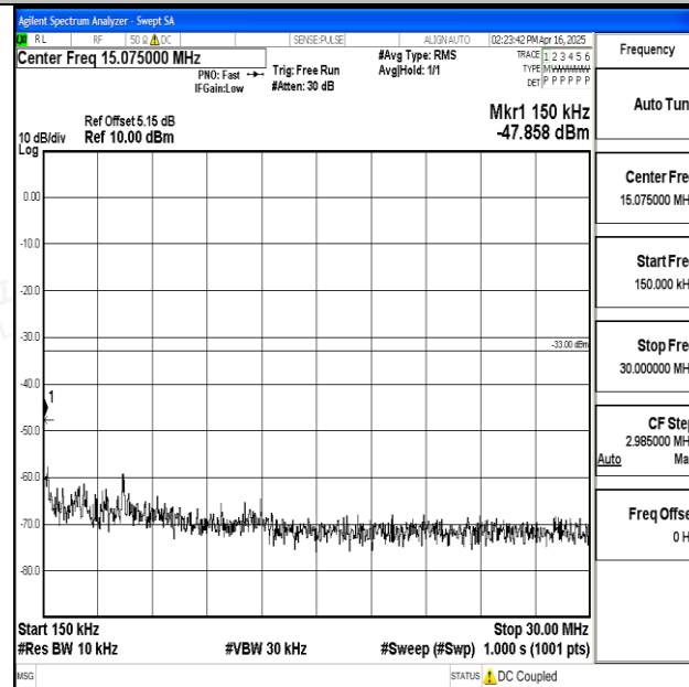
Band25_3MHz_QPSK_26365_1RB#0_0.15~30_0.15~30
