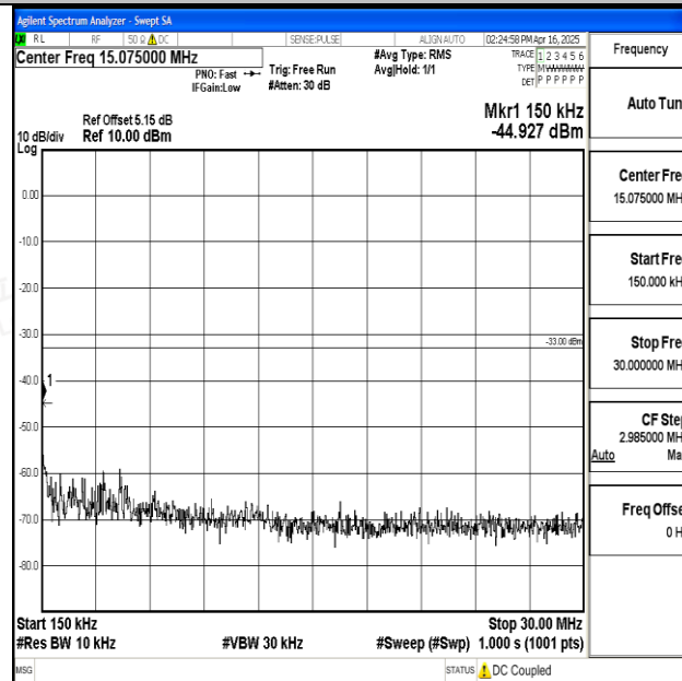
Band25_3MHz_QPSK_26675_1RB#0_0.15~30_0.15~30
