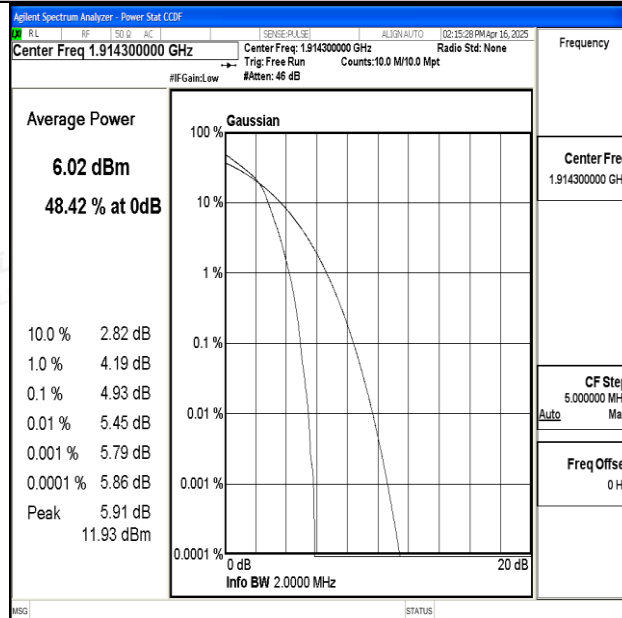
Band25-1.4MHz-16QAM-26683-6RB#0-PASS
