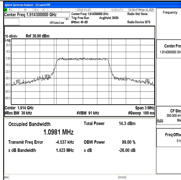
Band25-1.4MHz-QPSK-26683-6RB#0-PASS
