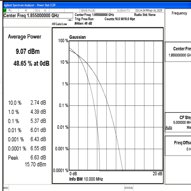
Band25-10MHz-16QAM-26090-50RB#0-PASS
