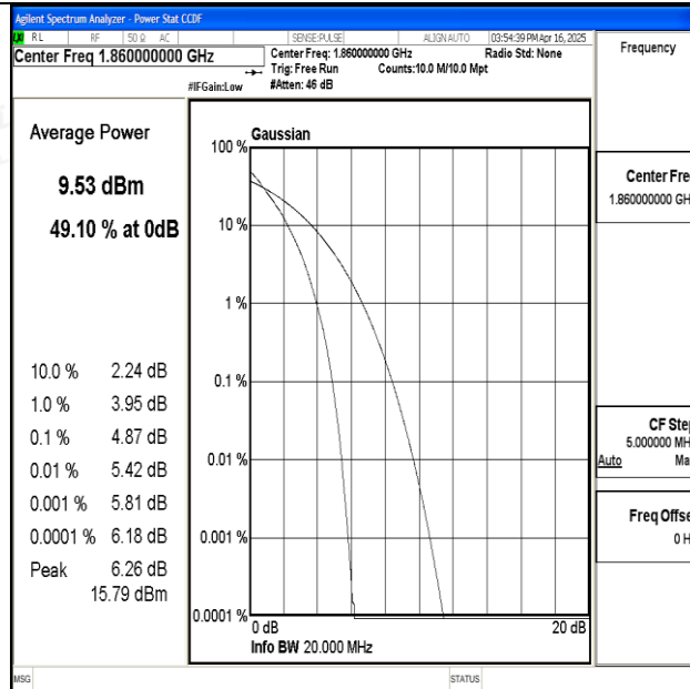
Band25-20MHz-QPSK-26140-100RB#0-PASS
