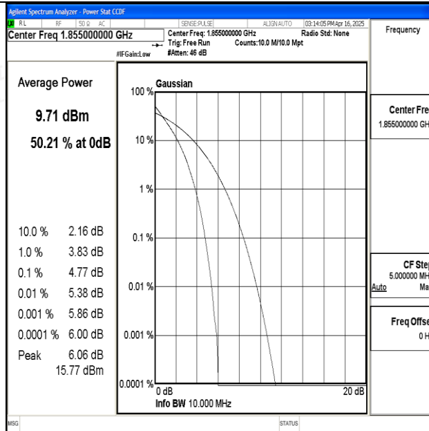
Band25-10MHz-QPSK-26090-50RB#0-PASS
