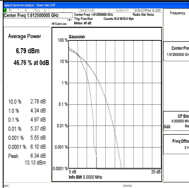
Band25-5MHz-16QAM-26665-1RB#0-PASS
