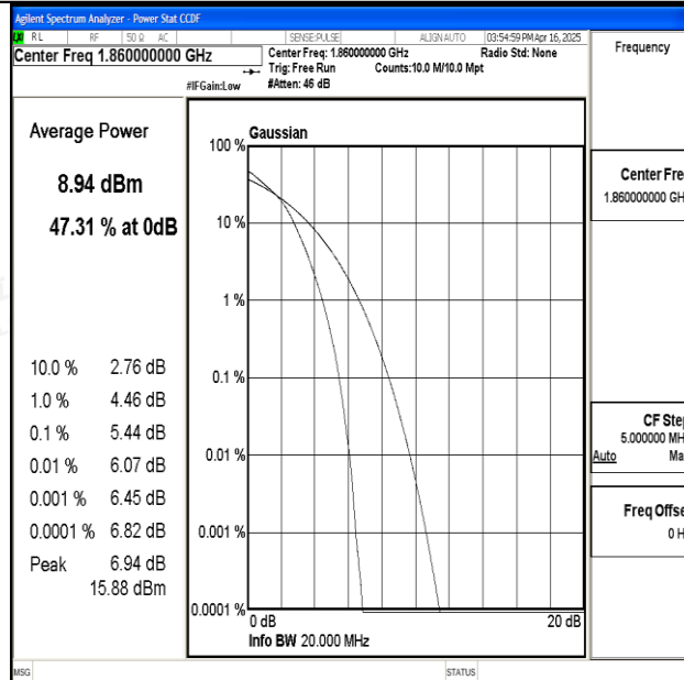
Band25-20MHz-16QAM-26140-100RB#0-PASS
