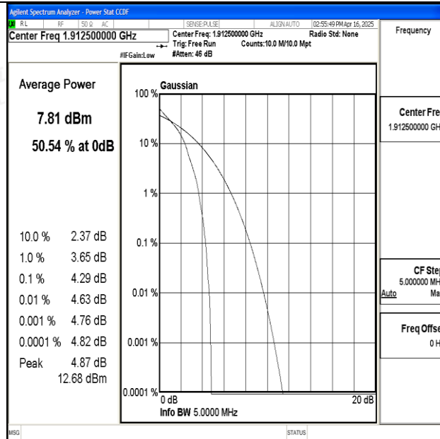
Band25-5MHz-QPSK-26665-1RB#0-PASS
