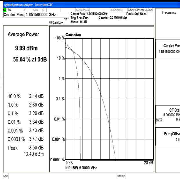
Band25-3MHz-16QAM-26055-1RB#0-PASS
