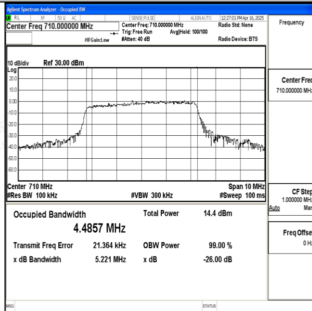
Band17-5MHz-16QAM-23790-25RB#0-PASS
