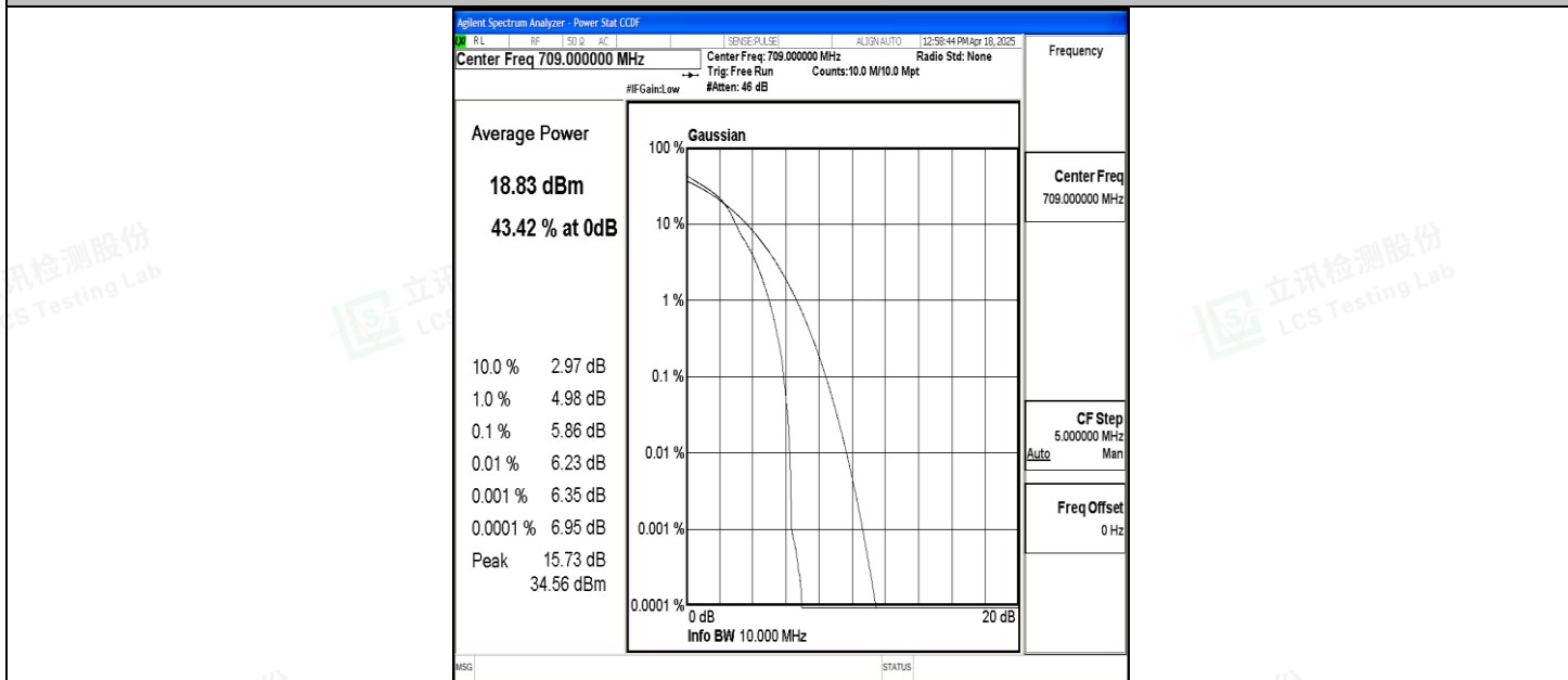
Band17-10MHz-16QAM-23780-1RB#0-PASS
