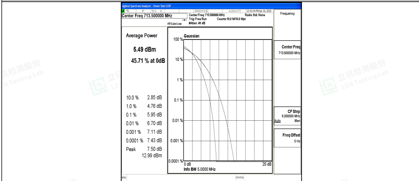
Band17-5MHz-16QAM-23825-25RB#0-PASS
