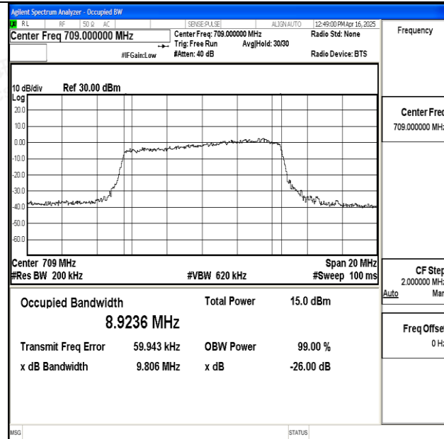
Band17-10MHz-QPSK-23780-50RB#0-PASS
