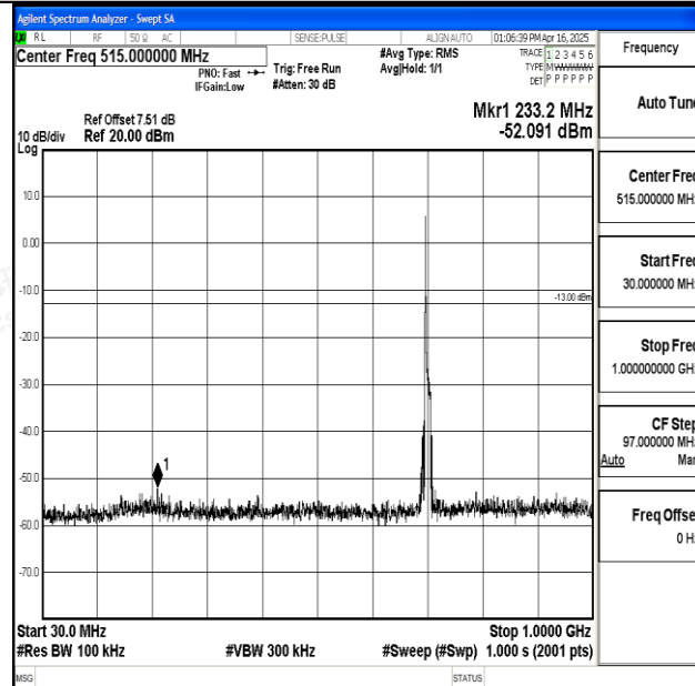
Band17_10MHz_16QAM_23780_1RB#0_30~1000_30~1000
