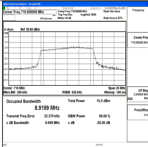
Band17-10MHz-QPSK-23790-50RB#0-PASS
