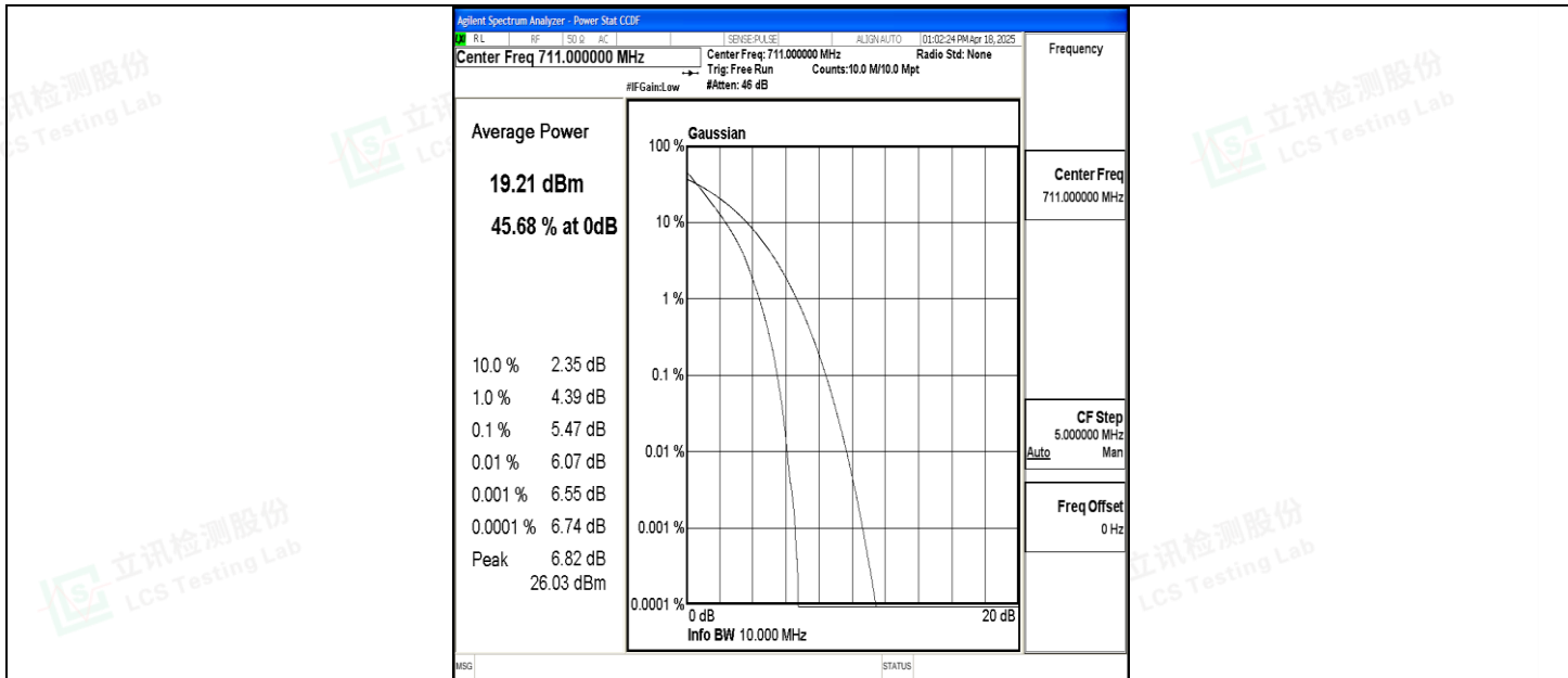
Band17-10MHz-QPSK-23800-50RB#0-PASS
