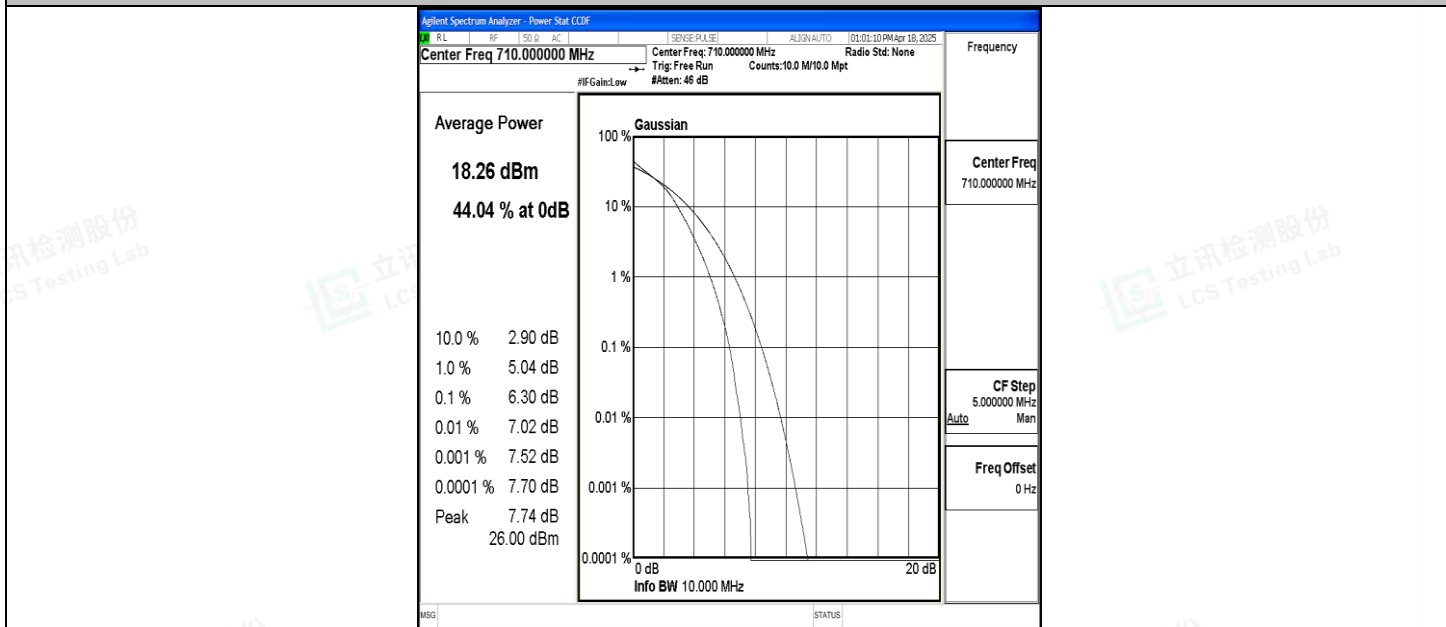
Band17-10MHz-16QAM-23790-50RB#0-PASS
