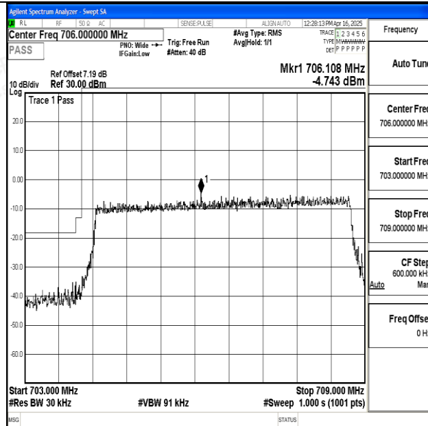
Band17_5MHz_16QAM_23755_25RB#0
