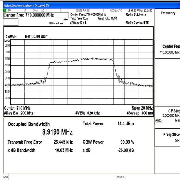
Band17-10MHz-16QAM-23790-50RB#0-PASS
