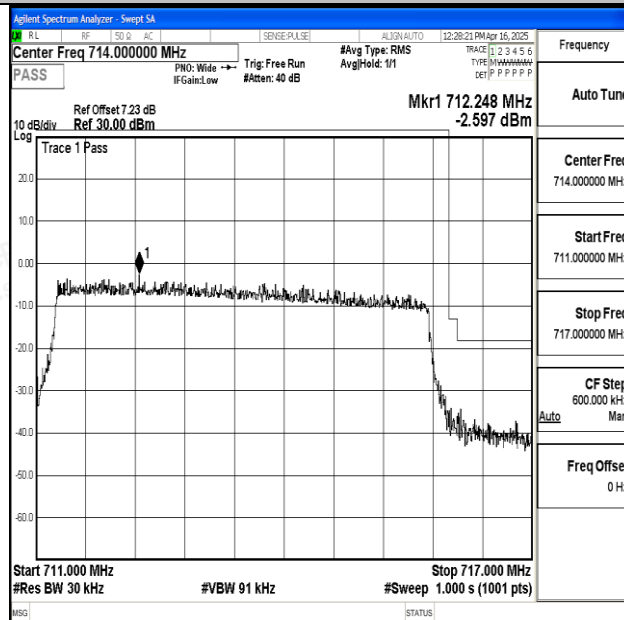
Band17_5MHz_QPSK_23825_25RB#0
