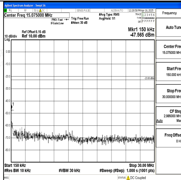
Band17_5MHz_QPSK_23755_1RB#0_0.15~30_0.15~30
