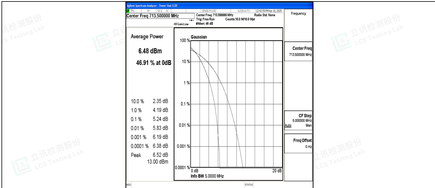
Band17-5MHz-QPSK-23825-25RB#0-PASS
