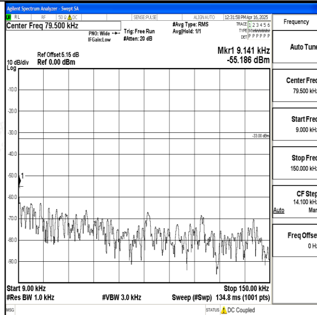
Band17_5MHz_16QAM_23825_1RB#0_0.009~0.15_0.009~0.15
