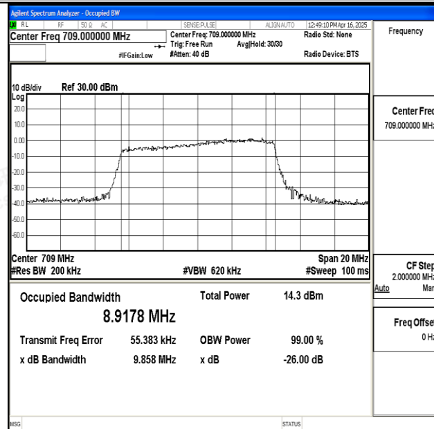
Band17-10MHz-16QAM-23780-50RB#0-PASS
