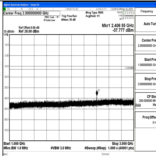
Band12_10MHz_QPSK_23130_1RB#0_1000~3000_1000~3000
