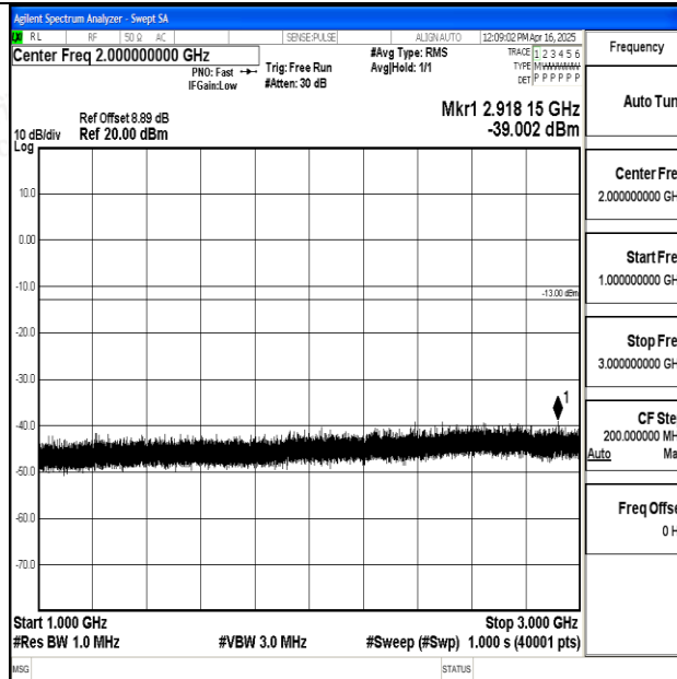
Band12_10MHz_16QAM_23095_1RB#0_1000~3000_1000~3000
