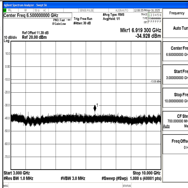
Band12_10MHz_QPSK_23095_1RB#0_3000~10000_3000~10000
