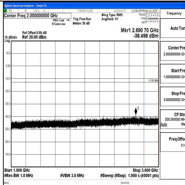
Band12_10MHz_QPSK_23095_1RB#0_1000~3000_1000~3000
