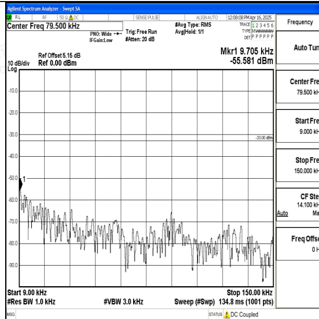
Band12_10MHz_QPSK_23095_1RB#0_0.009~0.15_0.009~0.15
