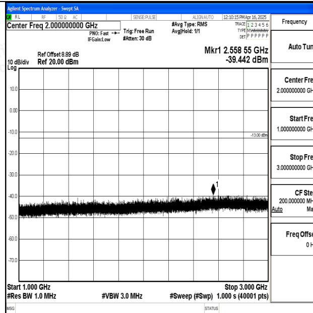
Band12_10MHz_16QAM_23130_1RB#0_1000~3000_1000~3000
