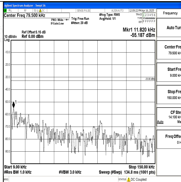
Band12_10MHz_QPSK_23130_1RB#0_0.009~0.15_0.009~0.15
