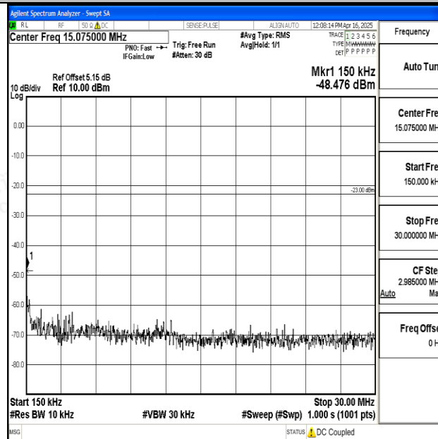
Band12_10MHz_QPSK_23095_1RB#0_0.15~30_0.15~30
