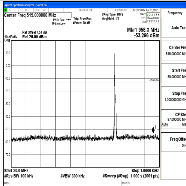
Band12_10MHz_QPSK_23130_1RB#0_30~1000_30~1000
