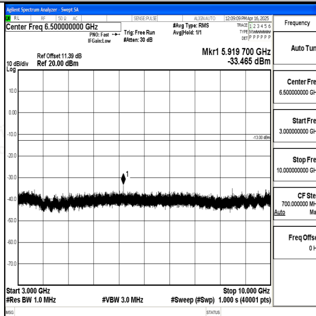
Band12_10MHz_16QAM_23095_1RB#0_3000~10000_3000~10000
