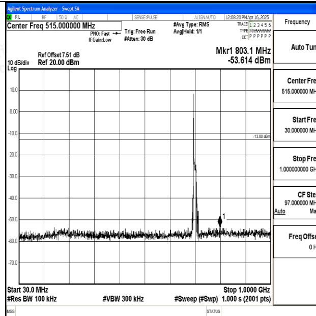
Band12_10MHz_QPSK_23095_1RB#0_30~1000_30~1000
