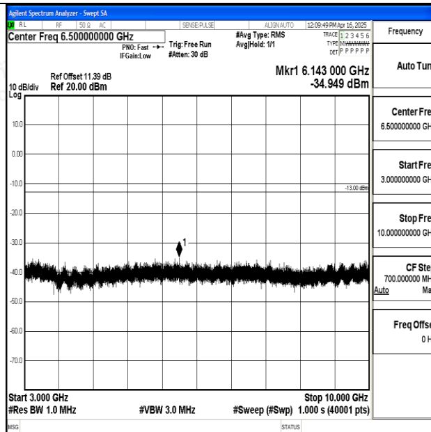
Band12_10MHz_QPSK_23130_1RB#0_3000~10000_3000~10000
