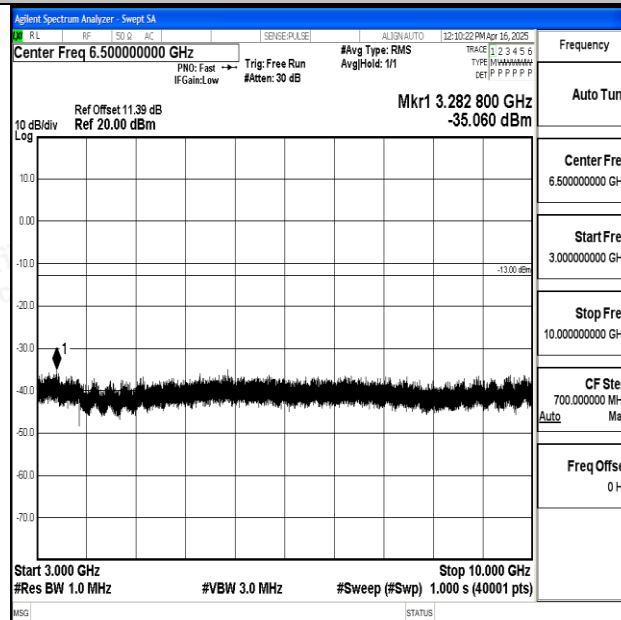
Band12_10MHz_16QAM_23130_1RB#0_3000~10000_3000~10000
