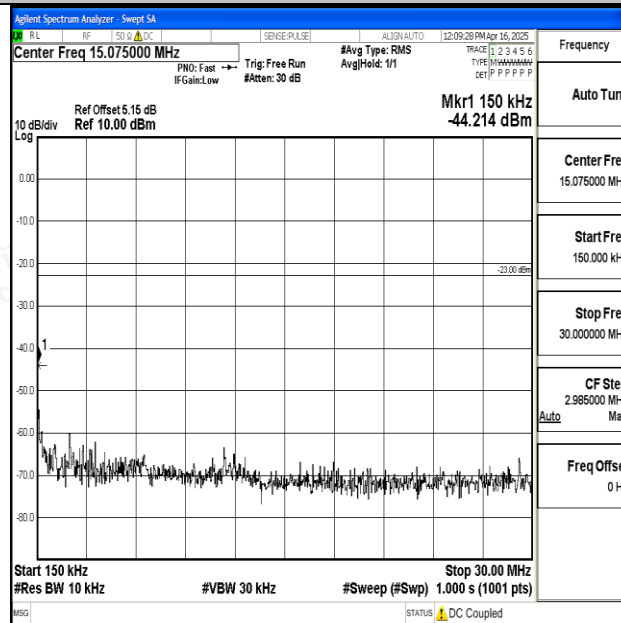
Band12_10MHz_QPSK_23130_1RB#0_0.15~30_0.15~30
