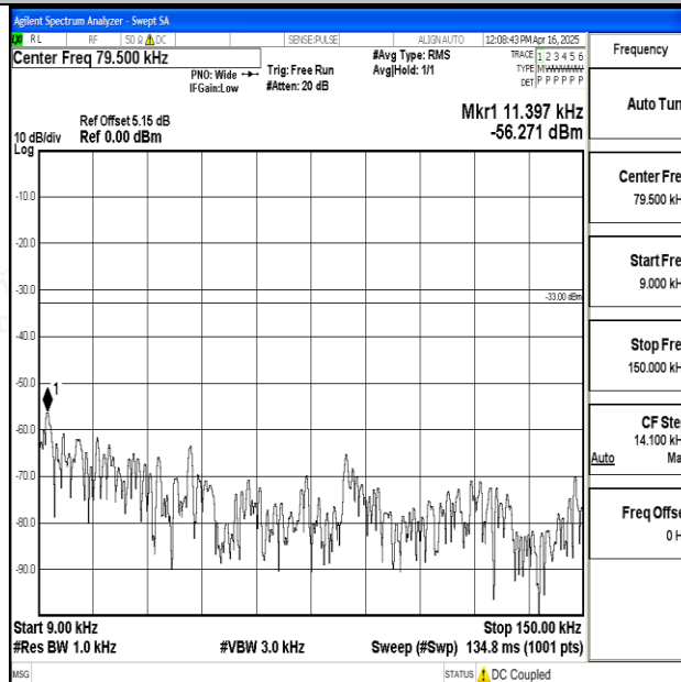
Band12_10MHz_16QAM_23095_1RB#0_0.009~0.15_0.009~0.15
