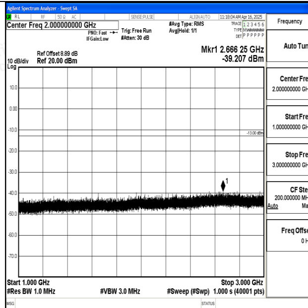
Band12_3MHz_16QAM_23025_1RB#0_1000~3000_1000~3000
