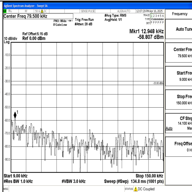
Band12_10MHz_16QAM_23060_1RB#0_0.009~0.15_0.009~0.15
