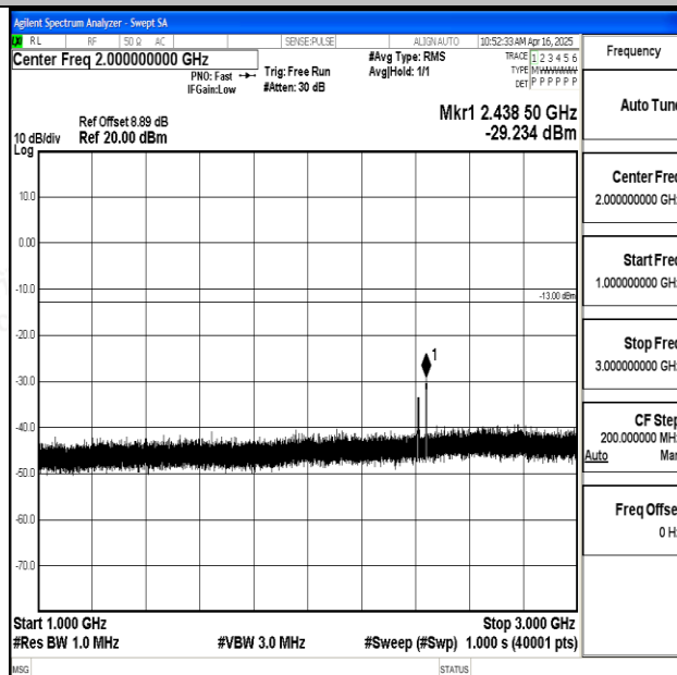
Band12_1.4MHz_QPSK_23173_1RB#0_1000~3000_1000~3000
