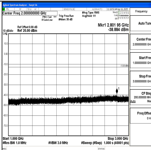
Band12_3MHz_QPSK_23095_1RB#0_1000~3000_1000~3000
