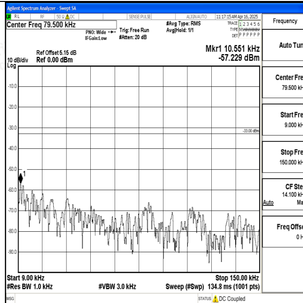
Band12_3MHz_QPSK_23025_1RB#0_0.009~0.15_0.009~0.15
