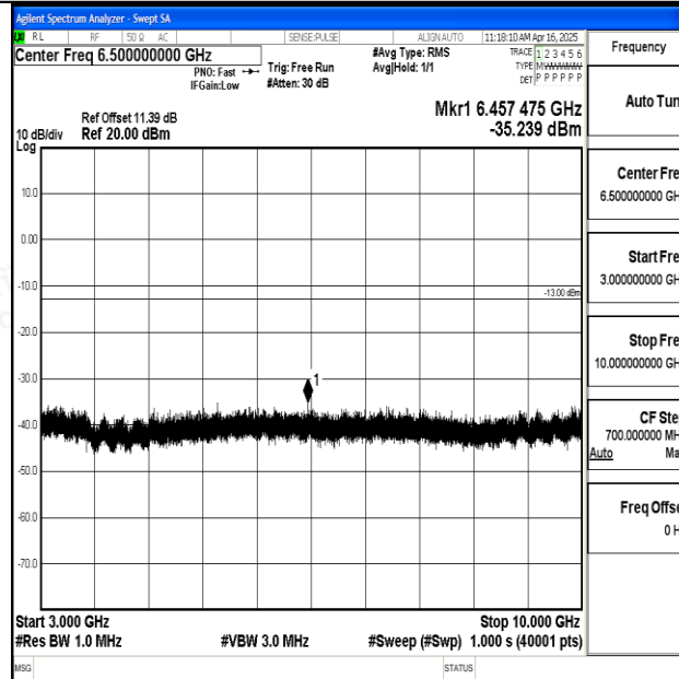
Band12_3MHz_16QAM_23025_1RB#0_3000~10000_3000~10000
