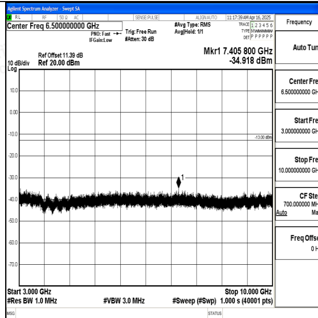
Band12_3MHz_QPSK_23025_1RB#0_3000~10000_3000~10000
