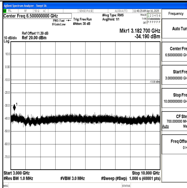
Band12_5MHz_16QAM_23155_1RB#0_3000~10000_3000~10000
