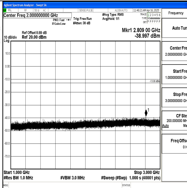
Band12_5MHz_16QAM_23155_1RB#0_1000~3000_1000~3000
