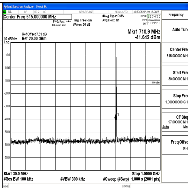
Band12_1.4MHz_QPSK_23173_1RB#0_30~1000_30~1000
