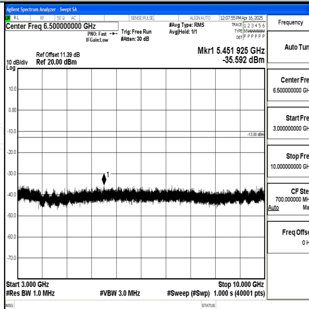
Band12_10MHz_16QAM_23060_1RB#0_3000~10000_3000~10000
