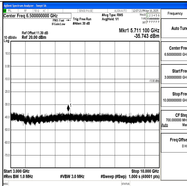
Band12_10MHz_QPSK_23060_1RB#0_3000~10000_3000~10000
