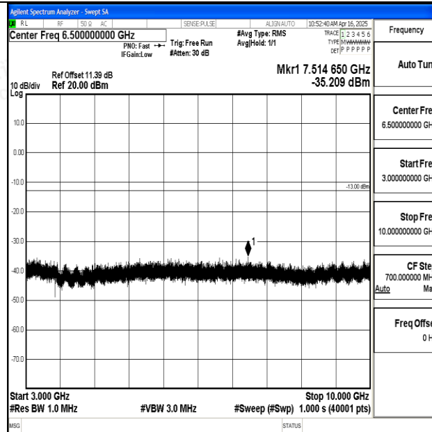
Band12_1.4MHz_QPSK_23173_1RB#0_3000~10000_3000~10000
