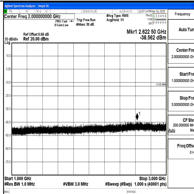
Band12_10MHz_QPSK_23060_1RB#0_1000~3000_1000~3000
