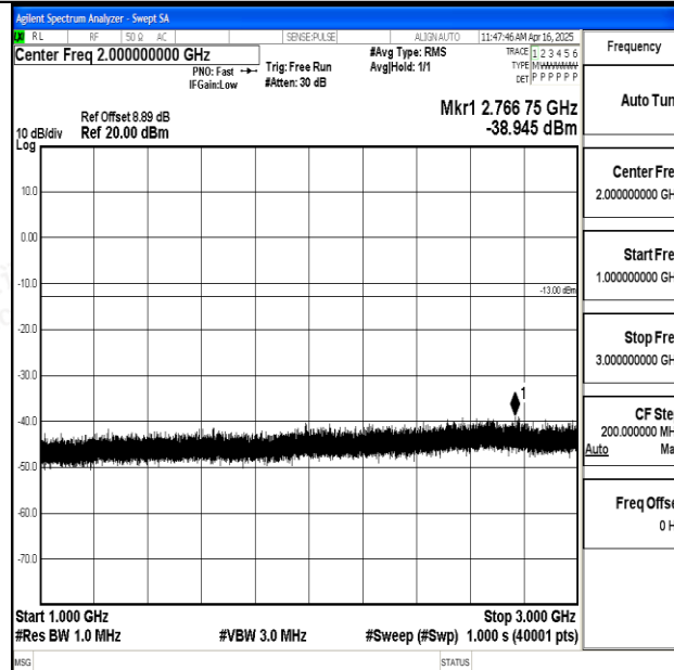
Band12_5MHz_QPSK_23155_1RB#0_1000~3000_1000~3000
