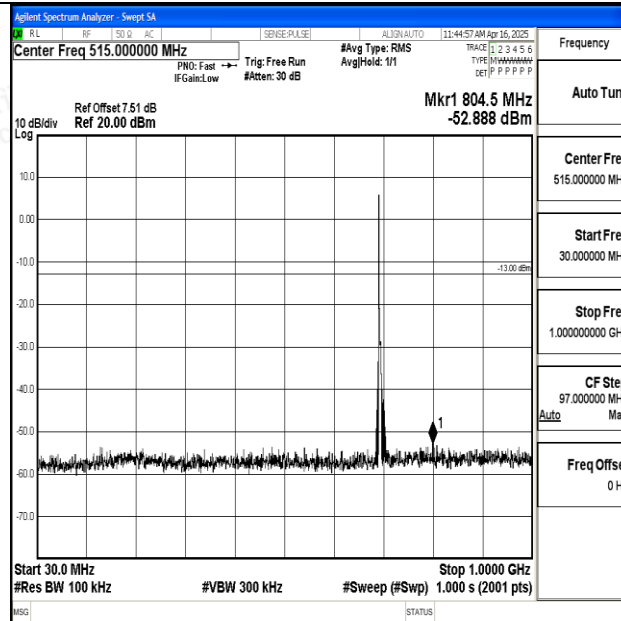
Band12_5MHz_QPSK_23035_1RB#0_30~1000_30~1000
