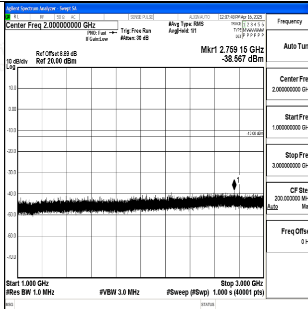
Band12_10MHz_16QAM_23060_1RB#0_1000~3000_1000~3000
