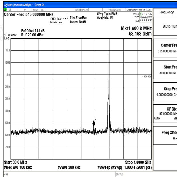
Band12_10MHz_QPSK_23060_1RB#0_30~1000_30~1000
