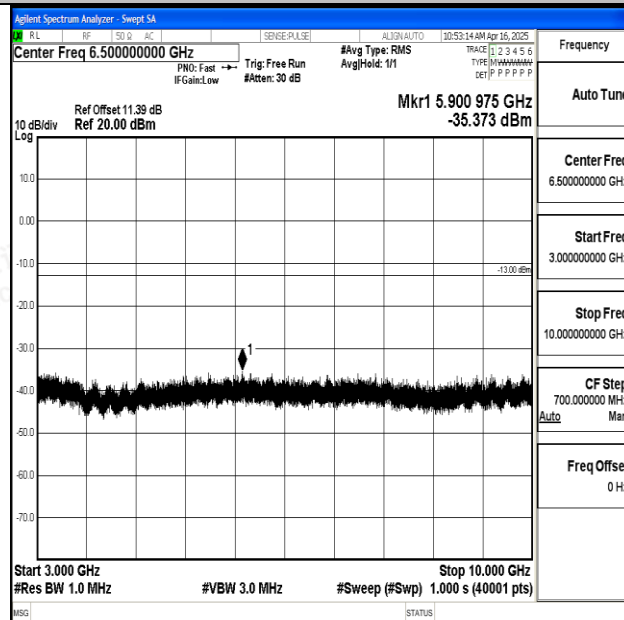
Band12_1.4MHz_16QAM_23173_1RB#0_3000~10000_3000~10000
