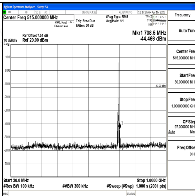
Band12_3MHz_QPSK_23025_1RB#0_30~1000_30~1000
