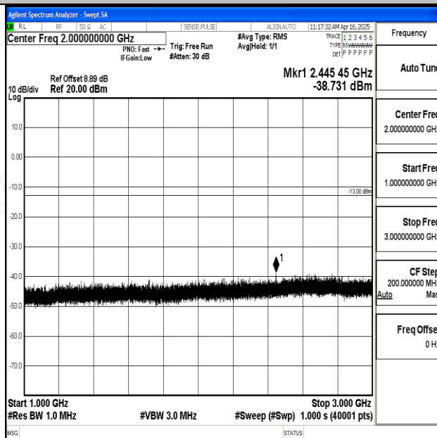
Band12_3MHz_QPSK_23025_1RB#0_1000~3000_1000~3000
