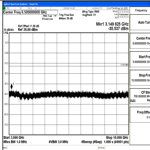
Band12_5MHz_QPSK_23155_1RB#0_3000~10000_3000~10000
