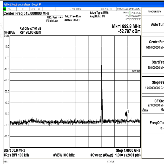
Band12_5MHz_QPSK_23155_1RB#0_30~1000_30~1000
