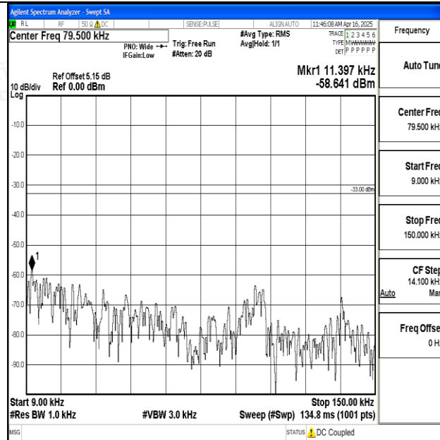
Band12_5MHz_QPSK_23095_1RB#0_0.009~0.15_0.009~0.15
