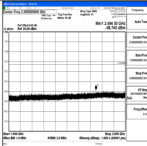
Band12_1.4MHz_16QAM_23173_1RB#0_1000~3000_1000~3000
