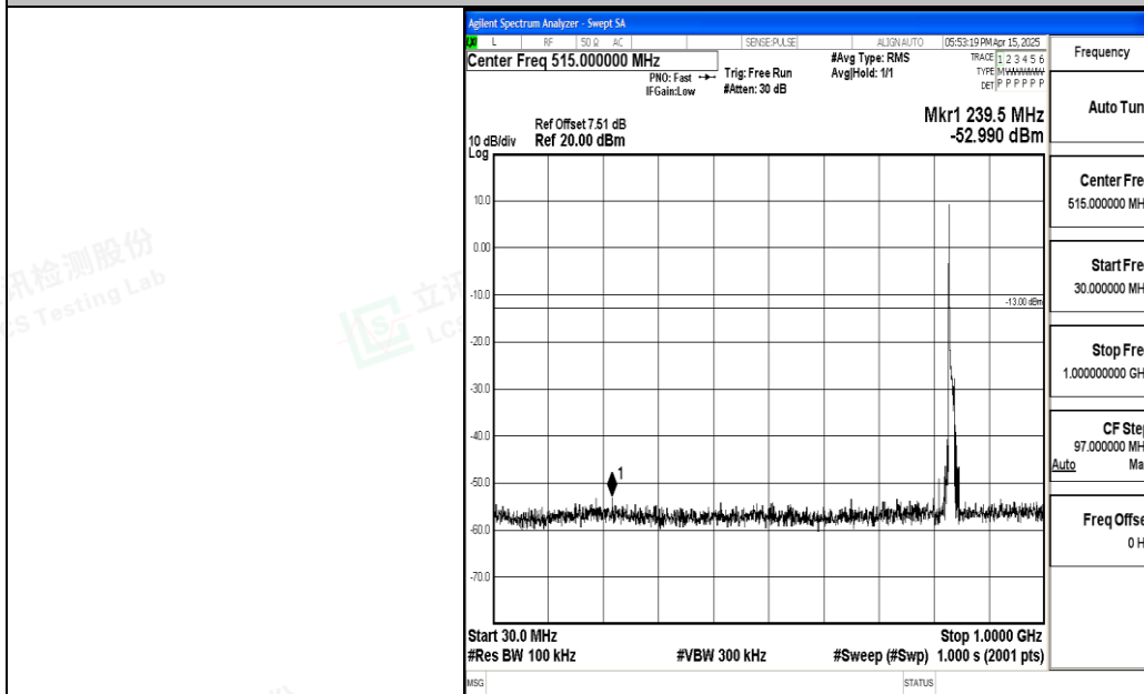
Band5_10MHz_16QAM_20525_1RB#0_30~1000_30~1000
