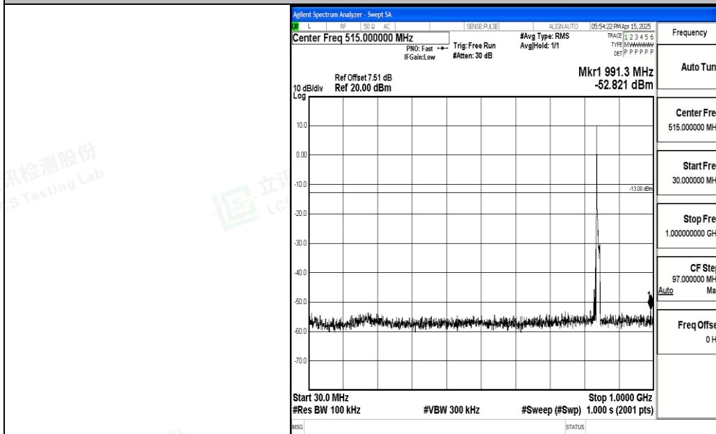
Band5_10MHz_16QAM_20600_1RB#0_30~1000_30~1000
