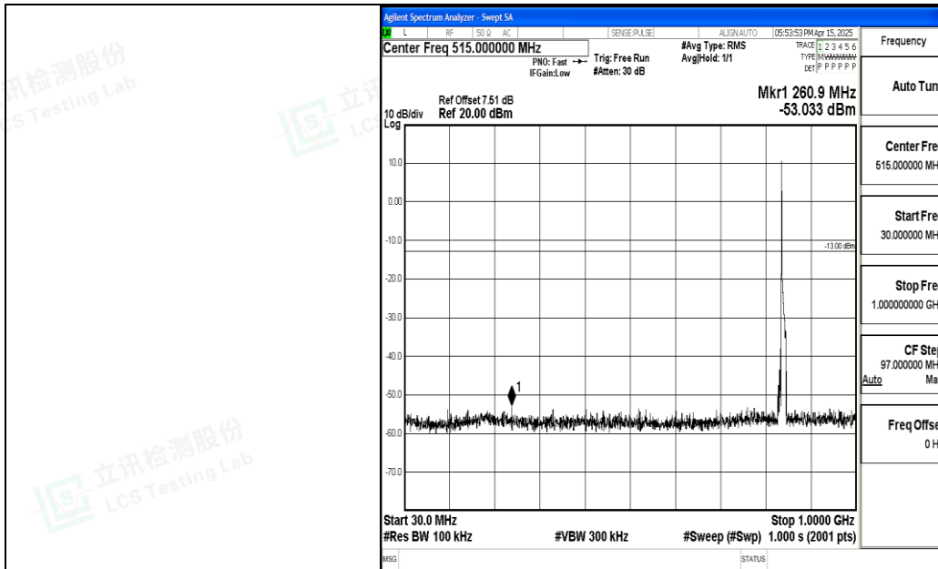
Band5_10MHz_QPSK_20600_1RB#0_30~1000_30~1000
