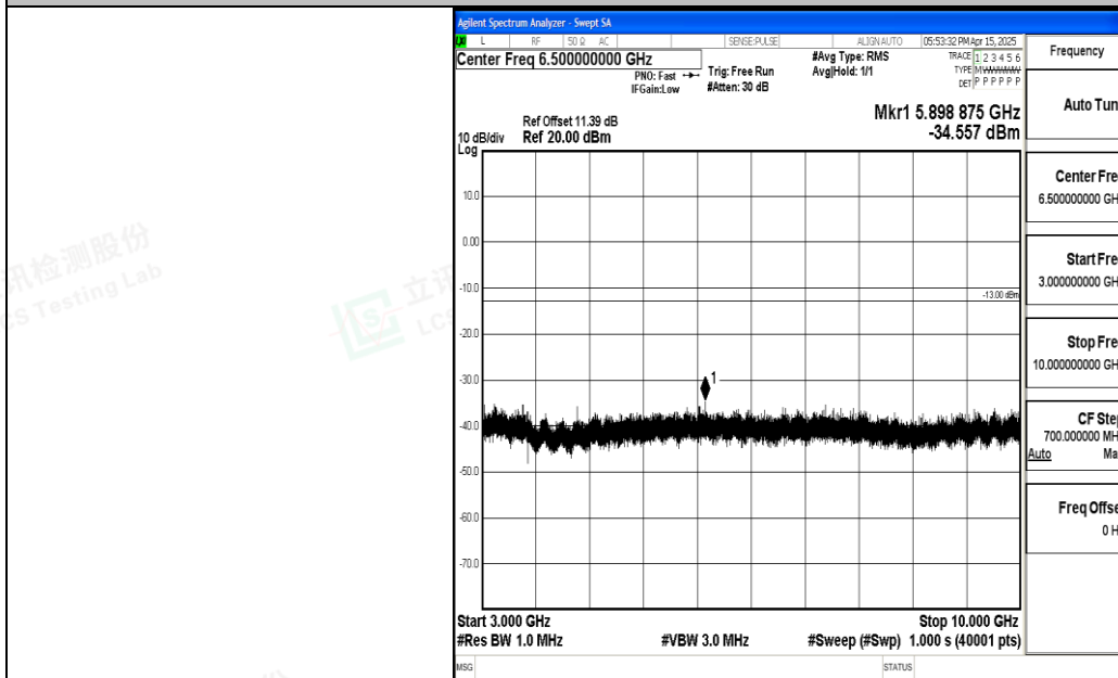
Band5_10MHz_16QAM_20525_1RB#0_3000~10000_3000~10000
