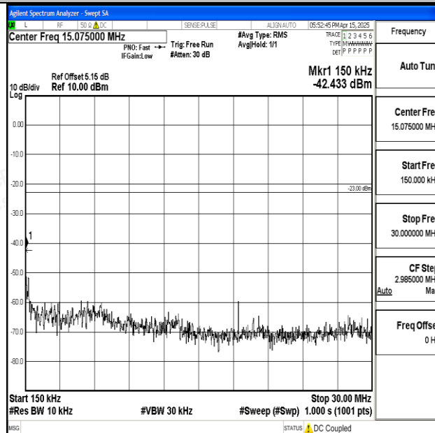
Band5_10MHz_QPSK_20525_1RB#0_0.15~30_0.15~30
