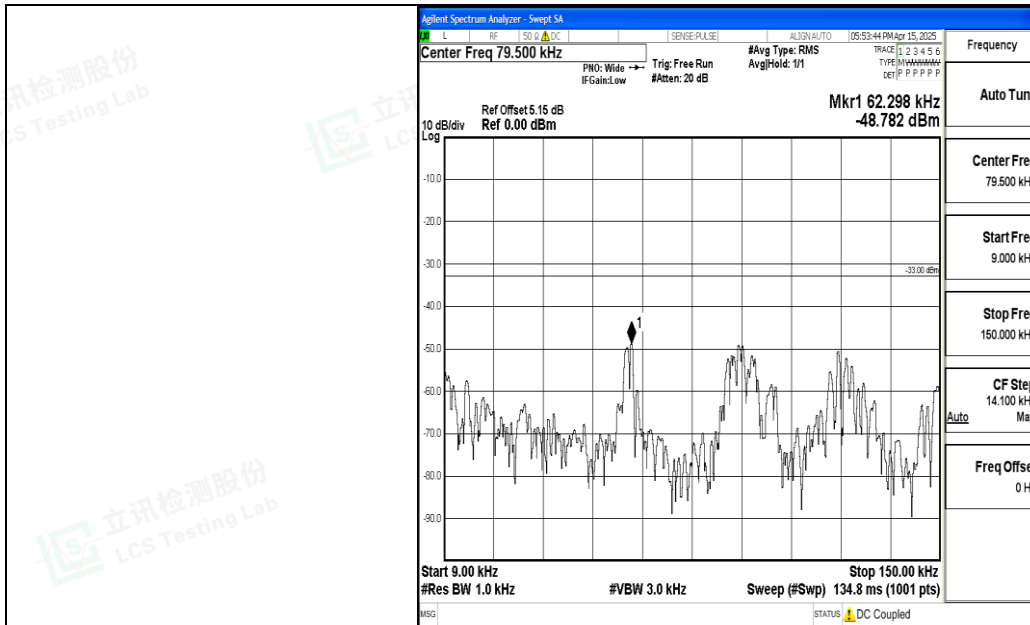
Band5_10MHz_QPSK_20600_1RB#0_0.009~0.15_0.009~0.15
