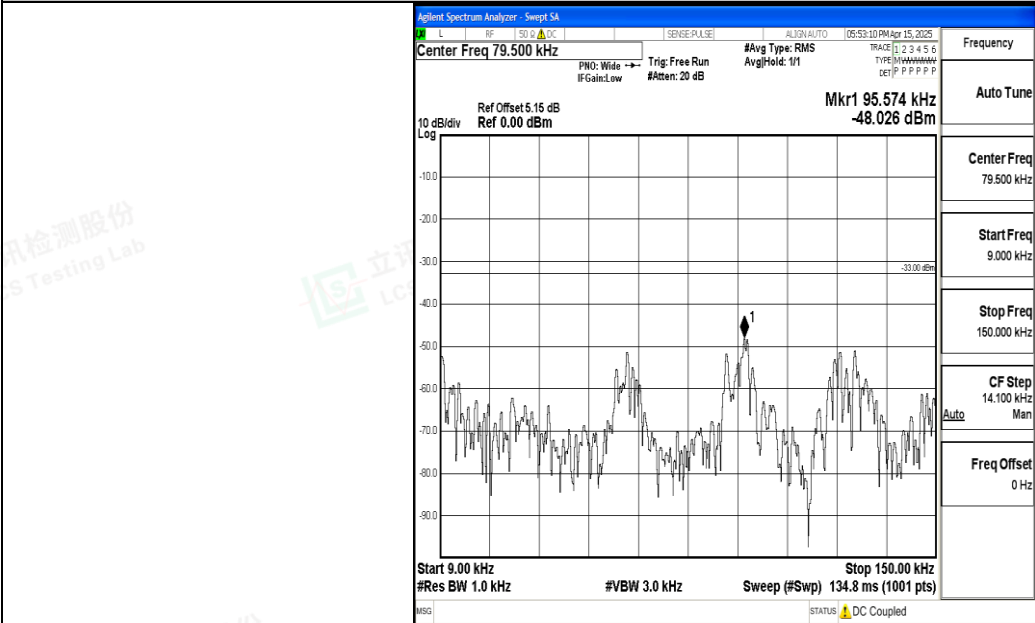
Band5_10MHz_16QAM_20525_1RB#0_0.009~0.15_0.009~0.15
