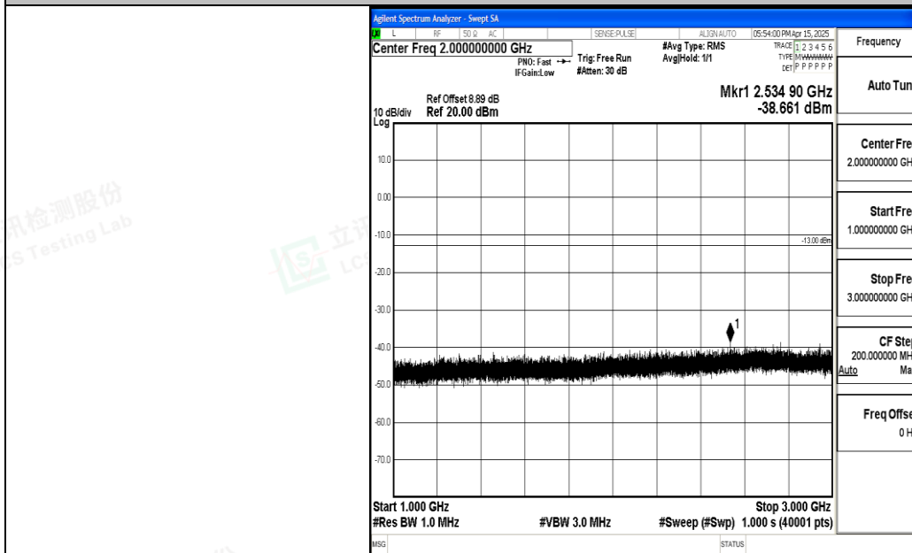
Band5_10MHz_QPSK_20600_1RB#0_1000~3000_1000~3000
