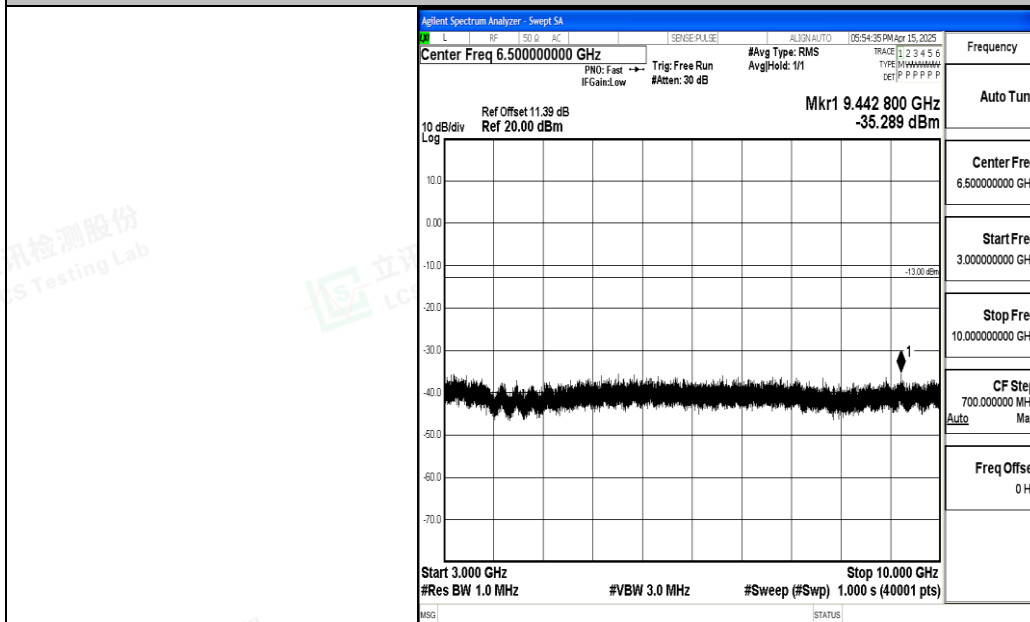
Band5_10MHz_16QAM_20600_1RB#0_3000~10000_3000~10000
