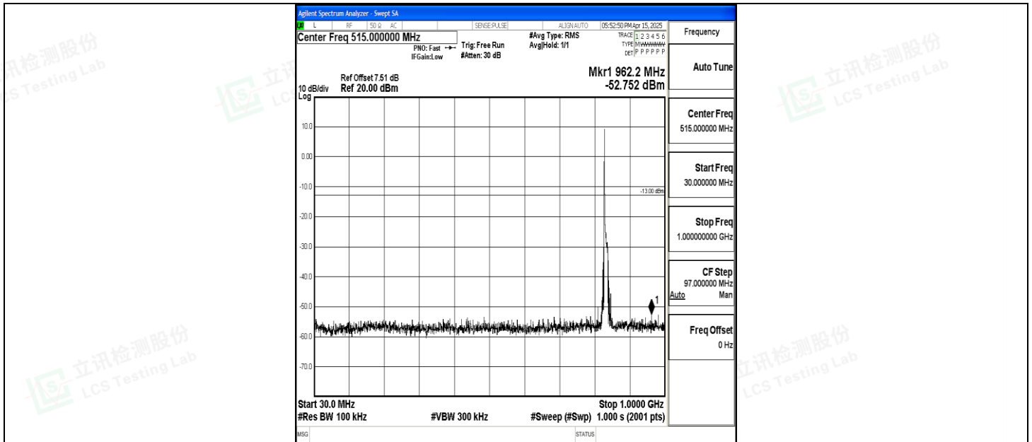
Band5_10MHz_QPSK_20525_1RB#0_30~1000_30~1000
