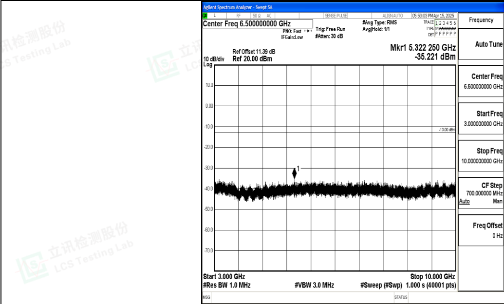
Band5_10MHz_QPSK_20525_1RB#0_3000~10000_3000~10000
