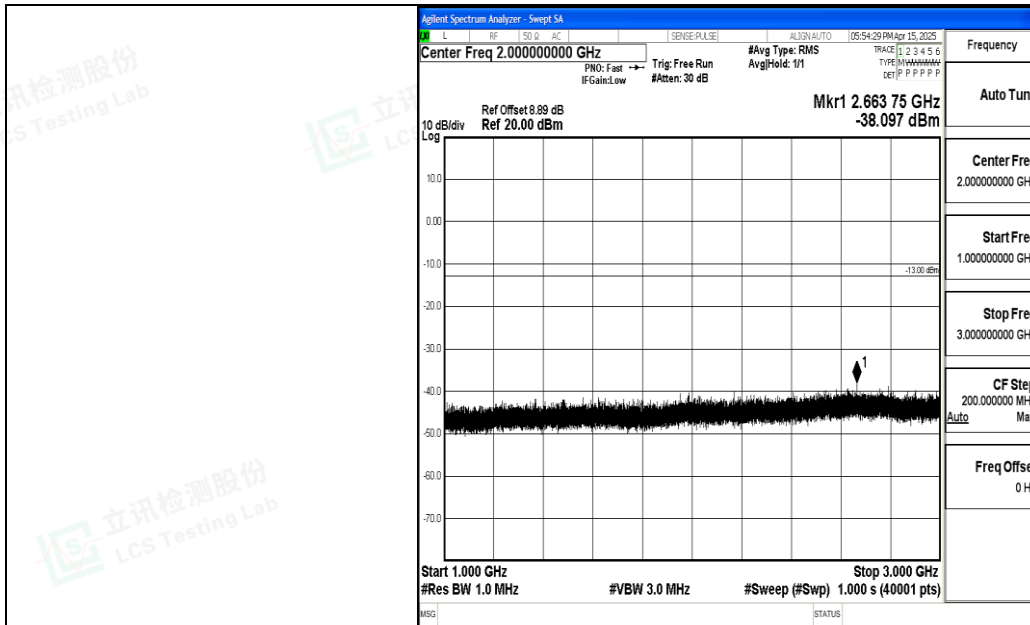
Band5_10MHz_16QAM_20600_1RB#0_1000~3000_1000~3000
