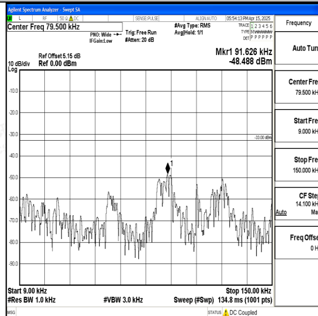
Band5_10MHz_16QAM_20600_1RB#0_0.009~0.15_0.009~0.15
