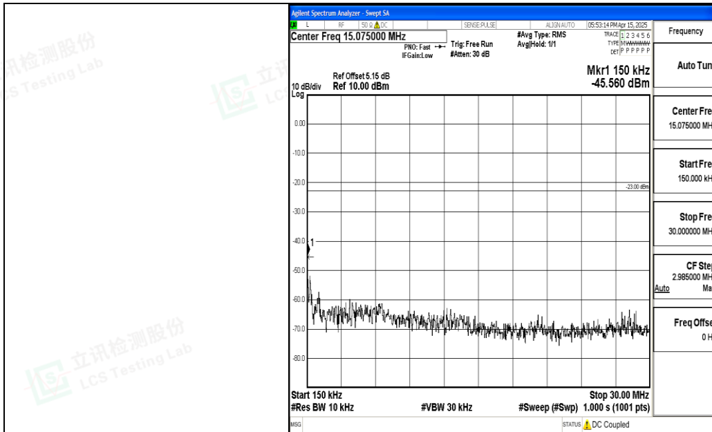
Band5_10MHz_16QAM_20525_1RB#0_0.15~30_0.15~30
