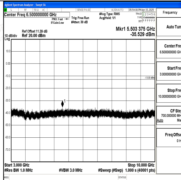
Band5_10MHz_QPSK_20600_1RB#0_3000~10000_3000~10000
