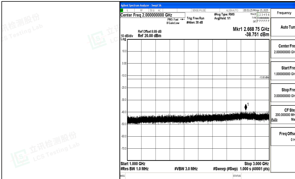
Band5_10MHz_16QAM_20525_1RB#0_1000~3000_1000~3000
