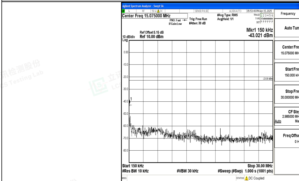
Band5_10MHz_QPSK_20600_1RB#0_0.15~30_0.15~30
