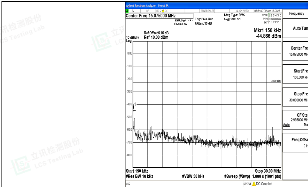
Band5_10MHz_16QAM_20600_1RB#0_0.15~30_0.15~30
