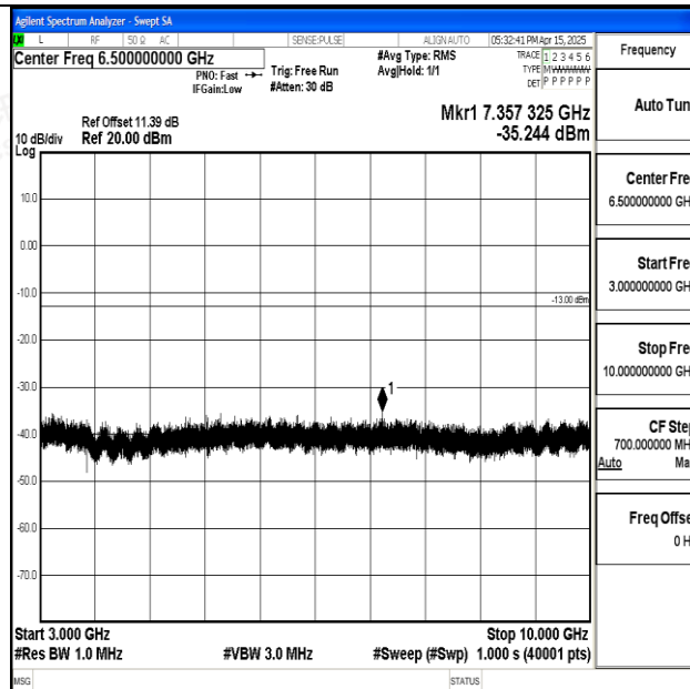
Band5_5MHz_QPSK_20525_1RB#0_3000~10000_3000~10000
