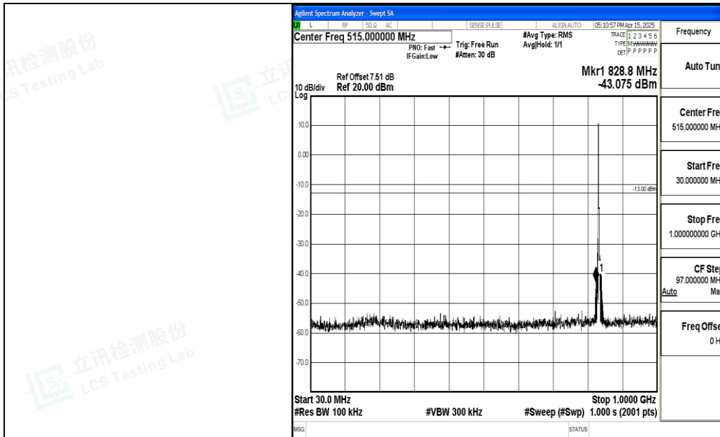
Band5_3MHz_QPSK_20525_1RB#0_30~1000_30~1000
