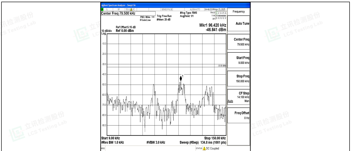
Band5_1.4MHz_QPSK_20643_1RB#0_0.009~0.15_0.009~0.15
