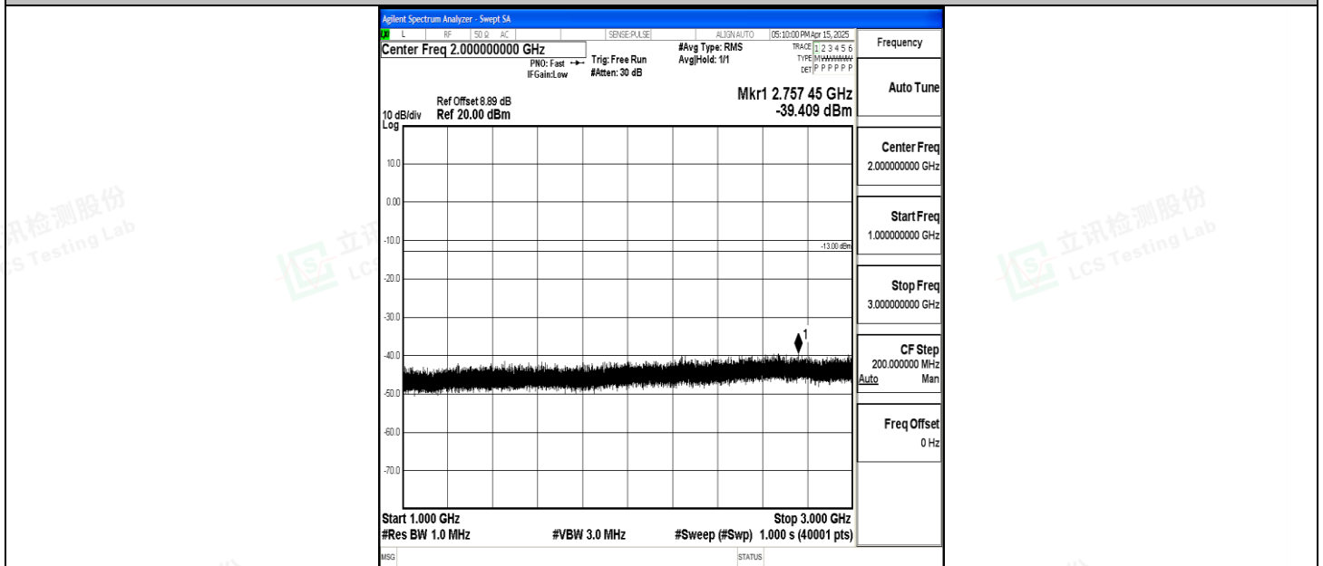
Band5_3MHz_QPSK_20415_1RB#0_1000~3000_1000~3000
