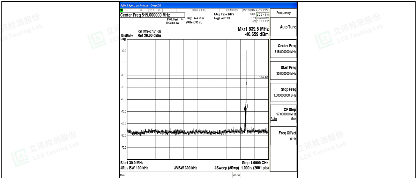
Band5_3MHz_QPSK_20635_1RB#0_30~1000_30~1000
