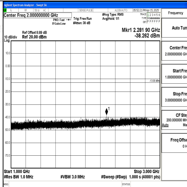
Band5_10MHz_16QAM_20450_1RB#0_1000~3000_1000~3000
