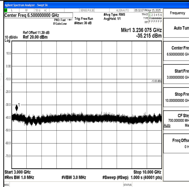
Band5_5MHz_16QAM_20425_1RB#0_3000~10000_3000~10000
