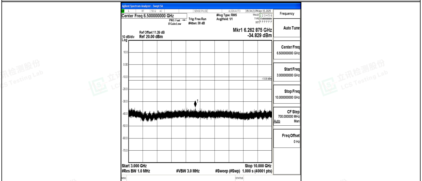
Band5_5MHz_16QAM_20625_1RB#0_3000~10000_3000~10000
