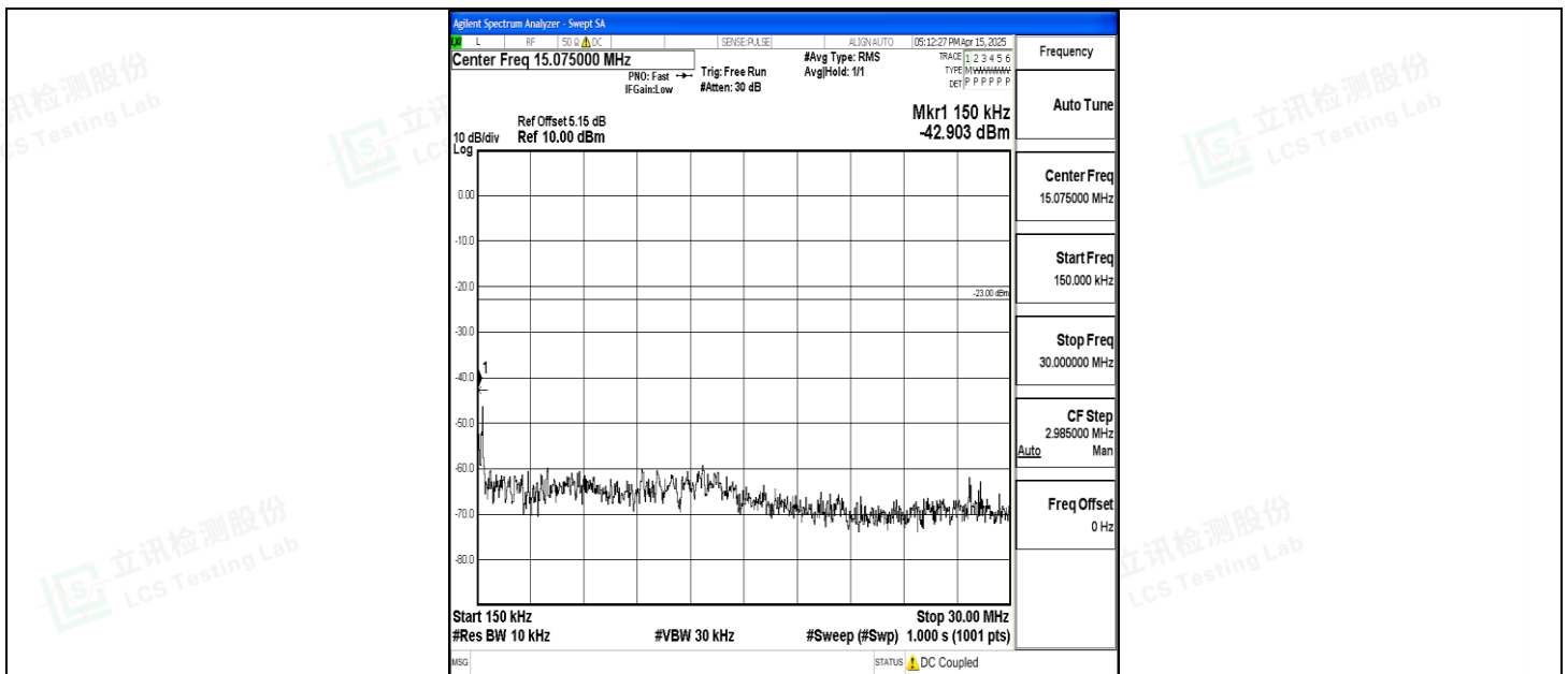
Band5_3MHz_16QAM_20635_1RB#0_0.15~30_0.15~30
