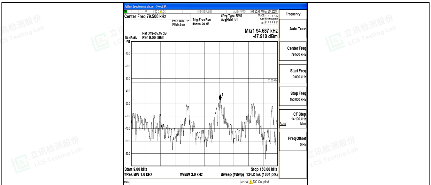
Band5_3MHz_QPSK_20525_1RB#0_0.009~0.15_0.009~0.15
