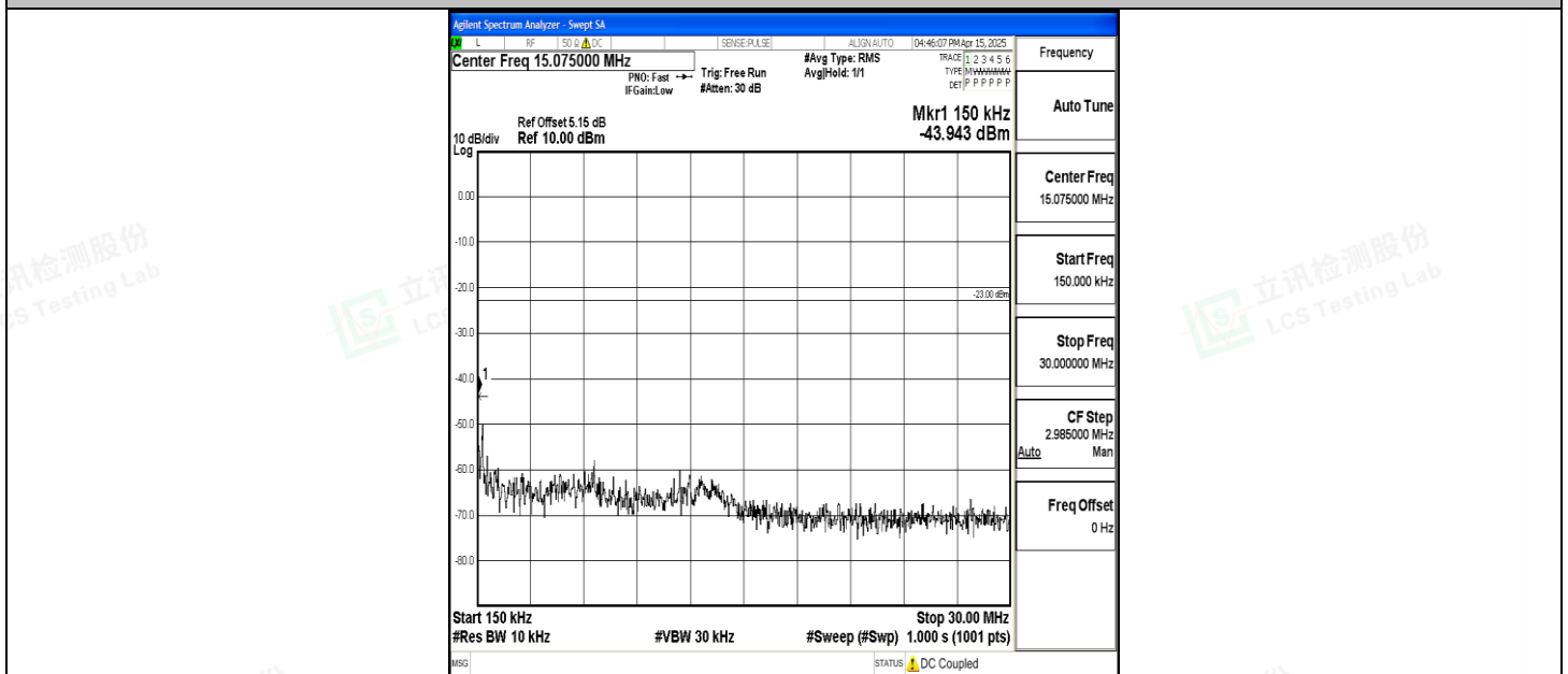
Band5_1.4MHz_QPSK_20643_1RB#0_0.15~30_0.15~30
