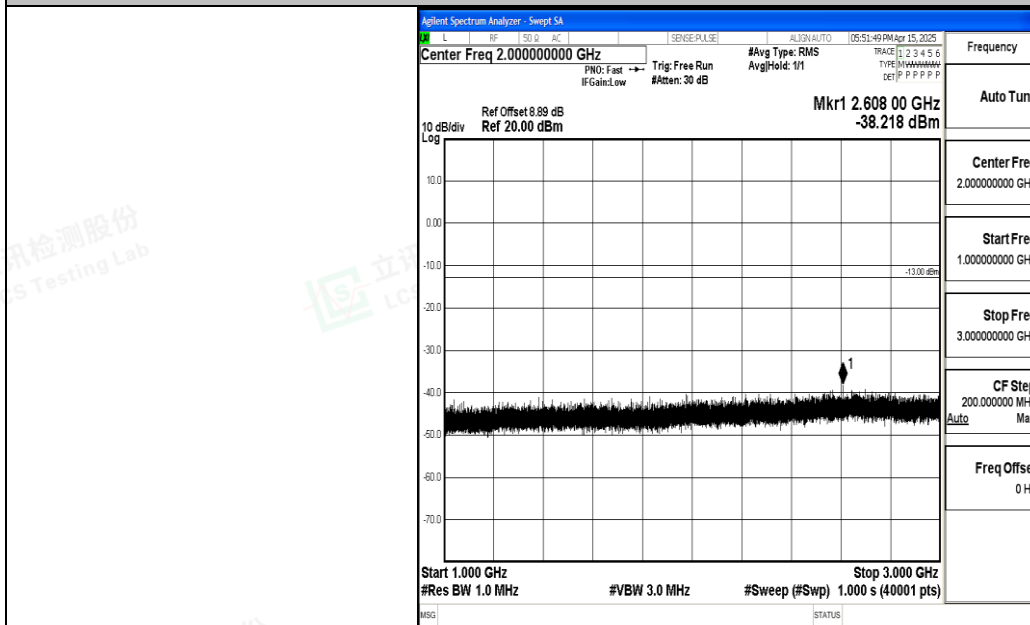
Band5_10MHz_QPSK_20450_1RB#0_1000~3000_1000~3000
