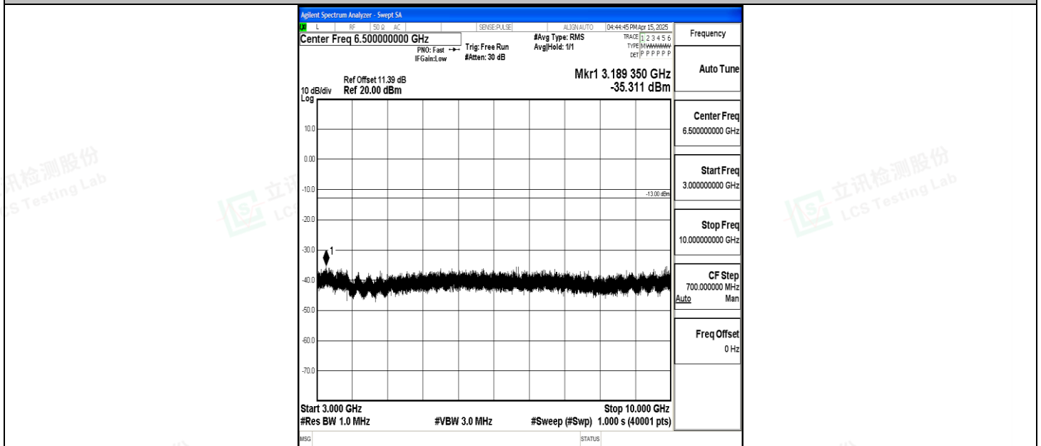
Band5_1.4MHz_16QAM_20407_1RB#0_3000~10000_3000~10000
