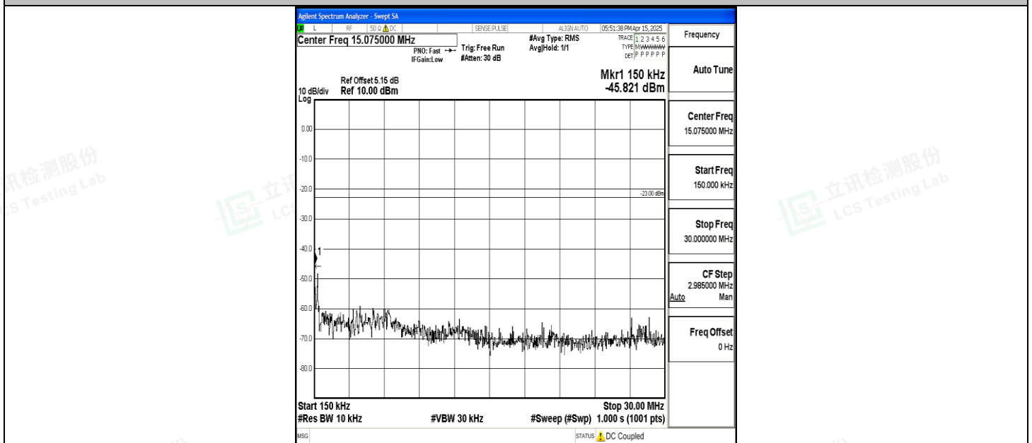
Band5_10MHz_QPSK_20450_1RB#0_0.15~30_0.15~30
