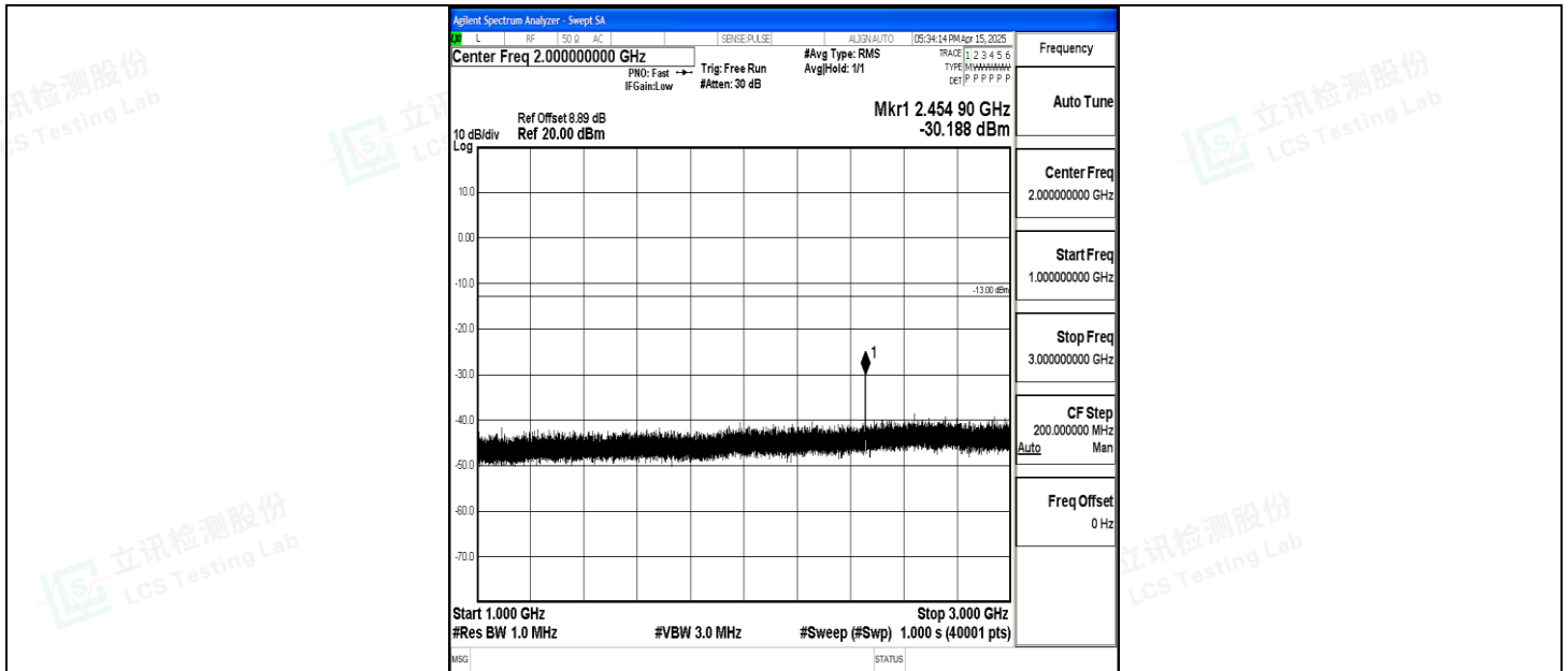
Band5_5MHz_16QAM_20625_1RB#0_1000~3000_1000~3000
