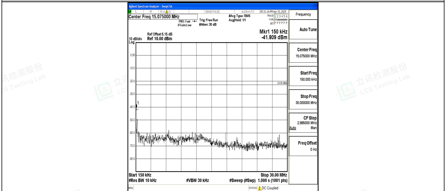
Band5_5MHz_QPSK_20425_1RB#0_0.15~30_0.15~30
