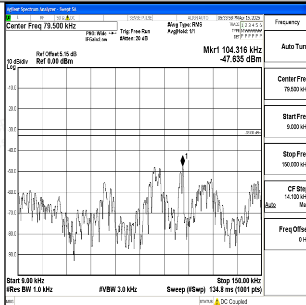
Band5_5MHz_16QAM_20625_1RB#0_0.009~0.15_0.009~0.15
