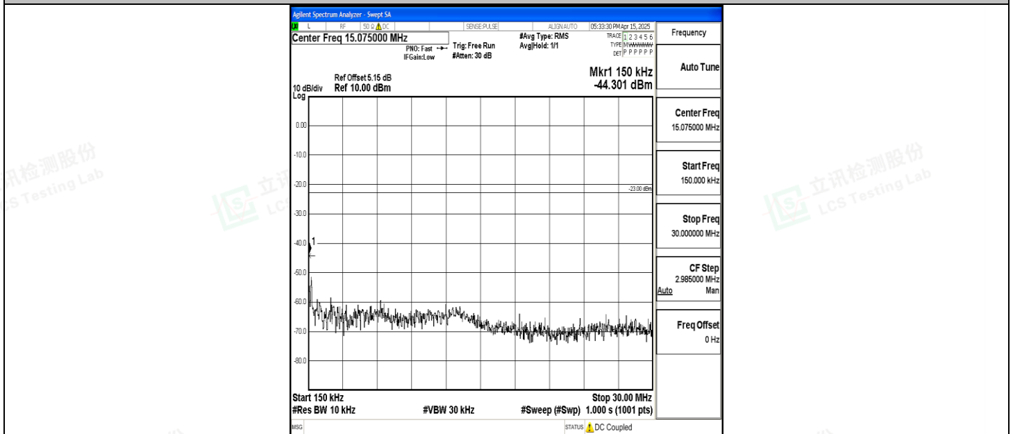
Band5_5MHz_QPSK_20625_1RB#0_0.15~30_0.15~30
