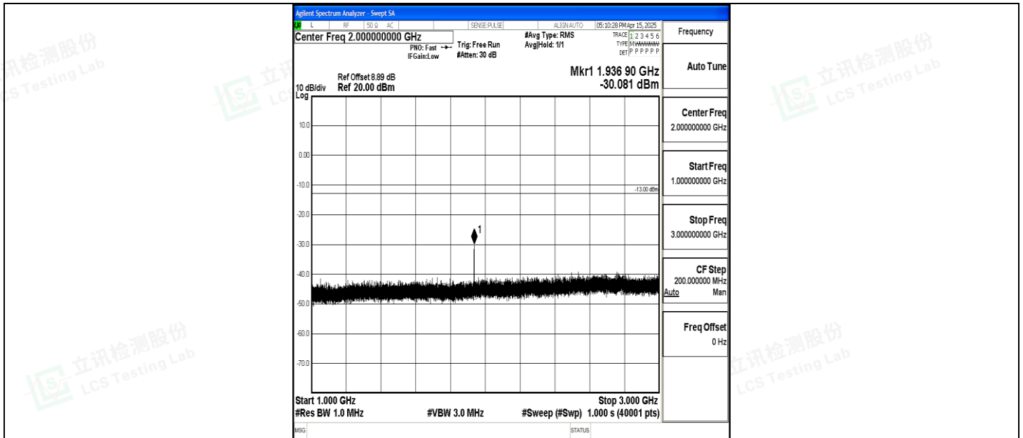
Band5_3MHz_16QAM_20415_1RB#0_1000~3000_1000~3000
