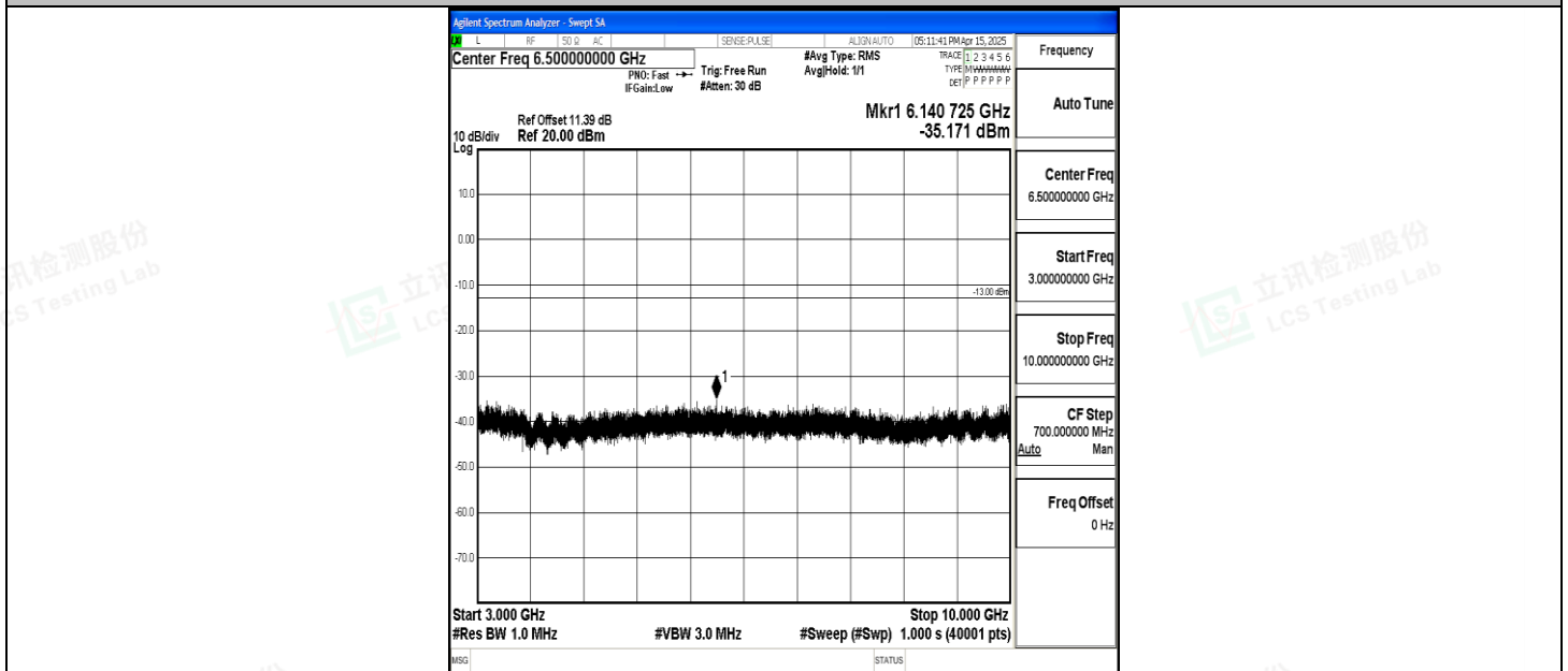
Band5_3MHz_16QAM_20525_1RB#0_3000~10000_3000~10000
