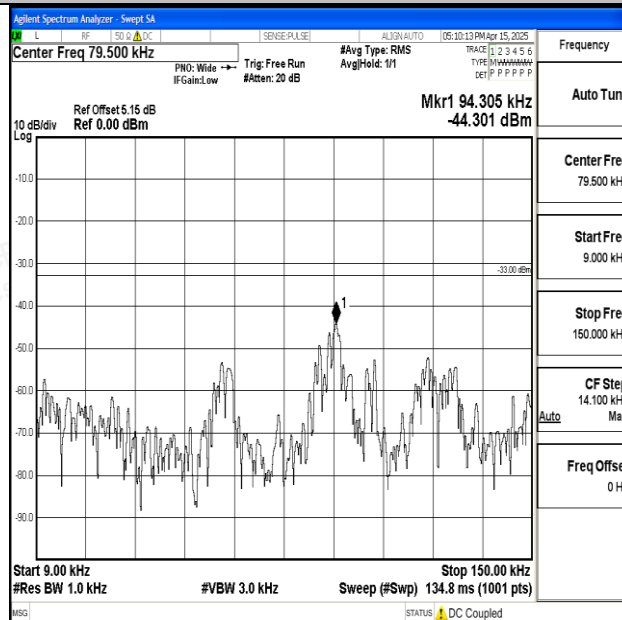
Band5_3MHz_16QAM_20415_1RB#0_0.009~0.15_0.009~0.15
