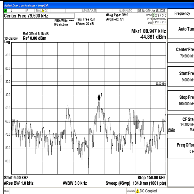
Band5_5MHz_16QAM_20425_1RB#0_0.009~0.15_0.009~0.15
