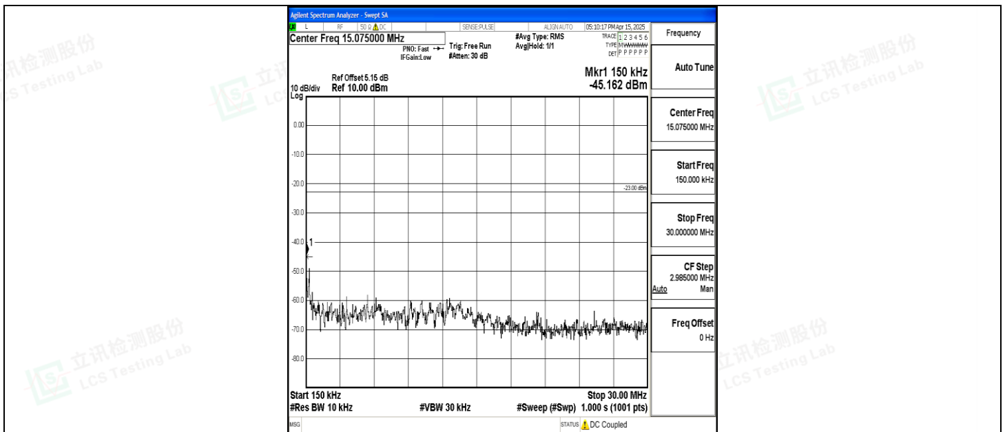
Band5_3MHz_16QAM_20415_1RB#0_0.15~30_0.15~30
