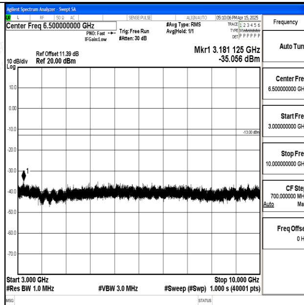
Band5_3MHz_QPSK_20415_1RB#0_3000~10000_3000~10000
