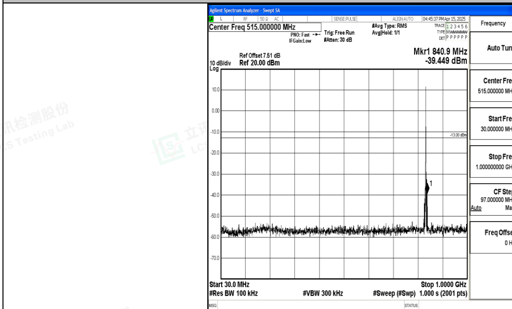
Band5_1.4MHz_16QAM_20525_1RB#0_30~1000_30~1000
