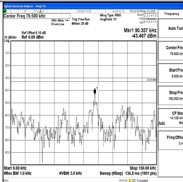
Band5_5MHz_16QAM_20525_1RB#0_0.009~0.15_0.009~0.15
