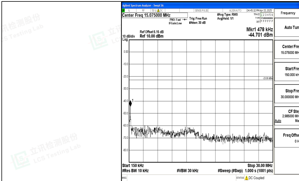
Band5_1.4MHz_16QAM_20525_1RB#0_0.15~30_0.15~30
