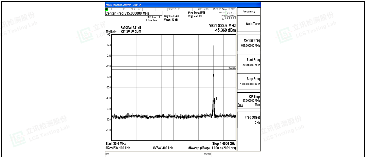
Band5_3MHz_QPSK_20415_1RB#0_30~1000_30~1000
