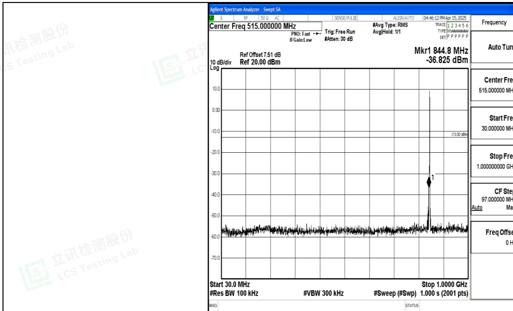
Band5_1.4MHz_QPSK_20643_1RB#0_30~1000_30~1000
