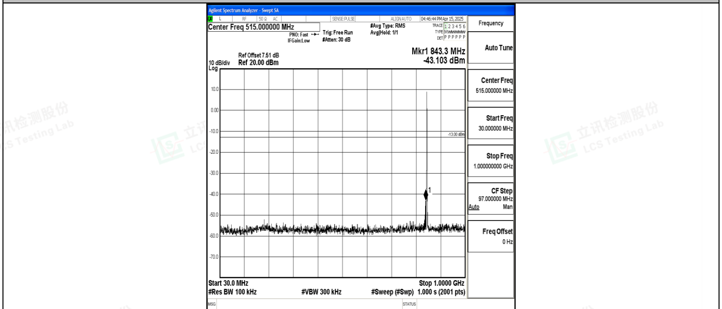
Band5_1.4MHz_16QAM_20643_1RB#0_30~1000_30~1000
