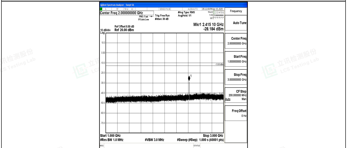
Band5_3MHz_QPSK_20635_1RB#0_1000~3000_1000~3000
