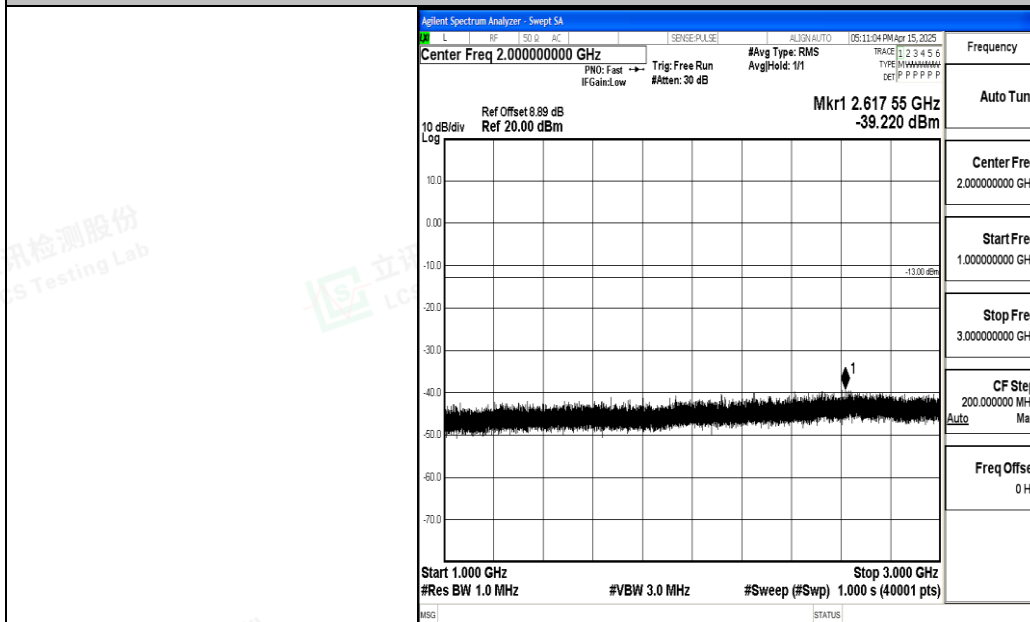
Band5_3MHz_QPSK_20525_1RB#0_1000~3000_1000~3000
