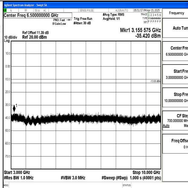
Band5_10MHz_QPSK_20450_1RB#0_3000~10000_3000~10000
