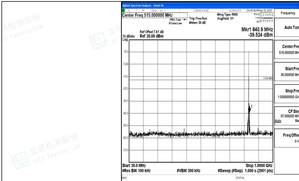
Band5_1.4MHz_QPSK_20525_1RB#0_30~1000_30~1000
