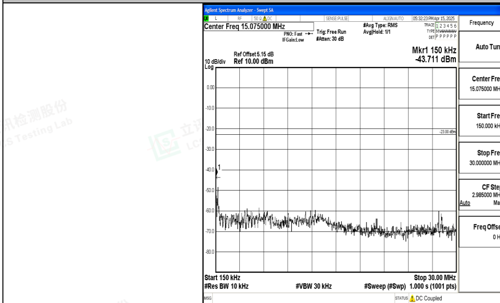
Band5_5MHz_QPSK_20525_1RB#0_0.15~30_0.15~30
