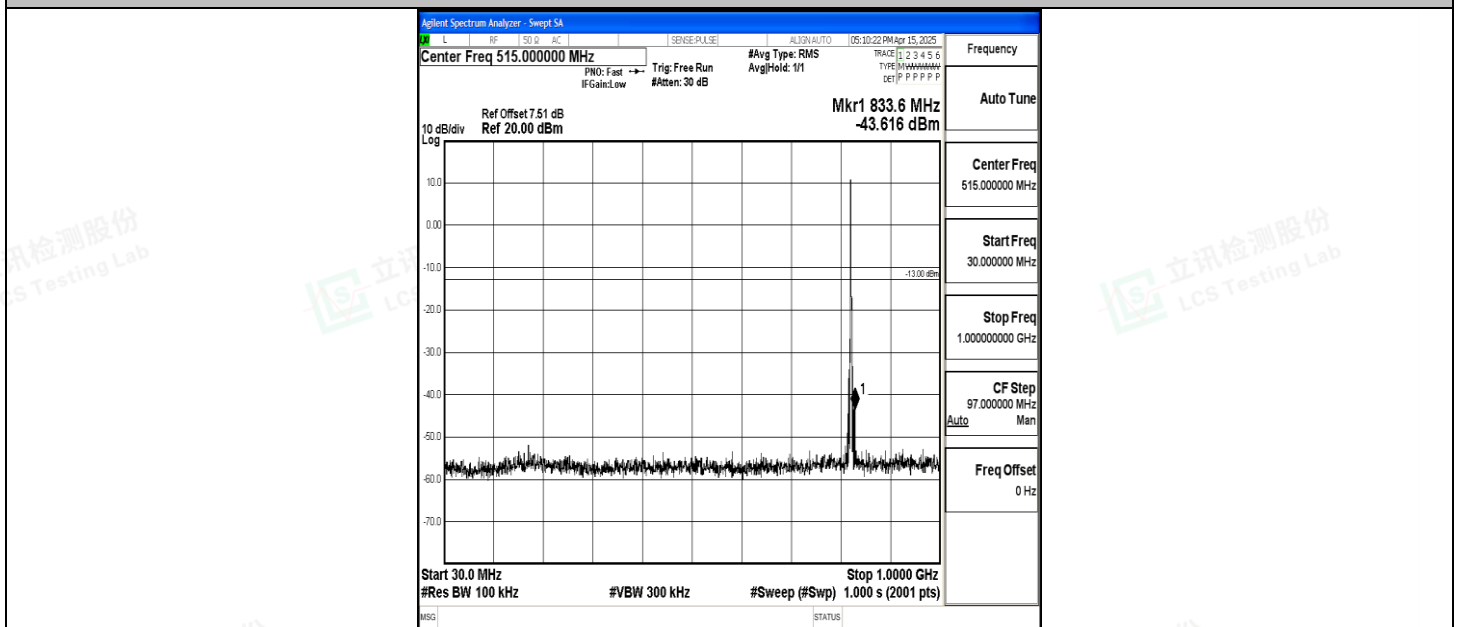
Band5_3MHz_16QAM_20415_1RB#0_30~1000_30~1000
