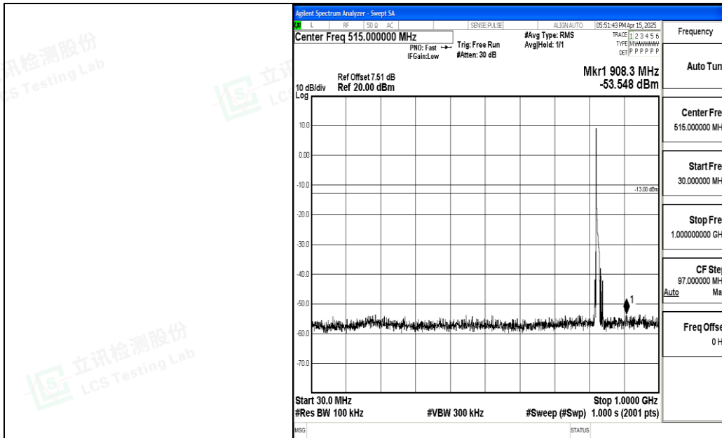
Band5_10MHz_QPSK_20450_1RB#0_30~1000_30~1000
