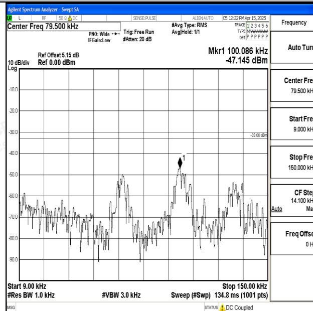
Band5_3MHz_16QAM_20635_1RB#0_0.009~0.15_0.009~0.15
