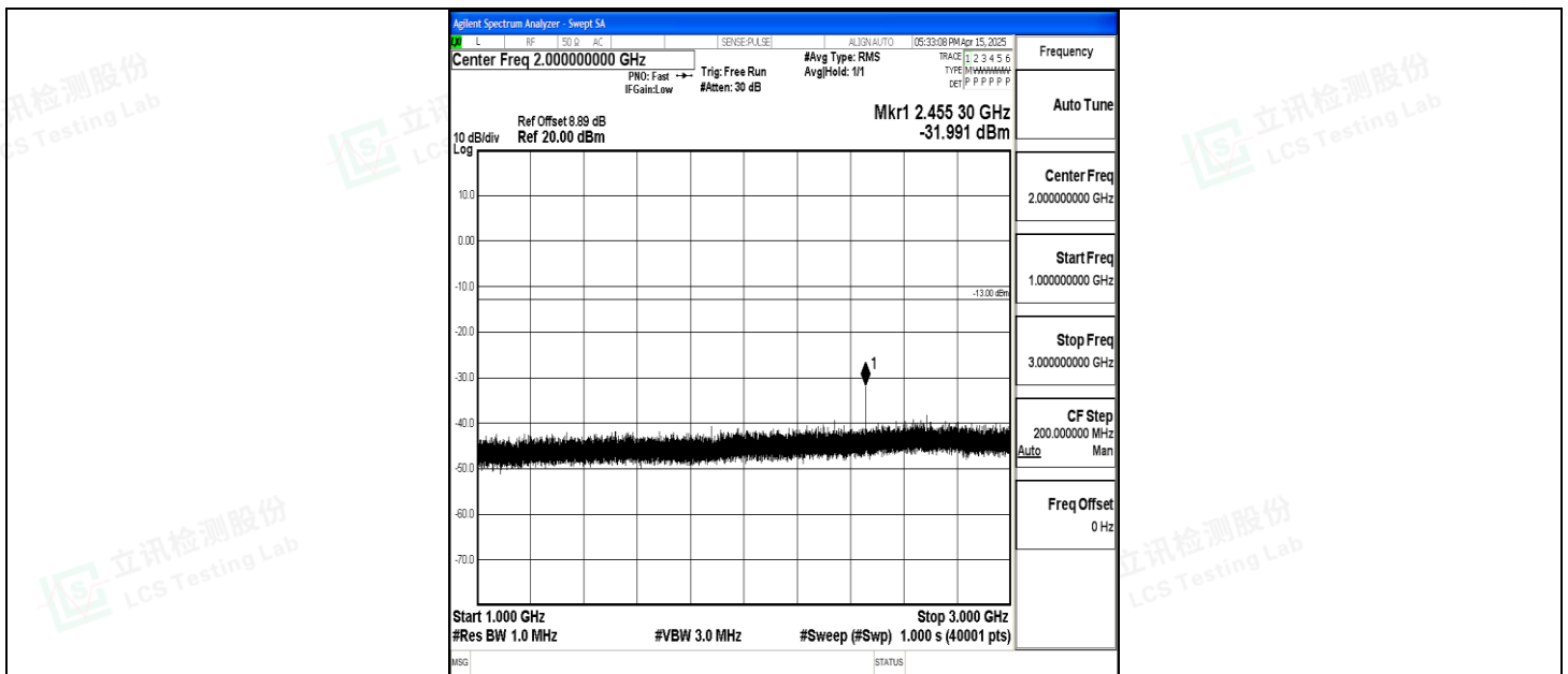
Band5_5MHz_16QAM_20525_1RB#0_1000~3000_1000~3000
