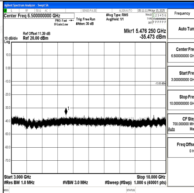
Band5_3MHz_QPSK_20525_1RB#0_3000~10000_3000~10000
