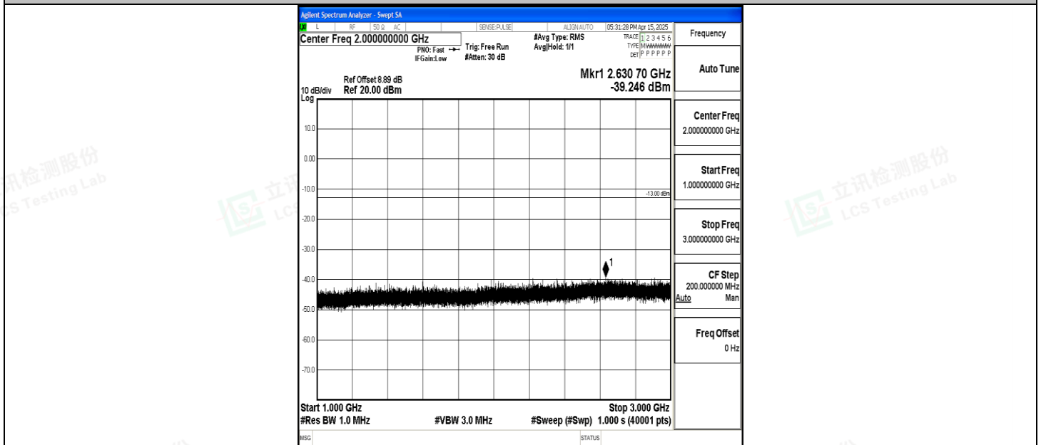
Band5_5MHz_QPSK_20425_1RB#0_1000~3000_1000~3000
