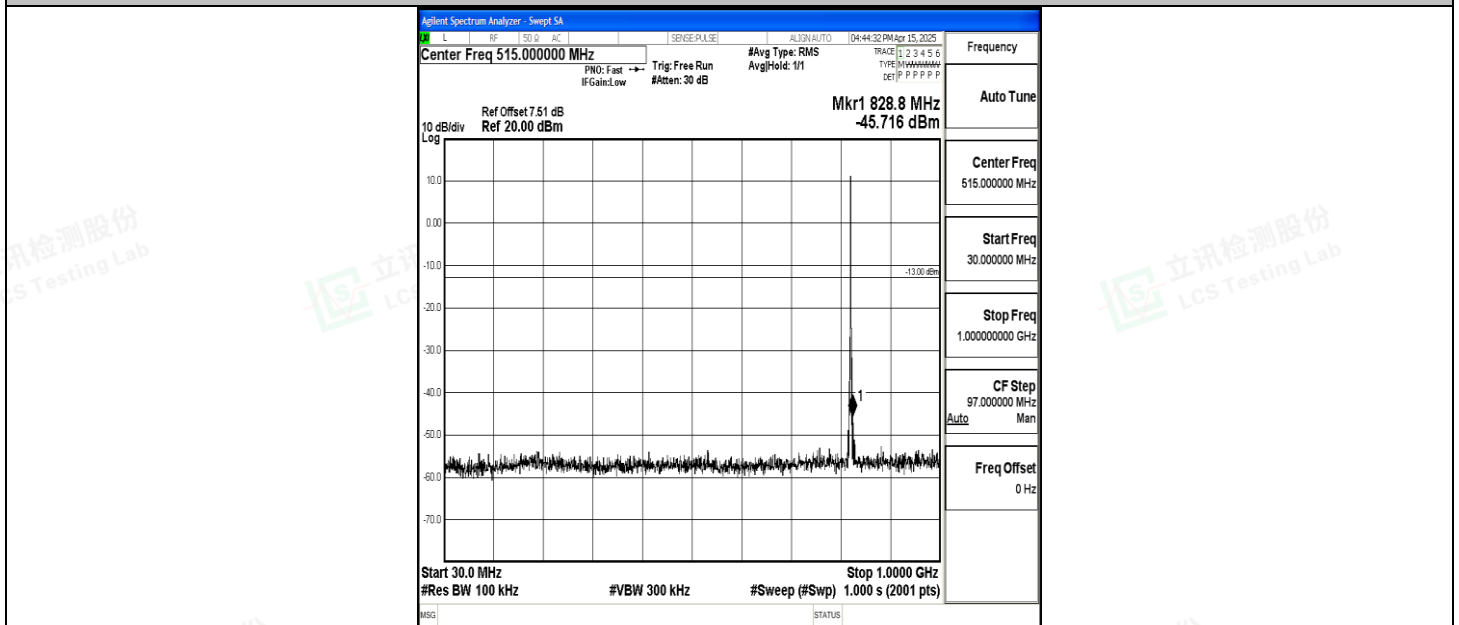
Band5_1.4MHz_16QAM_20407_1RB#0_30~1000_30~1000
