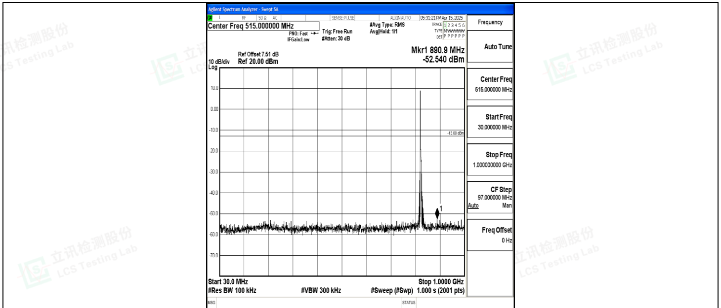
Band5_5MHz_QPSK_20425_1RB#0_30~1000_30~1000
