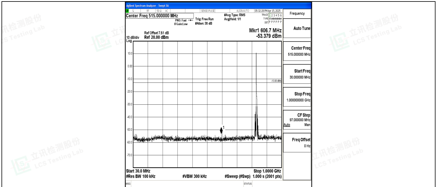
Band5_5MHz_QPSK_20525_1RB#0_30~1000_30~1000
