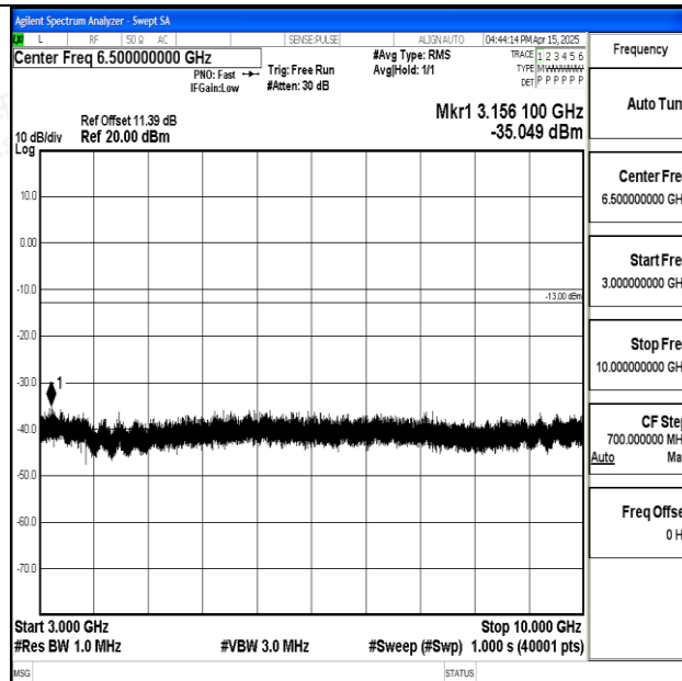
Band5_1.4MHz_QPSK_20407_1RB#0_3000~10000_3000~10000
