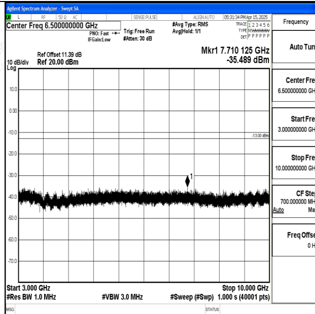
Band5_5MHz_QPSK_20425_1RB#0_3000~10000_3000~10000
