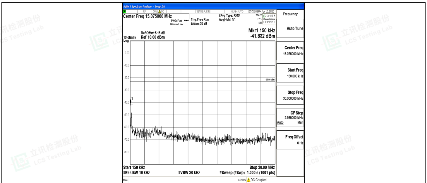
Band5_10MHz_16QAM_20450_1RB#0_0.15~30_0.15~30
