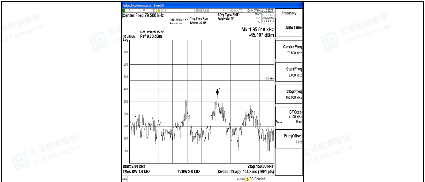
Band5_1.4MHz_QPSK_20525_1RB#0_0.009~0.15_0.009~0.15
