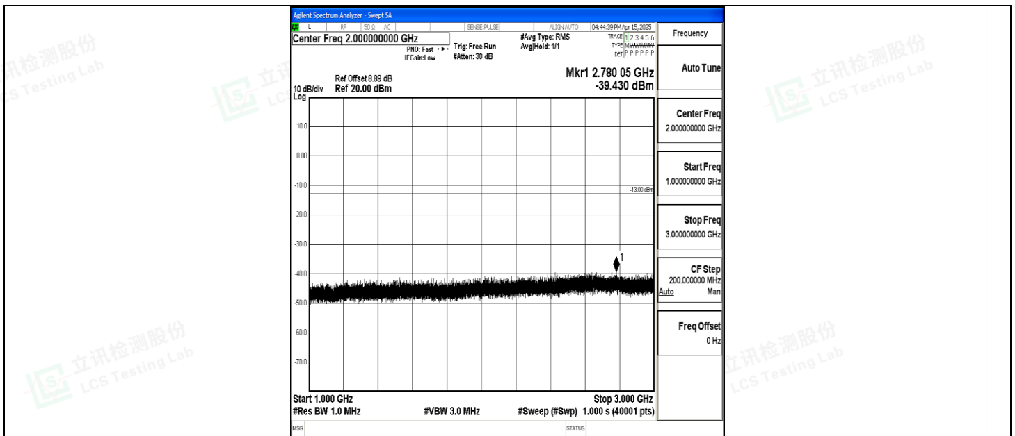
Band5_1.4MHz_16QAM_20407_1RB#0_1000~3000_1000~3000
