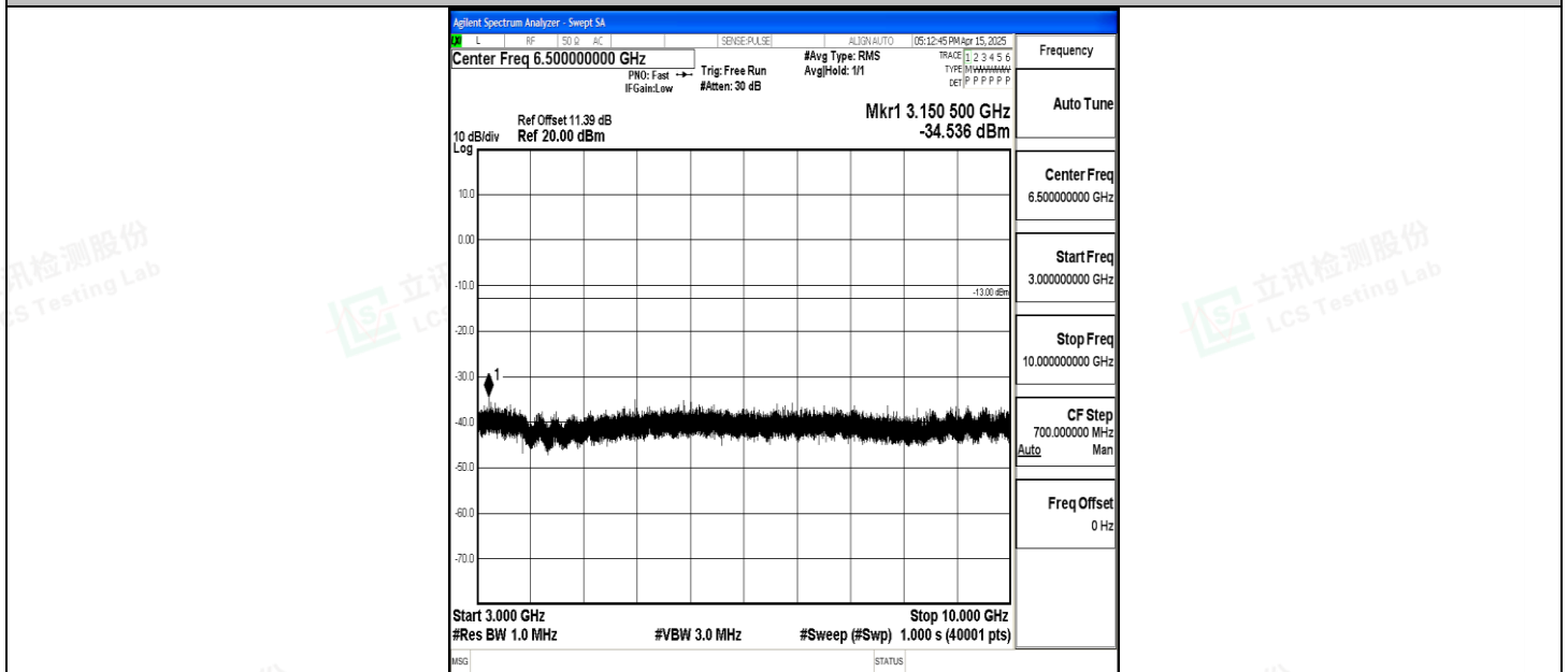
Band5_3MHz_16QAM_20635_1RB#0_3000~10000_3000~10000
