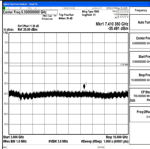
Band5_10MHz_16QAM_20450_1RB#0_3000~10000_3000~10000
