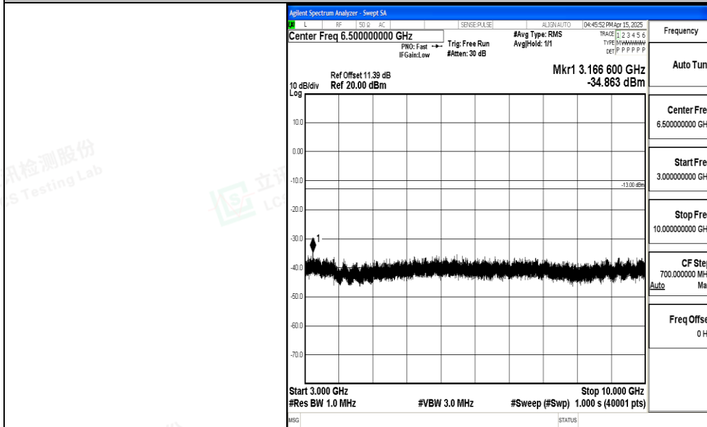
Band5_1.4MHz_16QAM_20525_1RB#0_3000~10000_3000~10000
