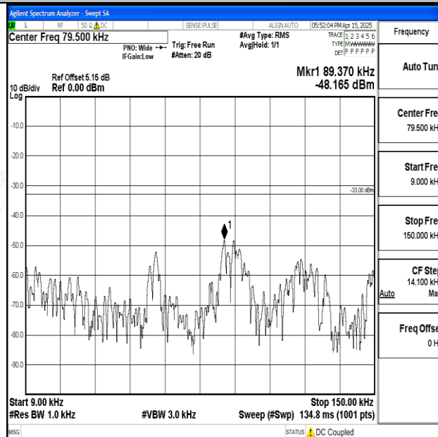
Band5_10MHz_16QAM_20450_1RB#0_0.009~0.15_0.009~0.15
