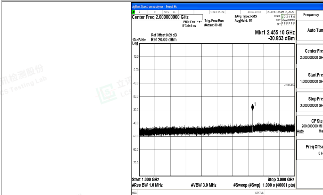
Band5_5MHz_QPSK_20625_1RB#0_1000~3000_1000~3000
