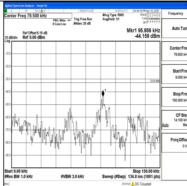
Band5_1.4MHz_16QAM_20643_1RB#0_0.009~0.15_0.009~0.15
