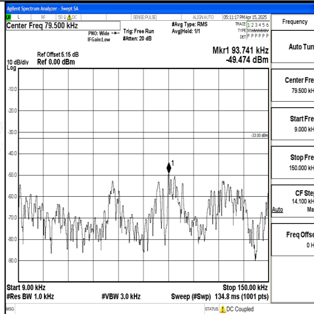
Band5_3MHz_16QAM_20525_1RB#0_0.009~0.15_0.009~0.15
