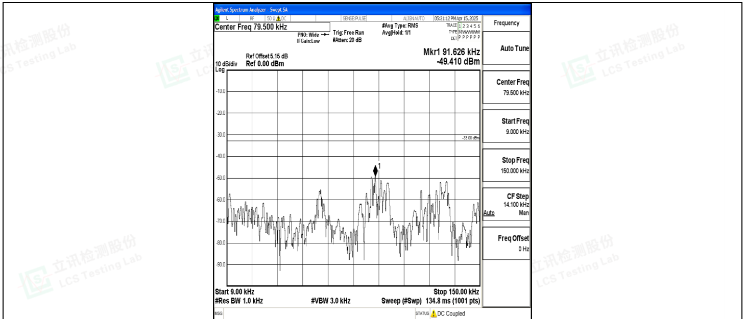
Band5_5MHz_QPSK_20425_1RB#0_0.009~0.15_0.009~0.15
