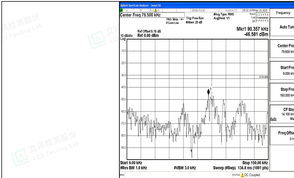
Band5_5MHz_QPSK_20525_1RB#0_0.009~0.15_0.009~0.15
