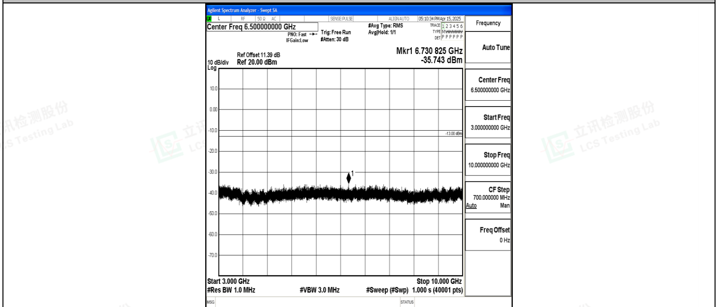
Band5_3MHz_16QAM_20415_1RB#0_3000~10000_3000~10000
