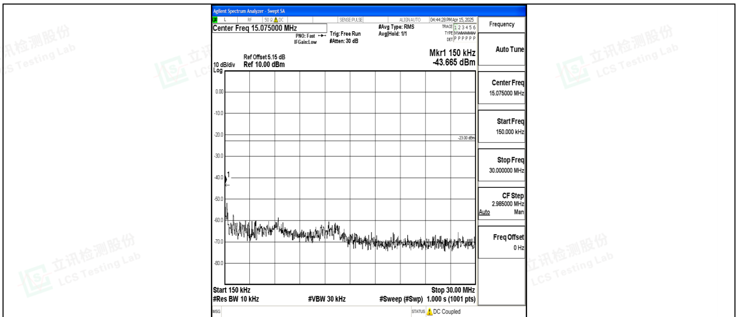
Band5_1.4MHz_16QAM_20407_1RB#0_0.15~30_0.15~30
