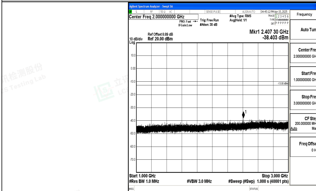
Band5_1.4MHz_QPSK_20525_1RB#0_1000~3000_1000~3000
