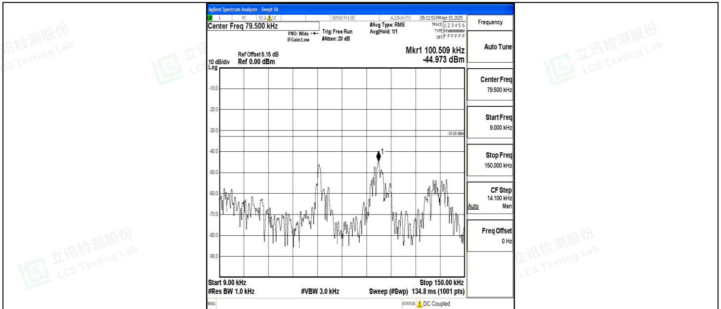
Band5_3MHz_QPSK_20635_1RB#0_0.009~0.15_0.009~0.15
