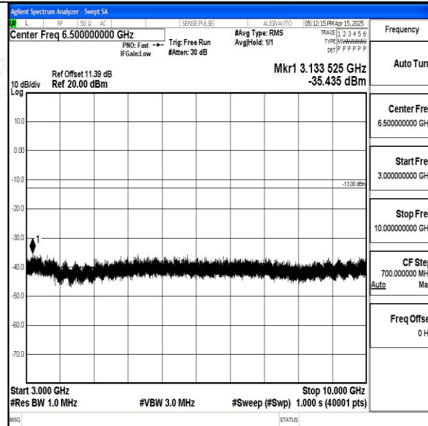
Band5_3MHz_QPSK_20635_1RB#0_3000~10000_3000~10000
