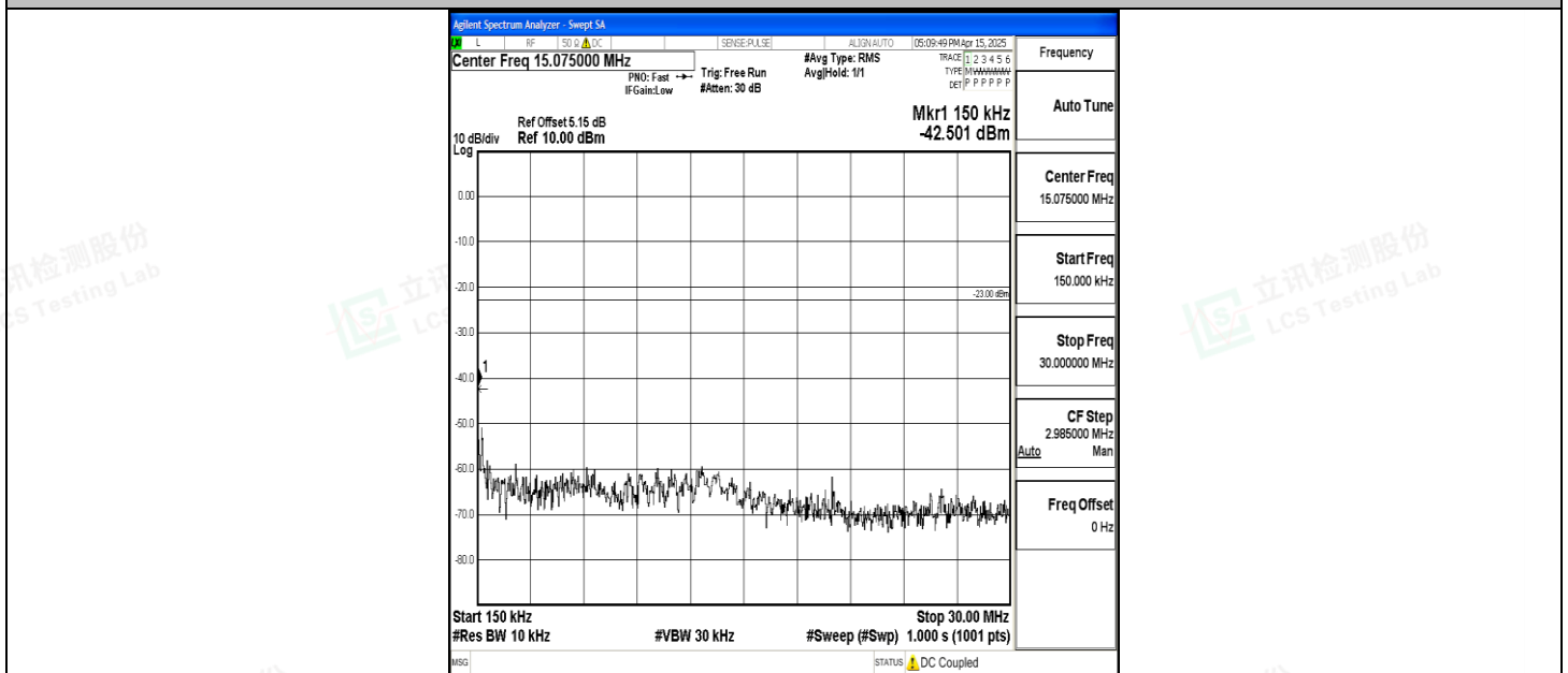
Band5_3MHz_QPSK_20415_1RB#0_0.15~30_0.15~30
