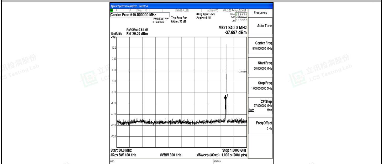
Band5_3MHz_16QAM_20635_1RB#0_30~1000_30~1000
