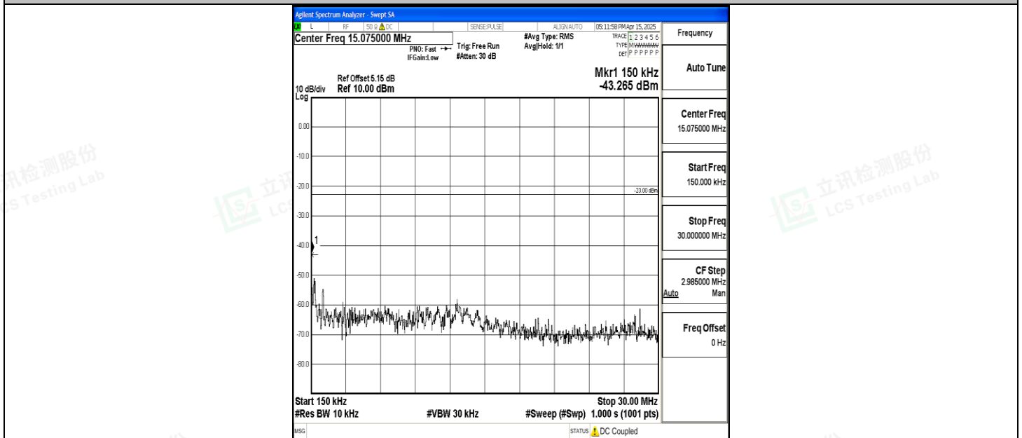
Band5_3MHz_QPSK_20635_1RB#0_0.15~30_0.15~30
