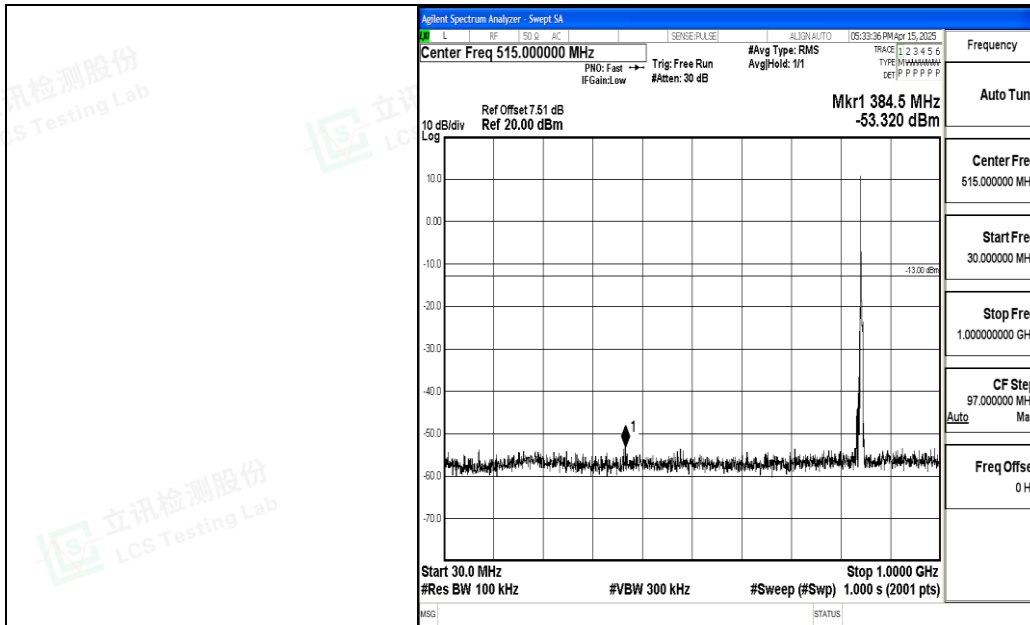
Band5_5MHz_QPSK_20625_1RB#0_30~1000_30~1000
