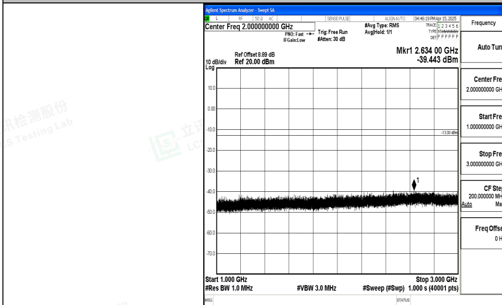
Band5_1.4MHz_QPSK_20643_1RB#0_1000~3000_1000~3000
