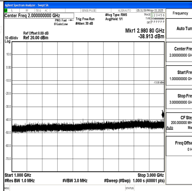
Band5_5MHz_16QAM_20425_1RB#0_1000~3000_1000~3000
