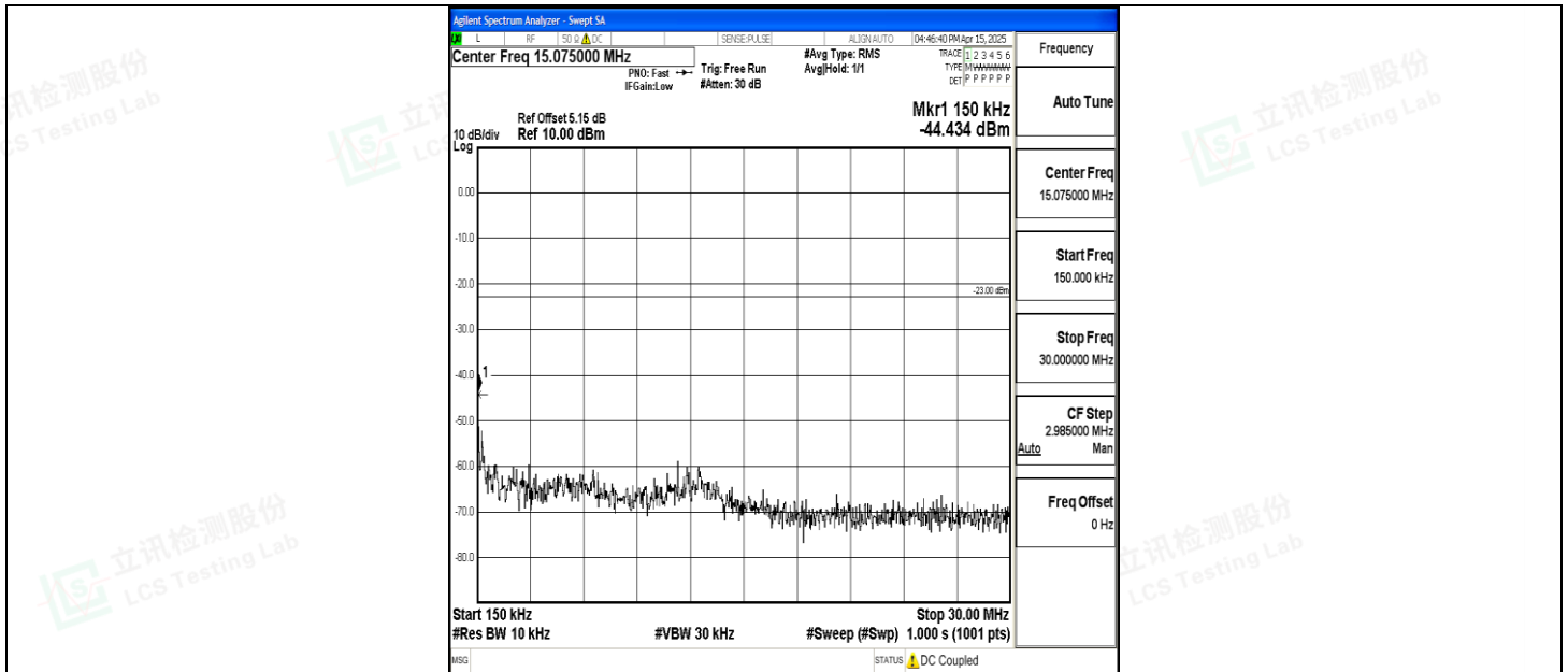
Band5_1.4MHz_16QAM_20643_1RB#0_0.15~30_0.15~30
