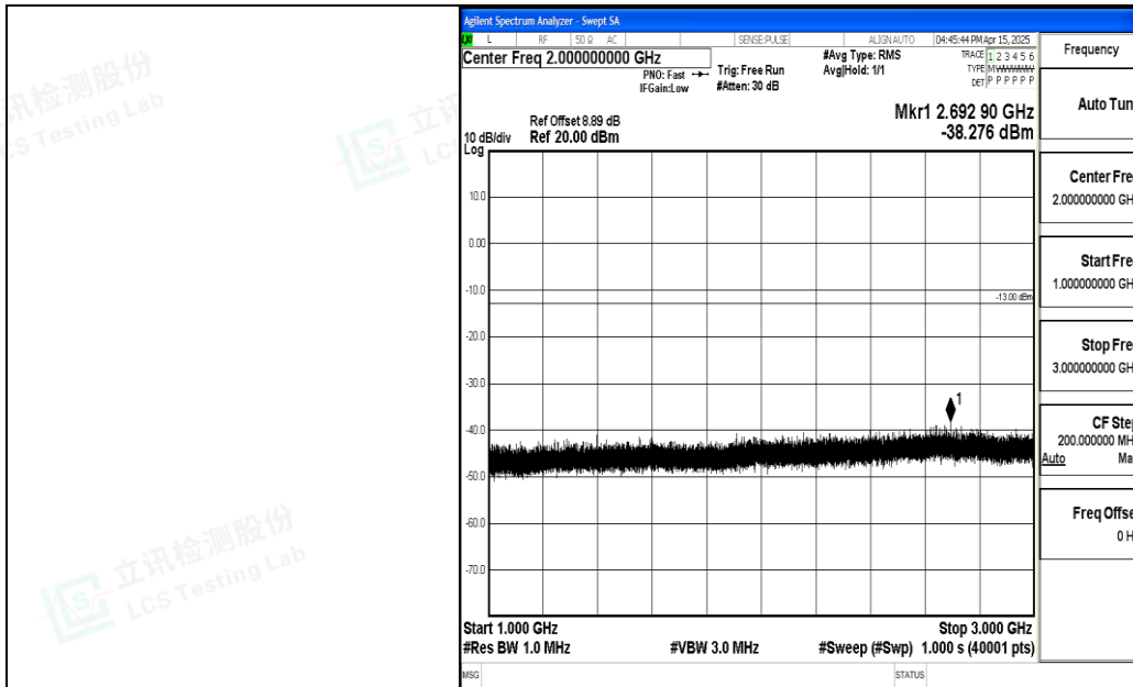
Band5_1.4MHz_16QAM_20525_1RB#0_1000~3000_1000~3000
