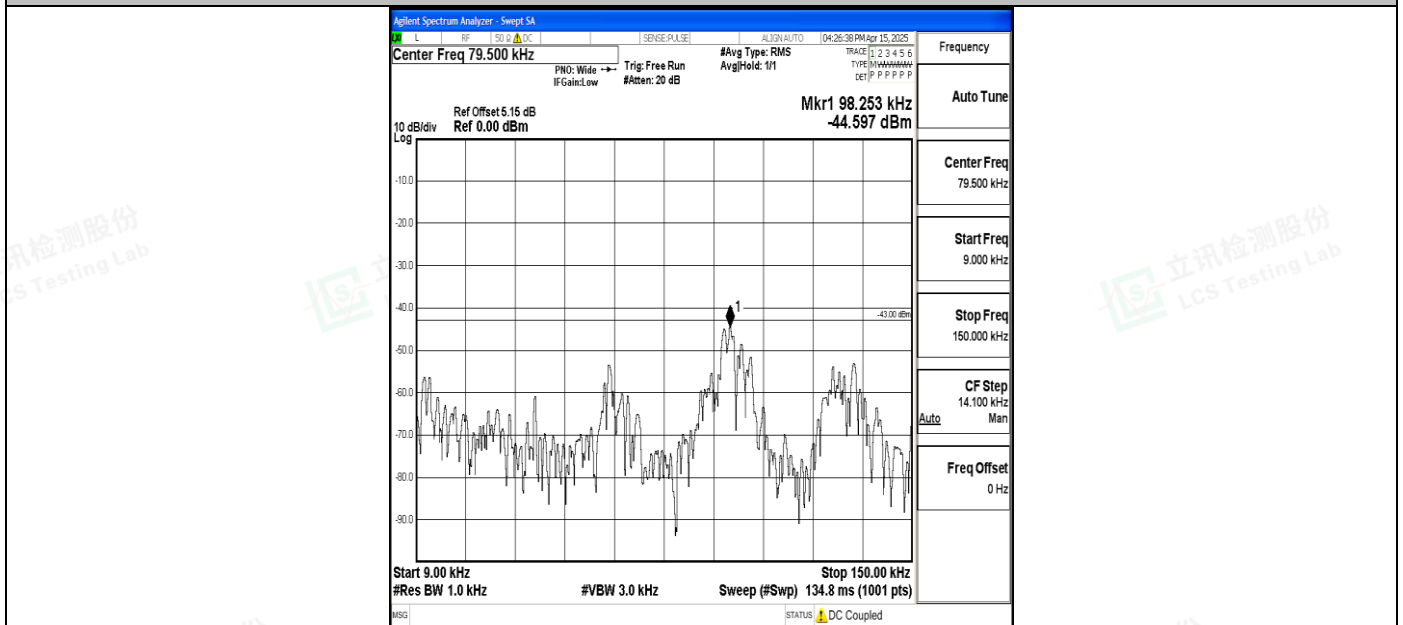
Band4_20MHz_QPSK_20050_1RB#0_0.009~0.15_0.009~0.15
