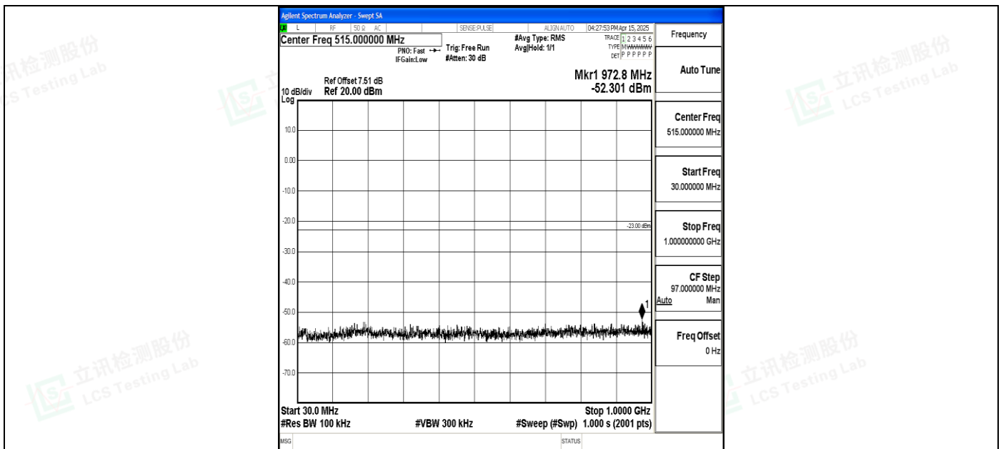
Band4_20MHz_QPSK_20175_1RB#0_30~1000_30~1000
