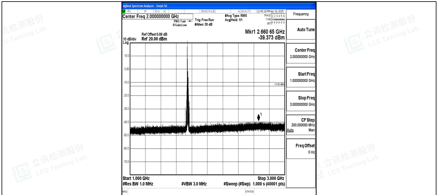
Band4_15MHz_16QAM_20325_1RB#0_1000~3000_1000~3000
