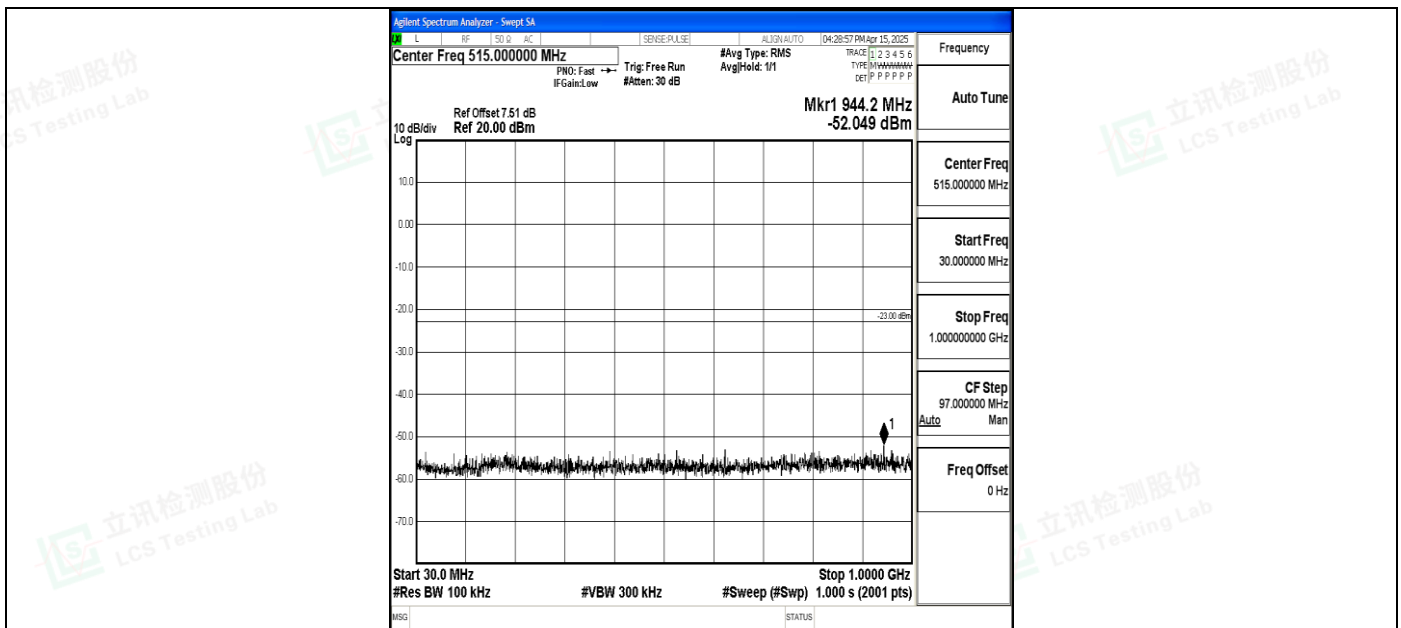
Band4_20MHz_QPSK_20300_1RB#0_30~1000_30~1000
