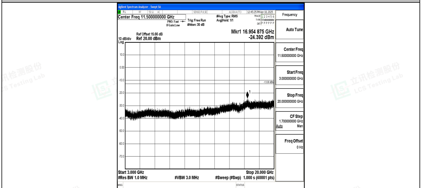
Band4_15MHz_16QAM_20325_1RB#0_3000~20000_3000~20000
