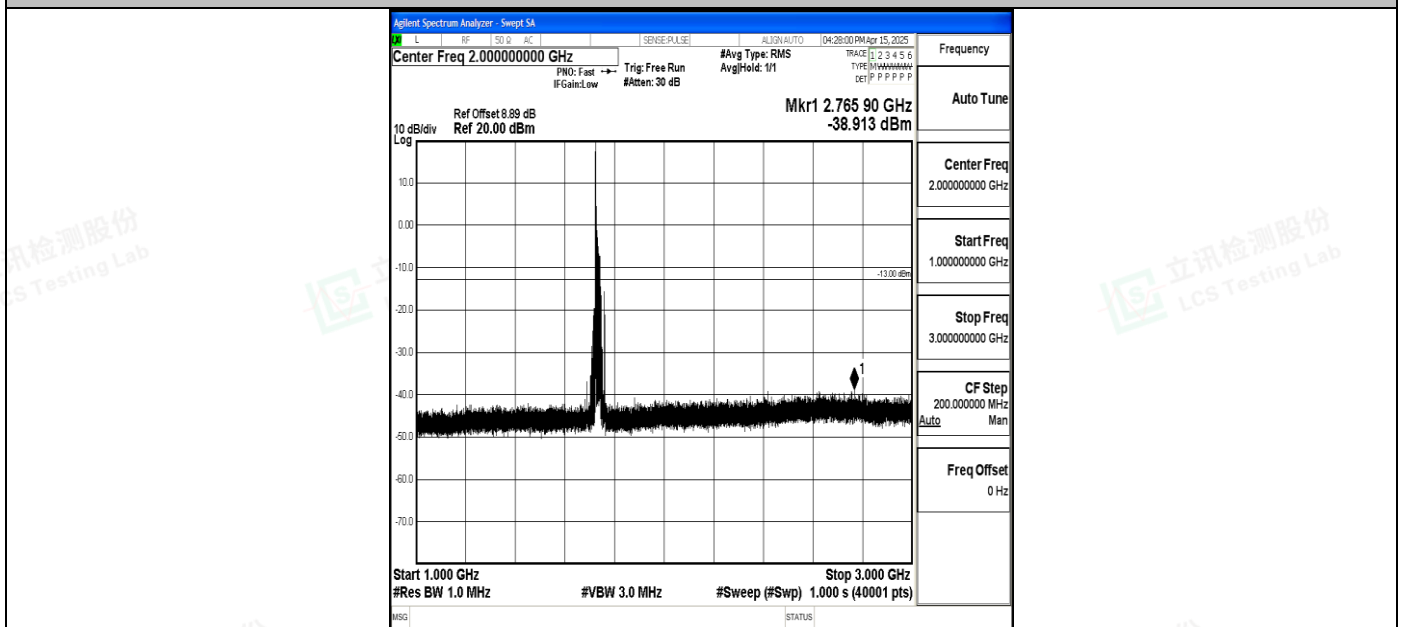
Band4_20MHz_QPSK_20175_1RB#0_1000~3000_1000~3000
