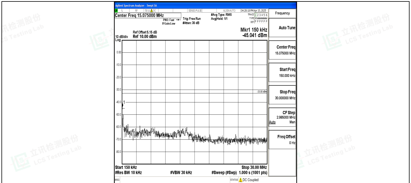
Band4_20MHz_16QAM_20175_1RB#0_0.15~30_0.15~30
