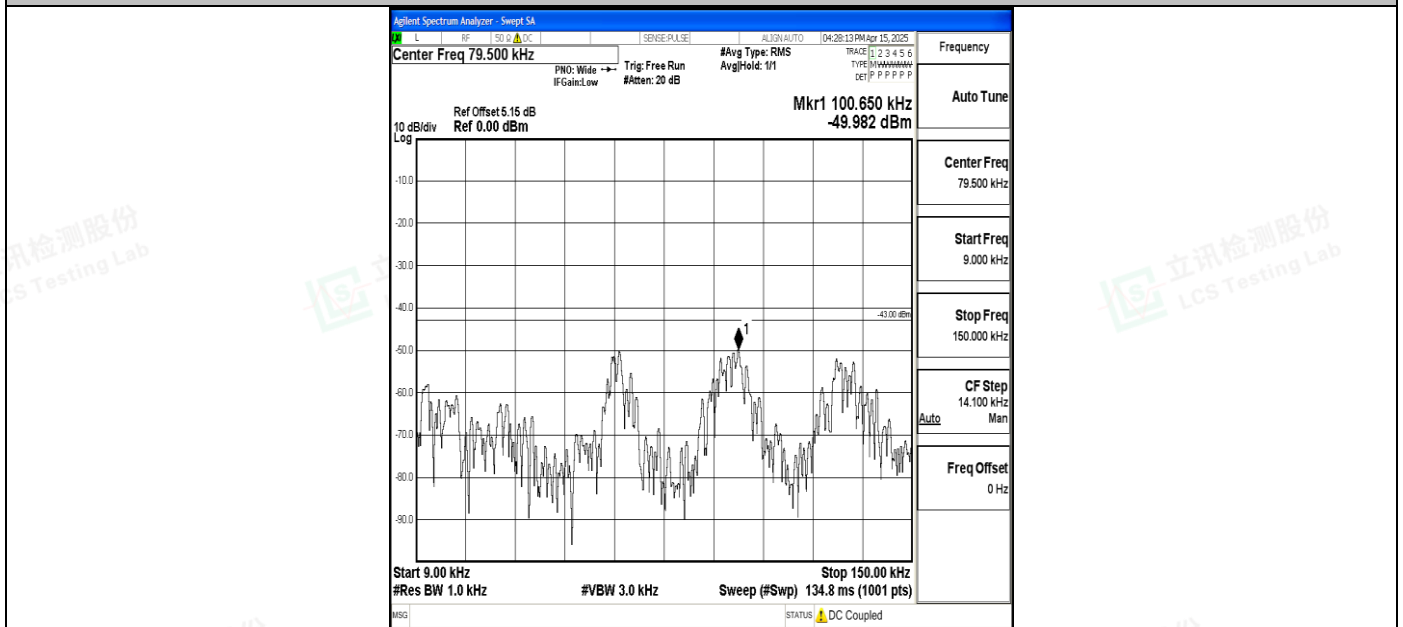
Band4_20MHz_16QAM_20175_1RB#0_0.009~0.15_0.009~0.15
