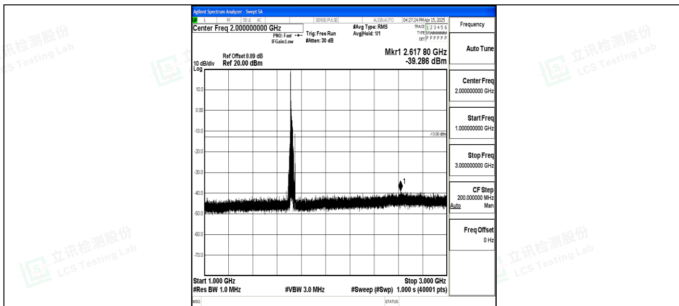
Band4_20MHz_16QAM_20050_1RB#0_1000~3000_1000~3000
