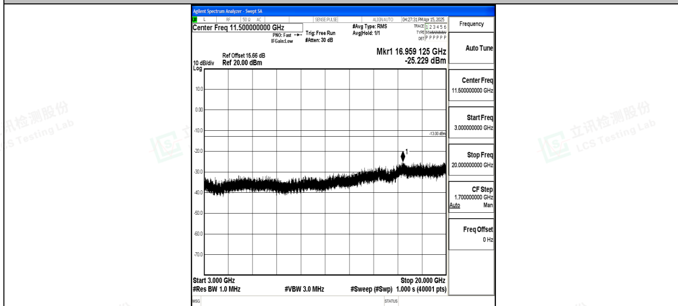
Band4_20MHz_16QAM_20050_1RB#0_3000~20000_3000~20000
