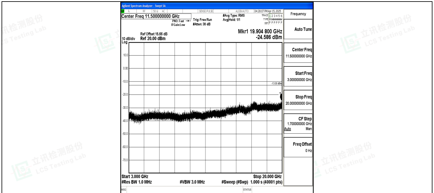
Band4_20MHz_QPSK_20175_1RB#0_3000~20000_3000~20000
