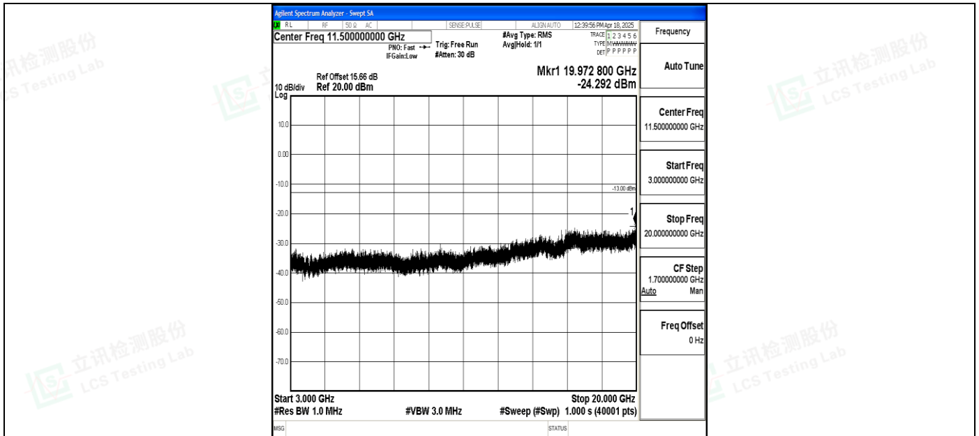
Band4_10MHz_QPSK_20175_1RB#0_3000~20000_3000~20000
