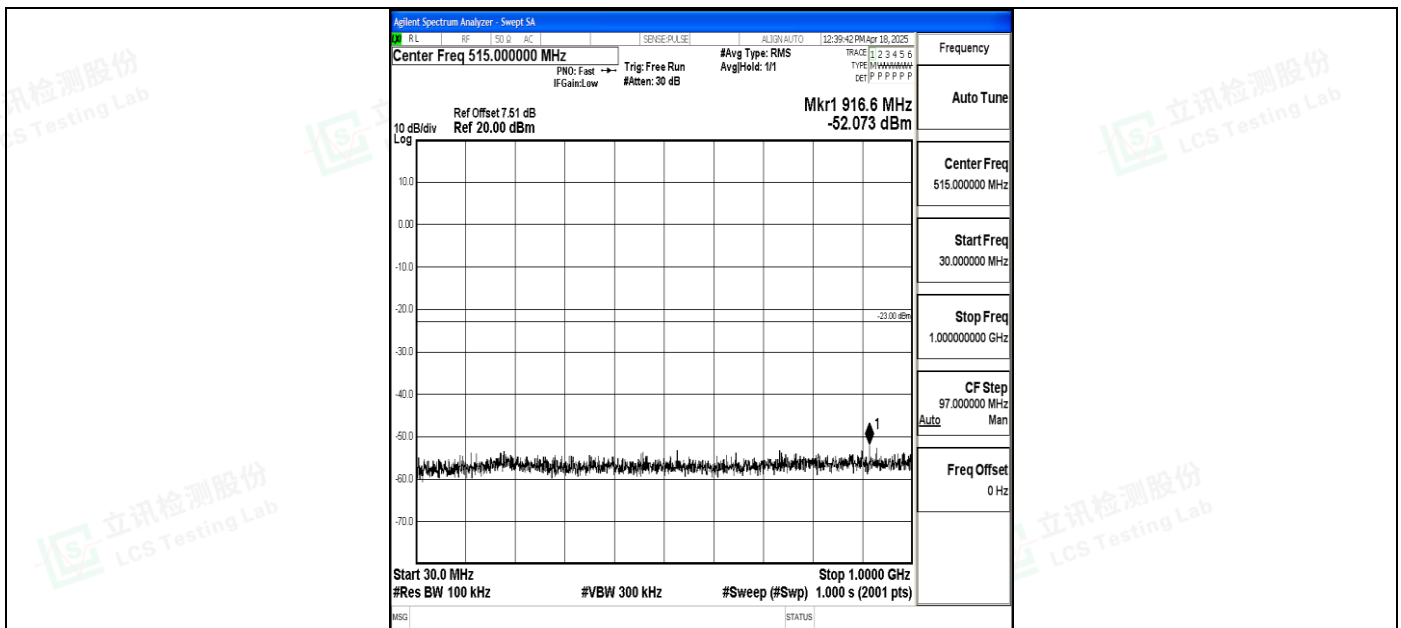
Band4_10MHz_QPSK_20175_1RB#0_30~1000_30~1000
