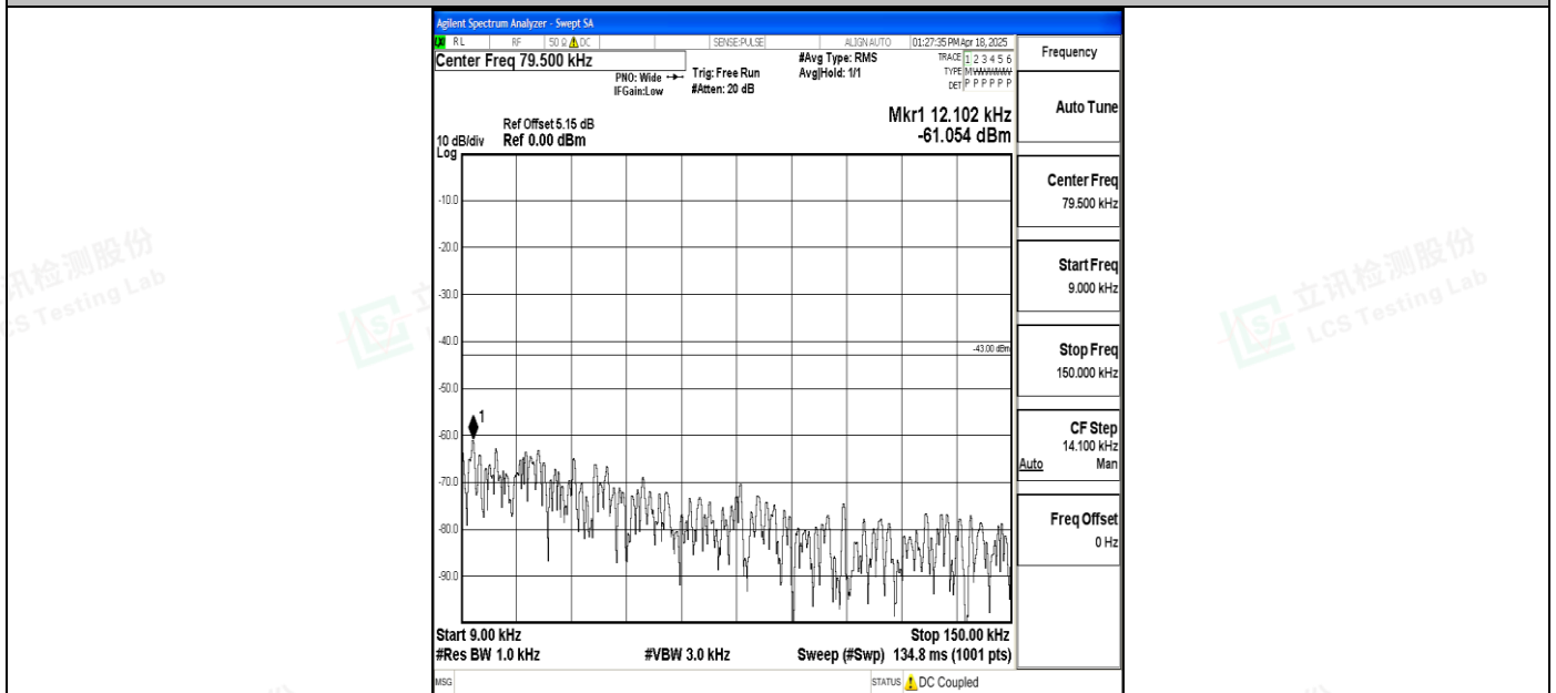
Band4_3MHz_16QAM_20385_1RB#0_0.009~0.15_0.009~0.15
