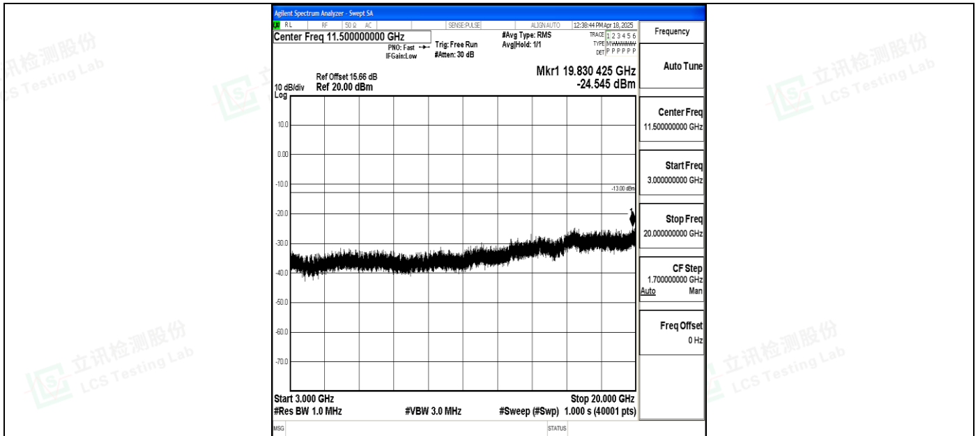
Band4_10MHz_QPSK_20000_1RB#0_3000~20000_3000~20000
