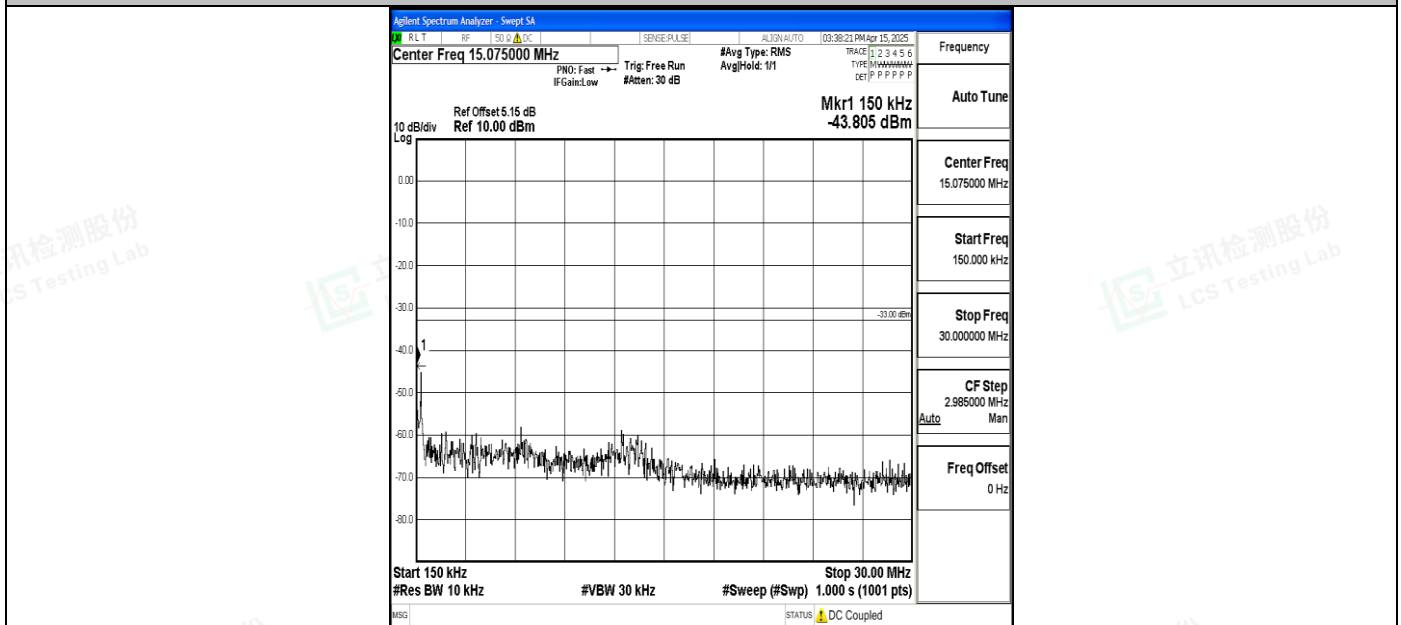
Band4_5MHz_QPSK_20375_1RB#0_0.15~30_0.15~30
