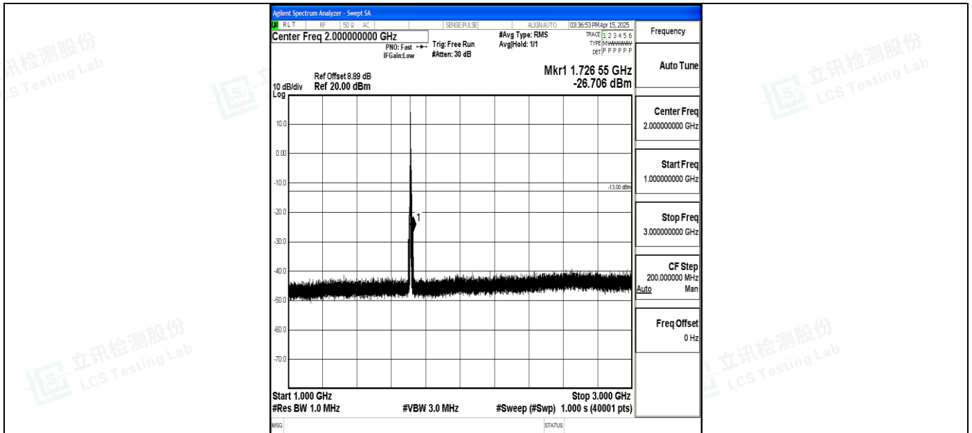
Band4_5MHz_16QAM_19975_1RB#0_1000~3000_1000~3000
