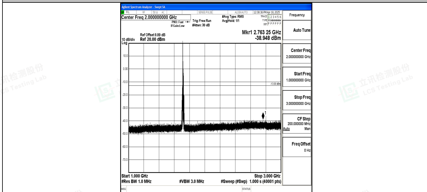
Band4_10MHz_QPSK_20000_1RB#0_1000~3000_1000~3000
