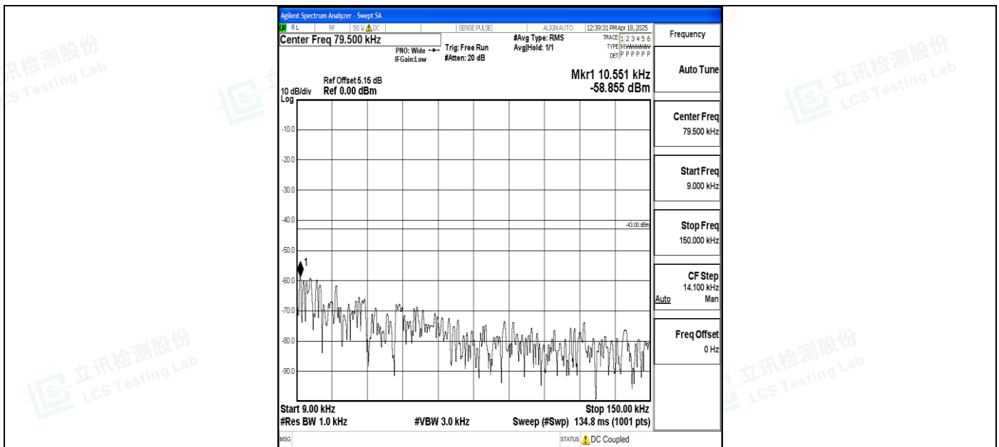
Band4_10MHz_QPSK_20175_1RB#0_0.009~0.15_0.009~0.15
