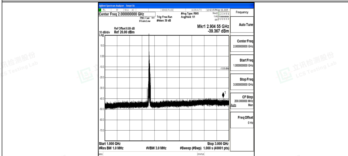
Band4_15MHz_QPSK_20025_1RB#0_1000~3000_1000~3000
