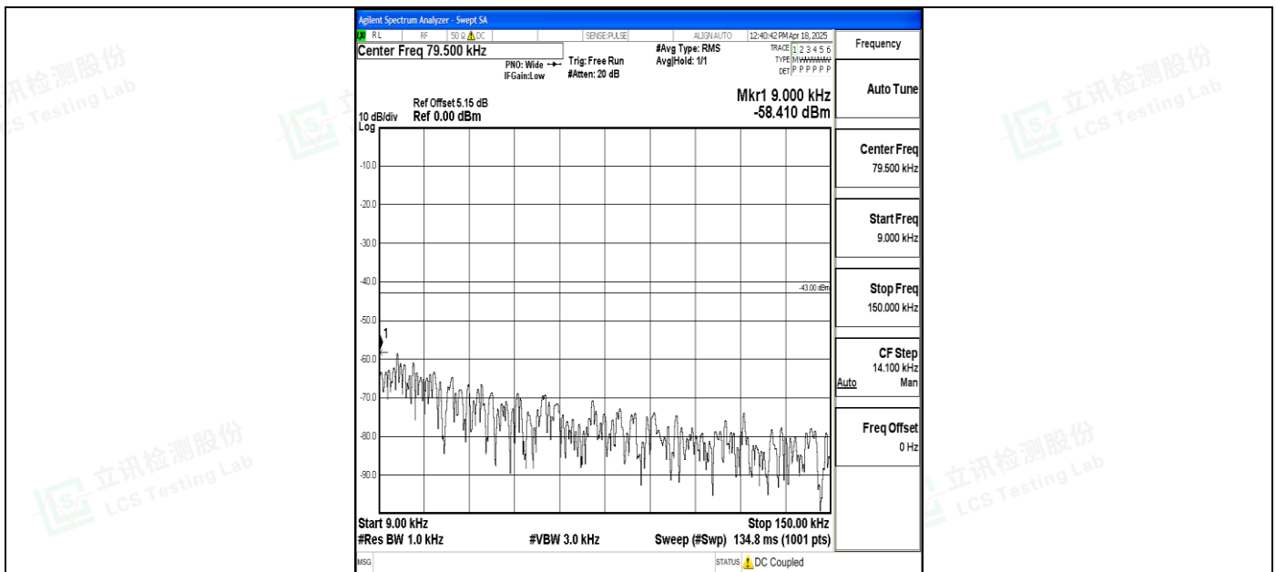
Band4_10MHz_QPSK_20350_1RB#0_0.009~0.15_0.009~0.15
