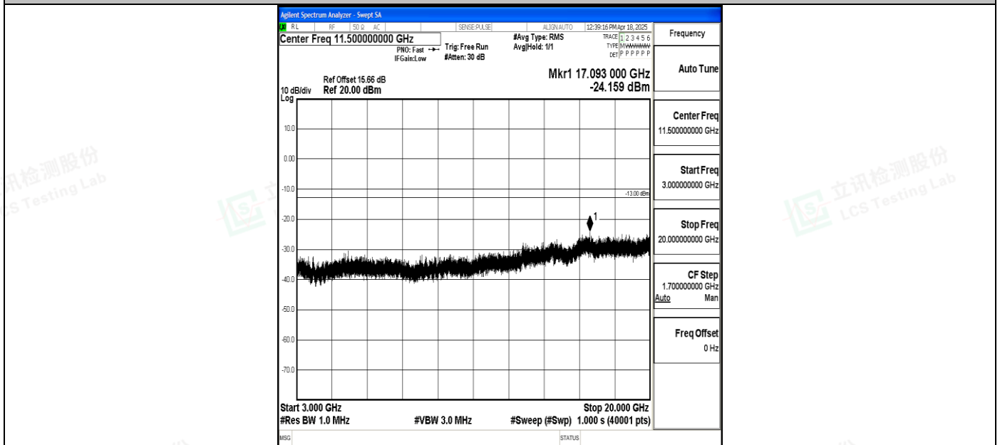
Band4_10MHz_16QAM_20000_1RB#0_3000~20000_3000~20000
