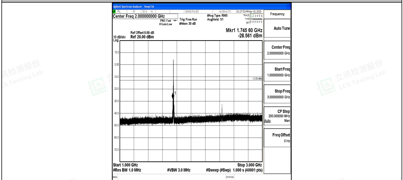
Band4_3MHz_16QAM_20385_1RB#0_1000~3000_1000~3000
