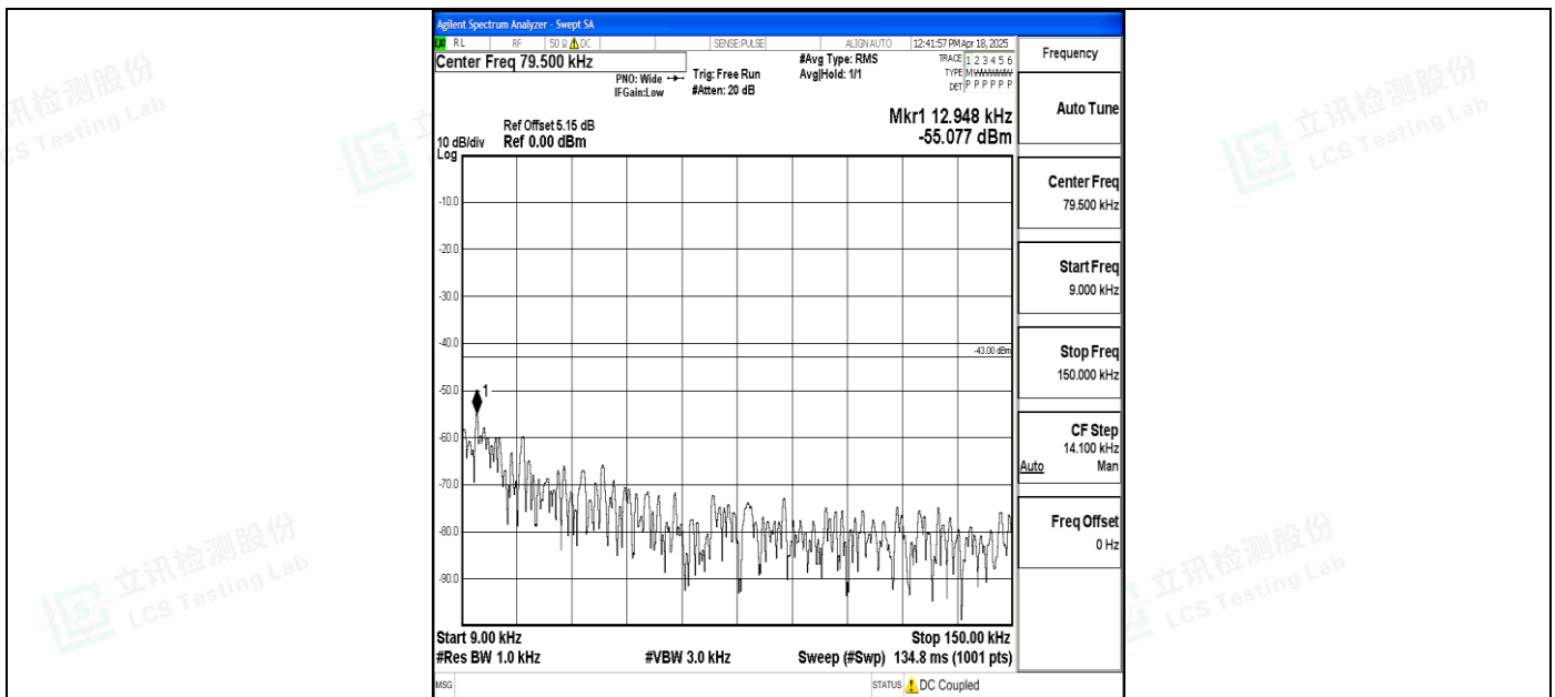
Band4_15MHz_QPSK_20025_1RB#0_0.009~0.15_0.009~0.15
