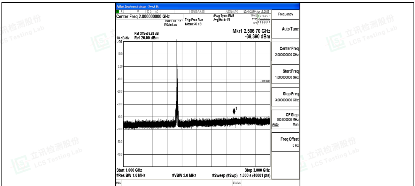
Band4_10MHz_16QAM_20175_1RB#0_1000~3000_1000~3000
