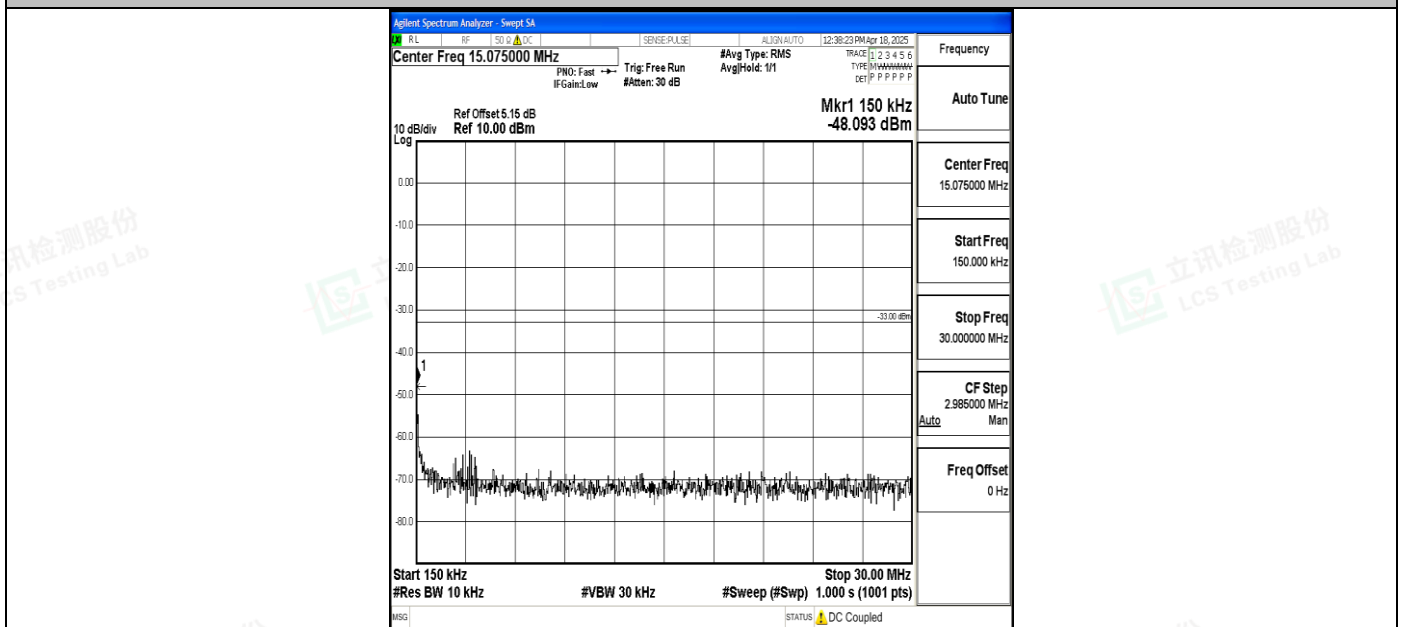
Band4_10MHz_QPSK_20000_1RB#0_0.15~30_0.15~30
