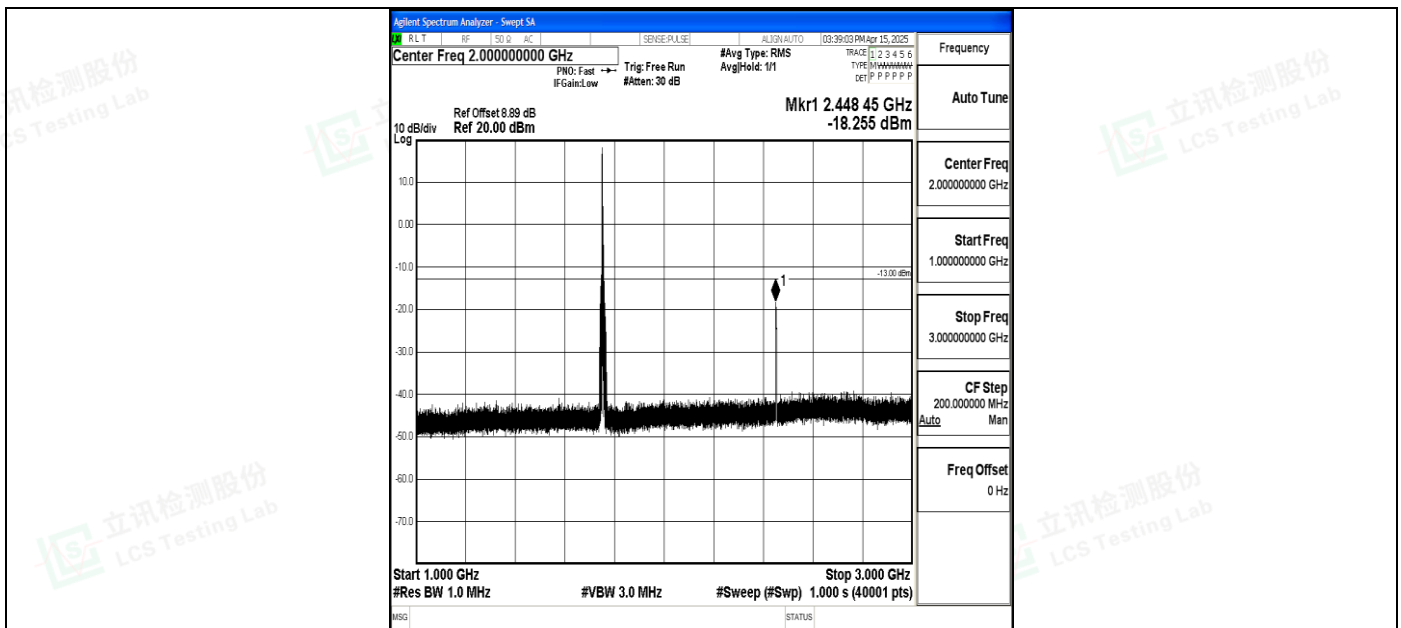
Band4_5MHz_16QAM_20375_1RB#0_1000~3000_1000~3000
