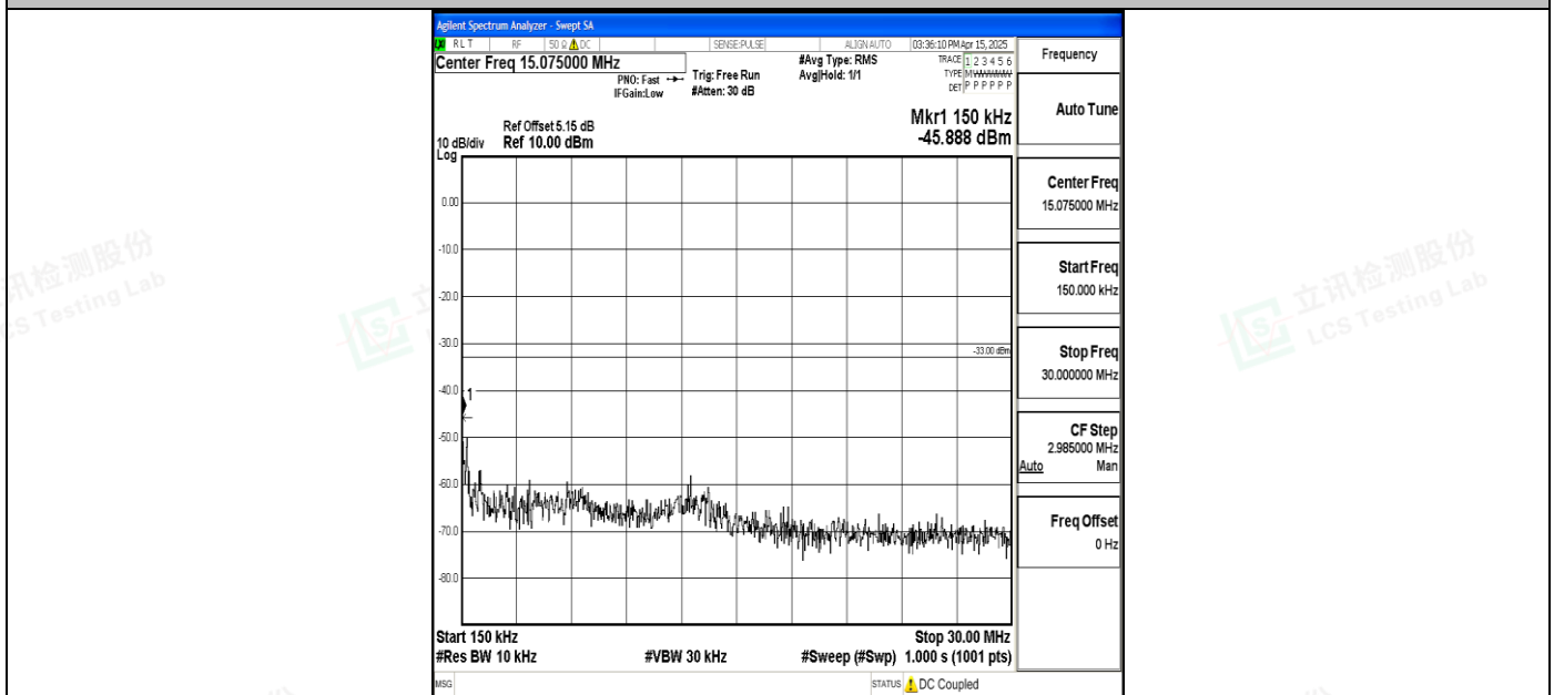
Band4_5MHz_QPSK_19975_1RB#0_0.15~30_0.15~30
