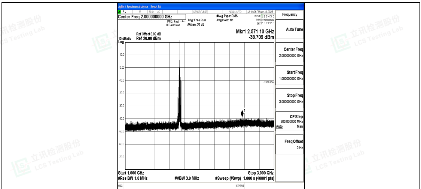
Band4_15MHz_16QAM_20175_1RB#0_1000~3000_1000~3000
