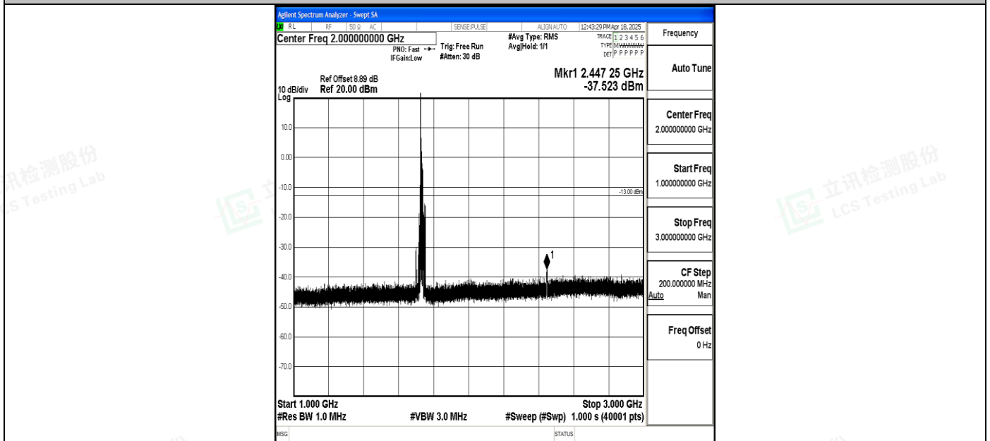
Band4_15MHz_QPSK_20175_1RB#0_1000~3000_1000~3000
