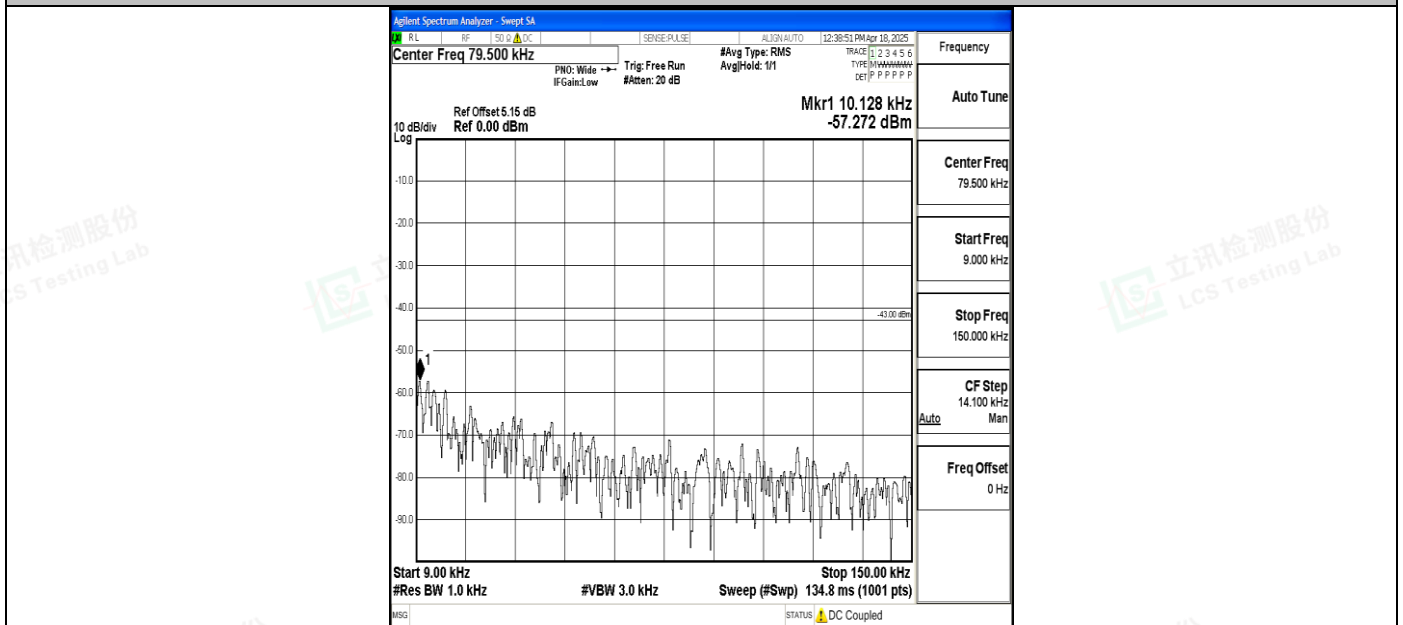
Band4_10MHz_16QAM_20000_1RB#0_0.009~0.15_0.009~0.15
