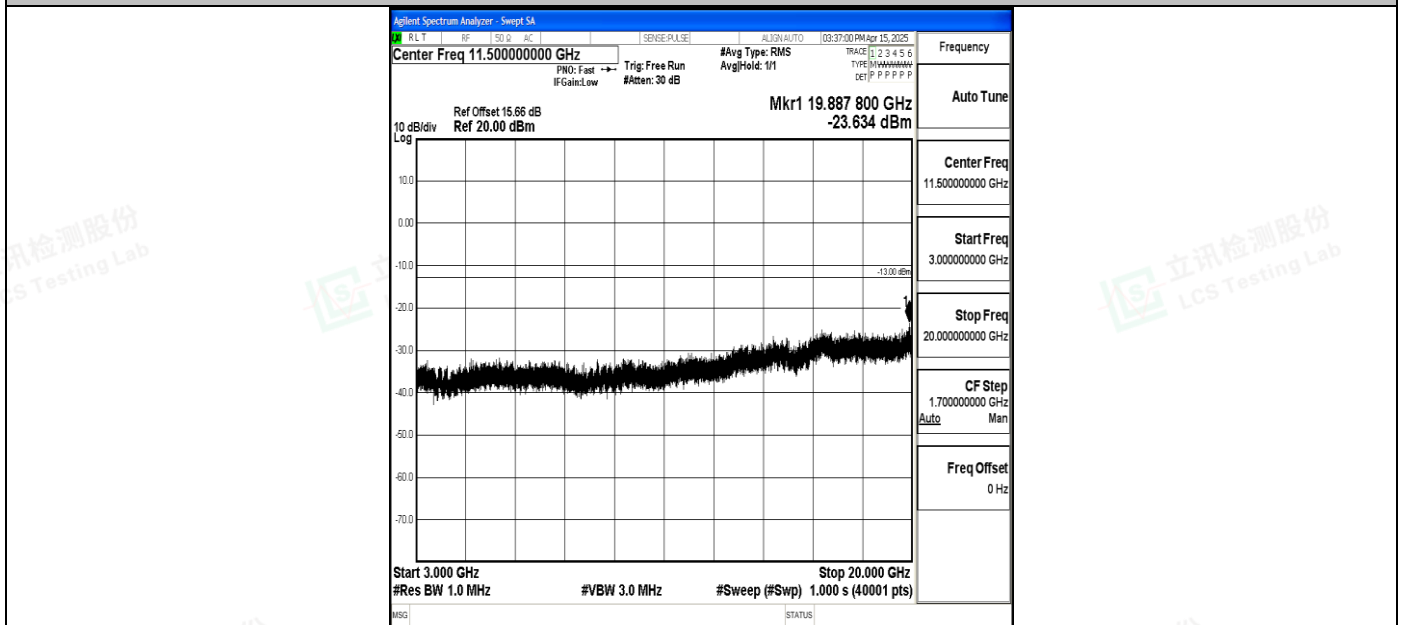
Band4_5MHz_16QAM_19975_1RB#0_3000~20000_3000~20000
