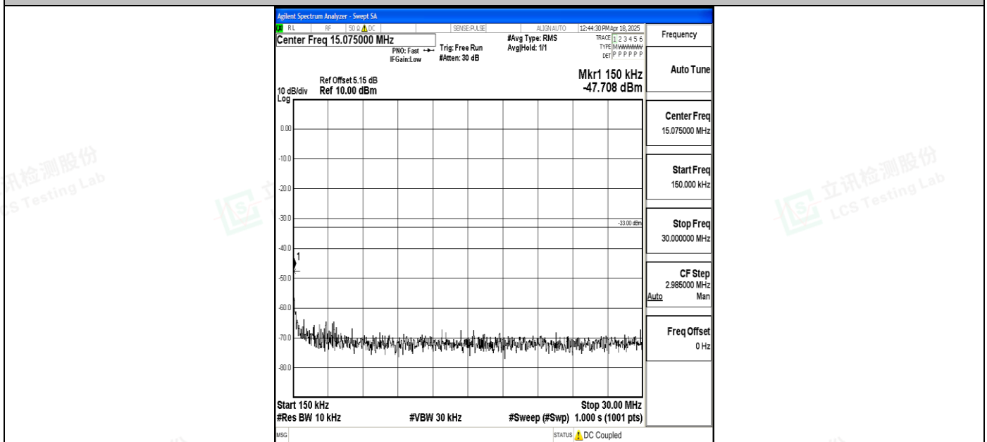
Band4_15MHz_QPSK_20325_1RB#0_0.15~30_0.15~30
