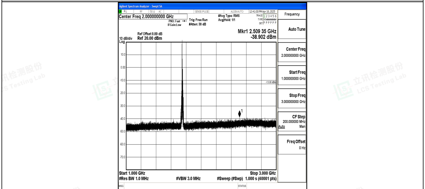
Band4_10MHz_QPSK_20350_1RB#0_1000~3000_1000~3000
