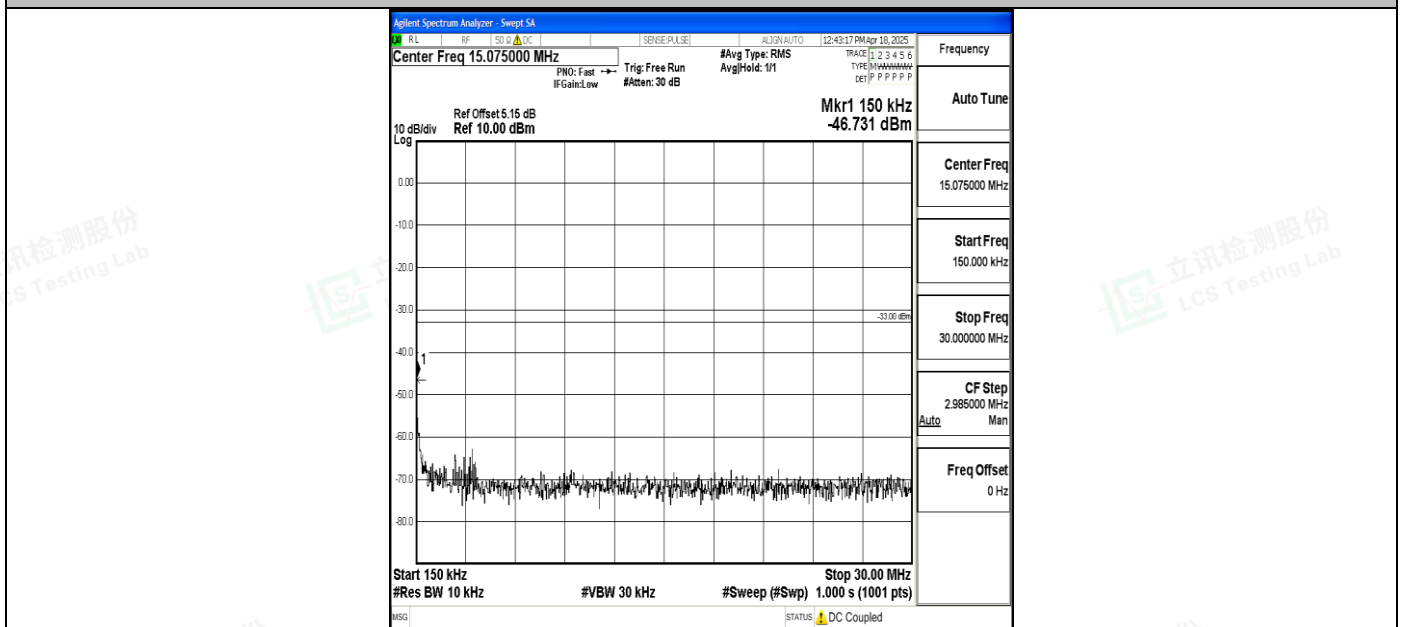
Band4_15MHz_QPSK_20175_1RB#0_0.15~30_0.15~30
