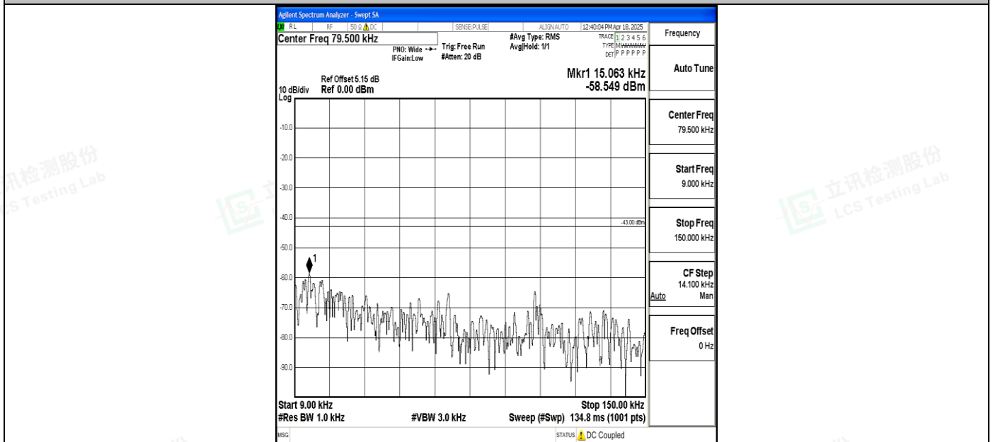
Band4_10MHz_16QAM_20175_1RB#0_0.009~0.15_0.009~0.15
