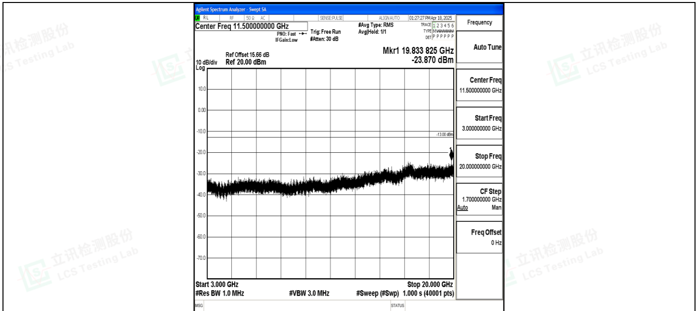
Band4_3MHz_QPSK_20385_1RB#0_3000~20000_3000~20000
