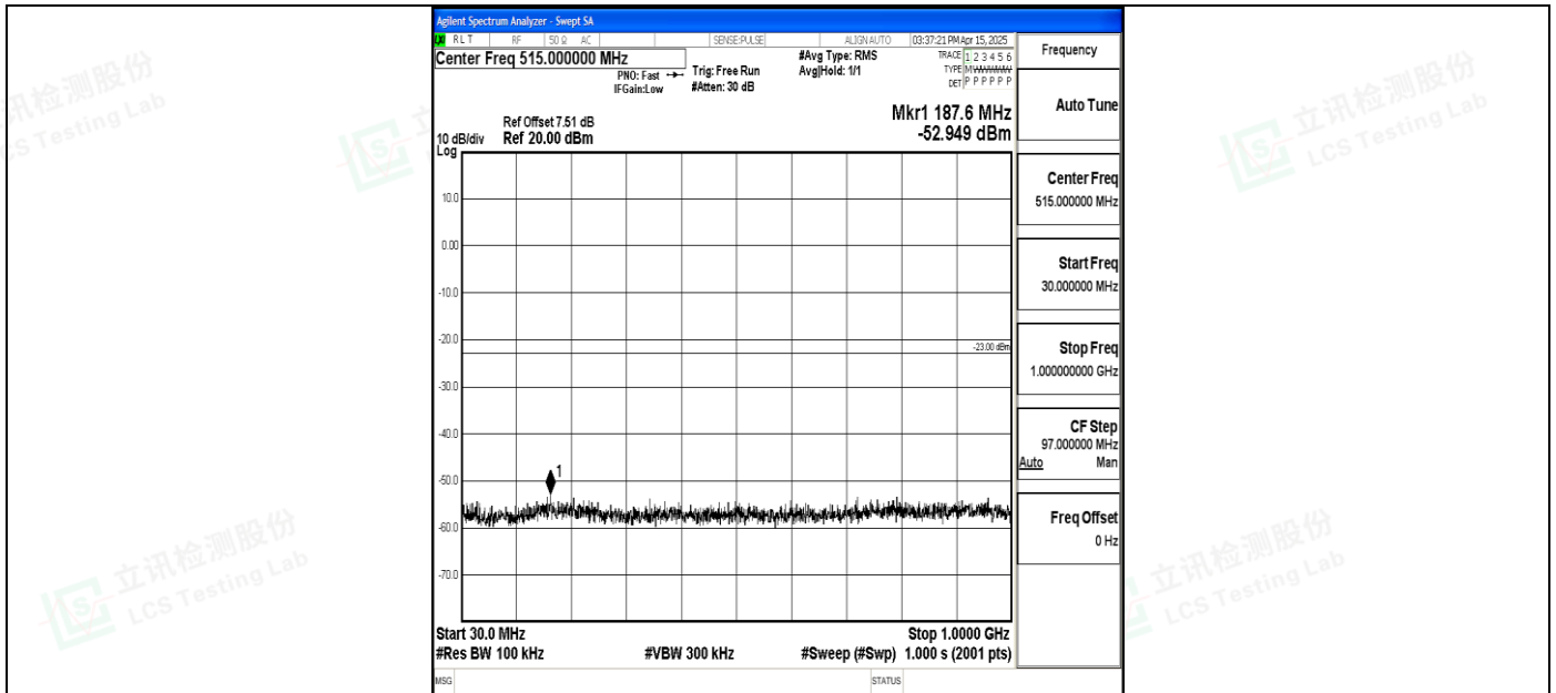
Band4_5MHz_QPSK_20175_1RB#0_30~1000_30~1000
