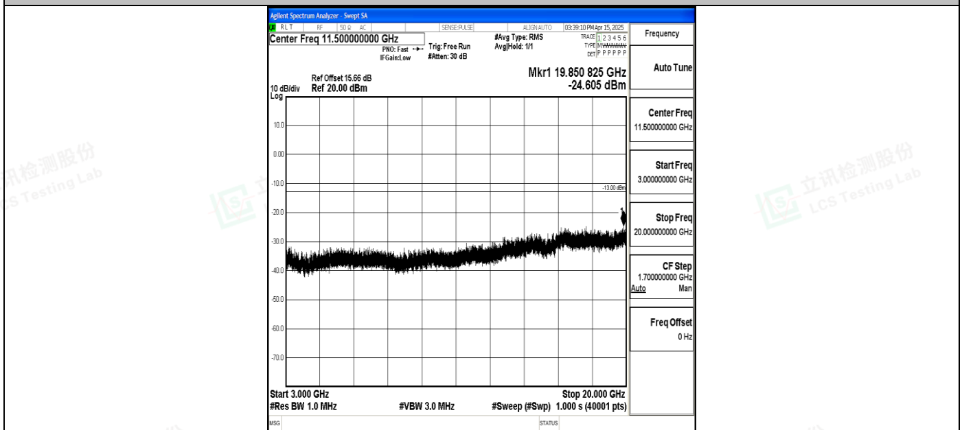
Band4_5MHz_16QAM_20375_1RB#0_3000~20000_3000~20000
