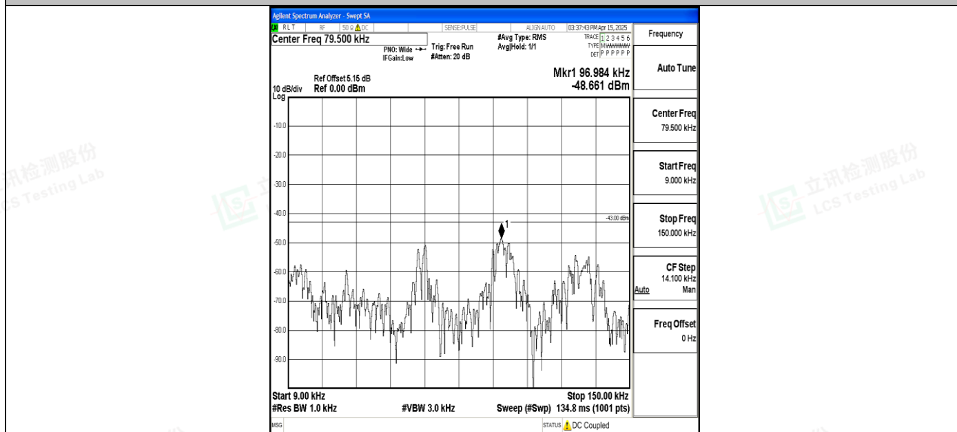
Band4_5MHz_16QAM_20175_1RB#0_0.009~0.15_0.009~0.15
