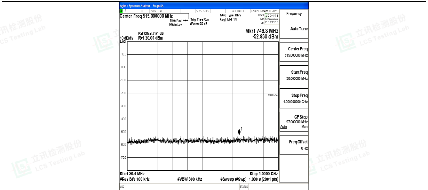
Band4_10MHz_QPSK_20350_1RB#0_30~1000_30~1000
