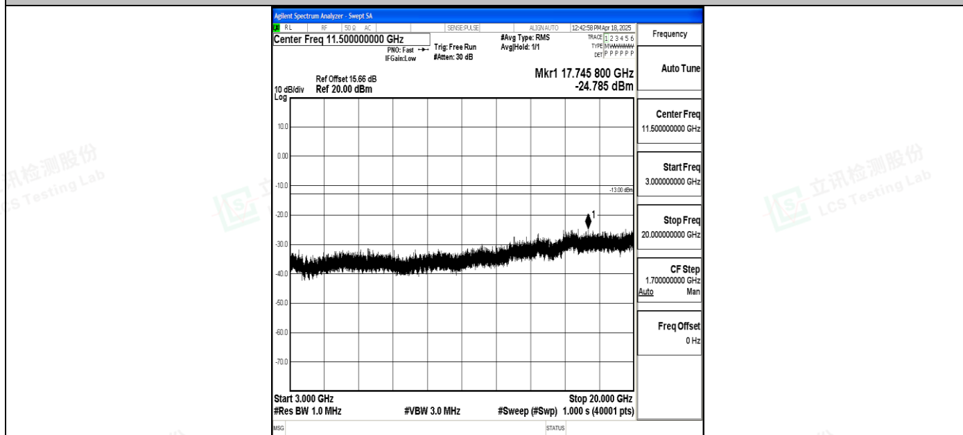
Band4_15MHz_16QAM_20025_1RB#0_3000~20000_3000~20000
