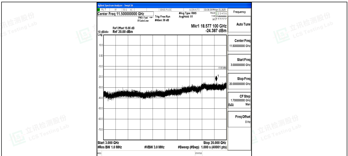
Band4_5MHz_QPSK_20375_1RB#0_3000~20000_3000~20000
