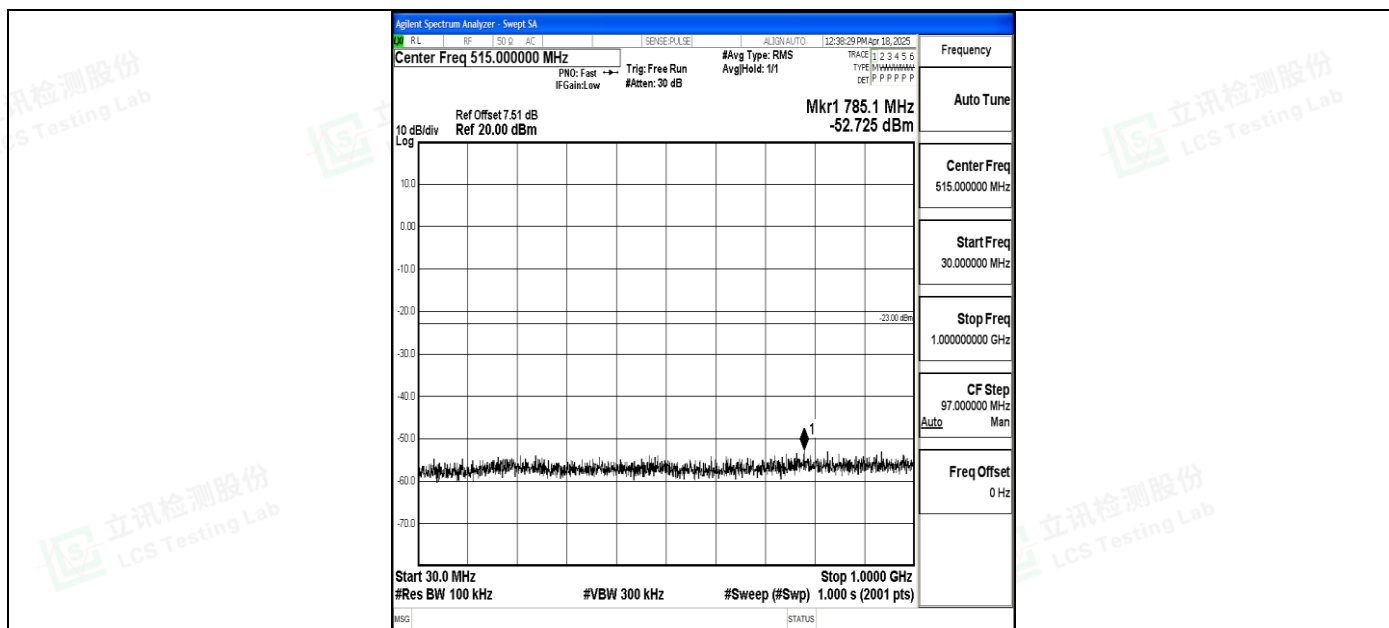
Band4_10MHz_QPSK_20000_1RB#0_30~1000_30~1000
