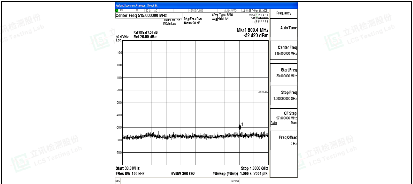
Band4_15MHz_QPSK_20325_1RB#0_30~1000_30~1000
