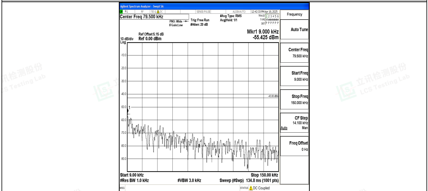
Band4_15MHz_16QAM_20025_1RB#0_0.009~0.15_0.009~0.15
