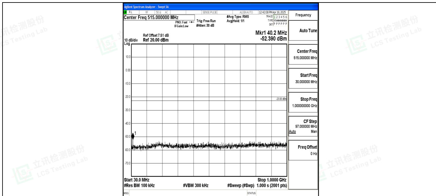
Band4_15MHz_QPSK_20025_1RB#0_30~1000_30~1000
