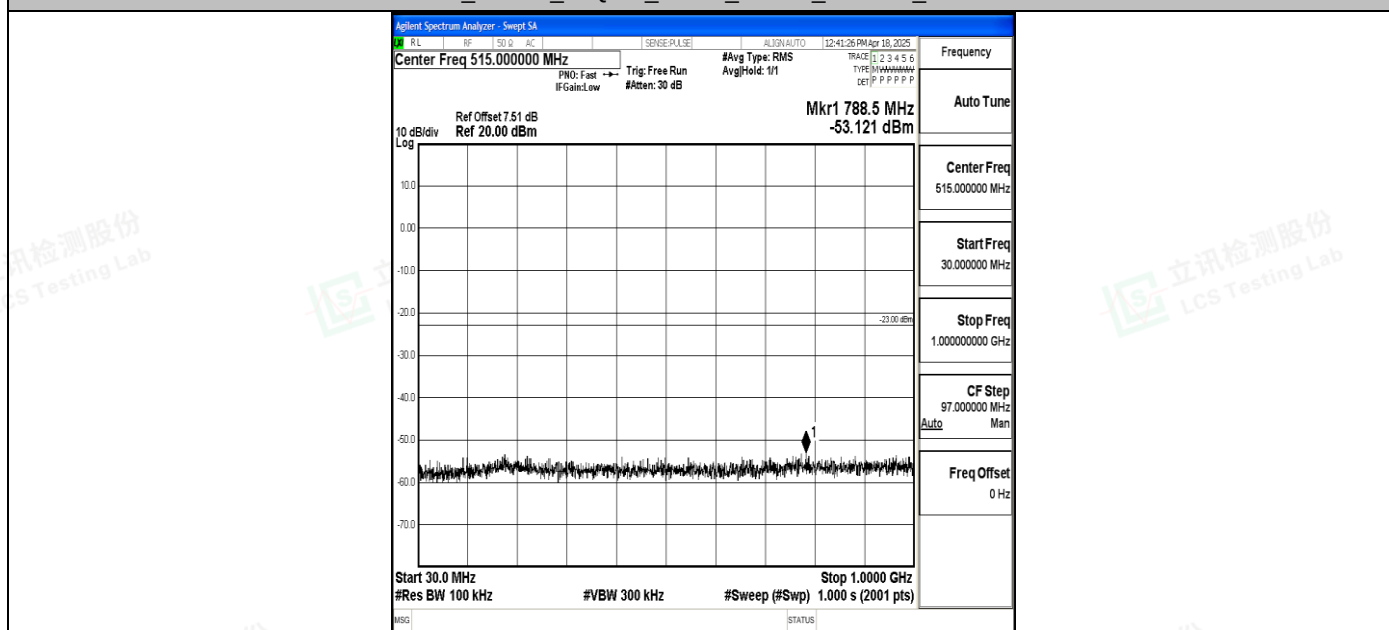
Band4_10MHz_16QAM_20350_1RB#0_30~1000_30~1000
