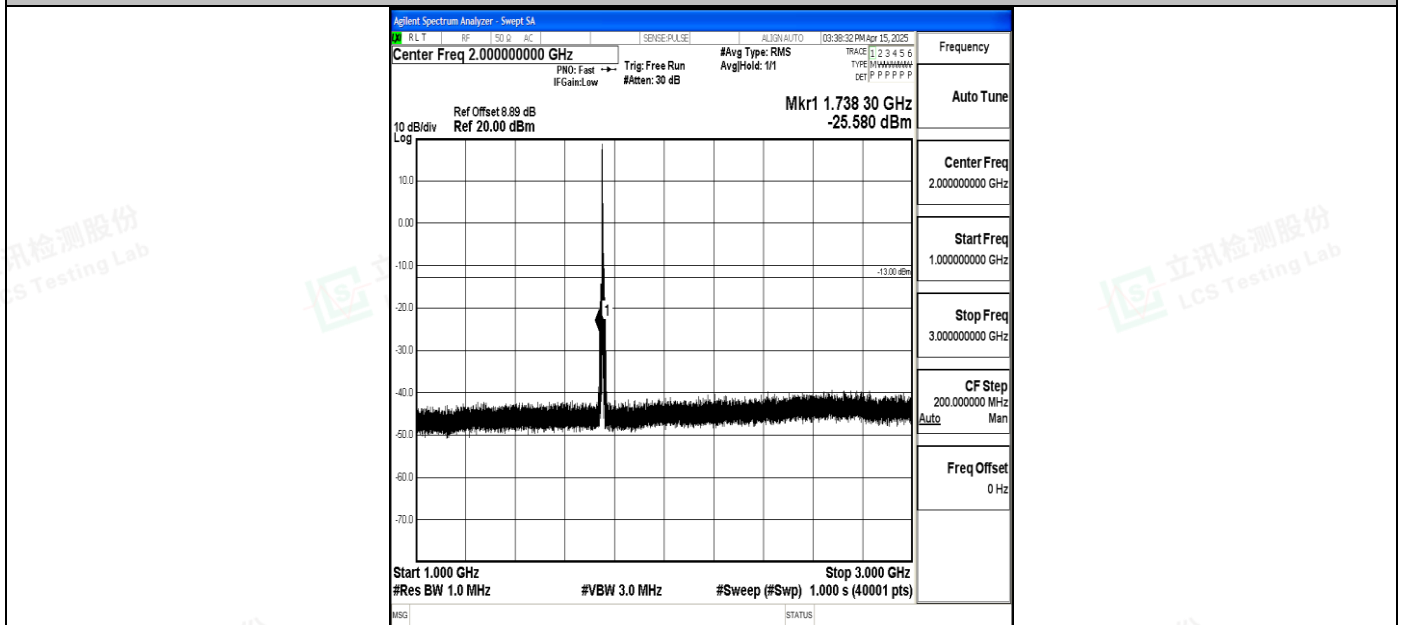
Band4_5MHz_QPSK_20375_1RB#0_1000~3000_1000~3000
