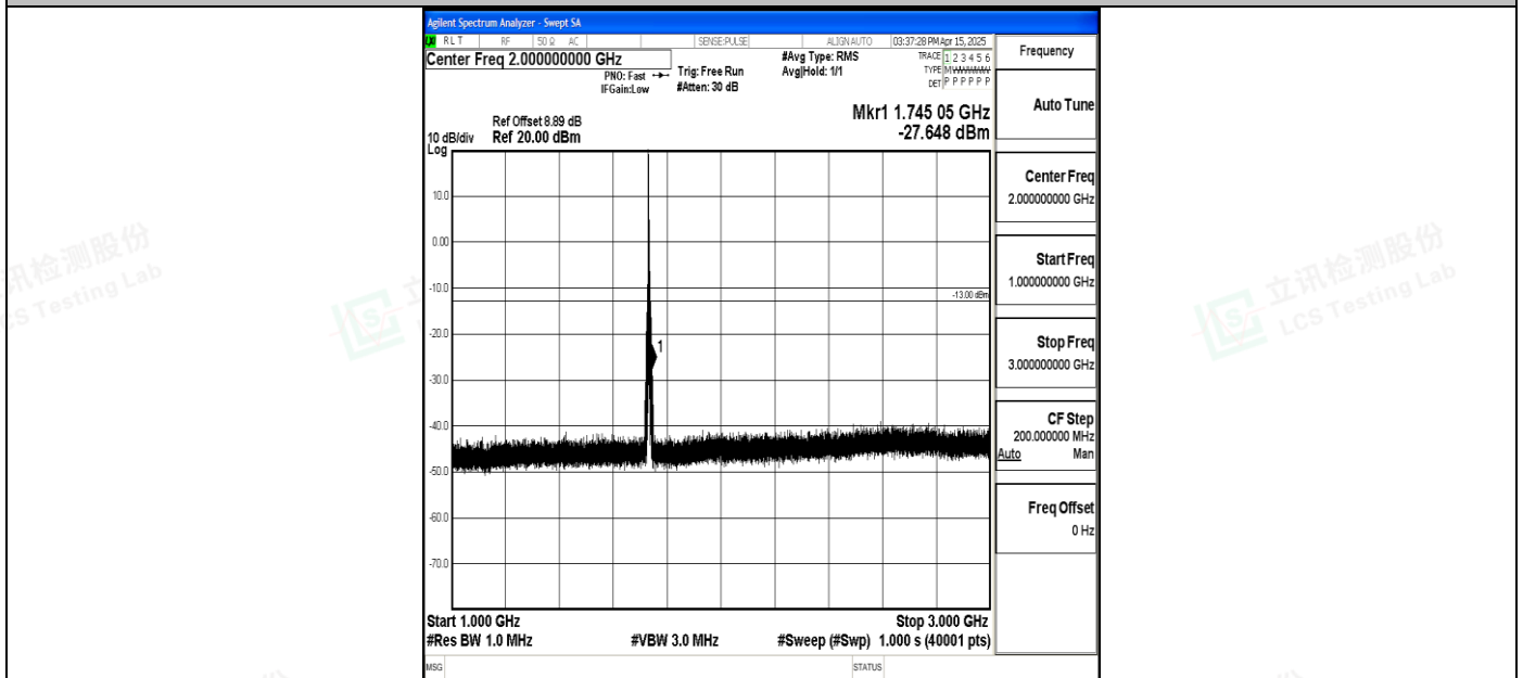
Band4_5MHz_QPSK_20175_1RB#0_1000~3000_1000~3000
