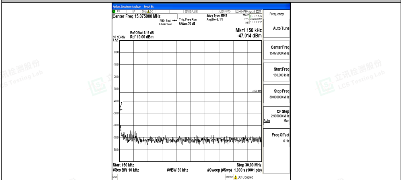
Band4_10MHz_QPSK_20350_1RB#0_0.15~30_0.15~30
