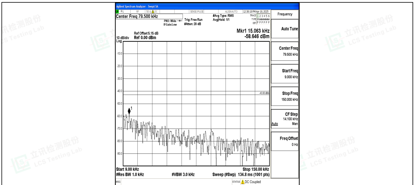
Band4_10MHz_QPSK_20000_1RB#0_0.009~0.15_0.009~0.15
