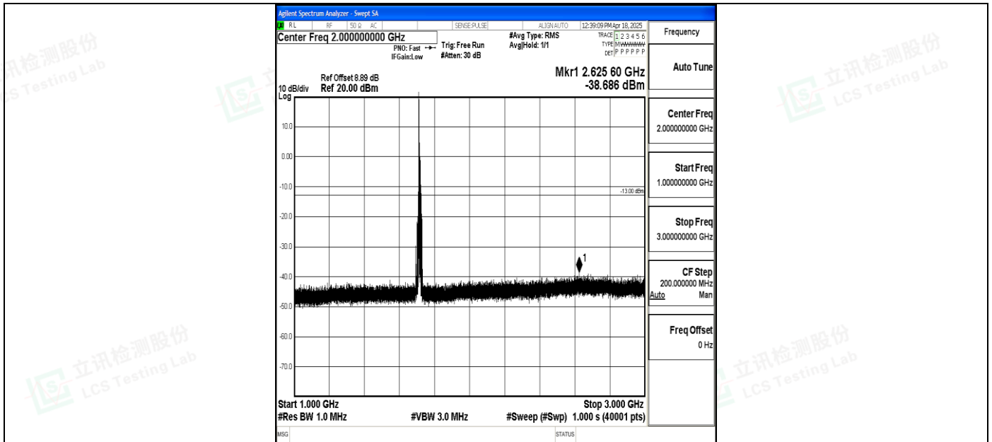
Band4_10MHz_16QAM_20000_1RB#0_1000~3000_1000~3000
