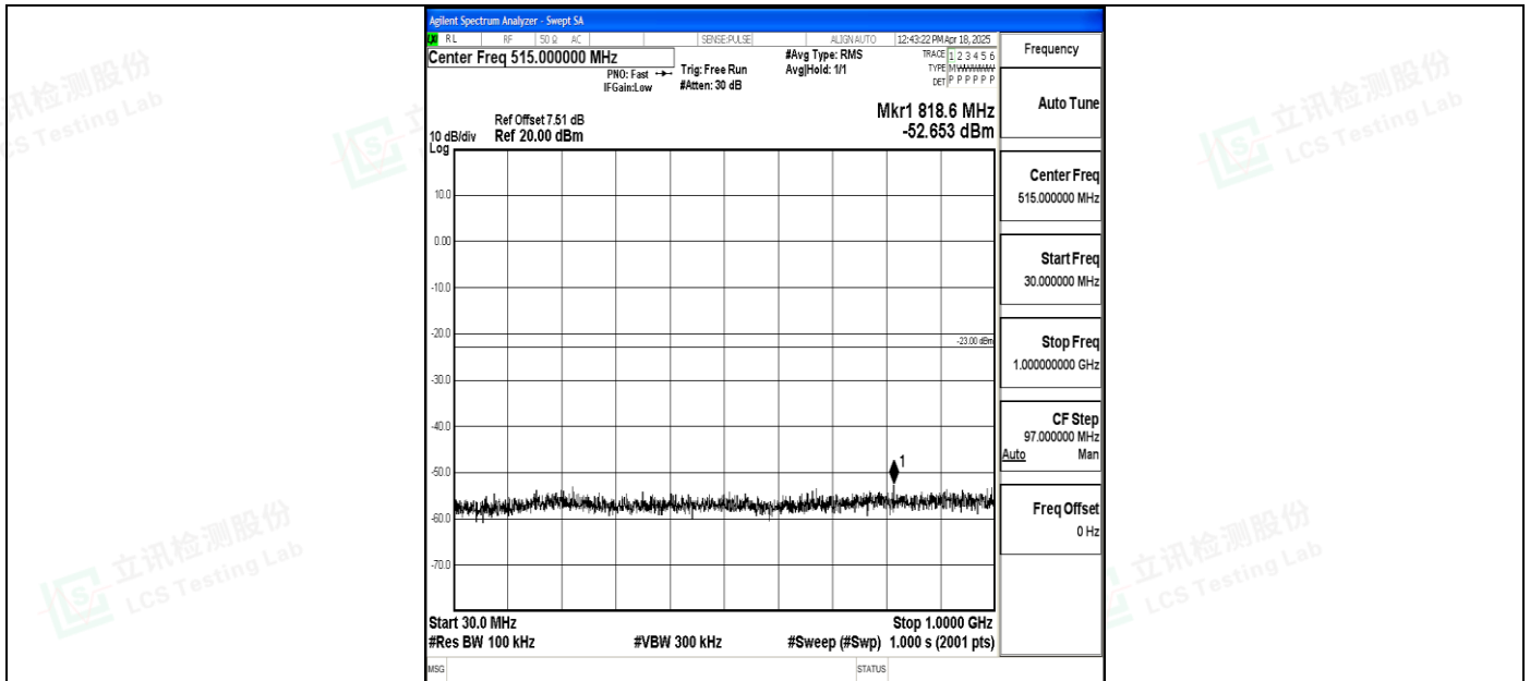
Band4_15MHz_QPSK_20175_1RB#0_30~1000_30~1000
