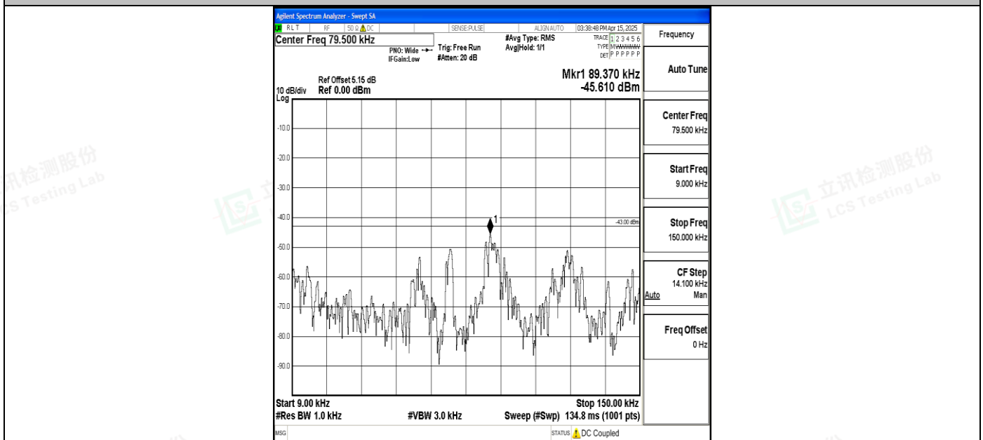
Band4_5MHz_16QAM_20375_1RB#0_0.009~0.15_0.009~0.15
