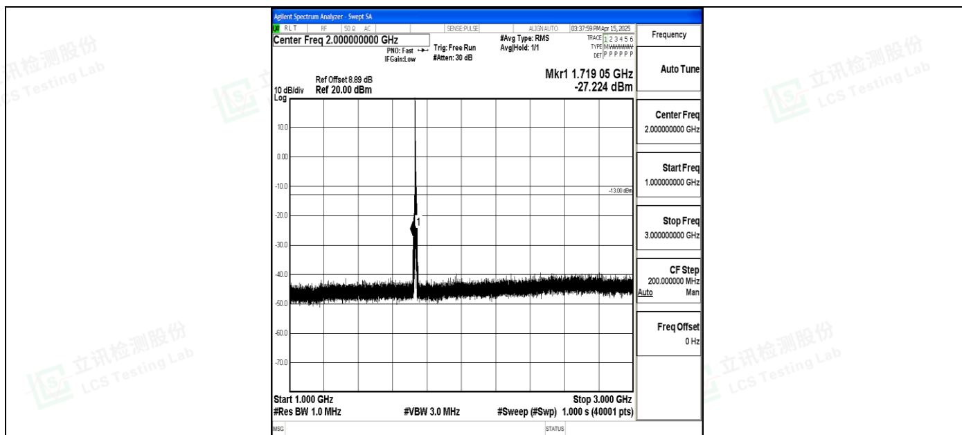
Band4_5MHz_16QAM_20175_1RB#0_1000~3000_1000~3000
