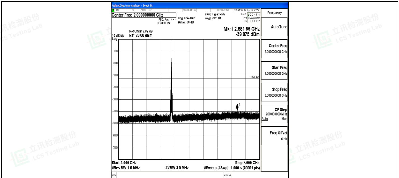
Band4_10MHz_16QAM_20350_1RB#0_1000~3000_1000~3000
