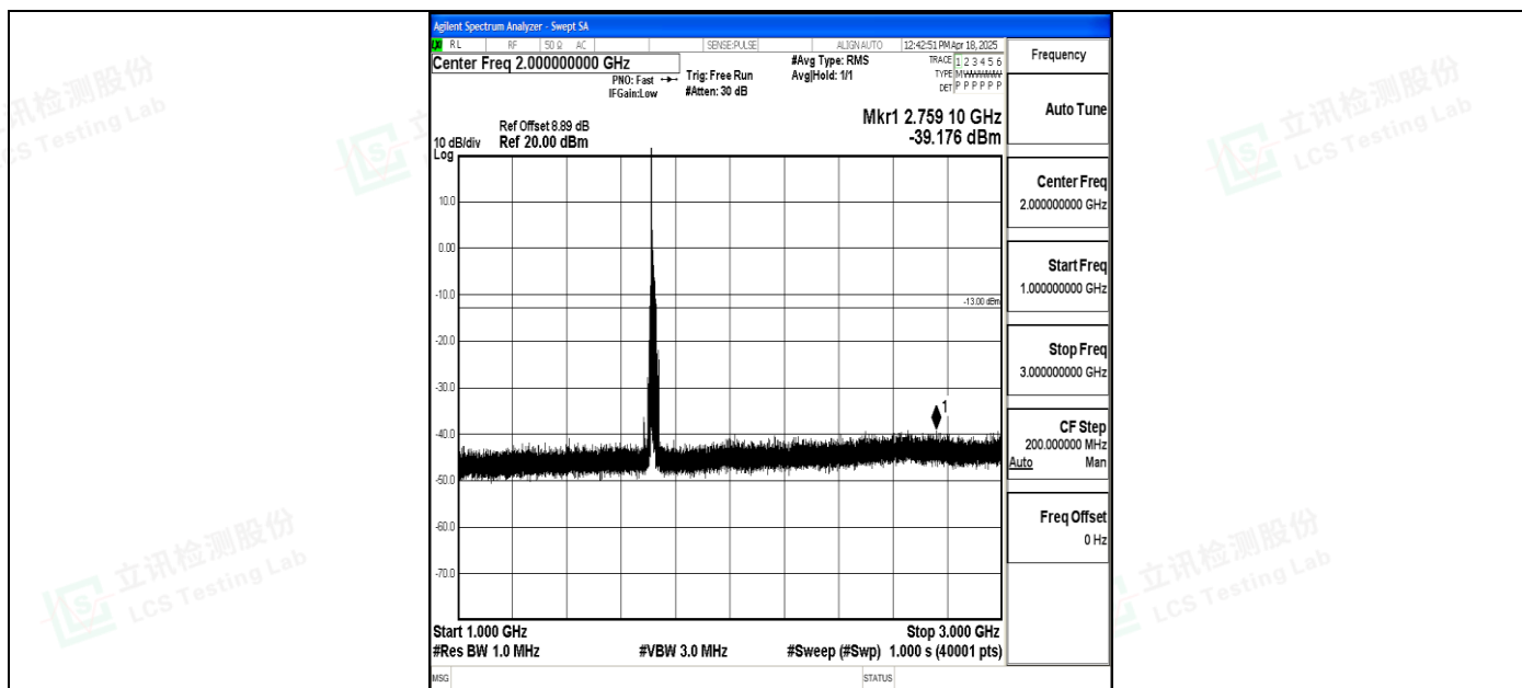
Band4_15MHz_16QAM_20025_1RB#0_1000~3000_1000~3000
