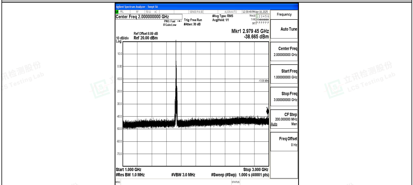
Band4_10MHz_QPSK_20175_1RB#0_1000~3000_1000~3000
