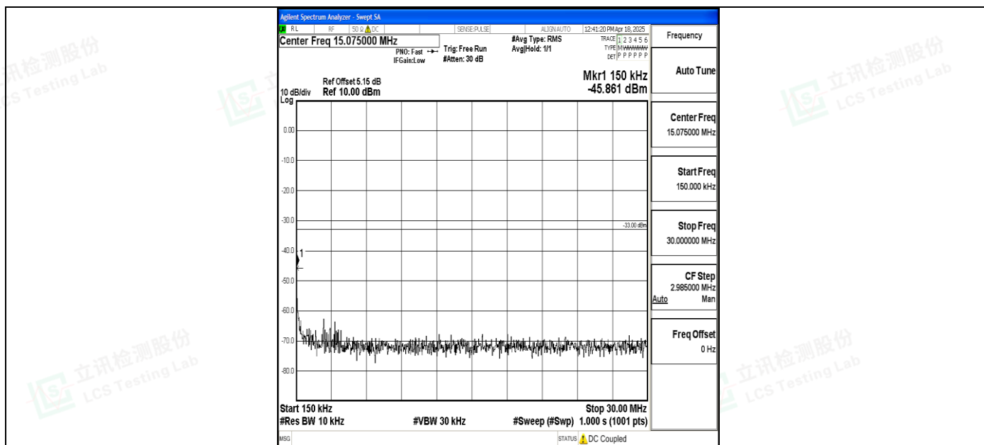
Band4_10MHz_16QAM_20350_1RB#0_0.15~30_0.15~30
