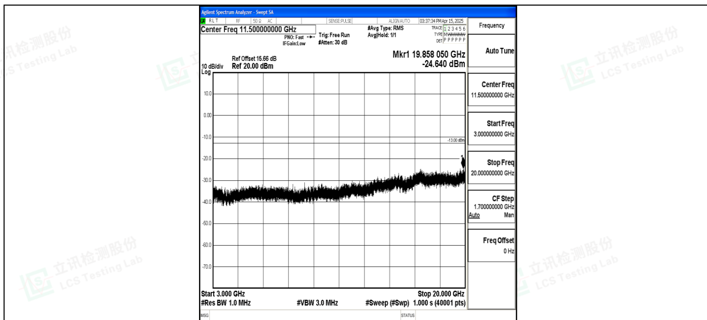
Band4_5MHz_QPSK_20175_1RB#0_3000~20000_3000~20000
