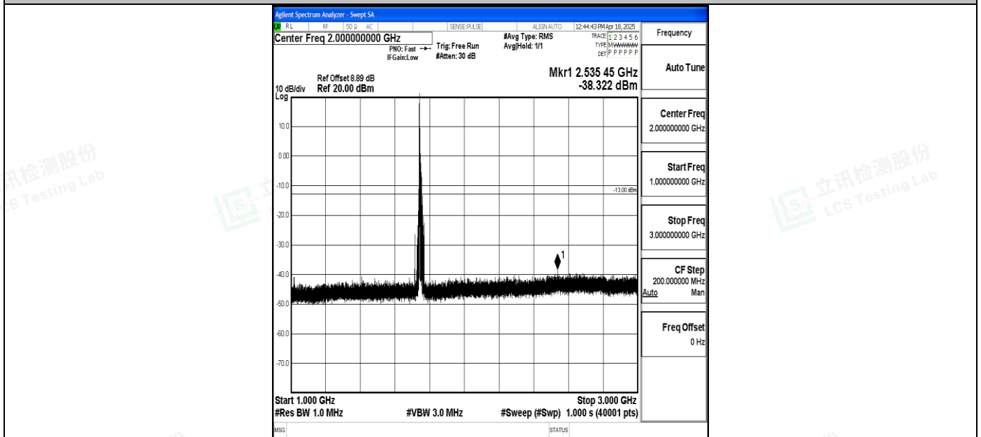
Band4_15MHz_QPSK_20325_1RB#0_1000~3000_1000~3000
