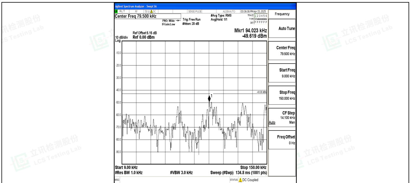
Band4_5MHz_QPSK_19975_1RB#0_0.009~0.15_0.009~0.15
