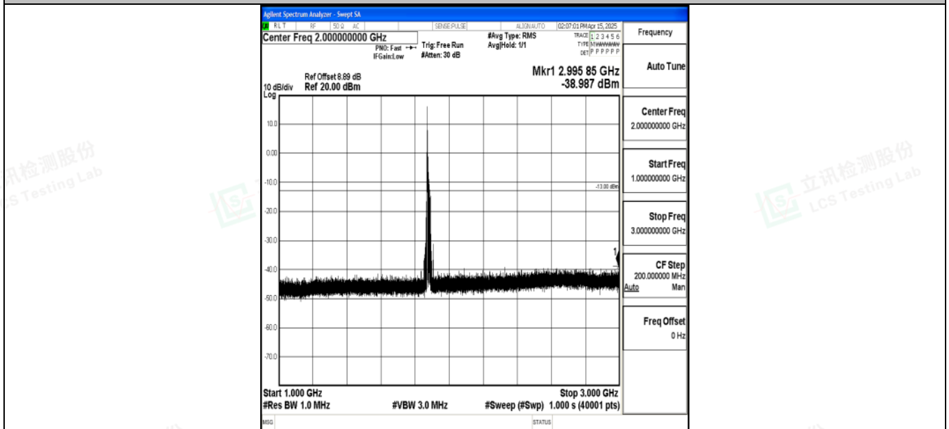
Band2_20MHz_QPSK_18900_1RB#0_1000~3000_1000~3000
