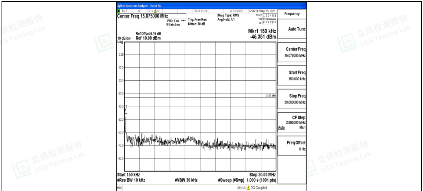
Band2_20MHz_16QAM_18700_1RB#0_0.15~30_0.15~30
