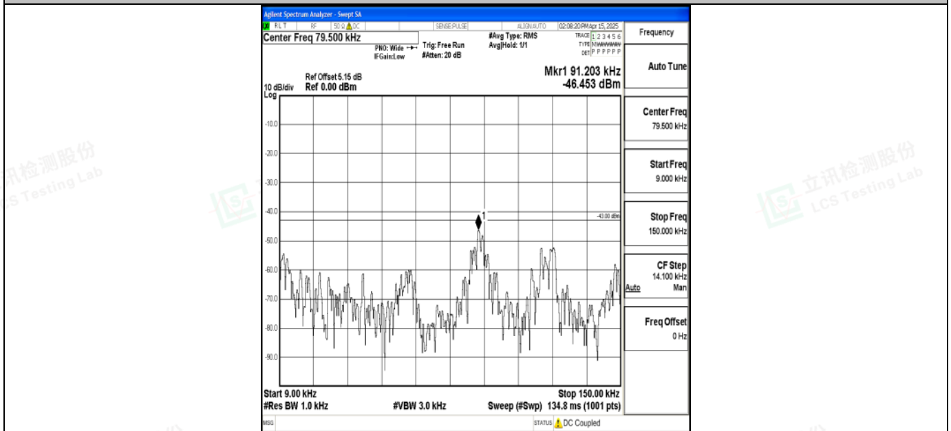
Band2_20MHz_16QAM_19100_1RB#0_0.009~0.15_0.009~0.15
