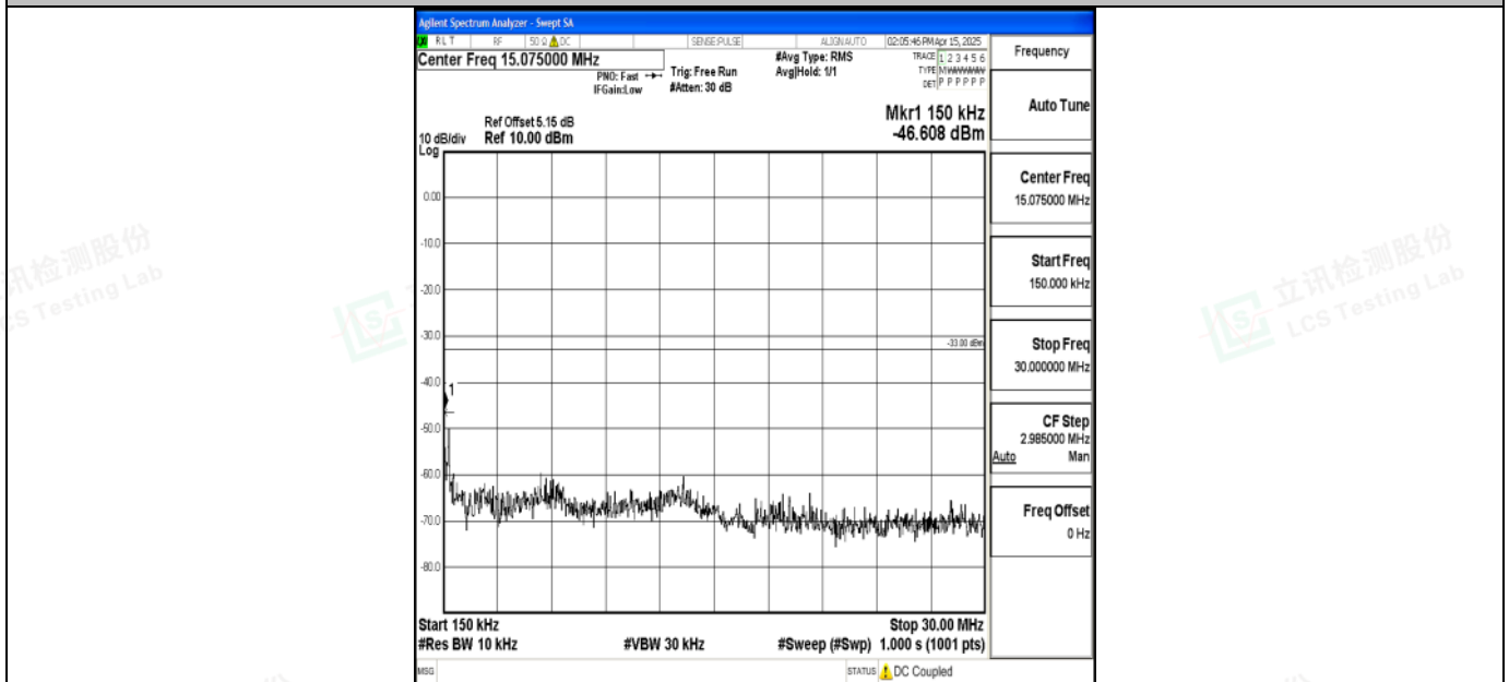
Band2_20MHz_QPSK_18700_1RB#0_0.15~30_0.15~30
