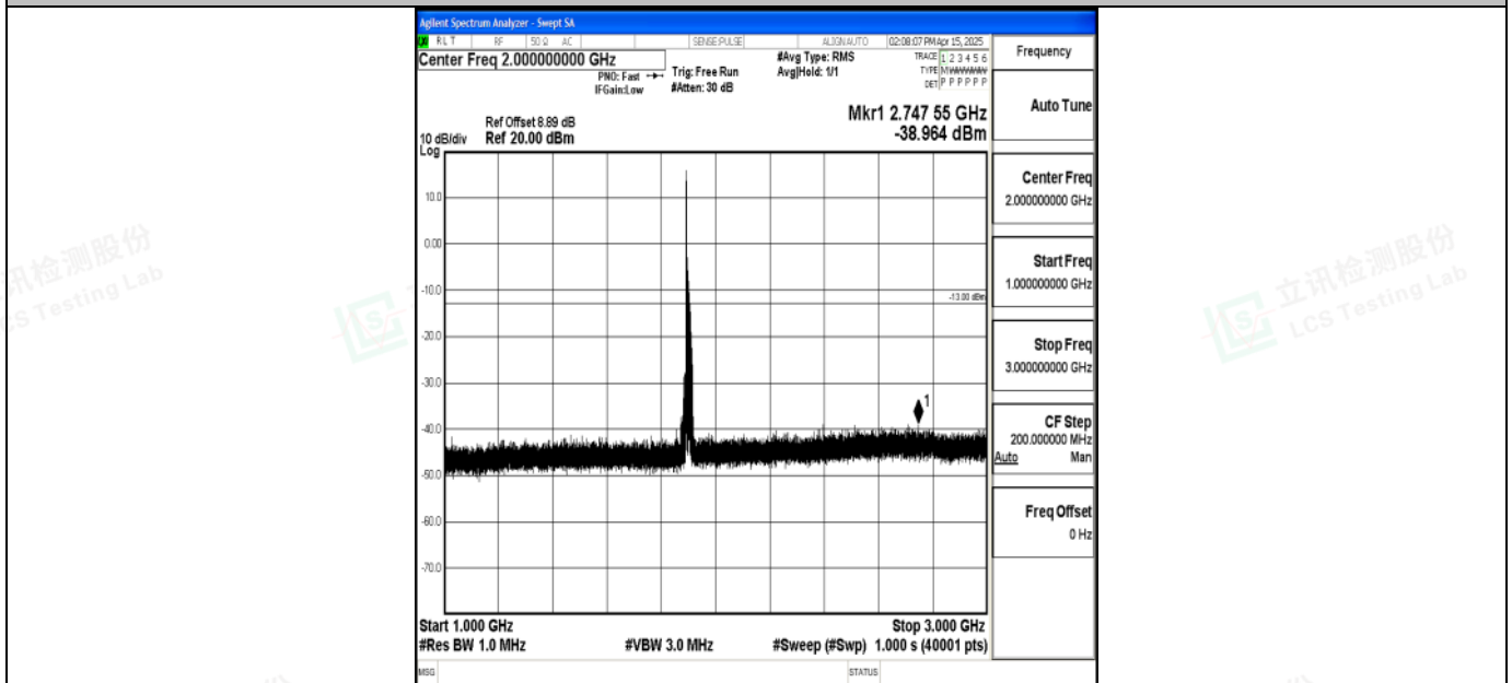
Band2_20MHz_QPSK_19100_1RB#0_1000~3000_1000~3000
