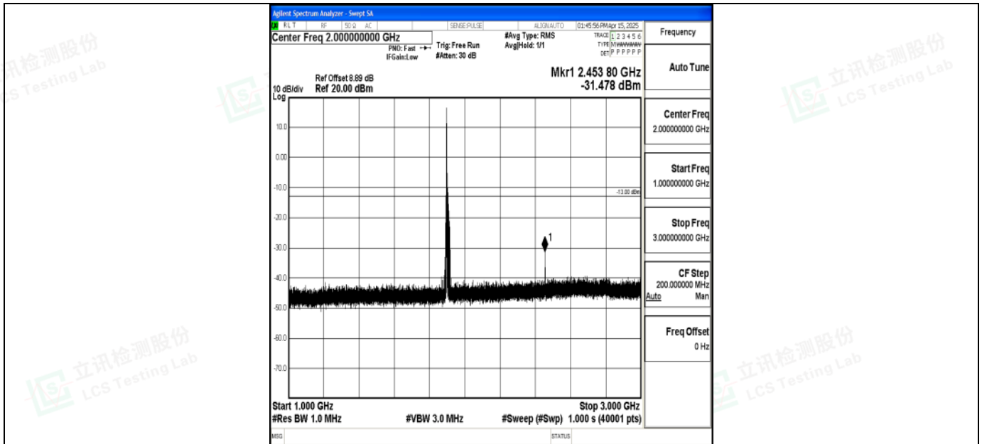
Band2_15MHz_16QAM_19125_1RB#0_1000~3000_1000~3000
