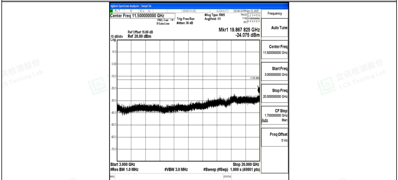
Band2_20MHz_16QAM_18700_1RB#0_3000~20000_3000~20000
