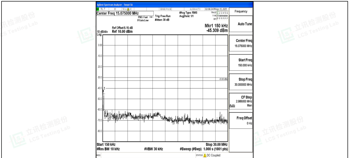
Band2_20MHz_16QAM_19100_1RB#0_0.15~30_0.15~30
