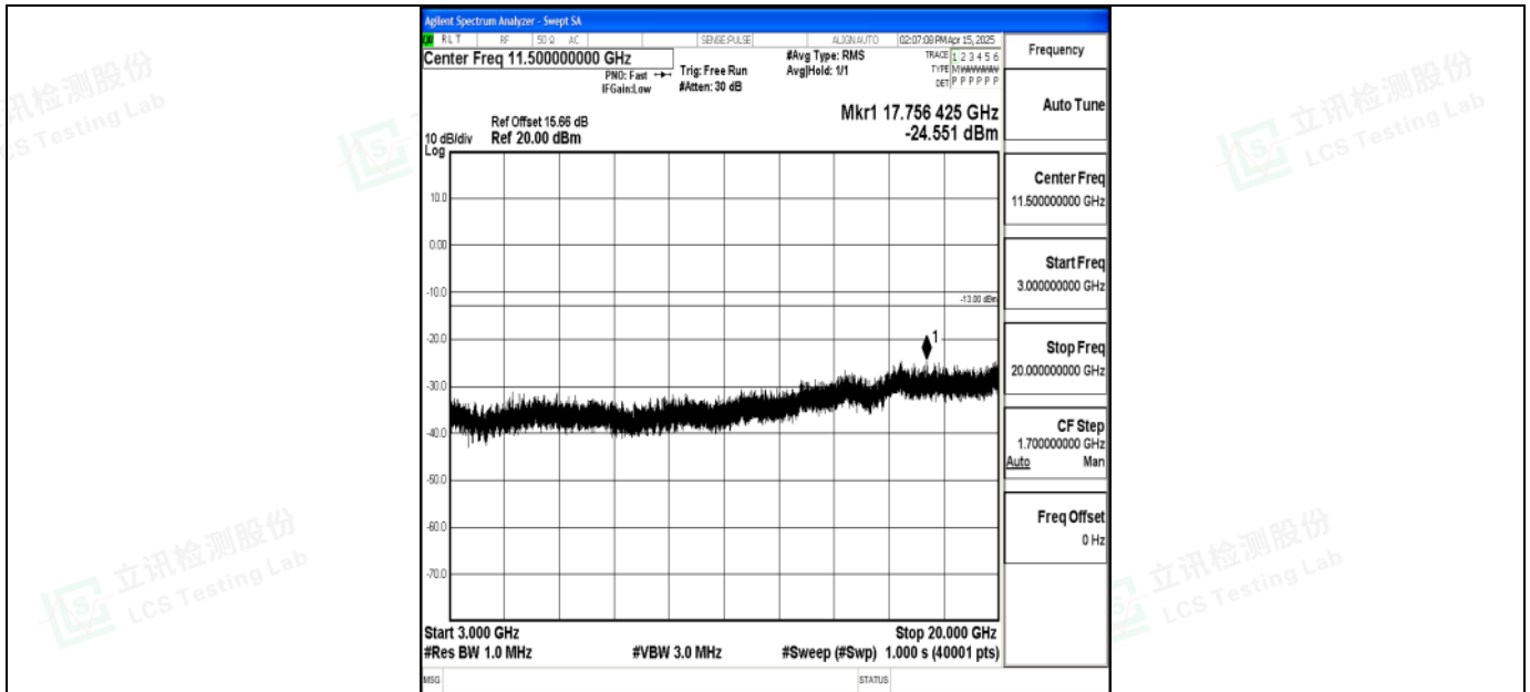
Band2_20MHz_QPSK_18900_1RB#0_3000~20000_3000~20000
