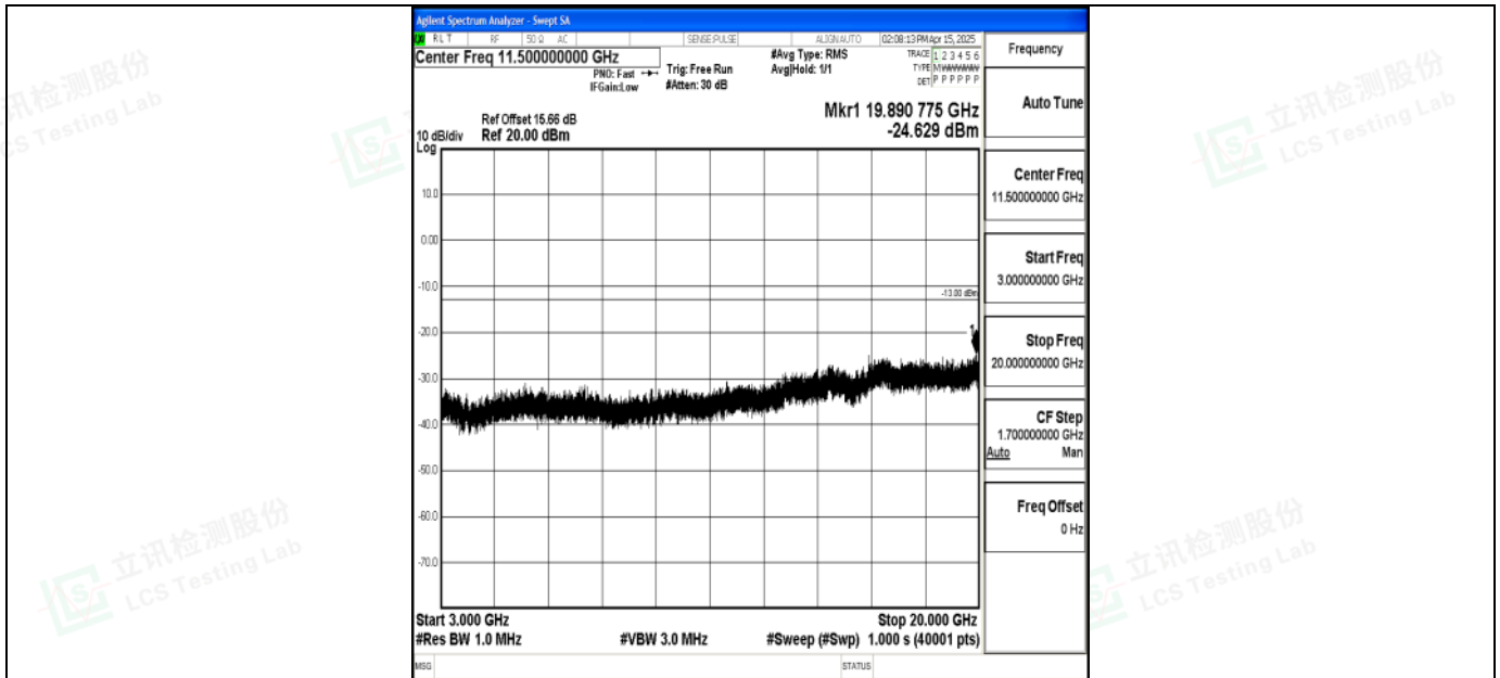
Band2_20MHz_QPSK_19100_1RB#0_3000~20000_3000~20000
