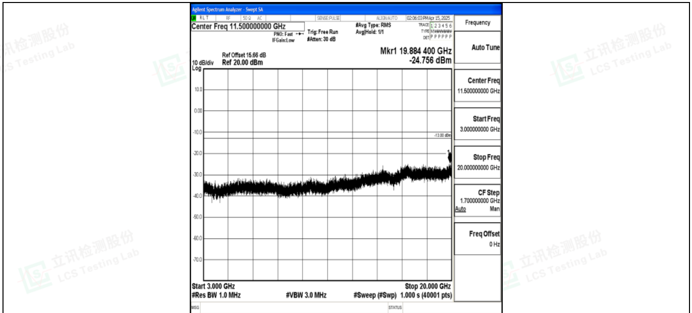
Band2_20MHz_QPSK_18700_1RB#0_3000~20000_3000~20000
