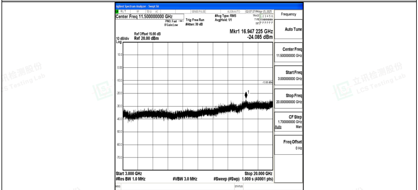
Band2_20MHz_16QAM_18900_1RB#0_3000~20000_3000~20000
