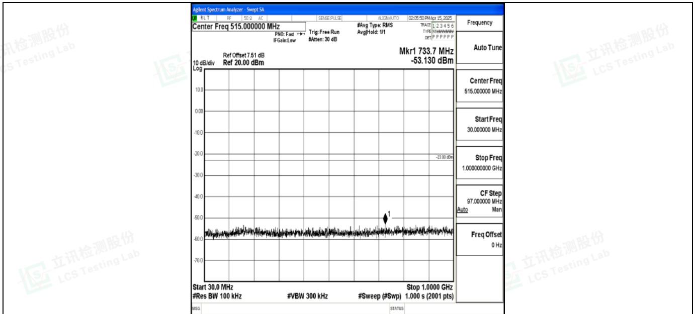
Band2_20MHz_QPSK_18700_1RB#0_30~1000_30~1000
