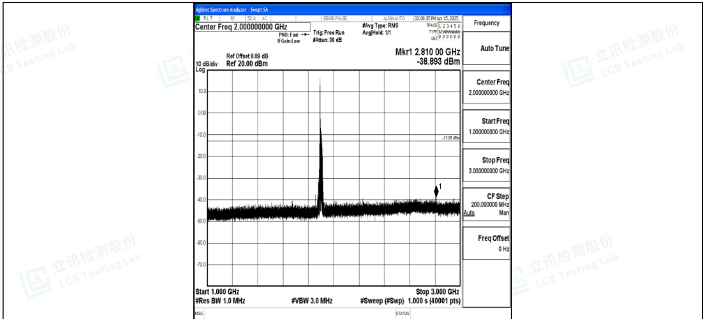
Band2_20MHz_16QAM_19100_1RB#0_1000~3000_1000~3000
