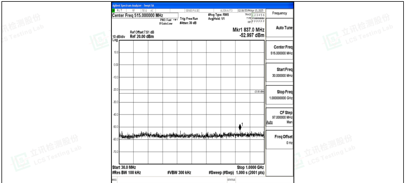
Band2_20MHz_QPSK_18900_1RB#0_30~1000_30~1000
