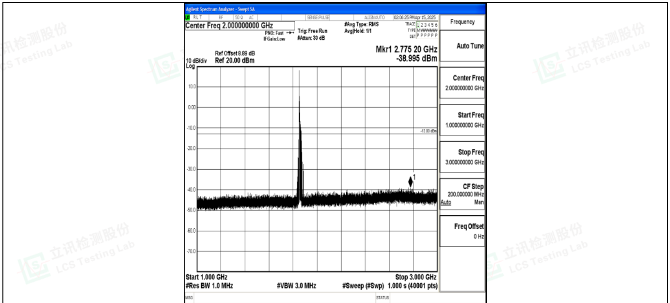
Band2_20MHz_16QAM_18700_1RB#0_1000~3000_1000~3000
