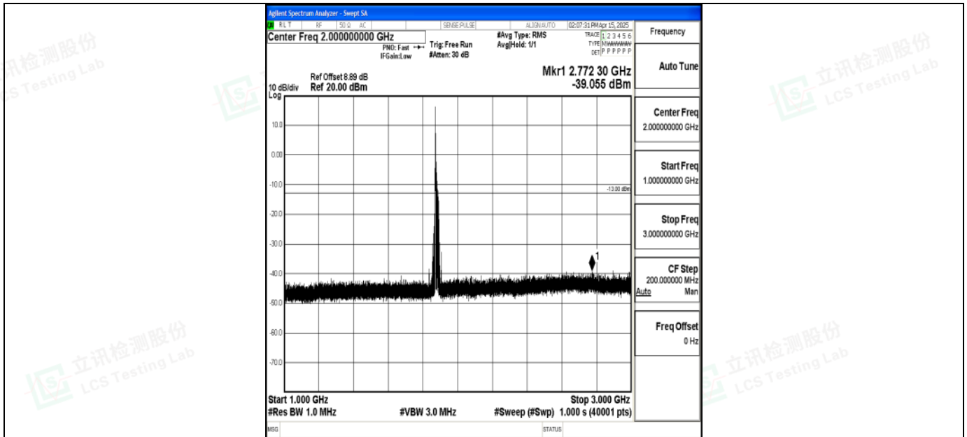
Band2_20MHz_16QAM_18900_1RB#0_1000~3000_1000~3000
