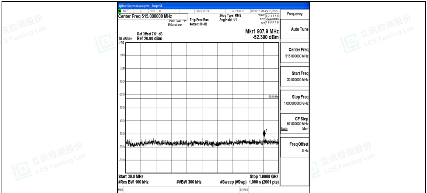
Band2_20MHz_QPSK_19100_1RB#0_30~1000_30~1000
