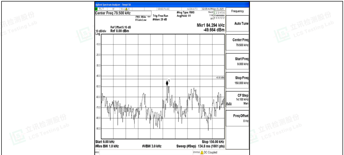
Band2_20MHz_QPSK_18700_1RB#0_0.009~0.15_0.009~0.15
