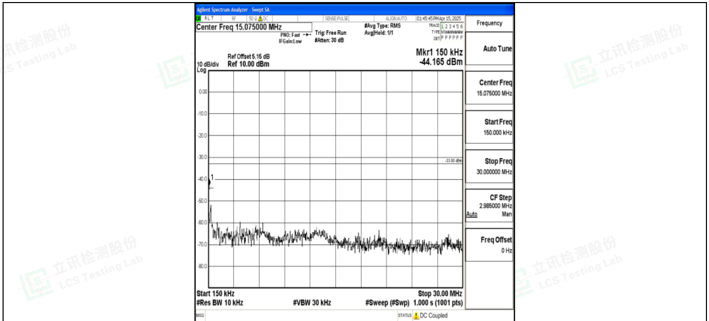
Band2_15MHz_16QAM_19125_1RB#0_0.15~30_0.15~30
