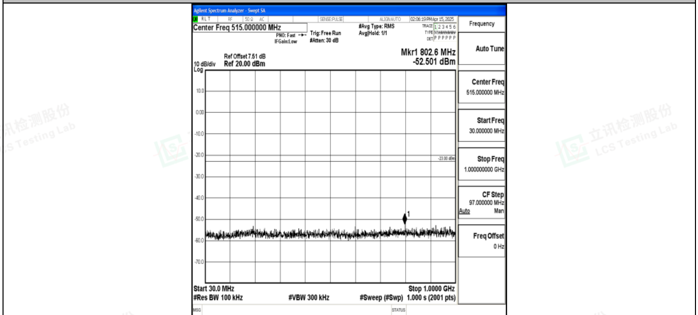
Band2_20MHz_16QAM_18700_1RB#0_30~1000_30~1000
