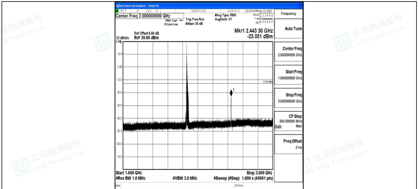
Band2_15MHz_16QAM_18675_1RB#0_1000~3000_1000~3000
