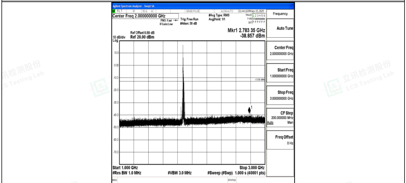
Band2_15MHz_QPSK_18900_1RB#0_1000~3000_1000~3000
