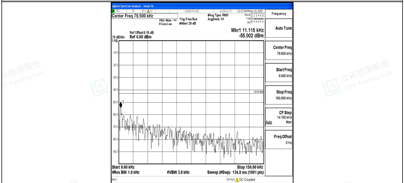
Band2_5MHz_16QAM_18625_1RB#0_0.009~0.15_0.009~0.15
