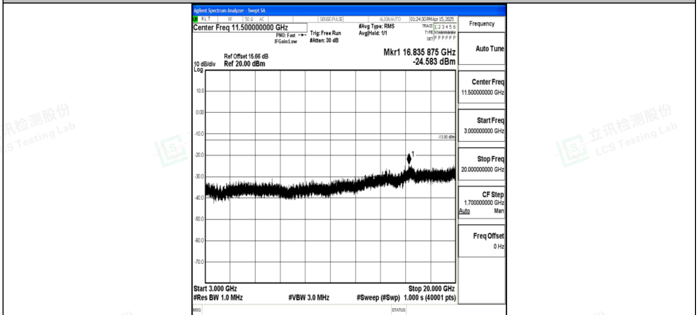
Band2_10MHz_16QAM_19150_1RB#0_3000~20000_3000~20000
