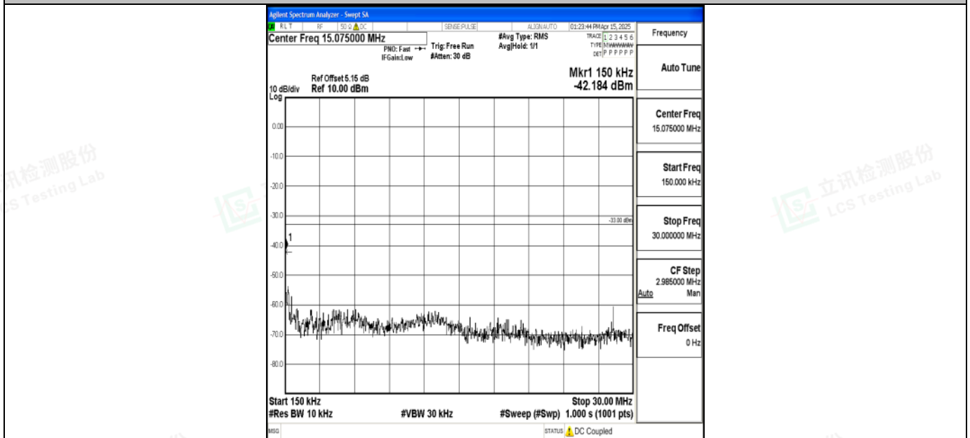
Band2_10MHz_QPSK_19150_1RB#0_0.15~30_0.15~30
