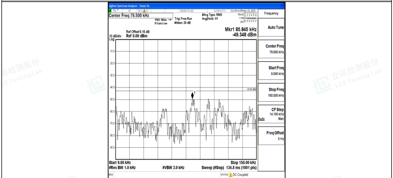
Band2_15MHz_16QAM_19125_1RB#0_0.009~0.15_0.009~0.15
