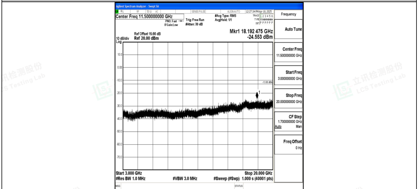
Band2_5MHz_16QAM_18625_1RB#0_3000~20000_3000~20000
