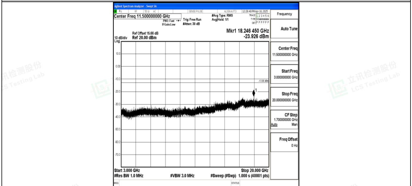
Band2_5MHz_16QAM_18900_1RB#0_3000~20000_3000~20000
