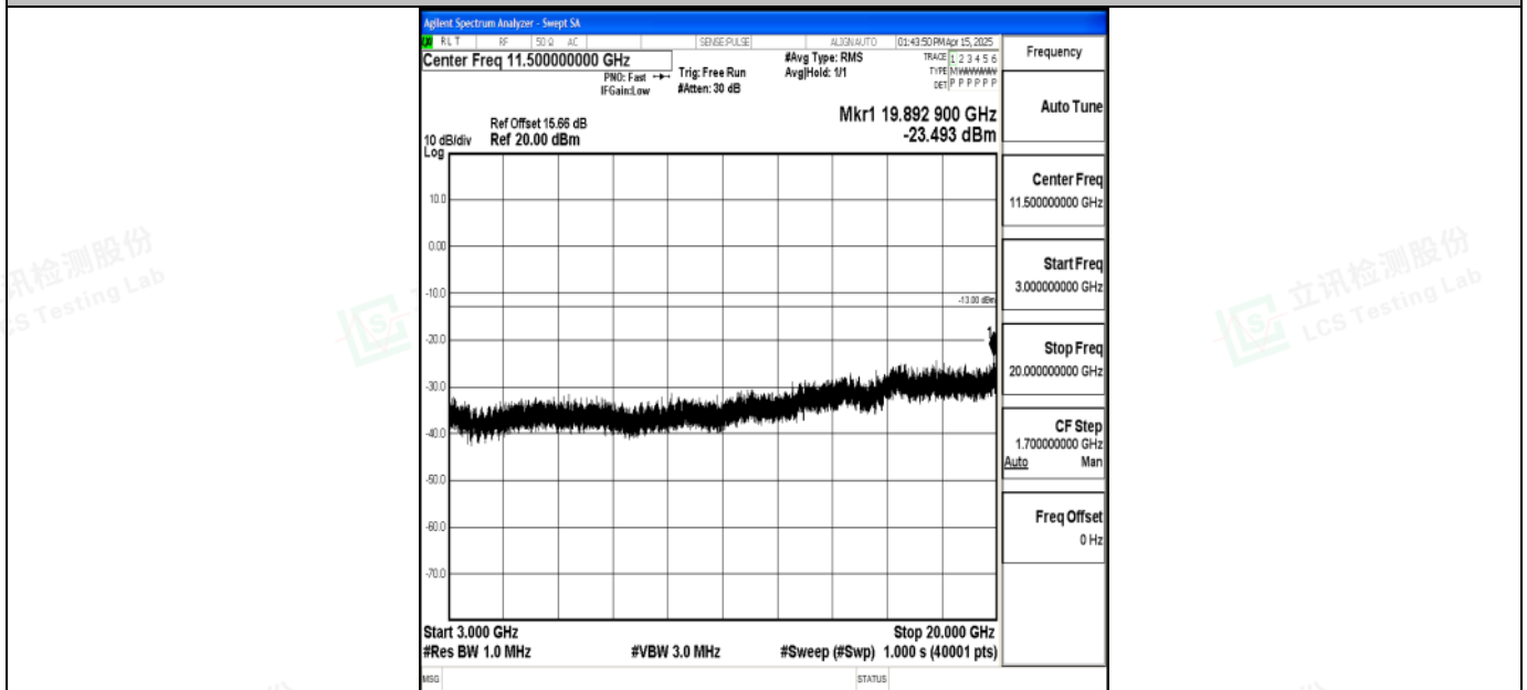
Band2_15MHz_16QAM_18675_1RB#0_3000~20000_3000~20000
