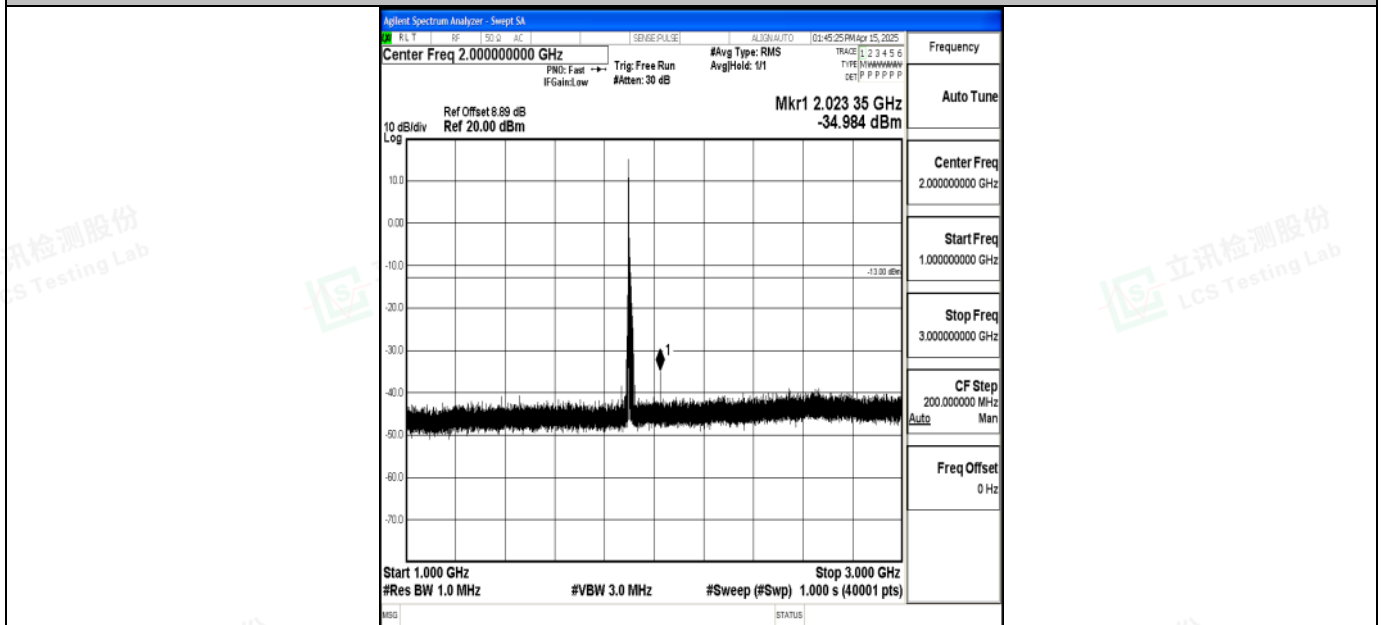
Band2_15MHz_QPSK_19125_1RB#0_1000~3000_1000~3000
