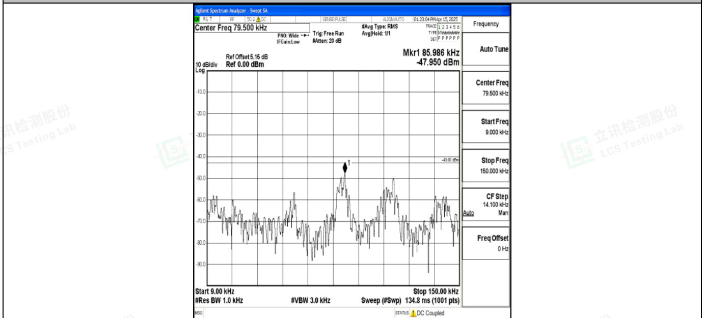
Band2_10MHz_16QAM_18900_1RB#0_0.009~0.15_0.009~0.15
