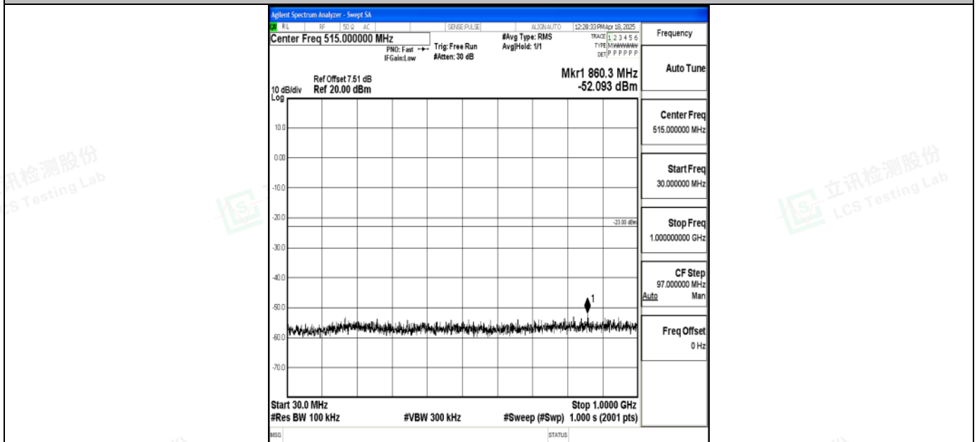
Band2_5MHz_16QAM_18900_1RB#0_30~1000_30~1000
