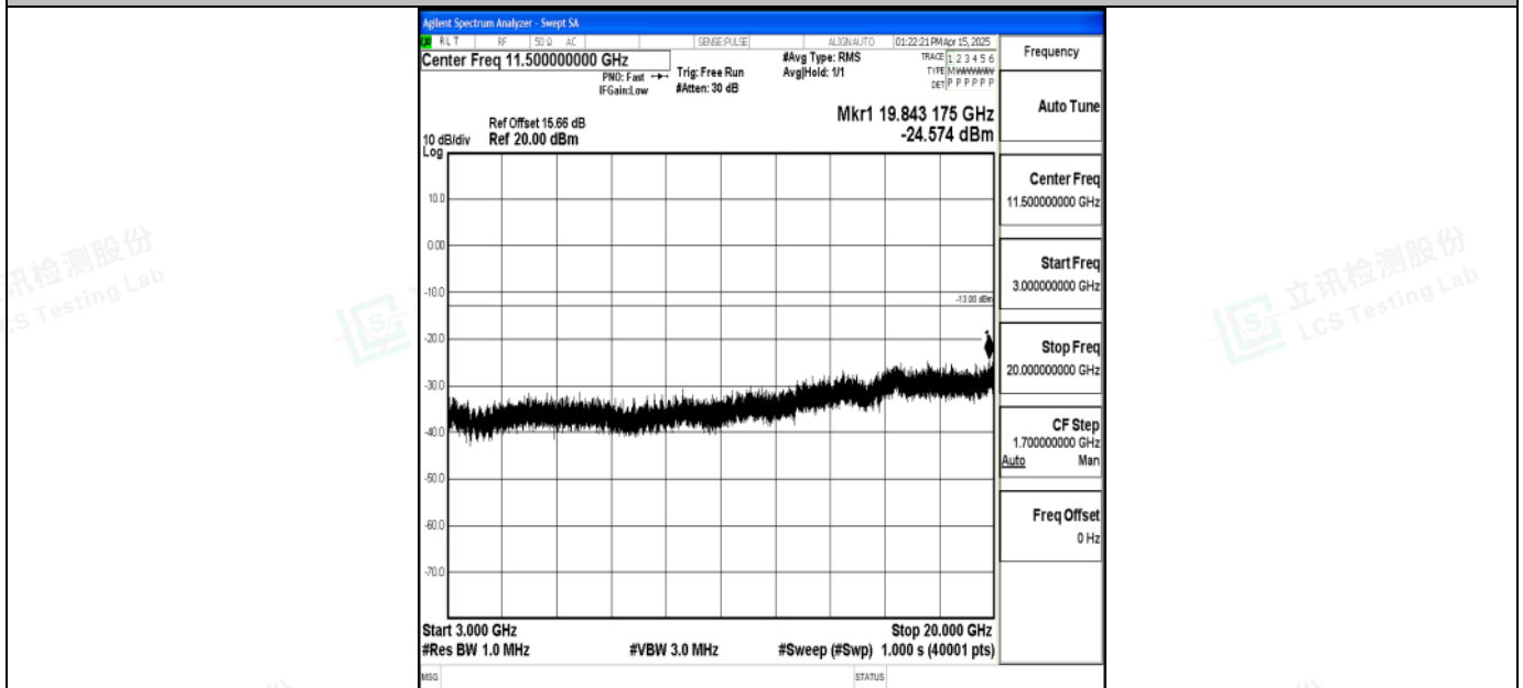
Band2_10MHz_16QAM_18650_1RB#0_3000~20000_3000~20000
