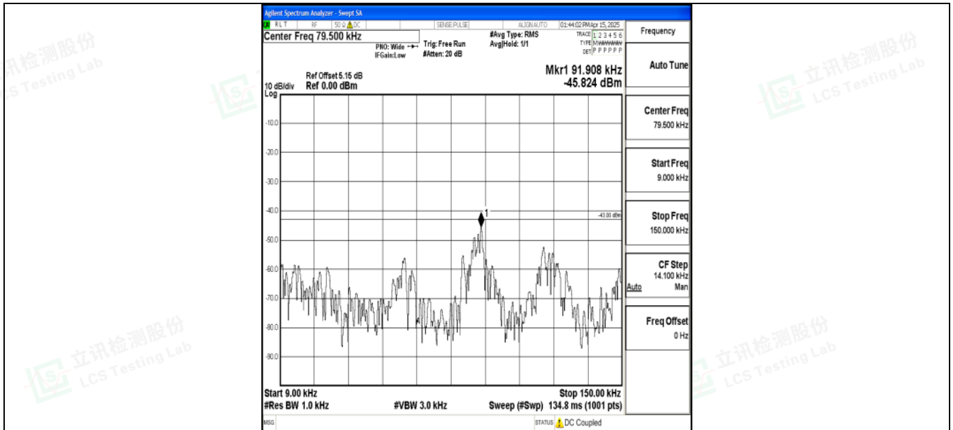
Band2_15MHz_QPSK_18900_1RB#0_0.009~0.15_0.009~0.15
