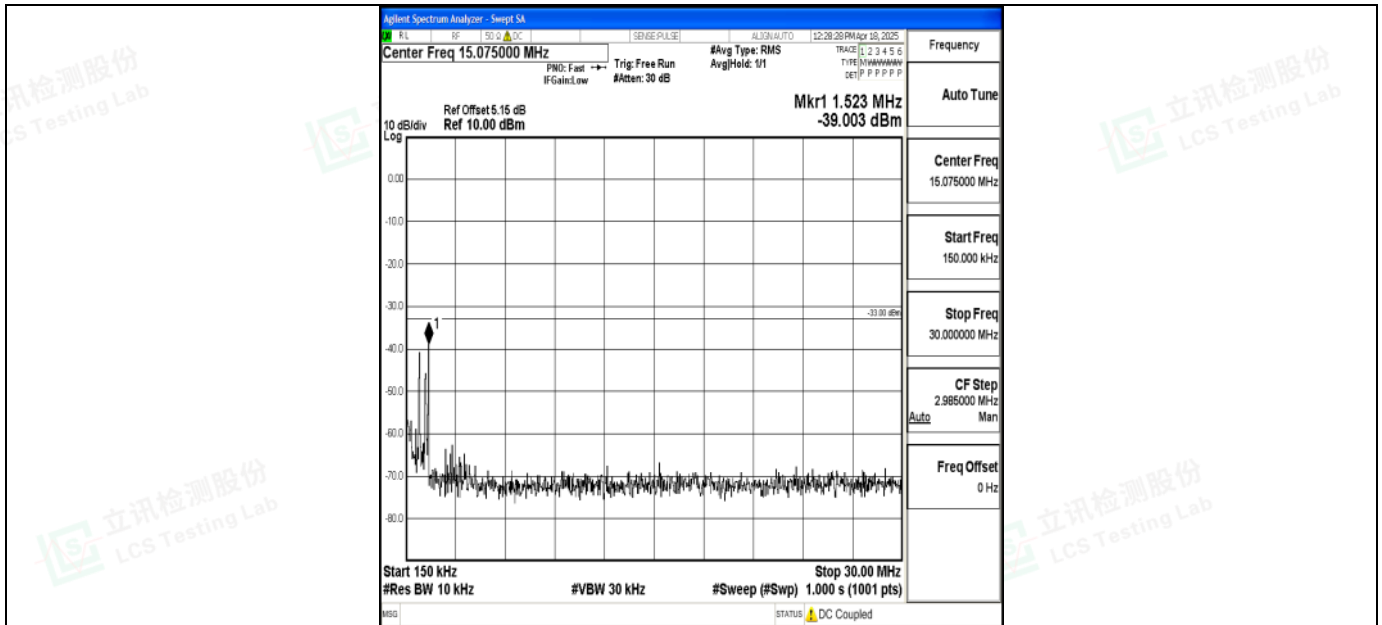
Band2_5MHz_16QAM_18900_1RB#0_0.15~30_0.15~30
