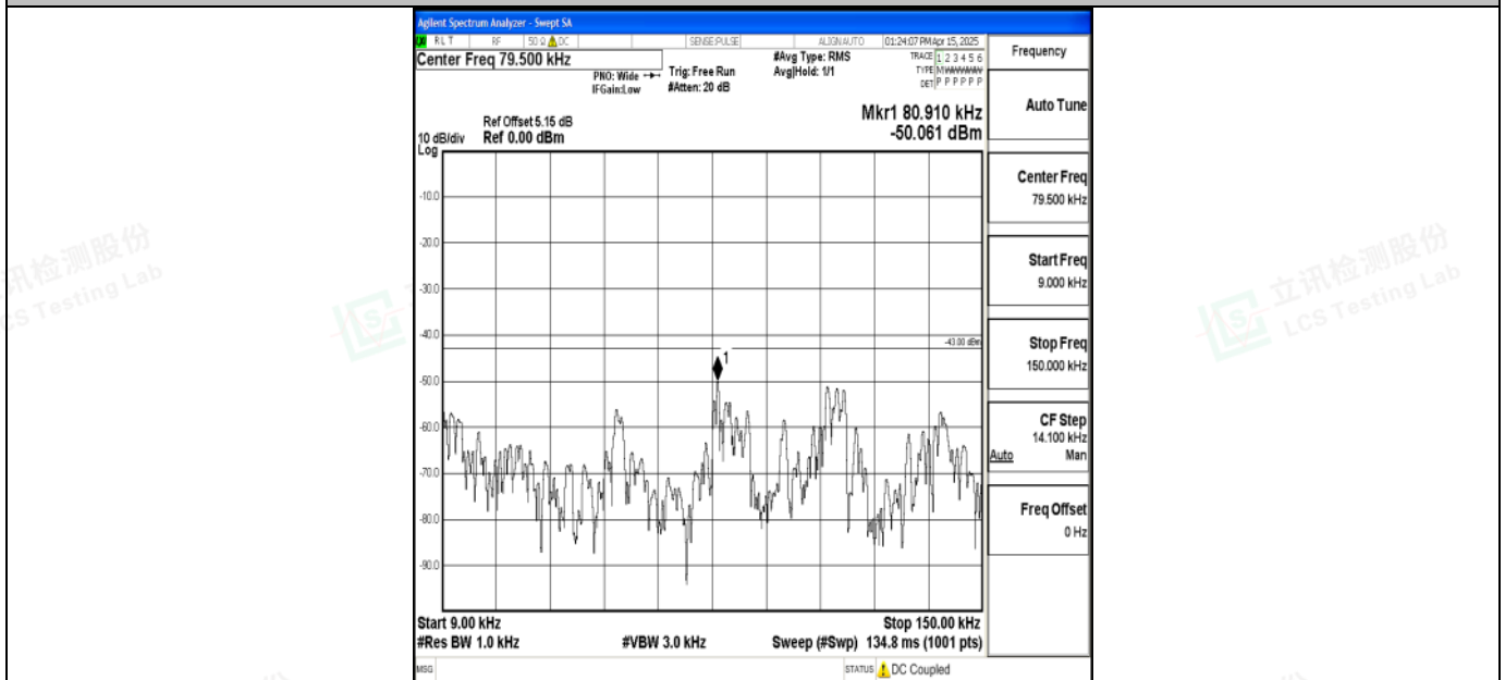
Band2_10MHz_16QAM_19150_1RB#0_0.009~0.15_0.009~0.15
