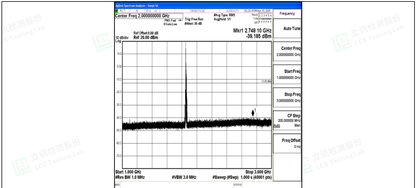
Band2_10MHz_16QAM_18650_1RB#0_1000~3000_1000~3000
