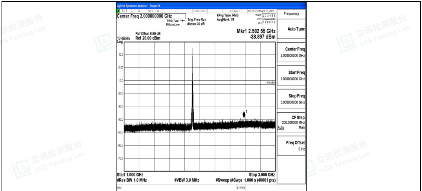
Band2_10MHz_16QAM_19150_1RB#0_1000~3000_1000~3000
