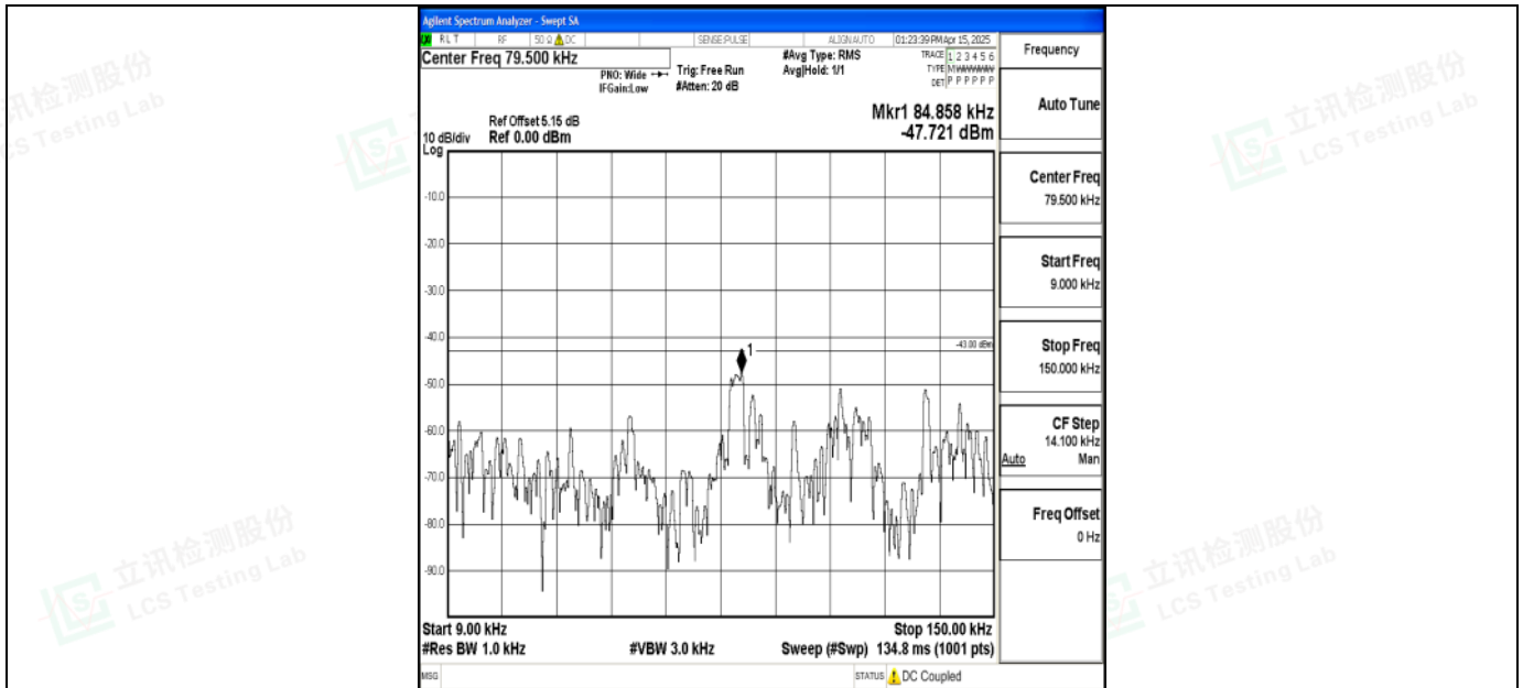
Band2_10MHz_QPSK_19150_1RB#0_0.009~0.15_0.009~0.15
