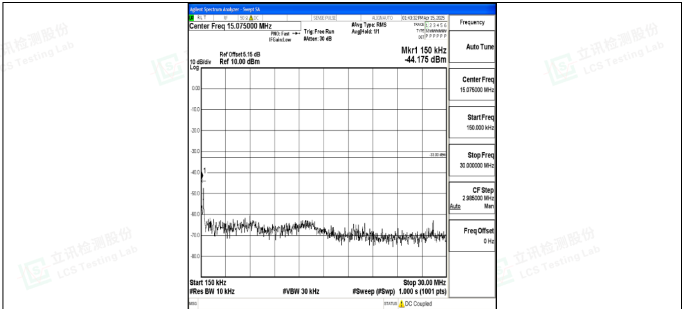
Band2_15MHz_16QAM_18675_1RB#0_0.15~30_0.15~30
