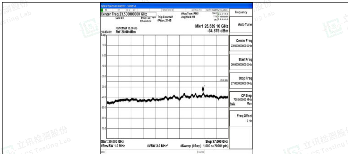
Band41_10MHz_QPSK_40620_1RB#0_20000~27000_20000~27000
