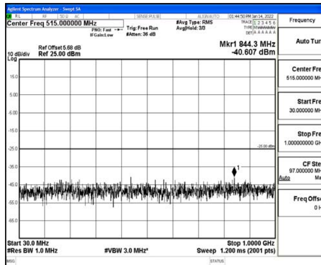
Band41-5MHz-QPSK-41565-1RB#0-Range4:1000~10000MHz
