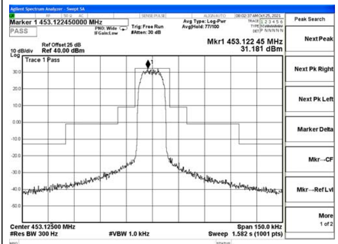
Channel 27 / 453.125 MHz
