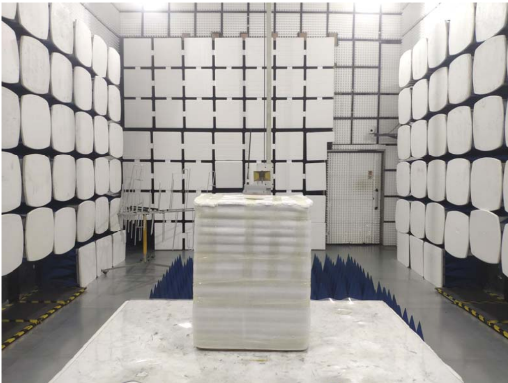
Fig.2 (Above 1GHz)
