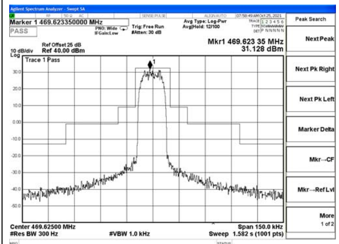
Channel 20 / 469.625 MHz
