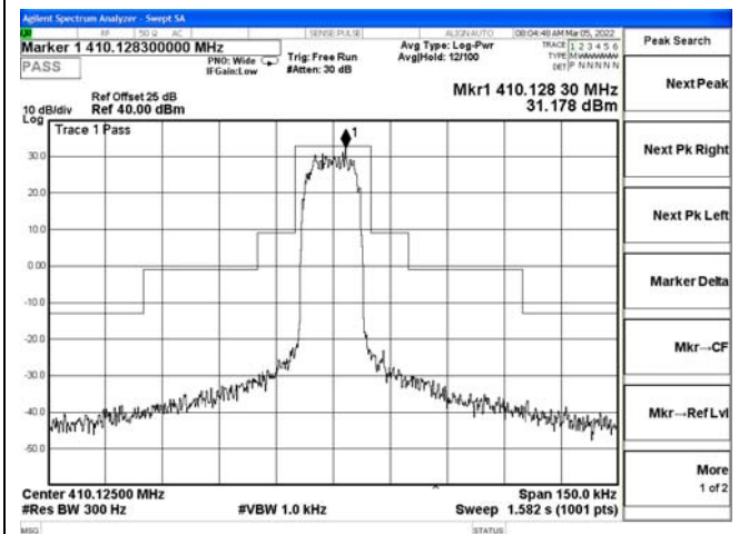
Channel 101 / 410.125 MHz
