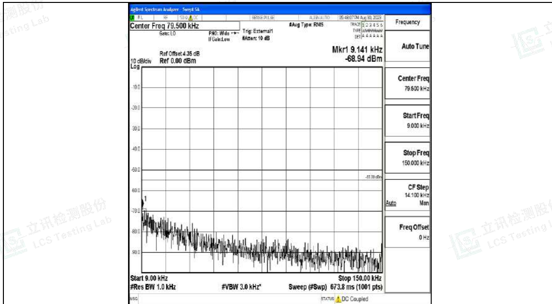
Band41_15MHz_QPSK_39725_1RB#0_0.009~0.15_0.009~0.15
