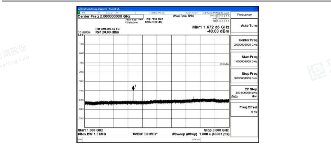
Band5_1.4MHz_QPSK_20525_1RB#0_1000~3000_1000~3000
