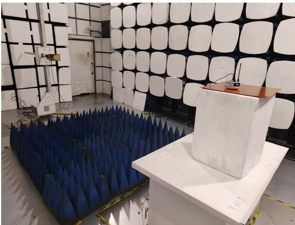
Fig.2 (Above 1GHz)
