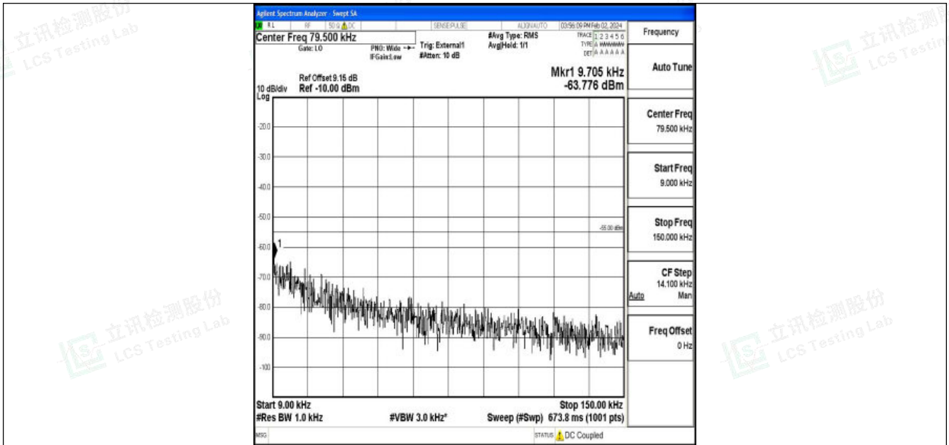
Band41_20MHz_QPSK_41490_1RB#0_0.009~0.15_0.009~0.15
