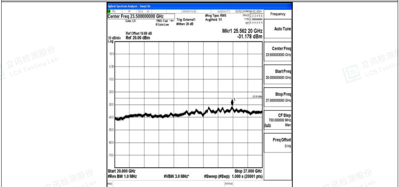
Band41_10MHz_16QAM_40620_1RB#0_20000~27000_20000~27000
