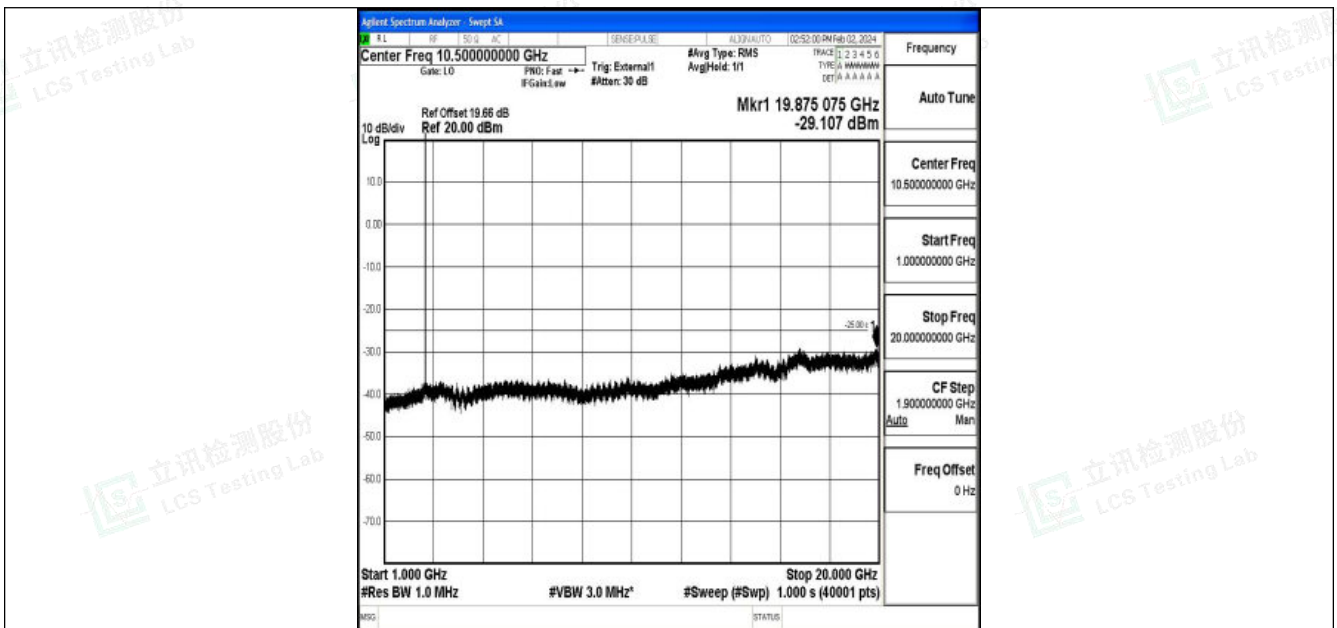
Band41_10MHz_16QAM_40620_1RB#0_1000~20000_1000~20000
