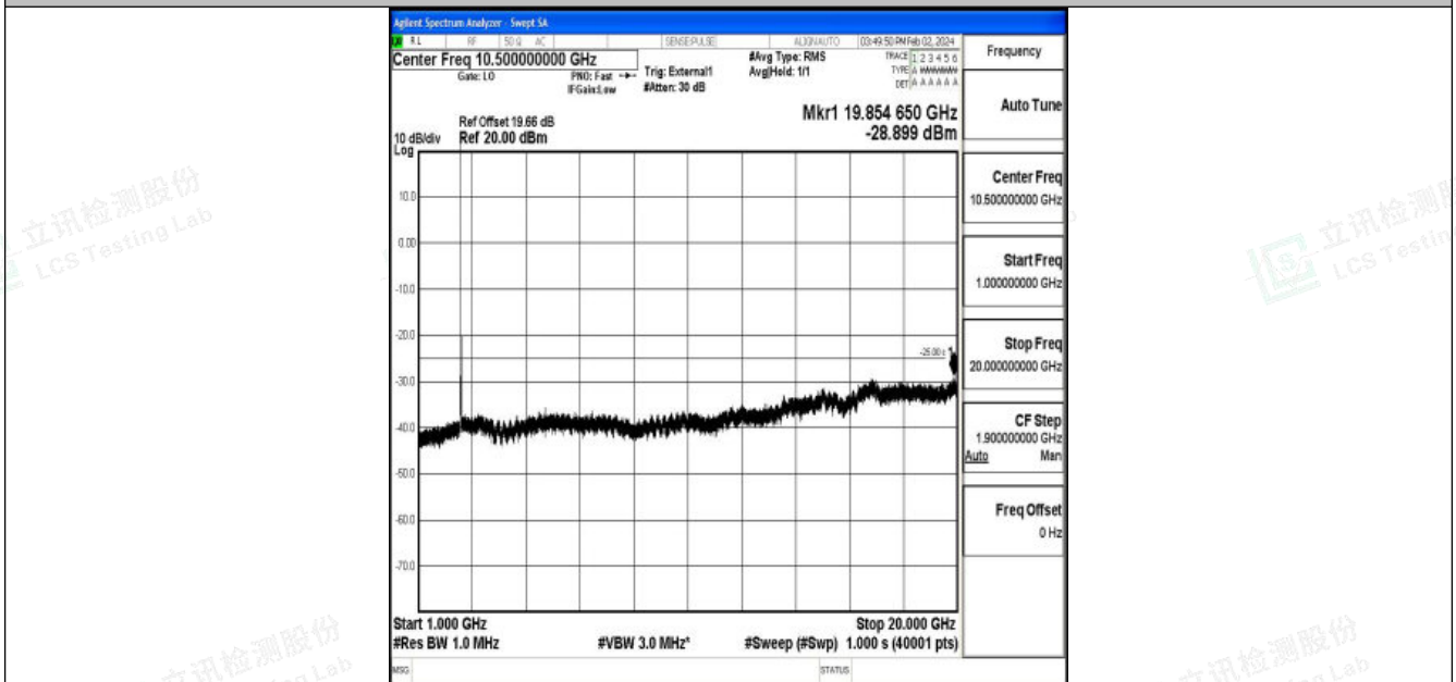
Band41_20MHz_QPSK_39750_1RB#0_1000~20000_1000~20000
