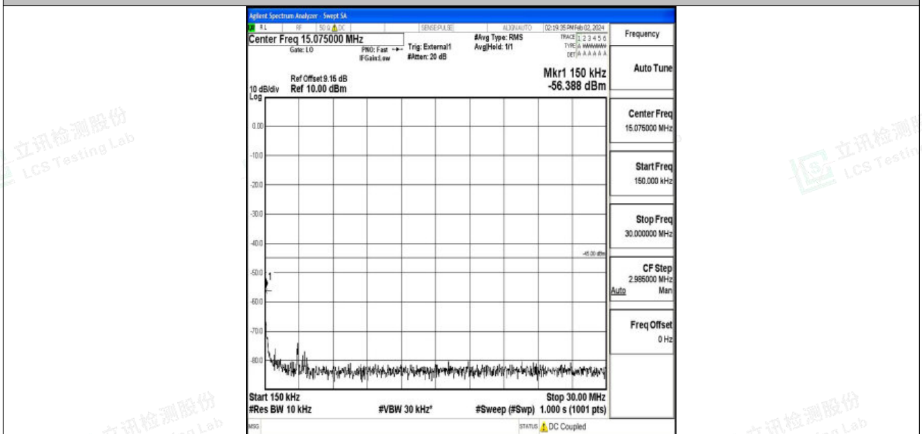
Band41_5MHz_QPSK_41565_1RB#0_0.15~30_0.15~30
