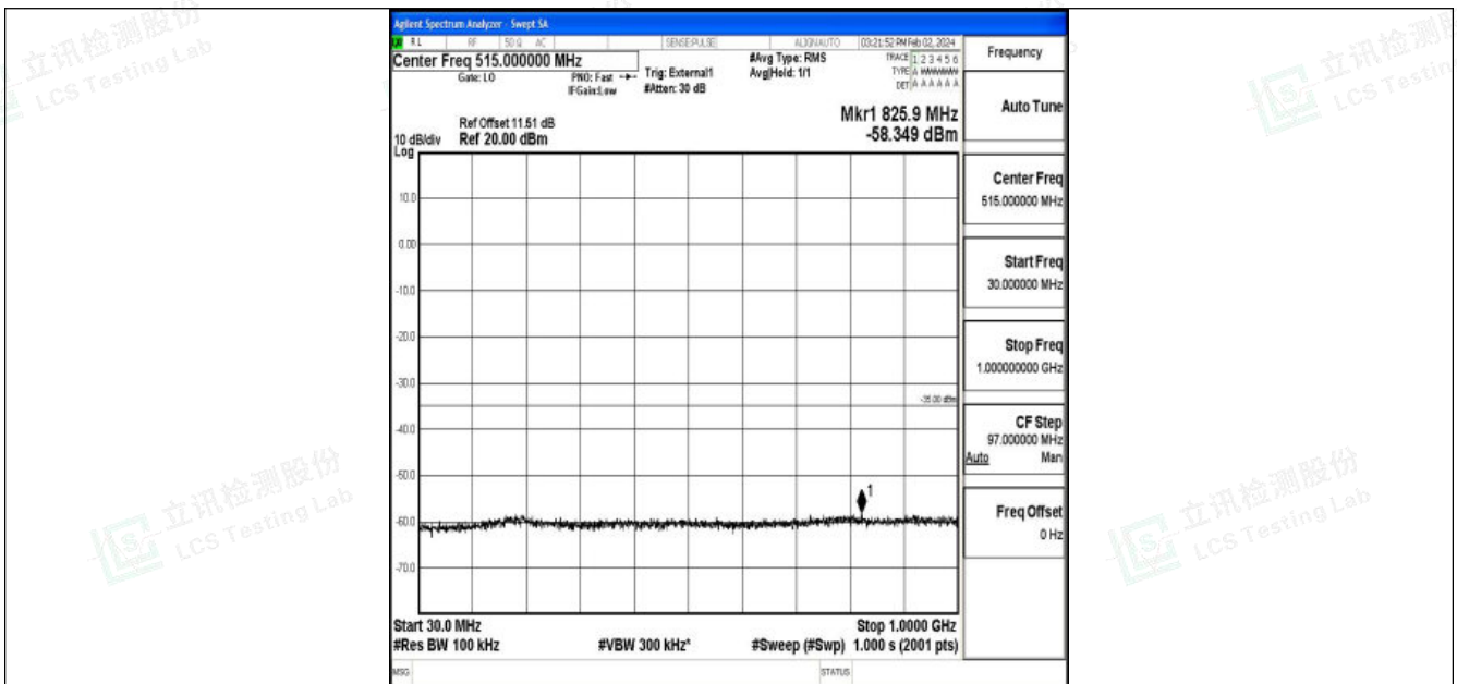
Band41_15MHz_QPSK_40620_1RB#0_30~1000_30~1000
