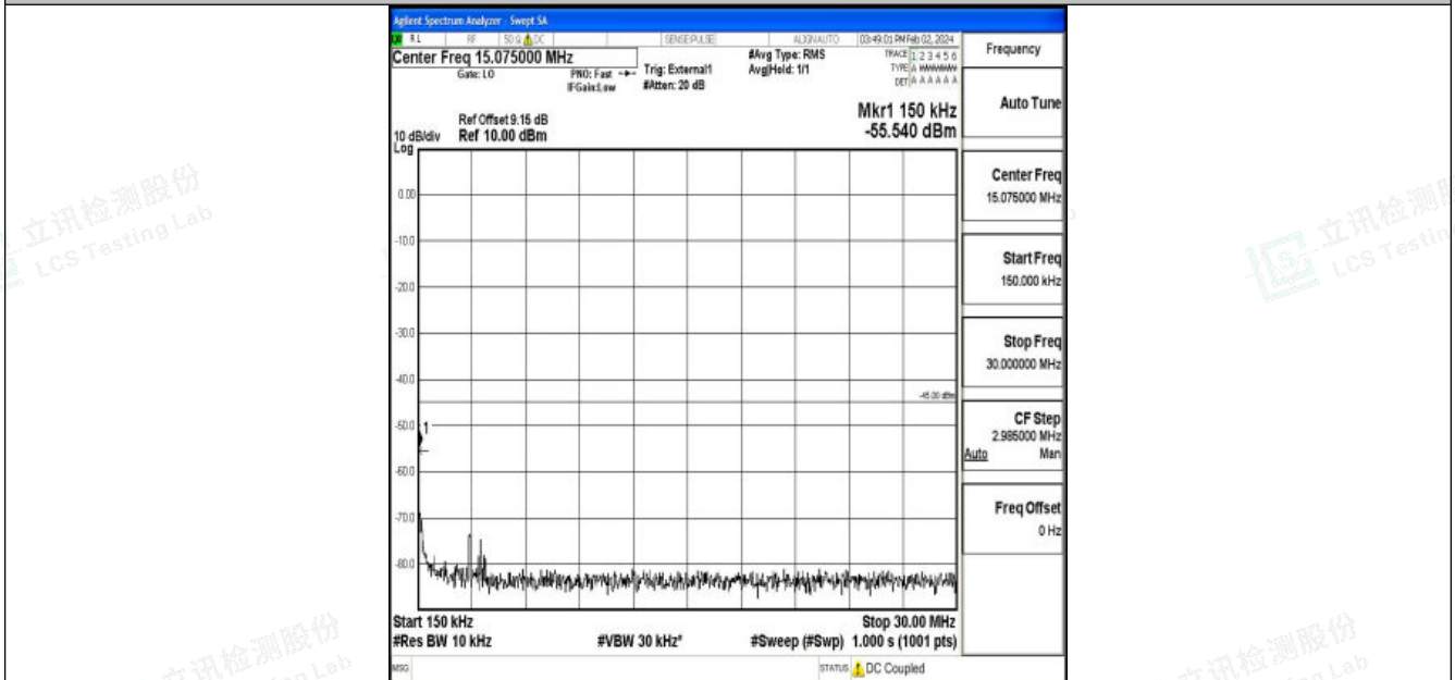
Band41_20MHz_QPSK_39750_1RB#0_0.15~30_0.15~30
