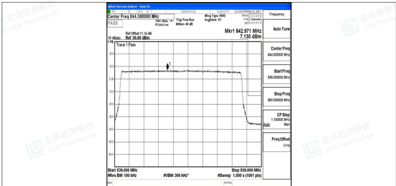
Band26_10MHz_QPSK_26990_50RB#0
