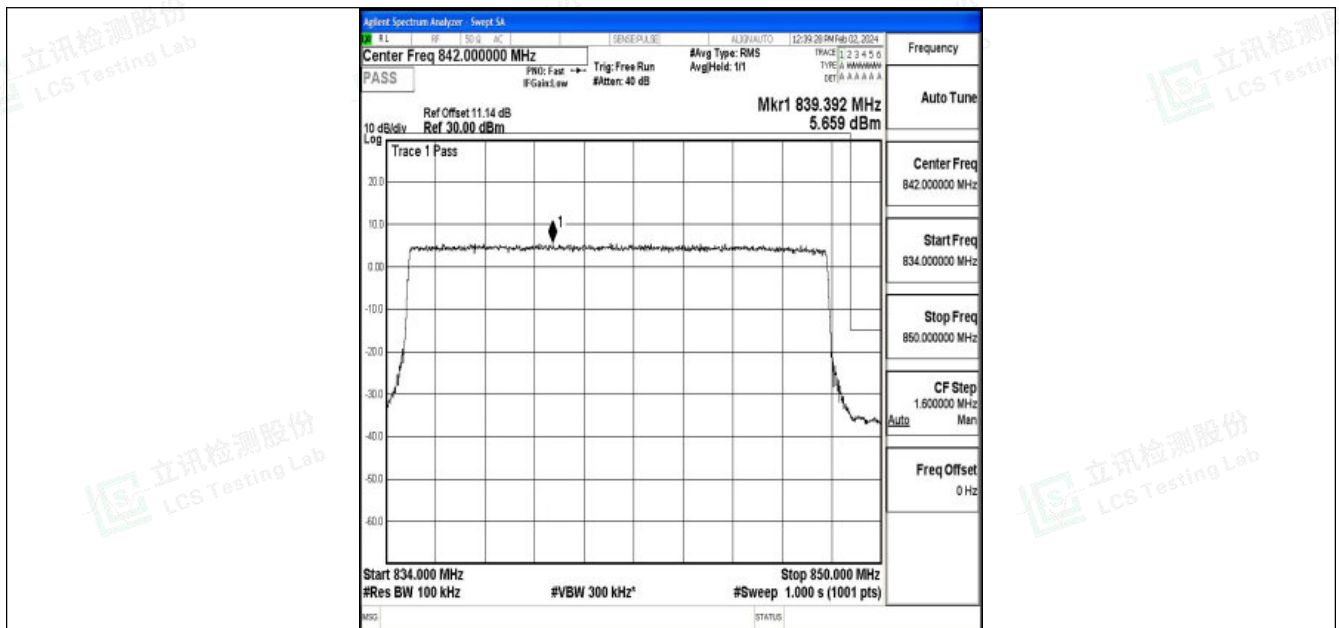
Band26_15MHz_QPSK_26965_75RB#0
