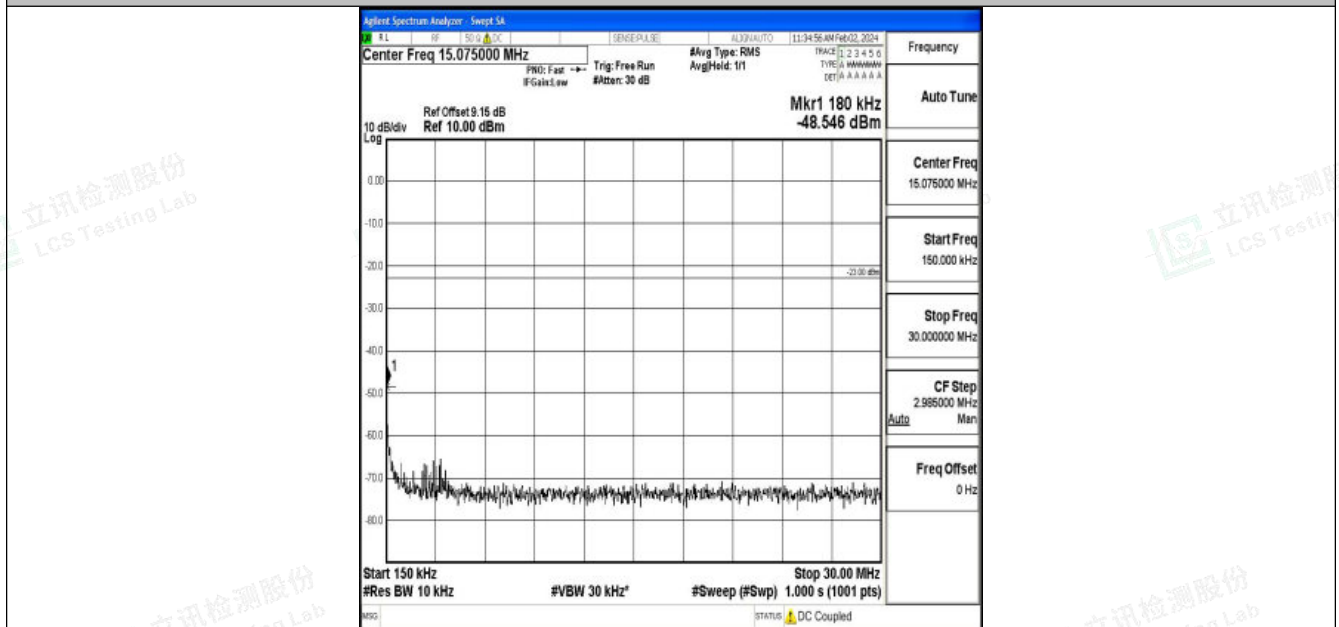
Band26_3MHz_QPSK_26805_1RB#0_0.15~30_0.15~30
