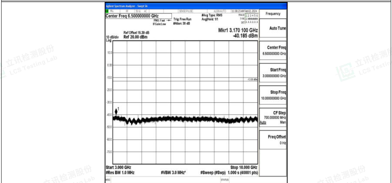
Band26_3MHz_16QAM_27025_1RB#0_3000~10000_3000~10000
