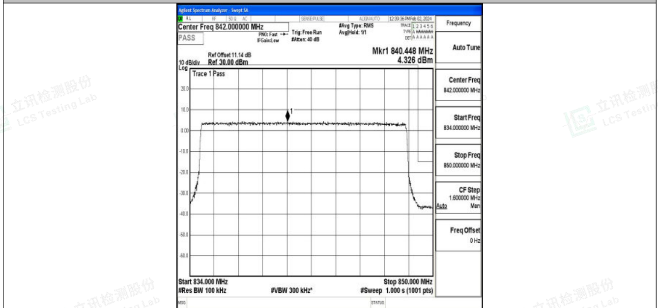
Band26_15MHz_16QAM_26965_75RB#0
