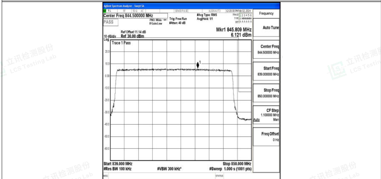
Band26_10MHz_16QAM_26990_50RB#0
