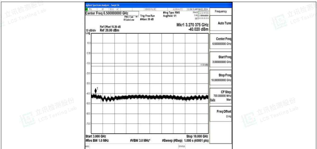
Band26_3MHz_QPSK_26915_1RB#0_3000~10000_3000~10000
