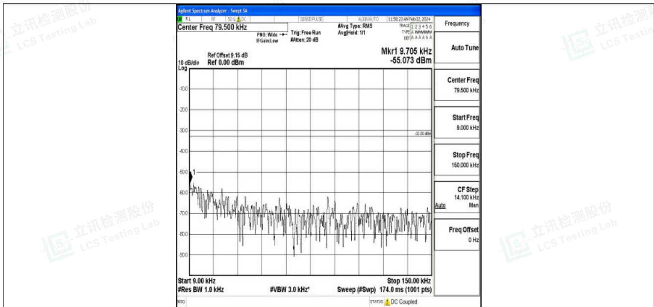
Band26_5MHz_QPSK_26915_1RB#0_0.009~0.15_0.009~0.15
