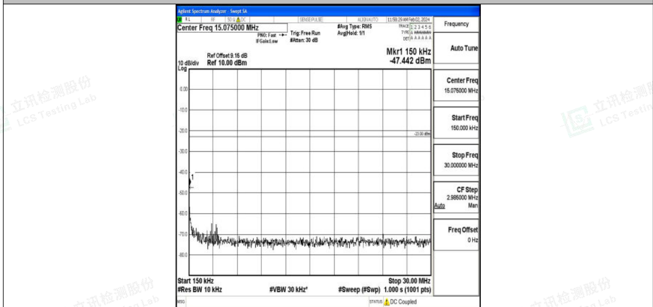
Band26_5MHz_QPSK_26915_1RB#0_0.15~30_0.15~30
