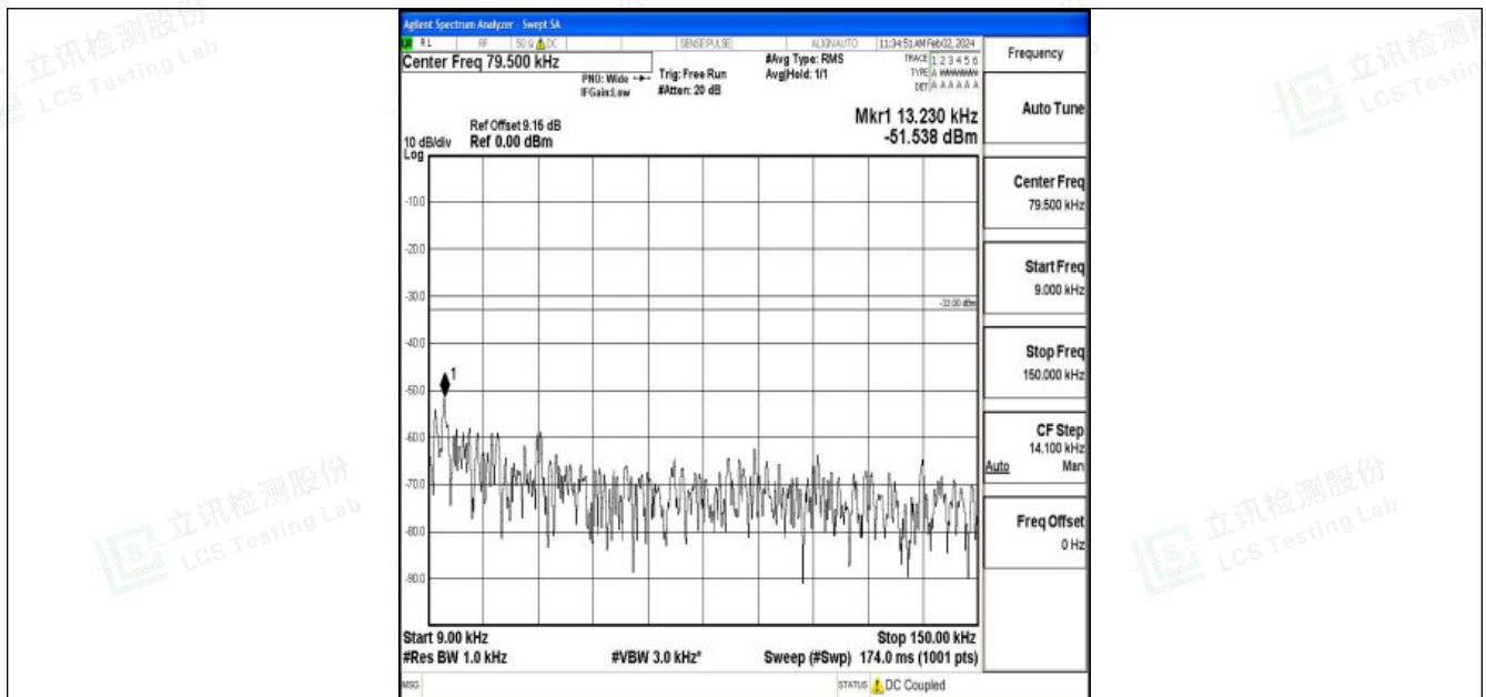
Band26_3MHz_QPSK_26805_1RB#0_0.009~0.15_0.009~0.15
