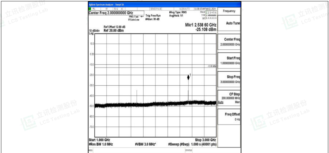
Band26_3MHz_16QAM_27025_1RB#0_1000~3000_1000~3000
