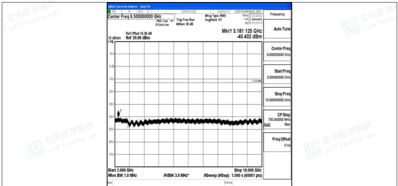
Band26_10MHz_QPSK_26740_1RB#0_3000~10000_3000~10000
