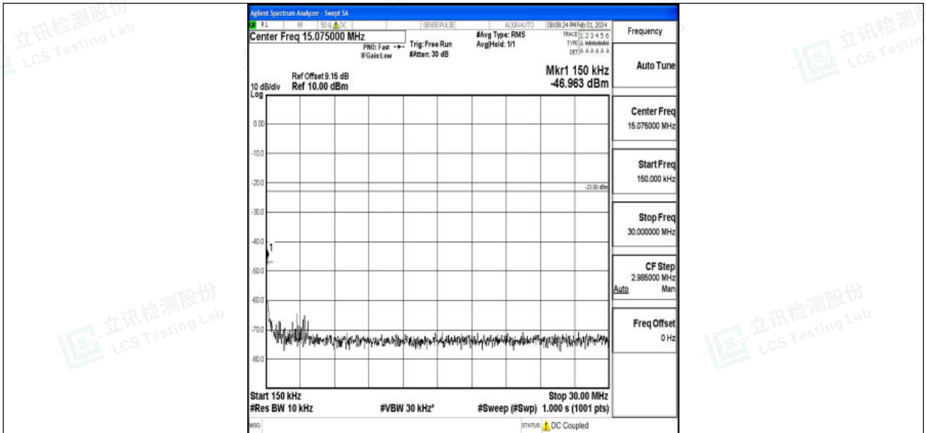
Band26_1.4MHz_16QAM_26783_1RB#0_0.15~30_0.15~30
