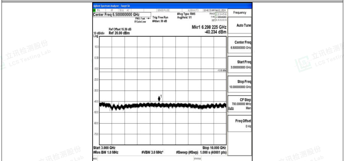
Band26_5MHz_16QAM_26715_1RB#0_3000~10000_3000~10000
