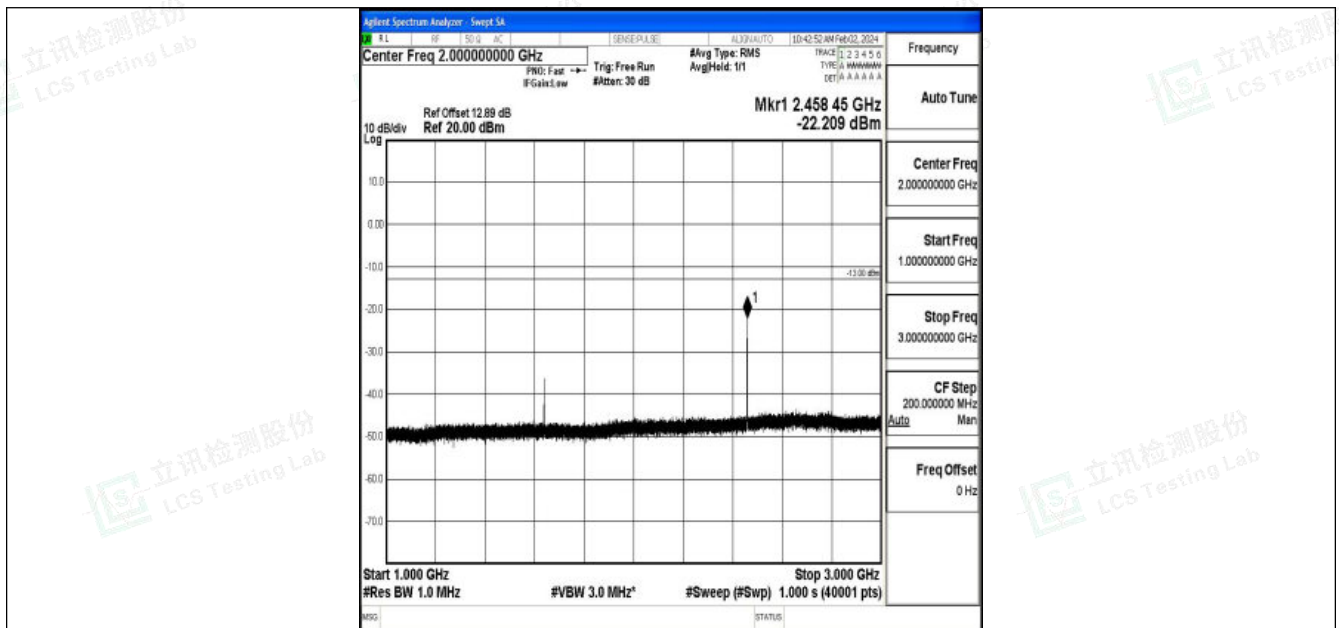
Band26_5MHz_16QAM_26765_1RB#0_1000~3000_1000~3000
