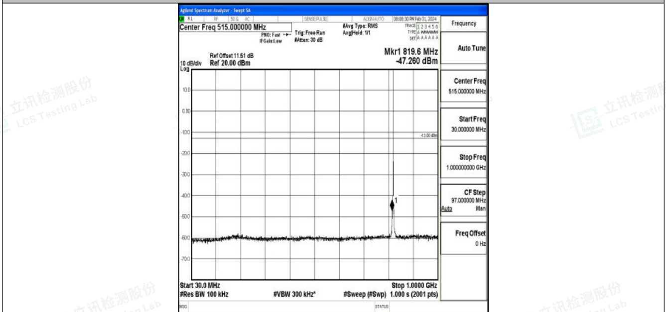
Band26_1.4MHz_16QAM_26783_1RB#0_30~1000_30~1000
