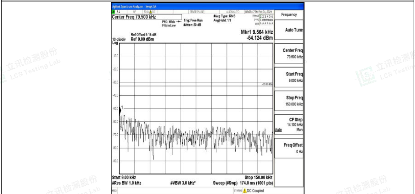
Band26_1.4MHz_16QAM_26783_1RB#0_0.009~0.15_0.009~0.15
