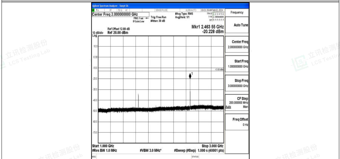
Band26_3MHz_QPSK_26775_1RB#0_1000~3000_1000~3000
