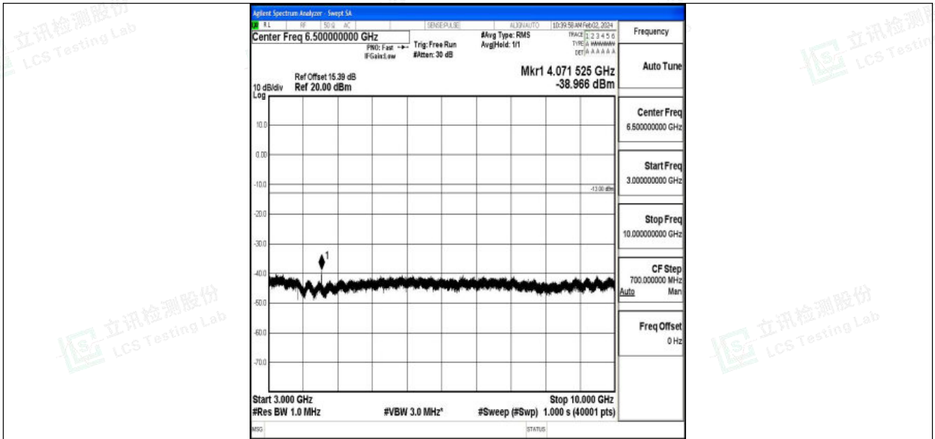
Band26_5MHz_QPSK_26715_1RB#0_3000~10000_3000~10000
