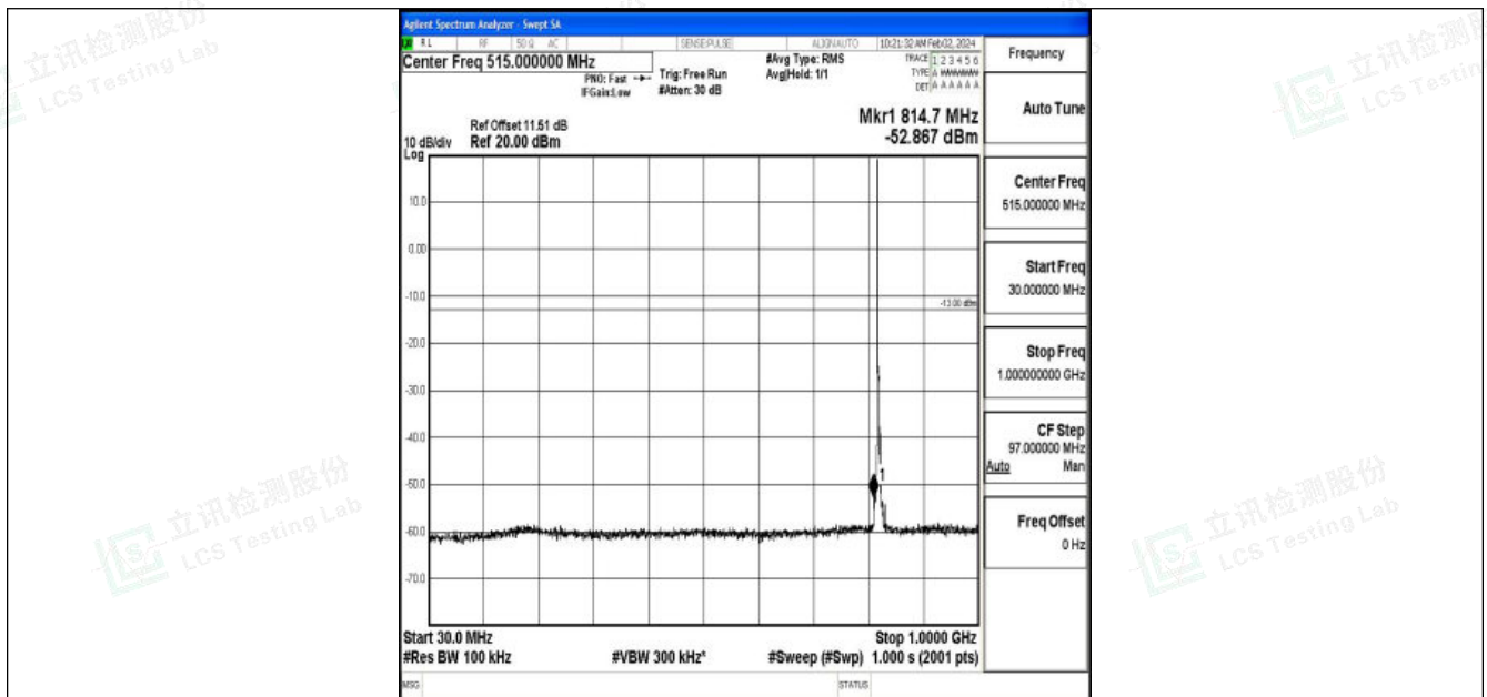
Band26_3MHz_QPSK_26775_1RB#0_30~1000_30~1000
