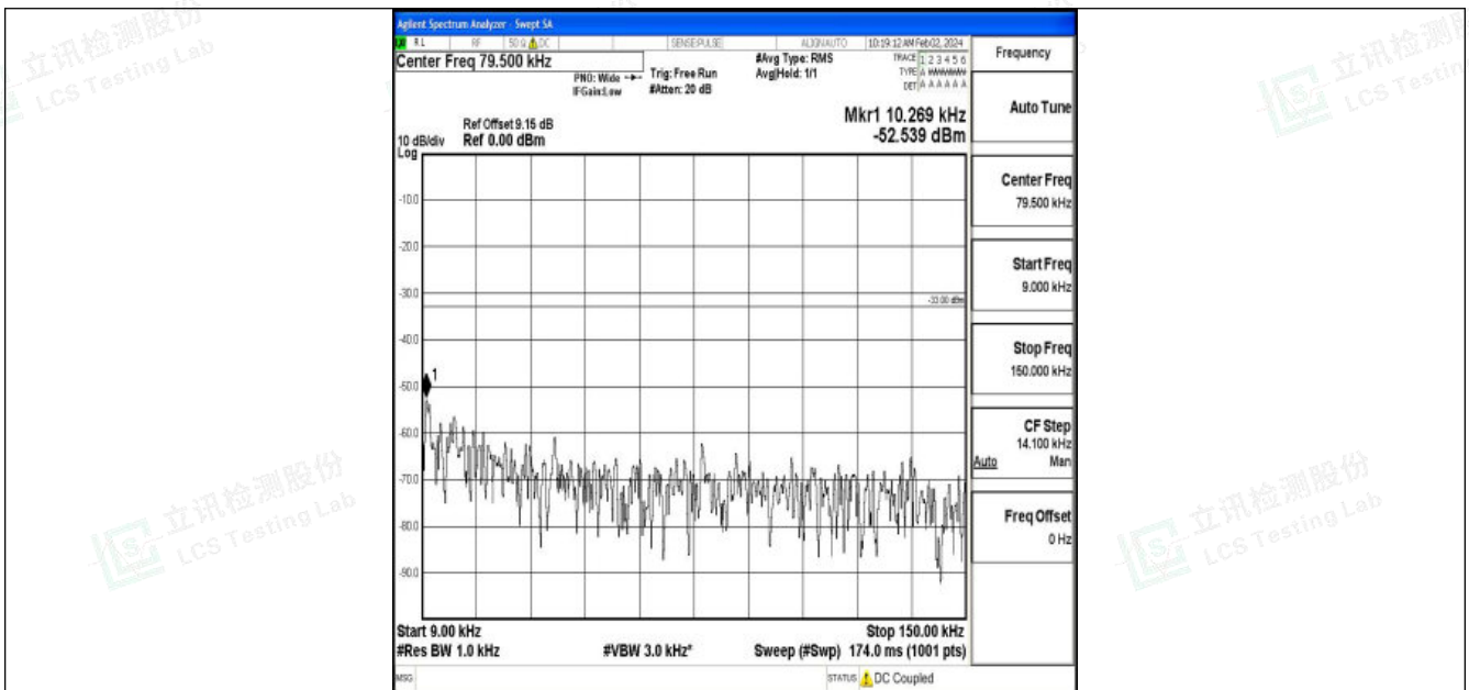
Band26_3MHz_QPSK_26705_1RB#0_0.009~0.15_0.009~0.15
