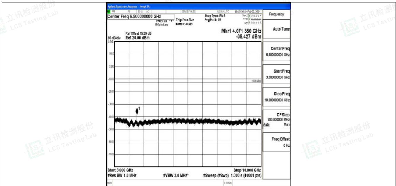
Band26_3MHz_QPSK_26705_1RB#0_3000~10000_3000~10000
