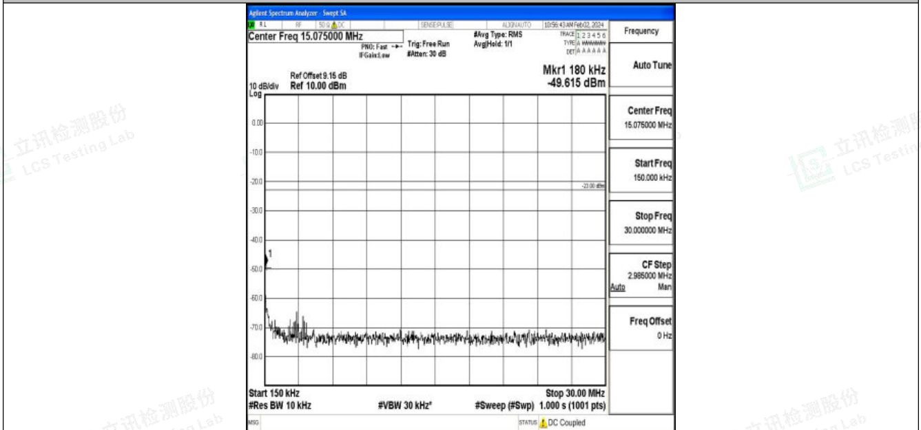
Band26_10MHz_QPSK_26740_1RB#0_0.15~30_0.15~30
