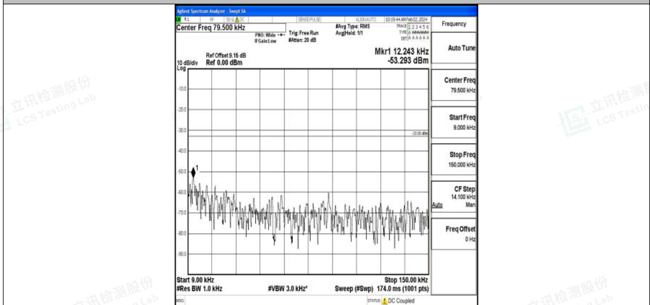
Band26_3MHz_16QAM_26705_1RB#0_0.009~0.15_0.009~0.15
