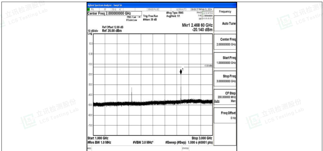
Band26_1.4MHz_16QAM_26783_1RB#0_1000~3000_1000~3000
