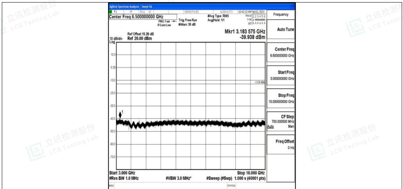
Band26_5MHz_QPSK_26765_1RB#0_3000~10000_3000~10000
