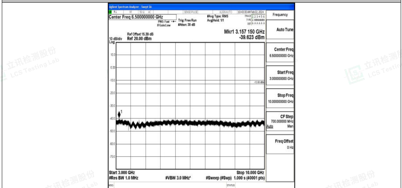
Band26_5MHz_16QAM_26765_1RB#0_3000~10000_3000~10000
