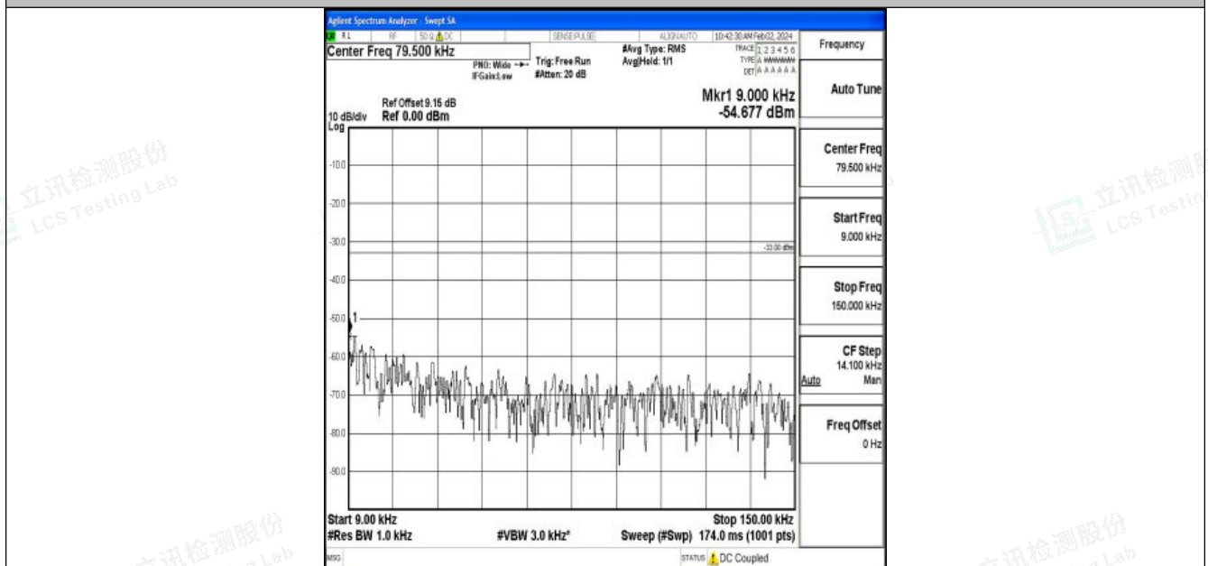
Band26_5MHz_16QAM_26765_1RB#0_0.009~0.15_0.009~0.15
