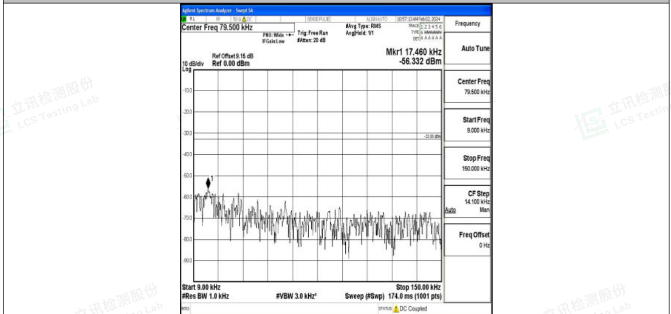
Band26_10MHz_16QAM_26740_1RB#0_0.009~0.15_0.009~0.15
