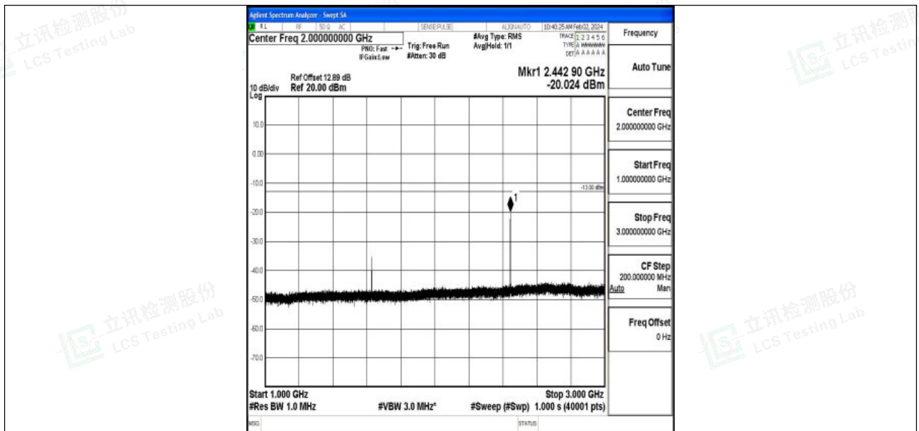
Band26_5MHz_16QAM_26715_1RB#0_1000~3000_1000~3000
