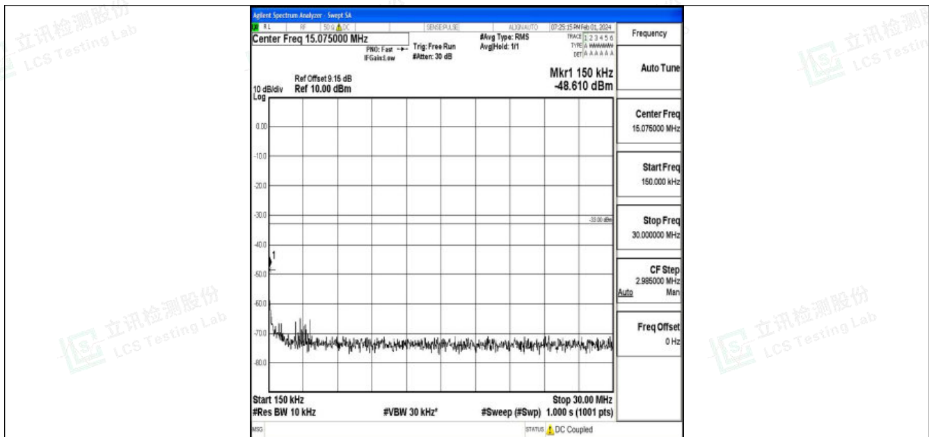
Band25_15MHz_16QAM_26615_1RB#0_0.15~30_0.15~30
