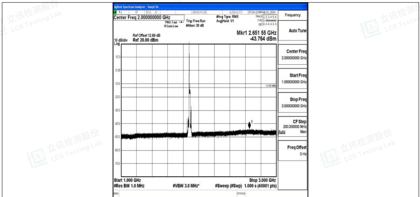
Band25_15MHz_16QAM_26365_1RB#0_1000~3000_1000~3000
