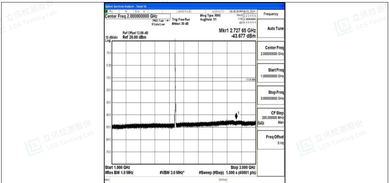
Band25_5MHz_16QAM_26365_1RB#0_1000~3000_1000~3000
