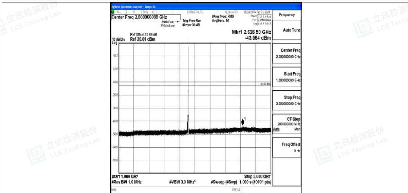
Band25_5MHz_16QAM_26665_1RB#0_1000~3000_1000~3000
