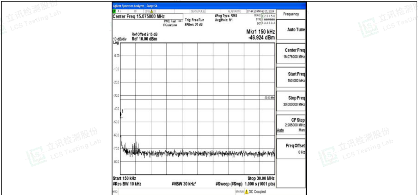
Band25_20MHz_16QAM_26140_1RB#0_0.15~30_0.15~30
