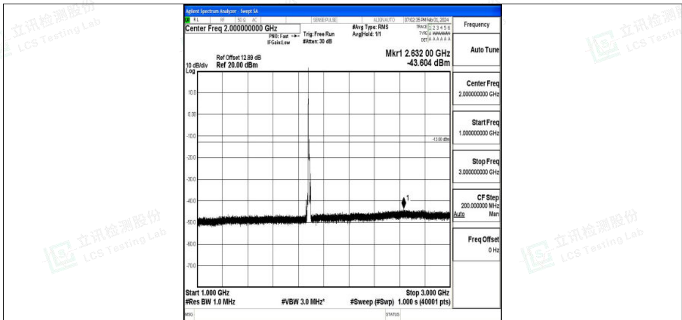
Band25_10MHz_16QAM_26365_1RB#0_1000~3000_1000~3000
