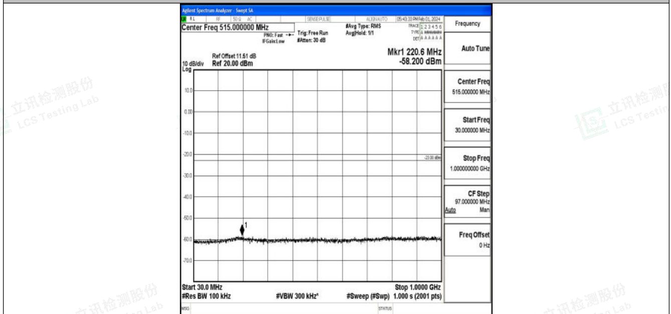
Band25_1.4MHz_16QAM_26683_1RB#0_30~1000_30~1000
