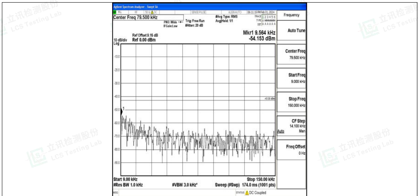
Band25_3MHz_QPSK_26055_1RB#0_0.009~0.15_0.009~0.15
