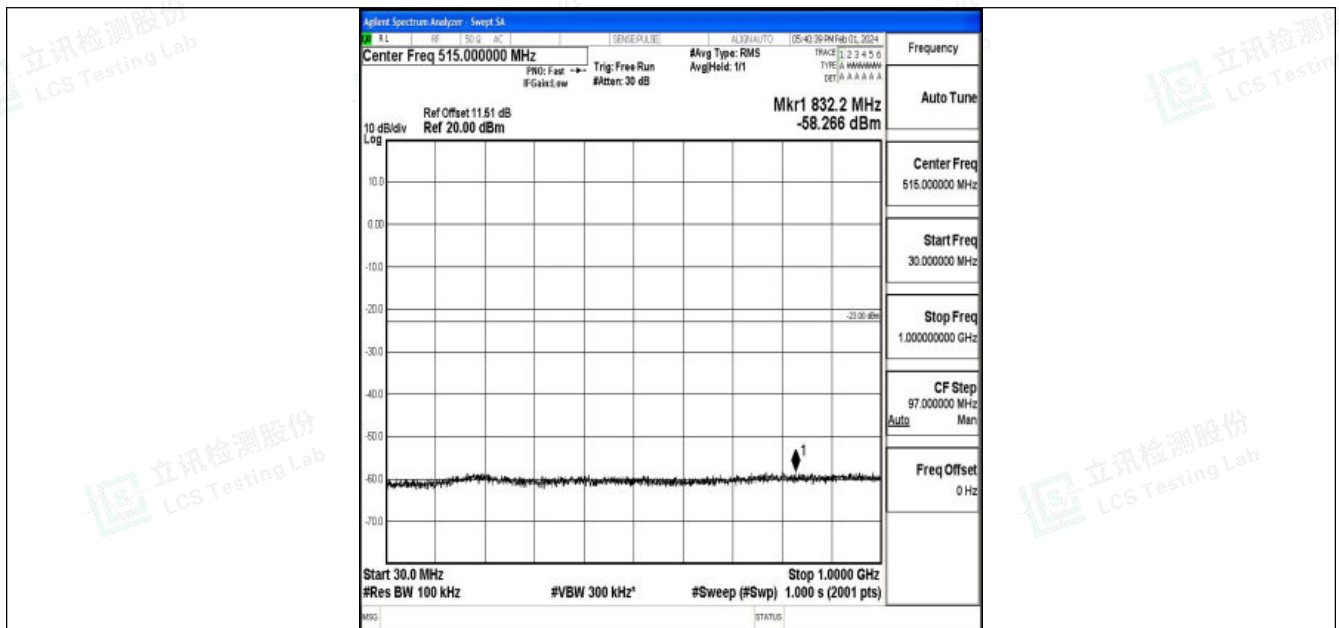
Band25_1.4MHz_QPSK_26047_1RB#0_30~1000_30~1000
