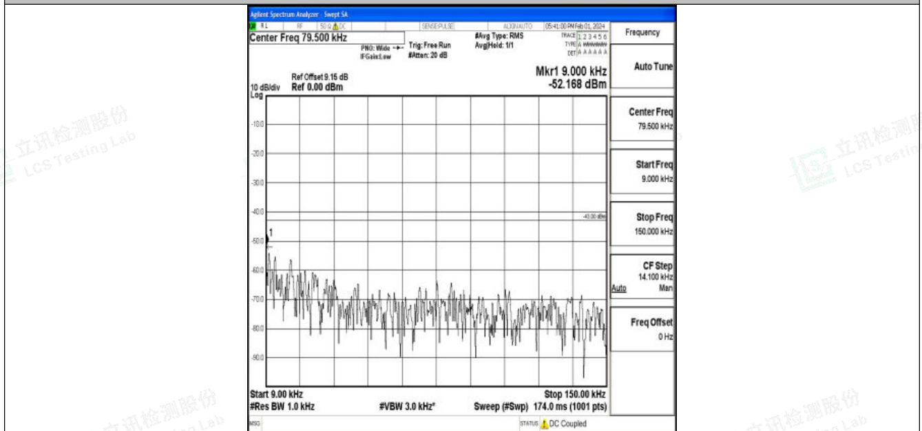
Band25_1.4MHz_16QAM_26047_1RB#0_0.009~0.15_0.009~0.15
