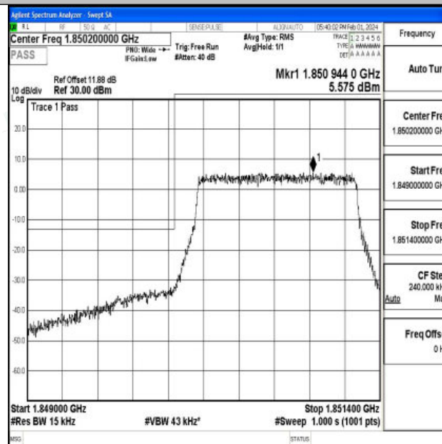
Band25_1.4MHz_16QAM_26047_6RB#0
