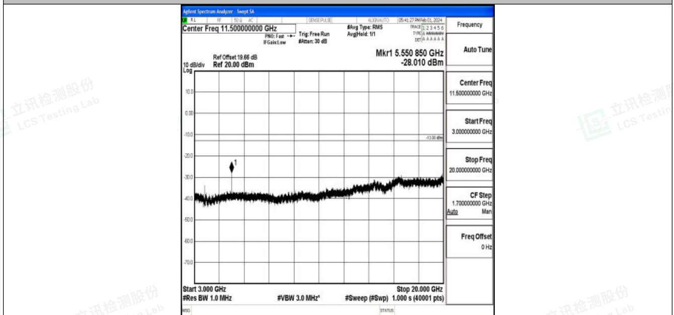
Band25_1.4MHz_16QAM_26047_1RB#0_3000~20000_3000~20000
