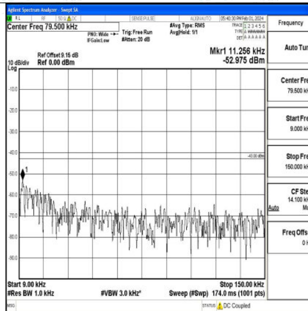
Band25_1.4MHz_QPSK_26047_1RB#0_0.009~0.15_0.009~0.15
