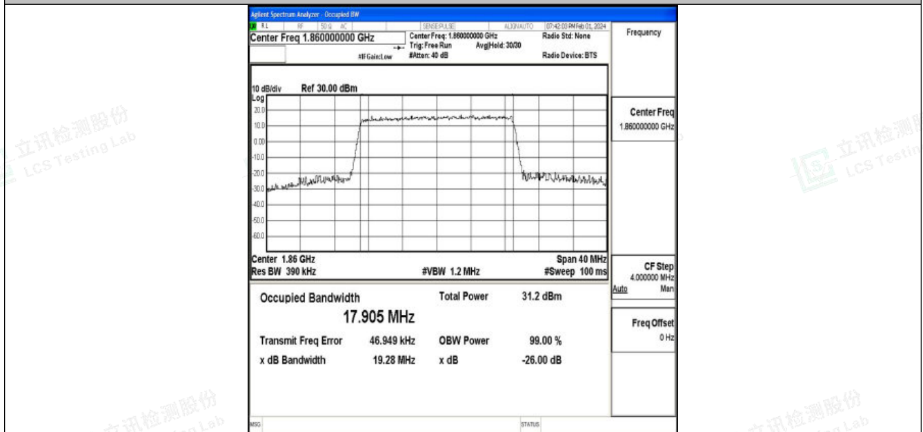
Band25-20MHz-16QAM-26140-100RB#0-PASS
