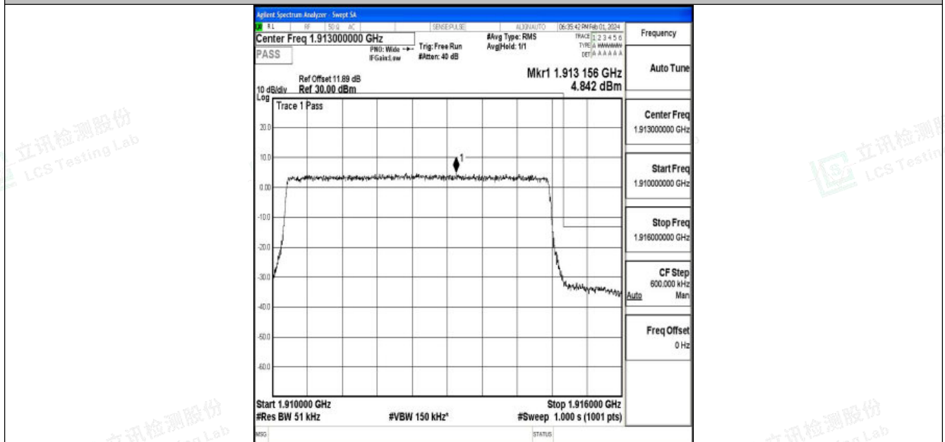
Band25_5MHz_16QAM_26665_25RB#0
