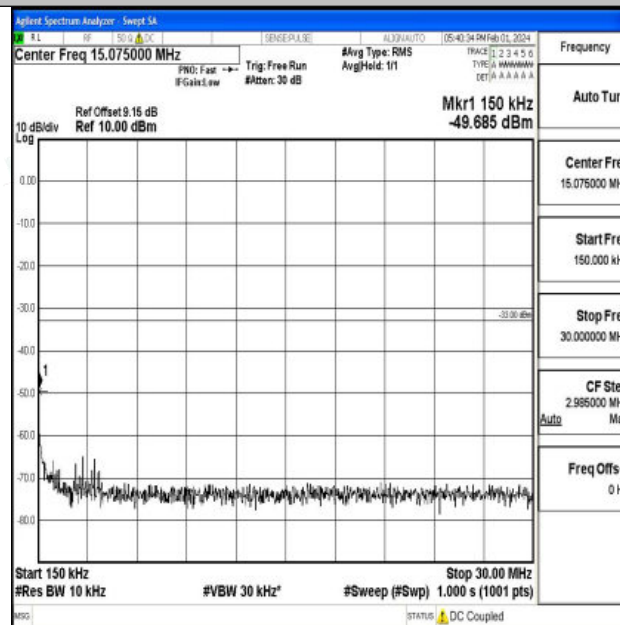
Band25_1.4MHz_QPSK_26047_1RB#0_0.15~30_0.15~30
