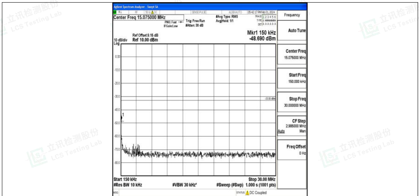
Band25_1.4MHz_16QAM_26365_1RB#0_0.15~30_0.15~30
