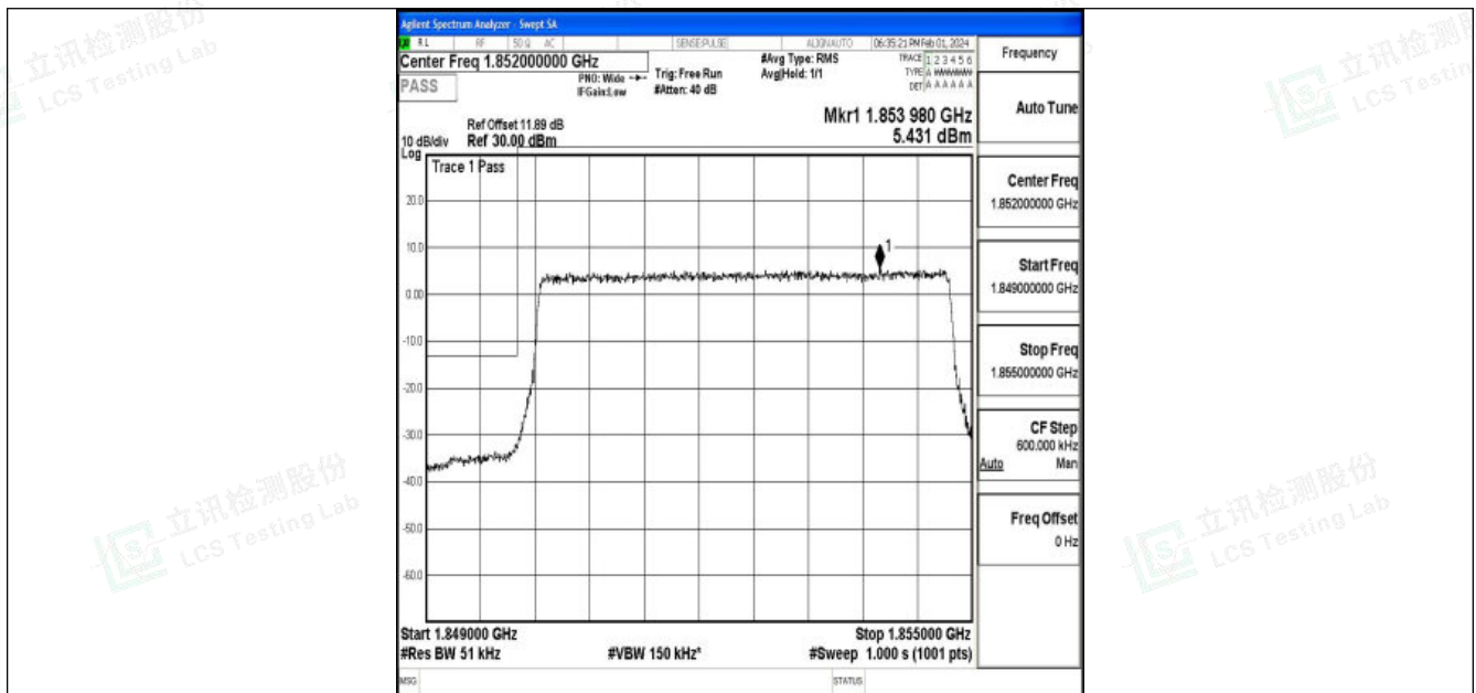
Band25_5MHz_QPSK_26065_25RB#0
