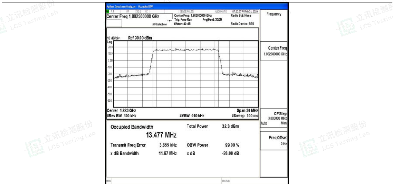
Band25-15MHz-QPSK-26365-75RB#0-PASS
