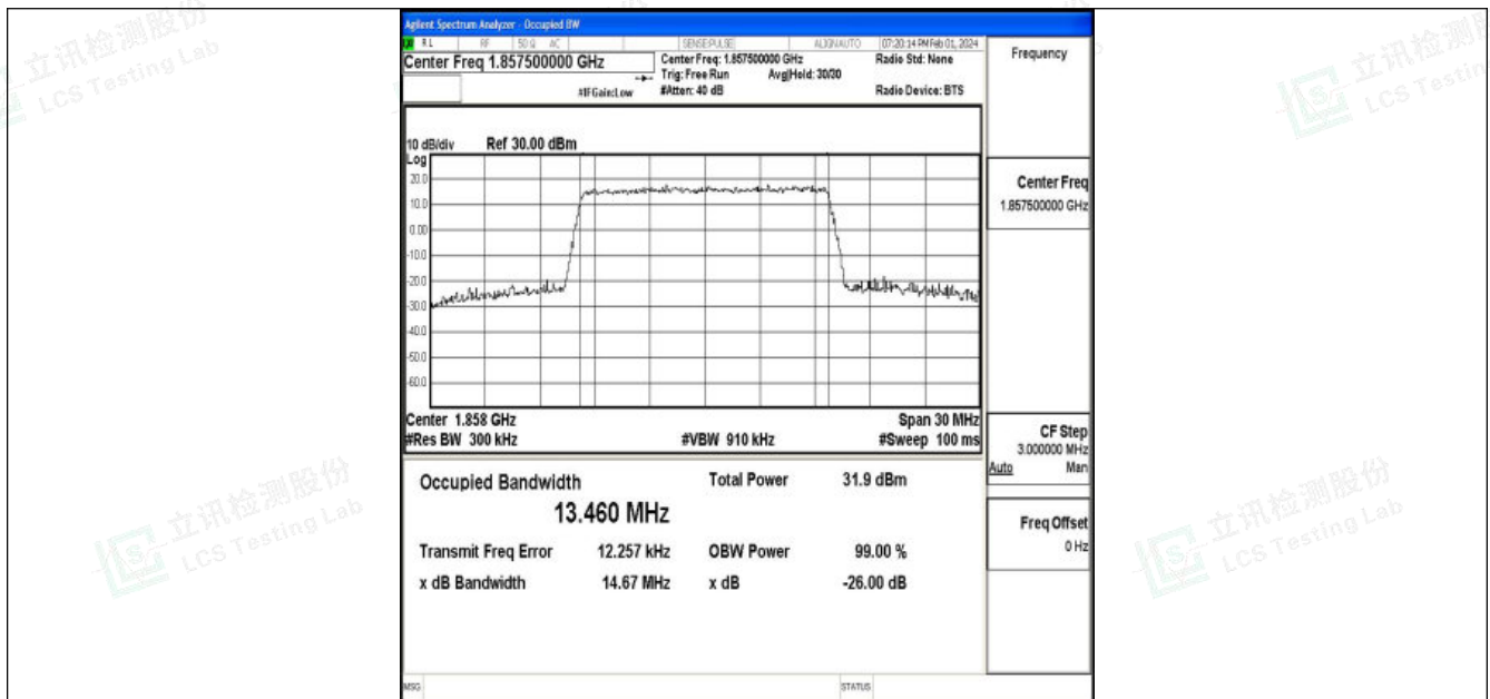
Band25-15MHz-QPSK-26115-75RB#0-PASS
