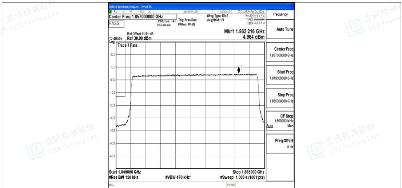
Band25_15MHz_QPSK_26115_75RB#0
