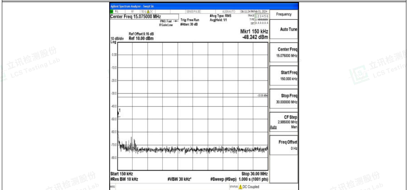
Band25_3MHz_QPSK_26055_1RB#0_0.15~30_0.15~30
