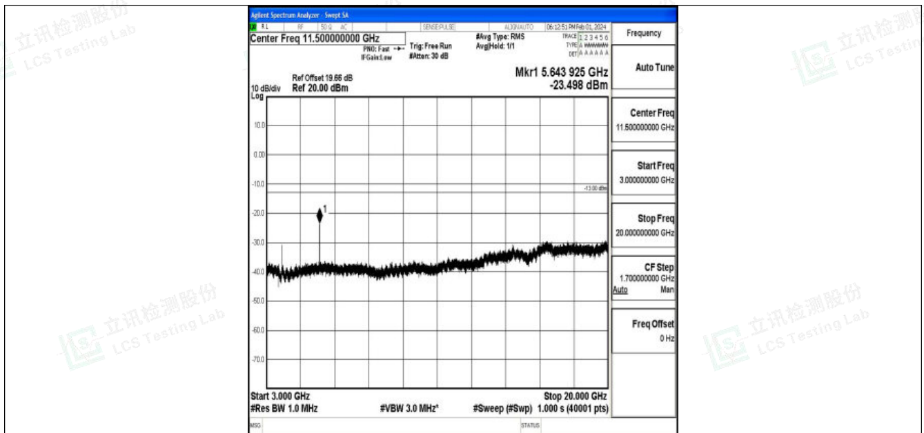
Band25_3MHz_QPSK_26365_1RB#0_3000~20000_3000~20000
