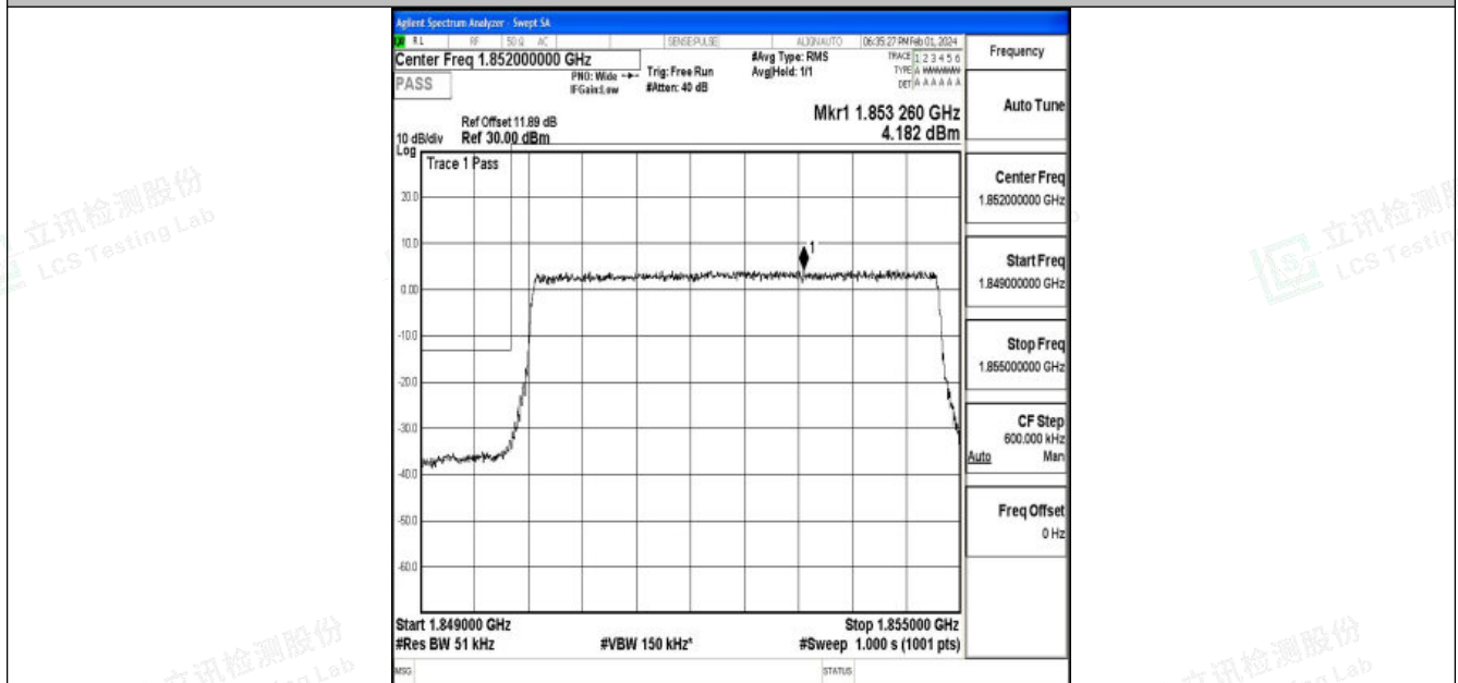
Band25_5MHz_16QAM_26065_25RB#0
