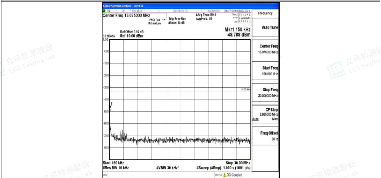
Band25_5MHz_QPSK_26365_1RB#0_0.15~30_0.15~30
