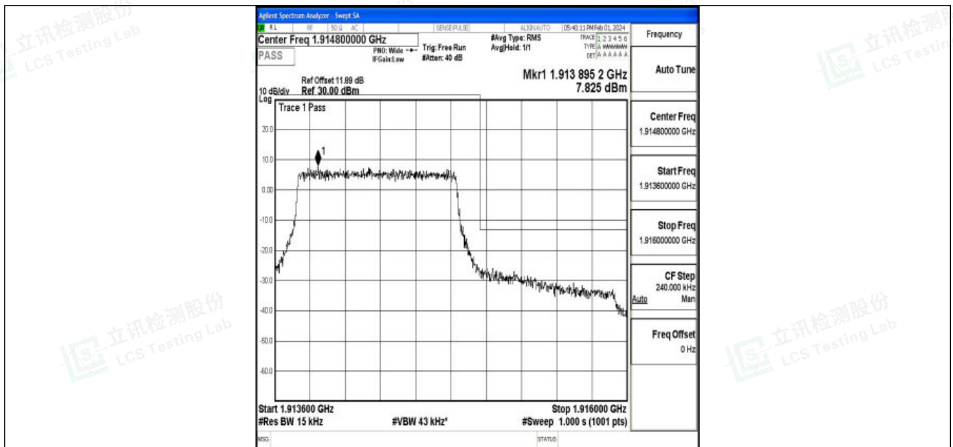
Band25_1.4MHz_QPSK_26683_6RB#0
