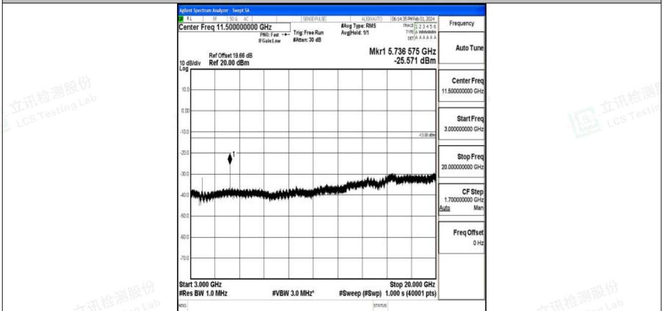
Band25_3MHz_16QAM_26675_1RB#0_3000~20000_3000~20000
