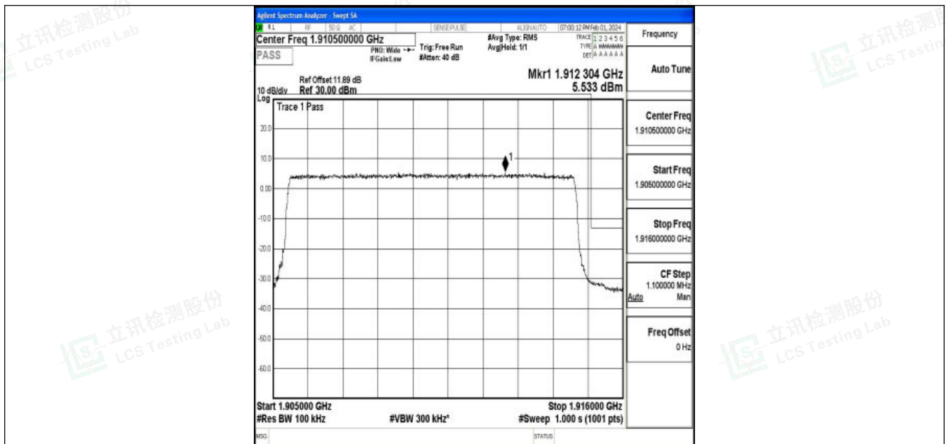
Band25_10MHz_QPSK_26640_50RB#0
