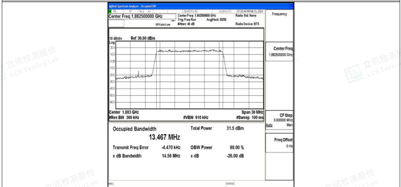
Band25-15MHz-16QAM-26365-75RB#0-PASS
