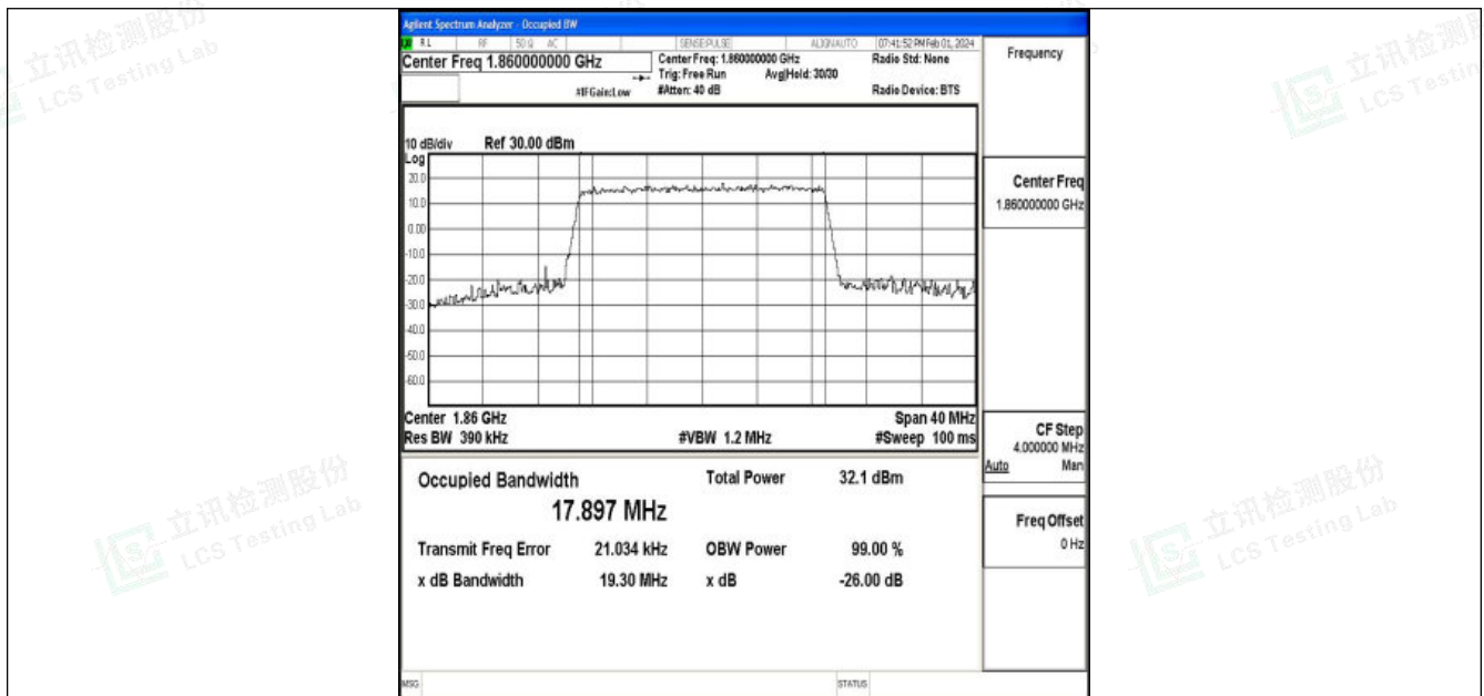
Band25-20MHz-QPSK-26140-100RB#0-PASS
