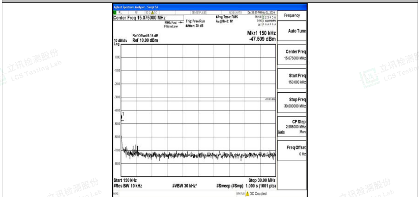
Band25_5MHz_QPSK_26065_1RB#0_0.15~30_0.15~30
