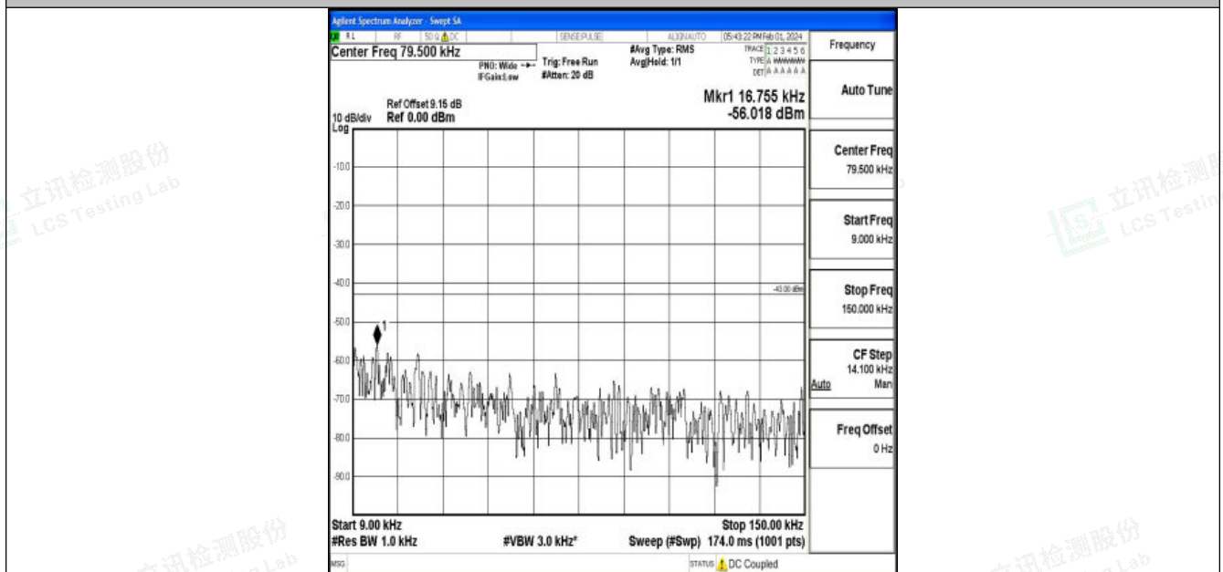
Band25_1.4MHz_16QAM_26683_1RB#0_0.009~0.15_0.009~0.15
