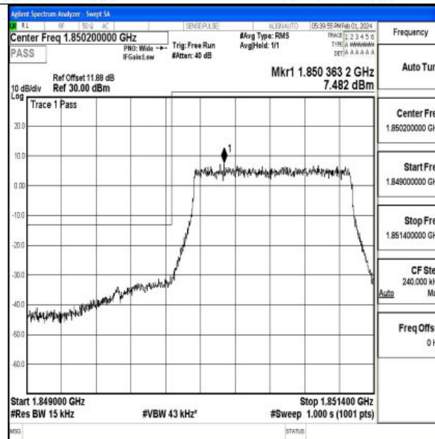
Band25_1.4MHz_QPSK_26047_6RB#0
