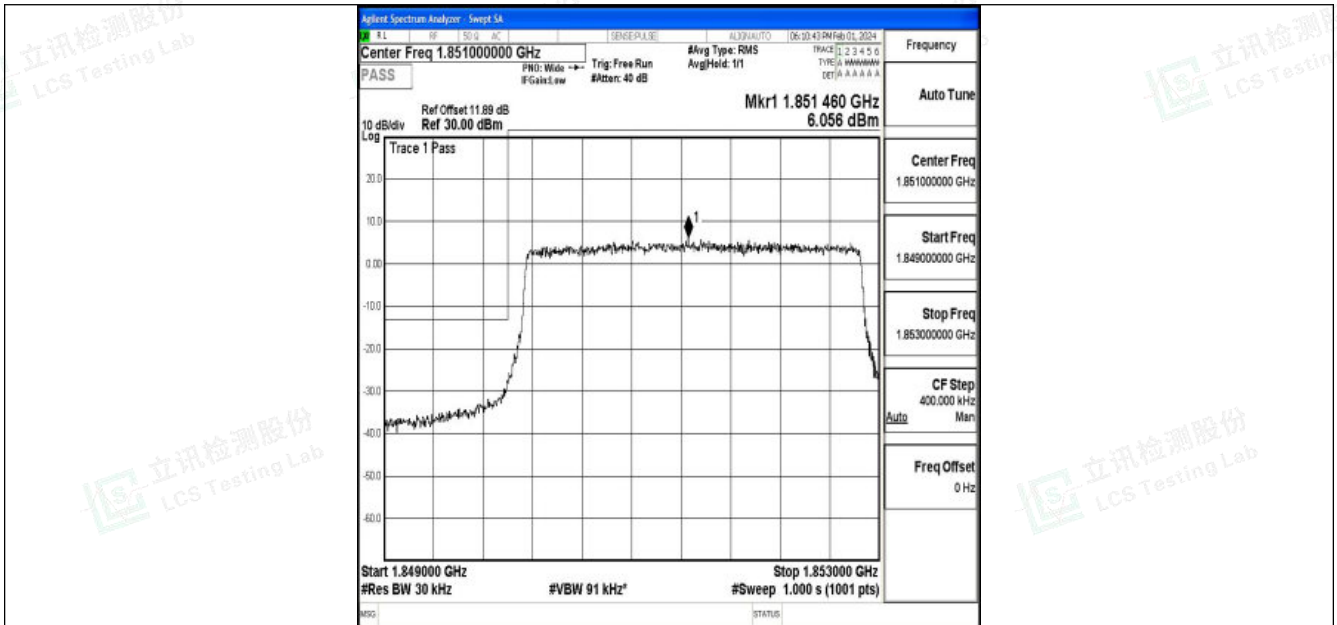
Band25_3MHz_QPSK_26055_15RB#0
