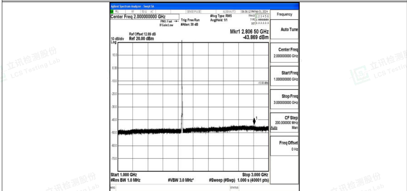
Band25_5MHz_QPSK_26065_1RB#0_1000~3000_1000~3000
