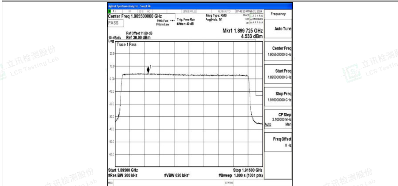
Band25_20MHz_16QAM_26590_100RB#0
