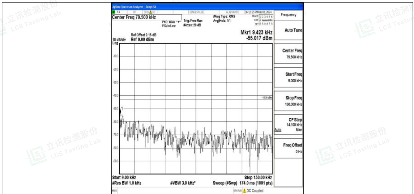
Band25_3MHz_QPSK_26365_1RB#0_0.009~0.15_0.009~0.15
