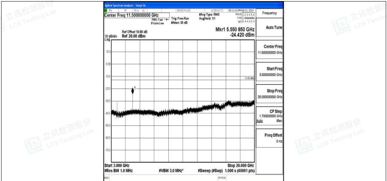
Band25_3MHz_QPSK_26055_1RB#0_3000~20000_3000~20000
