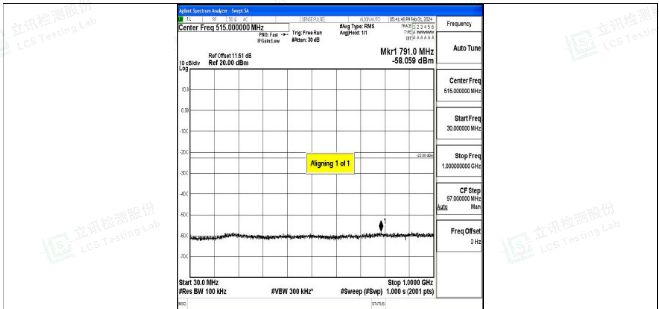
Band25_1.4MHz_QPSK_26365_1RB#0_30~1000_30~1000
