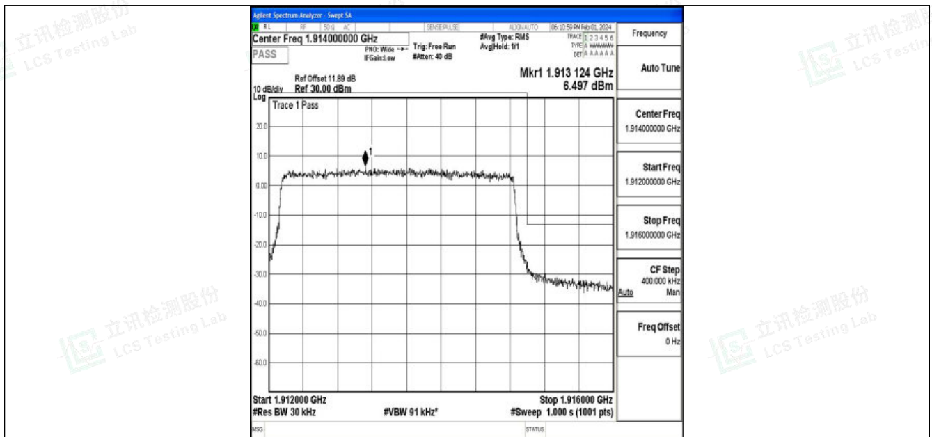
Band25_3MHz_QPSK_26675_15RB#0
