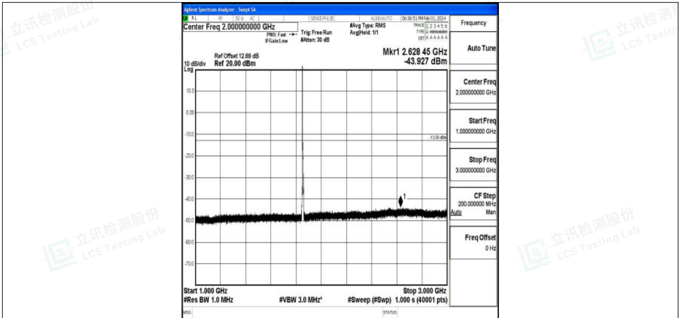
Band25_5MHz_16QAM_26065_1RB#0_1000~3000_1000~3000
