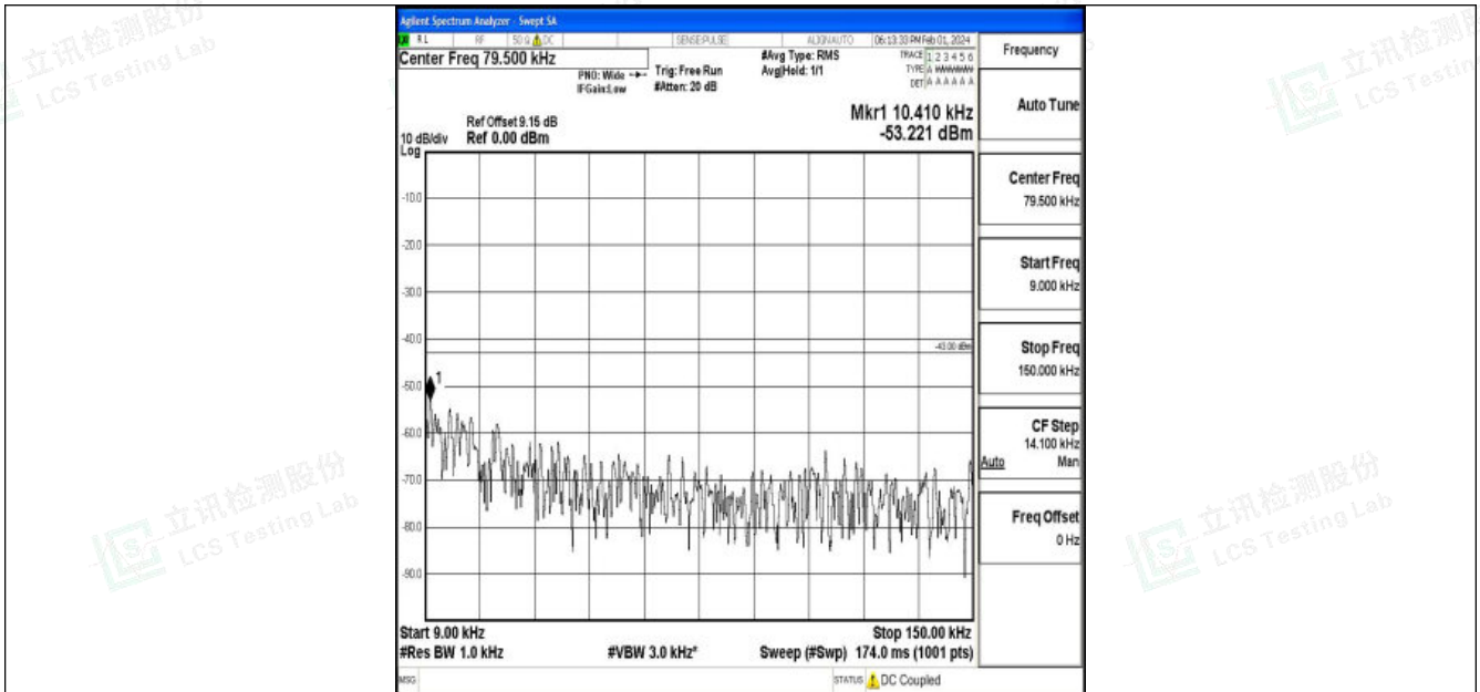
Band25_3MHz_QPSK_26675_1RB#0_0.009~0.15_0.009~0.15
