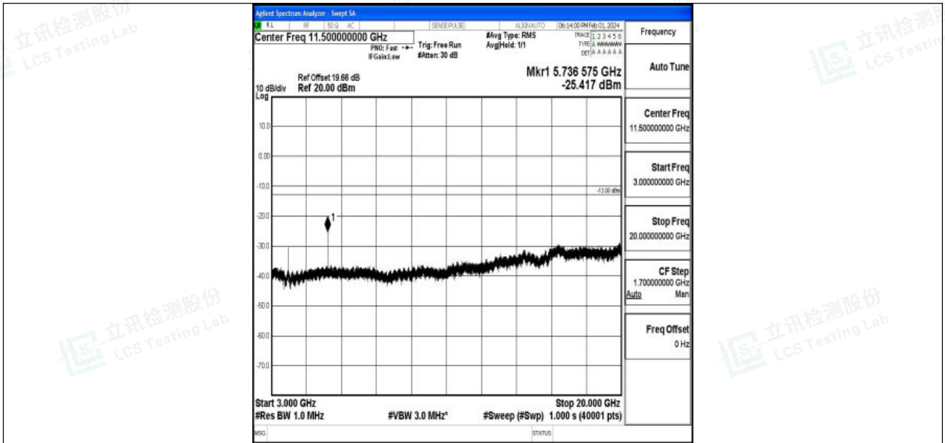
Band25_3MHz_QPSK_26675_1RB#0_3000~20000_3000~20000
