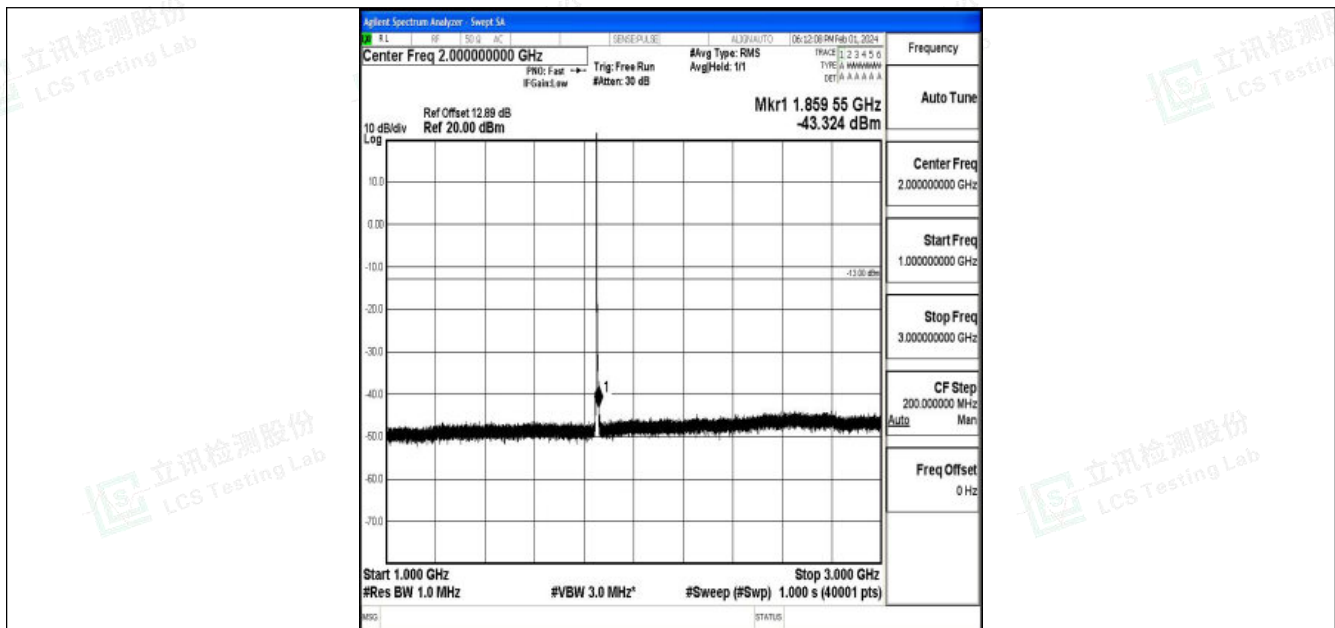
Band25_3MHz_16QAM_26055_1RB#0_1000~3000_1000~3000
