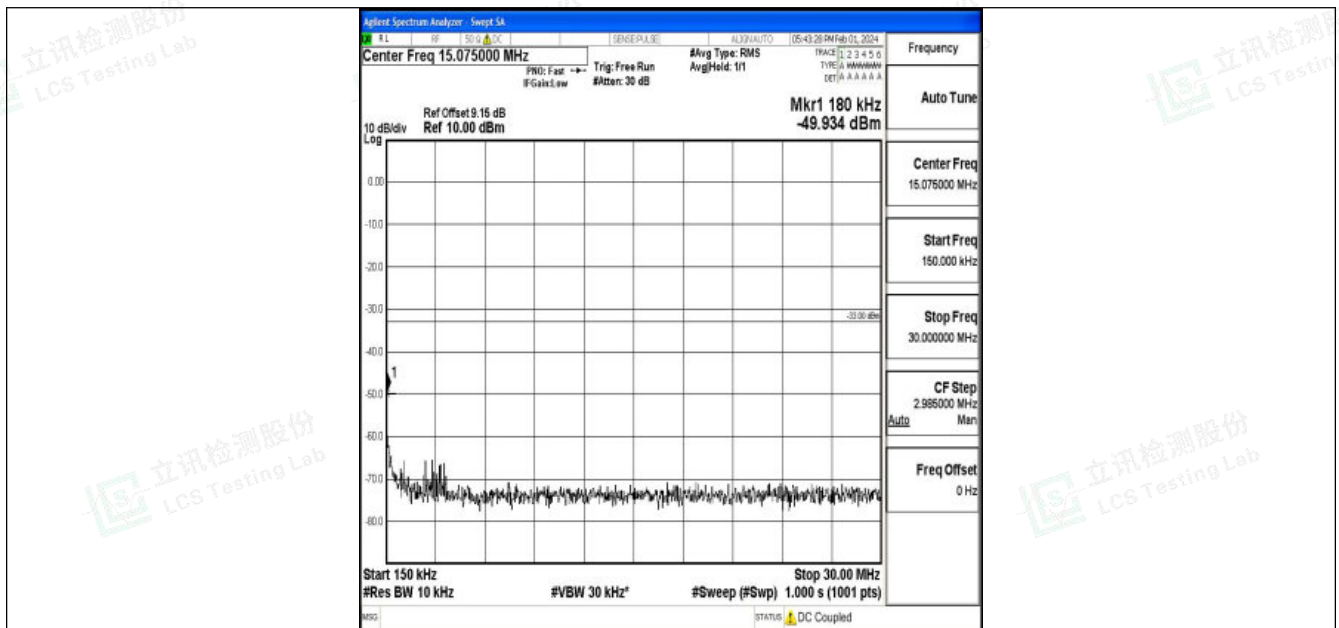
Band25_1.4MHz_16QAM_26683_1RB#0_0.15~30_0.15~30
