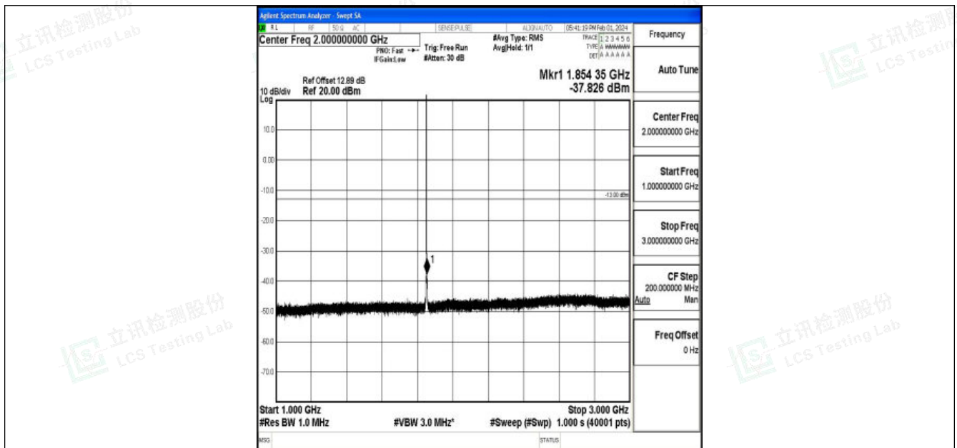
Band25_1.4MHz_16QAM_26047_1RB#0_1000~3000_1000~3000
