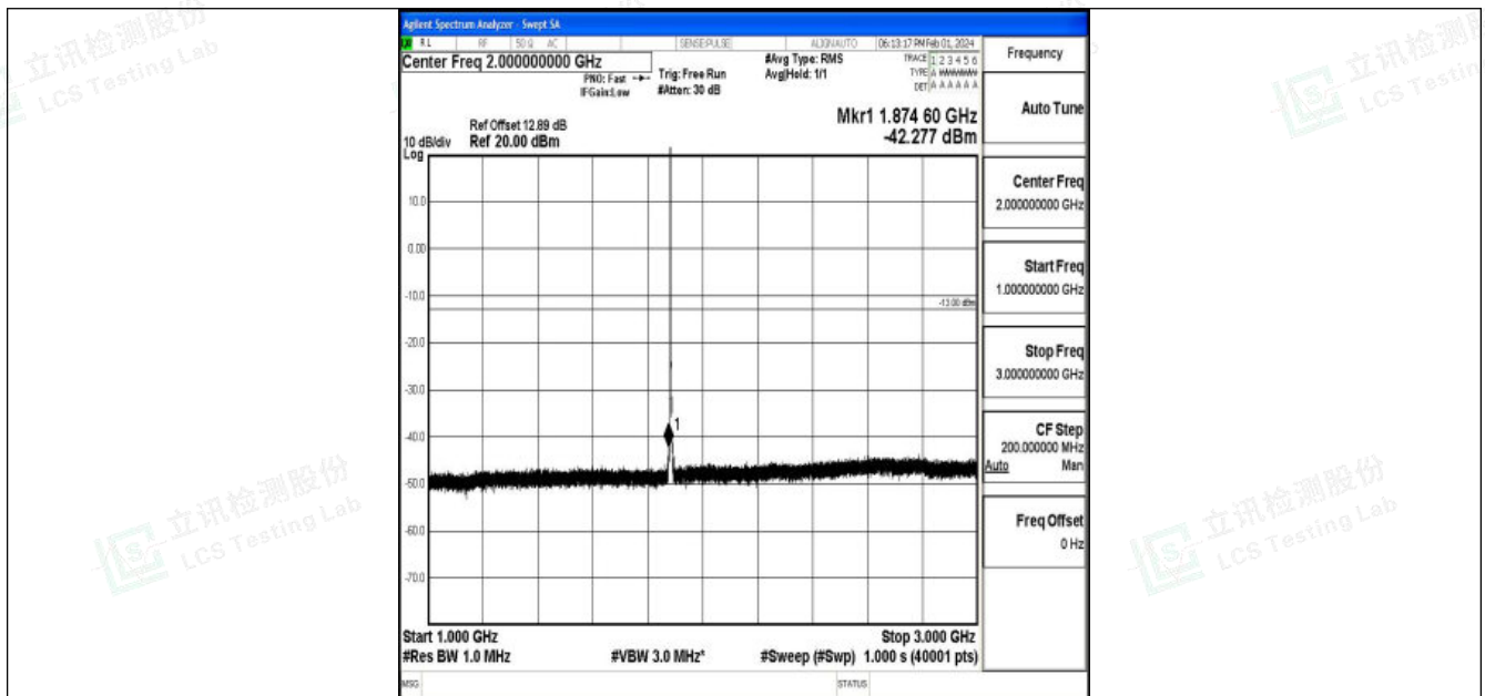
Band25_3MHz_16QAM_26365_1RB#0_1000~3000_1000~3000
