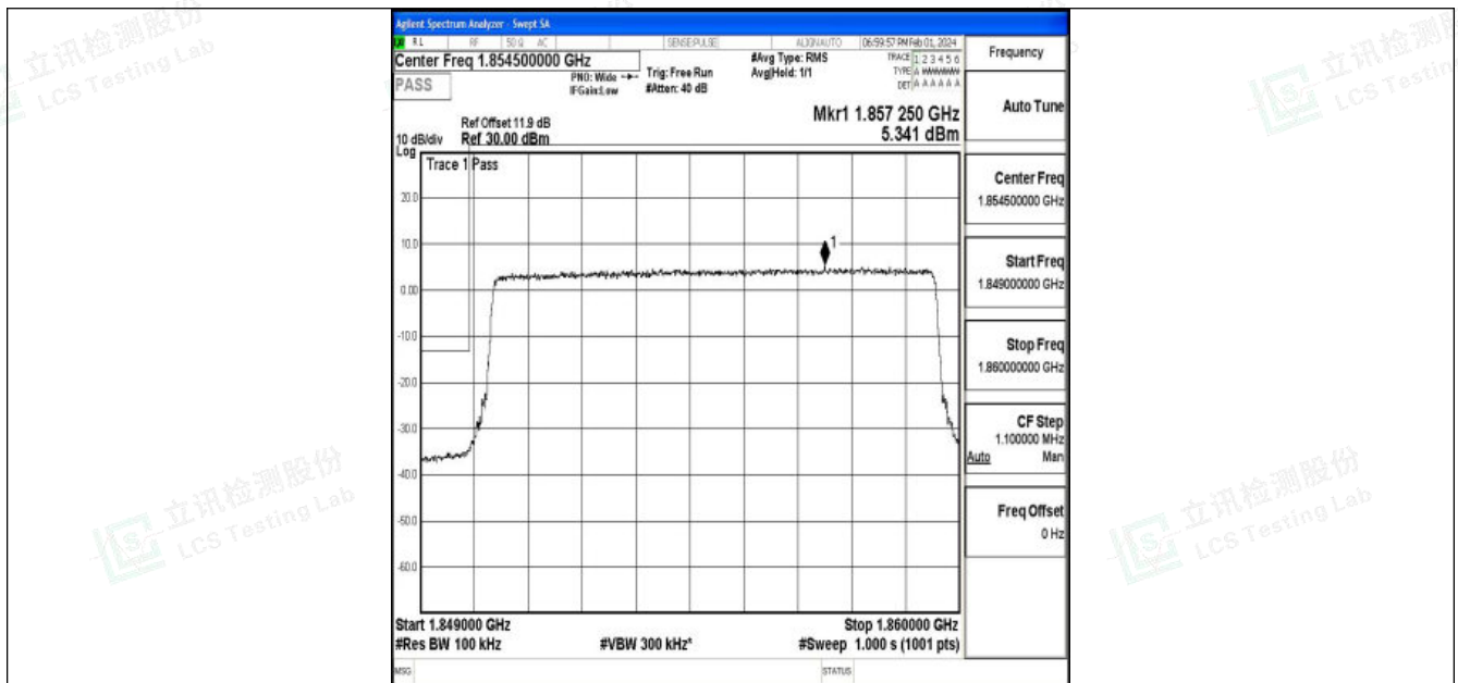
Band25_10MHz_QPSK_26090_50RB#0
