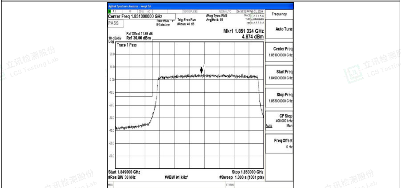
Band25_3MHz_16QAM_26055_15RB#0
