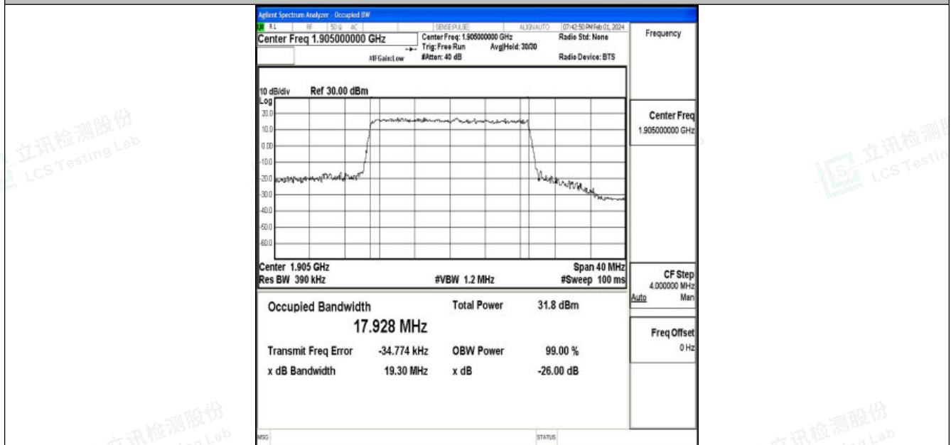
Band25-20MHz-16QAM-26590-100RB#0-PASS
