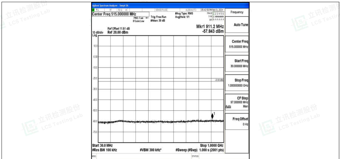
Band25_1.4MHz_QPSK_26683_1RB#0_30~1000_30~1000
