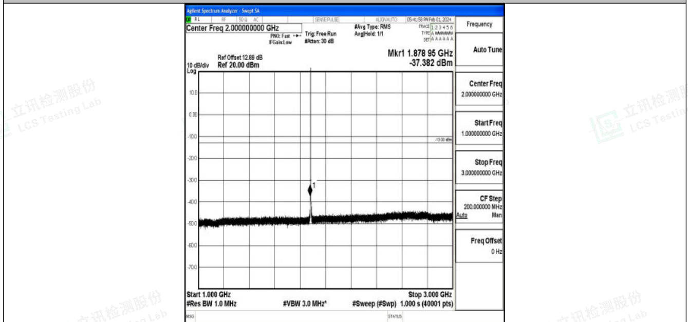
Band25_1.4MHz_QPSK_26365_1RB#0_1000~3000_1000~3000
