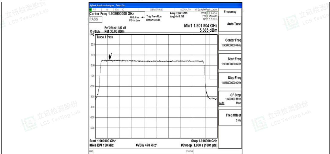
Band25_15MHz_QPSK_26615_75RB#0
