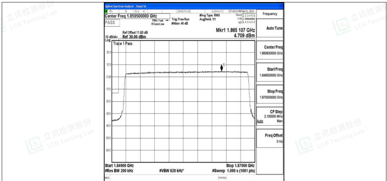
Band25_20MHz_QPSK_26140_100RB#0
