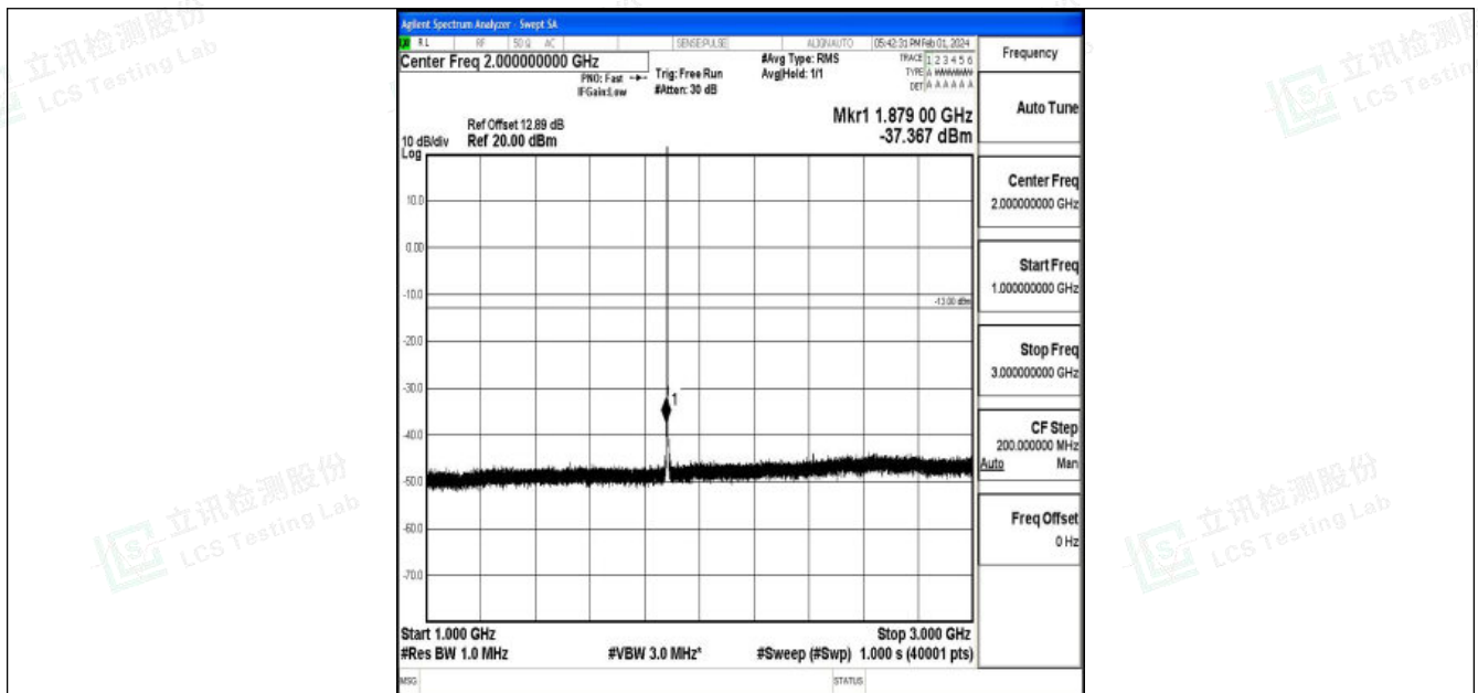
Band25_1.4MHz_16QAM_26365_1RB#0_1000~3000_1000~3000
