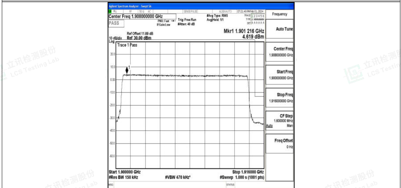
Band25_15MHz_16QAM_26615_75RB#0
