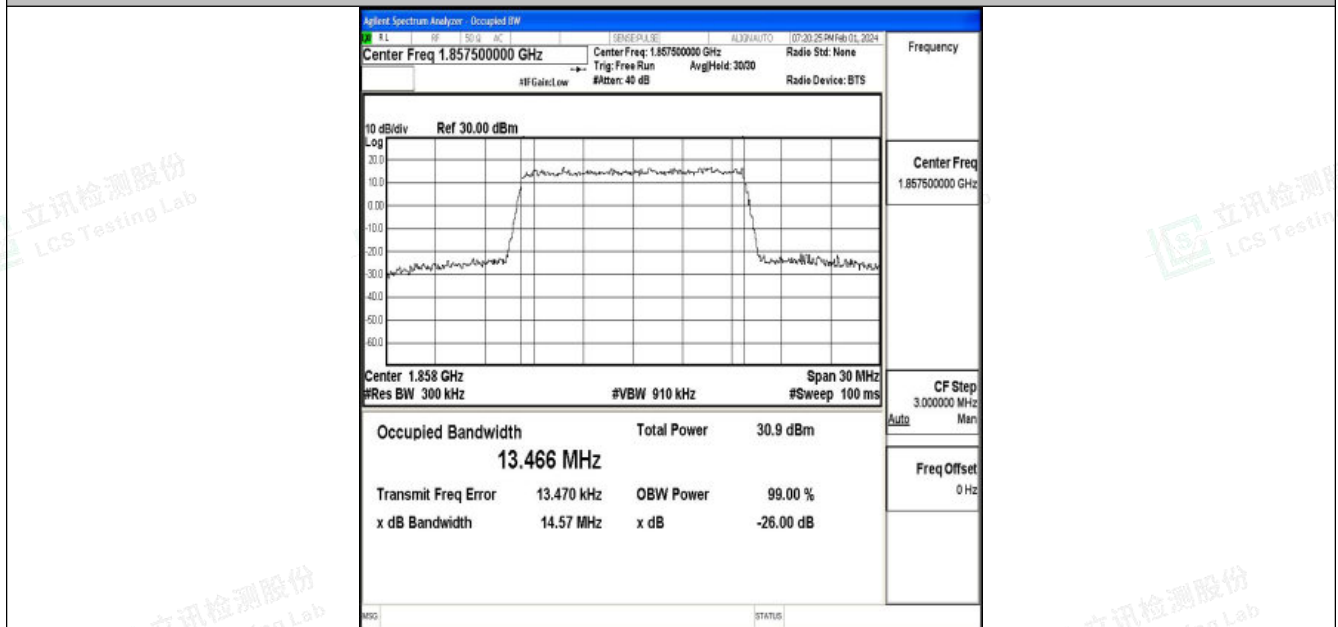
Band25-15MHz-16QAM-26115-75RB#0-PASS
