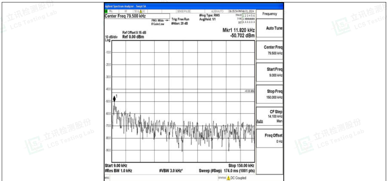
Band25_5MHz_QPSK_26065_1RB#0_0.009~0.15_0.009~0.15
