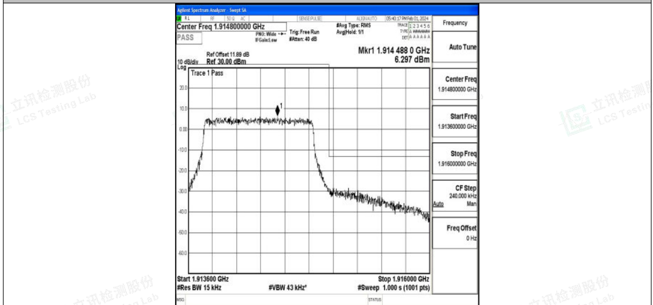
Band25_1.4MHz_16QAM_26683_6RB#0
