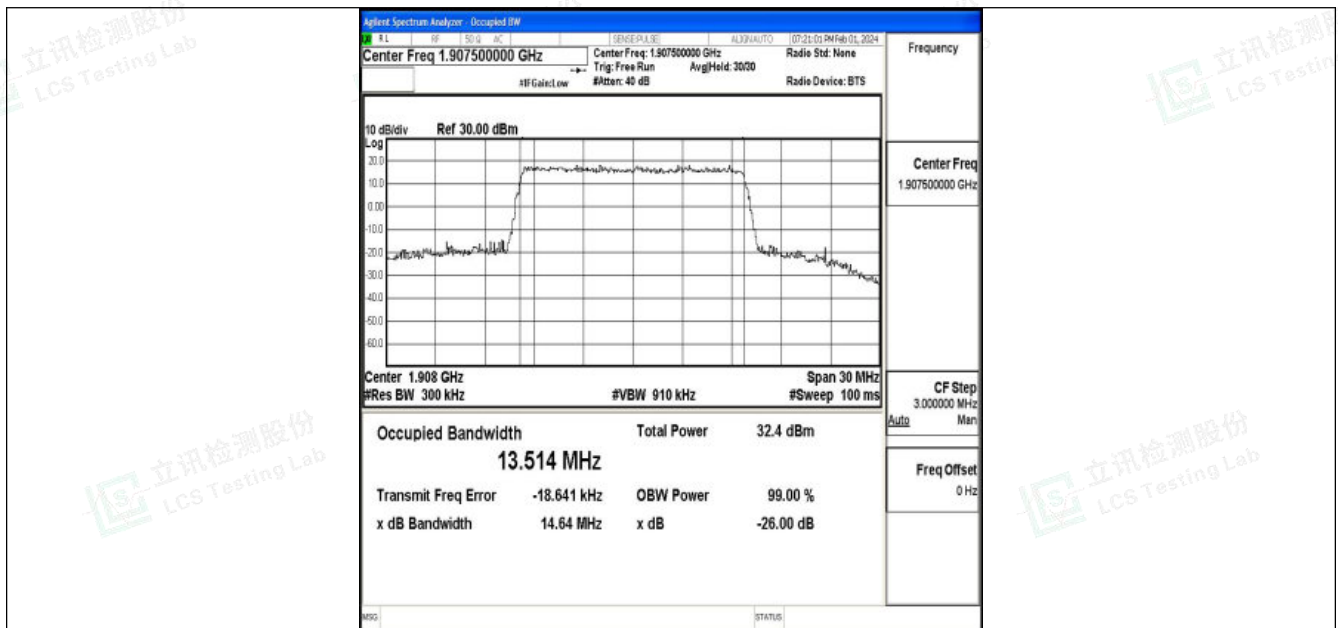
Band25-15MHz-QPSK-26615-75RB#0-PASS
