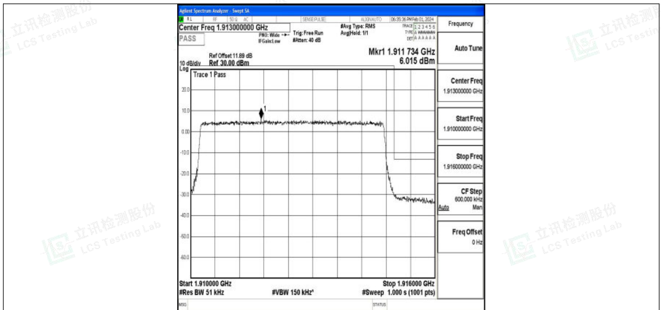
Band25_5MHz_QPSK_26665_25RB#0
