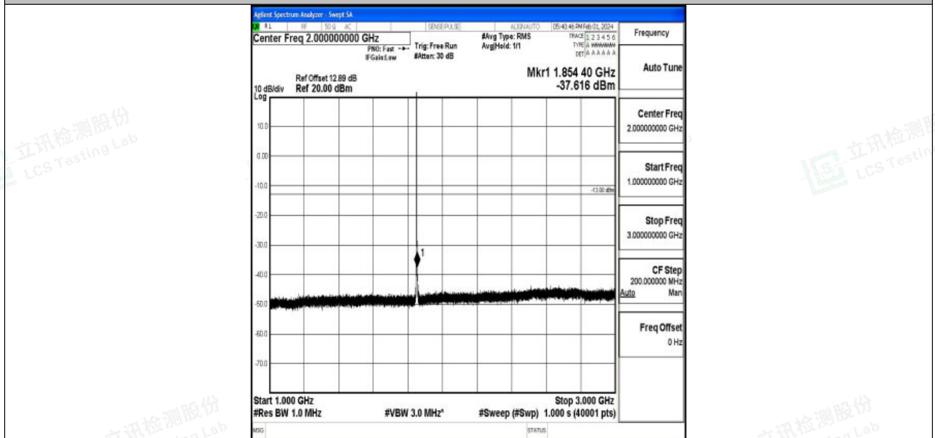
Band25_1.4MHz_QPSK_26047_1RB#0_1000~3000_1000~3000
