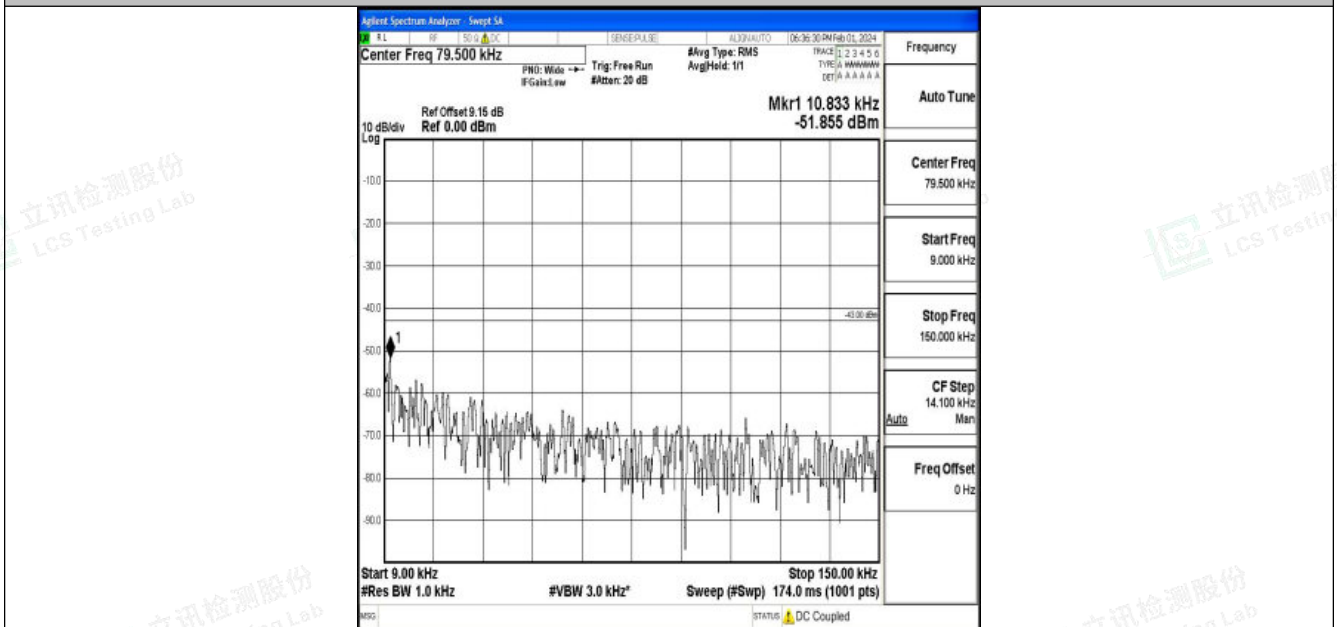
Band25_5MHz_16QAM_26065_1RB#0_0.009~0.15_0.009~0.15
