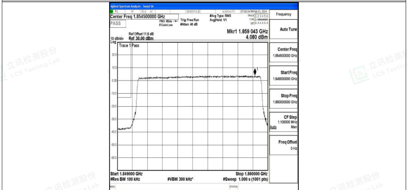
Band25_10MHz_16QAM_26090_50RB#0
