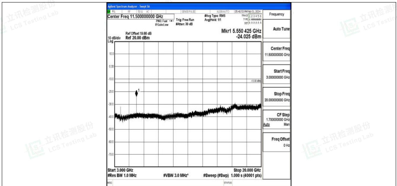
Band25_1.4MHz_QPSK_26047_1RB#0_3000~20000_3000~20000
