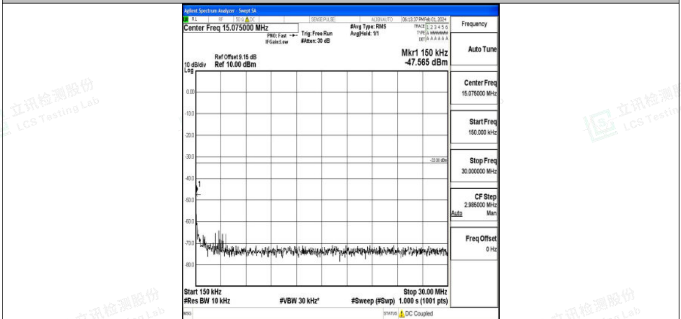
Band25_3MHz_QPSK_26675_1RB#0_0.15~30_0.15~30
