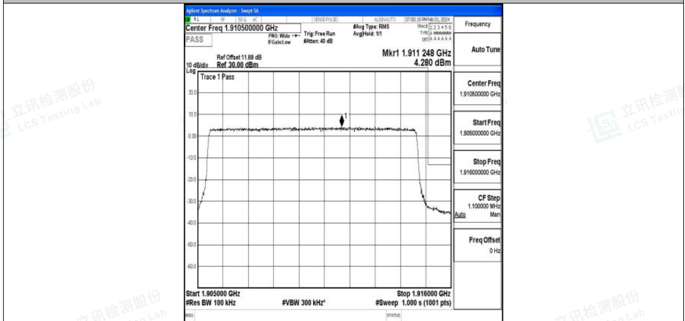
Band25_10MHz_16QAM_26640_50RB#0
