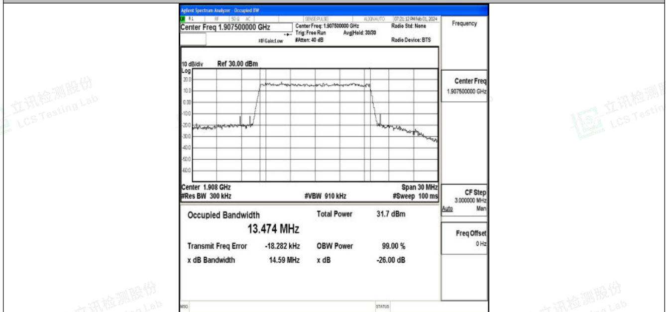
Band25-15MHz-16QAM-26615-75RB#0-PASS
