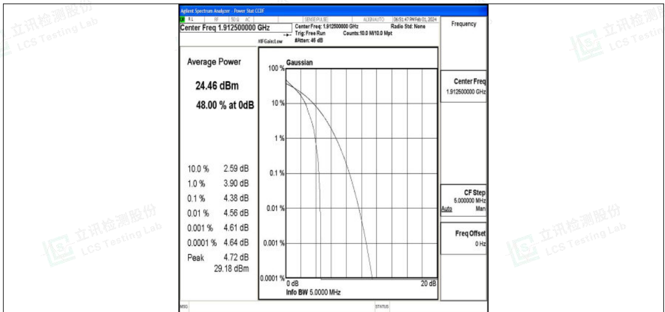
Band25-5MHz-QPSK-26665-1RB#0-PASS
