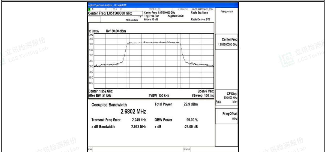
Band25-3MHz-16QAM-26055-15RB#0-PASS
