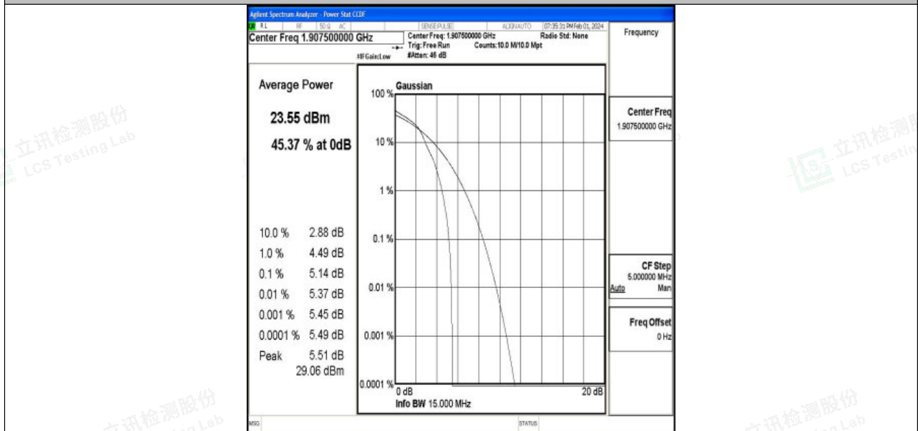
Band25-15MHz-16QAM-26615-1RB#0-PASS
