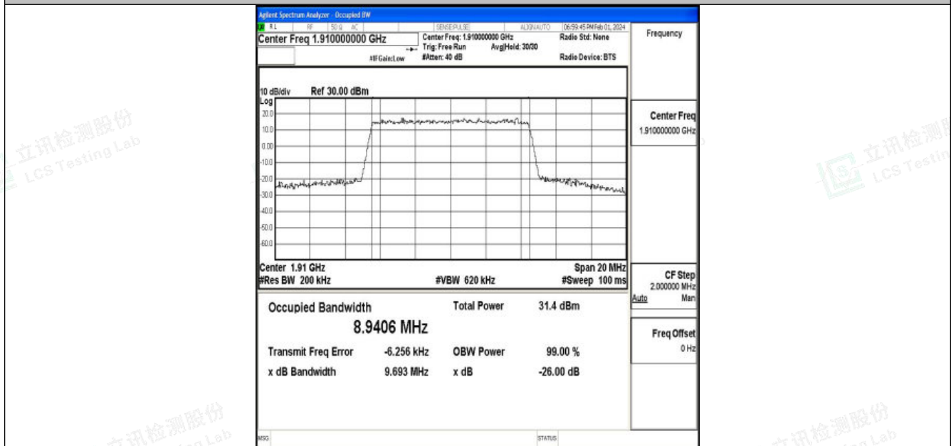
Band25-10MHz-16QAM-26640-50RB#0-PASS
