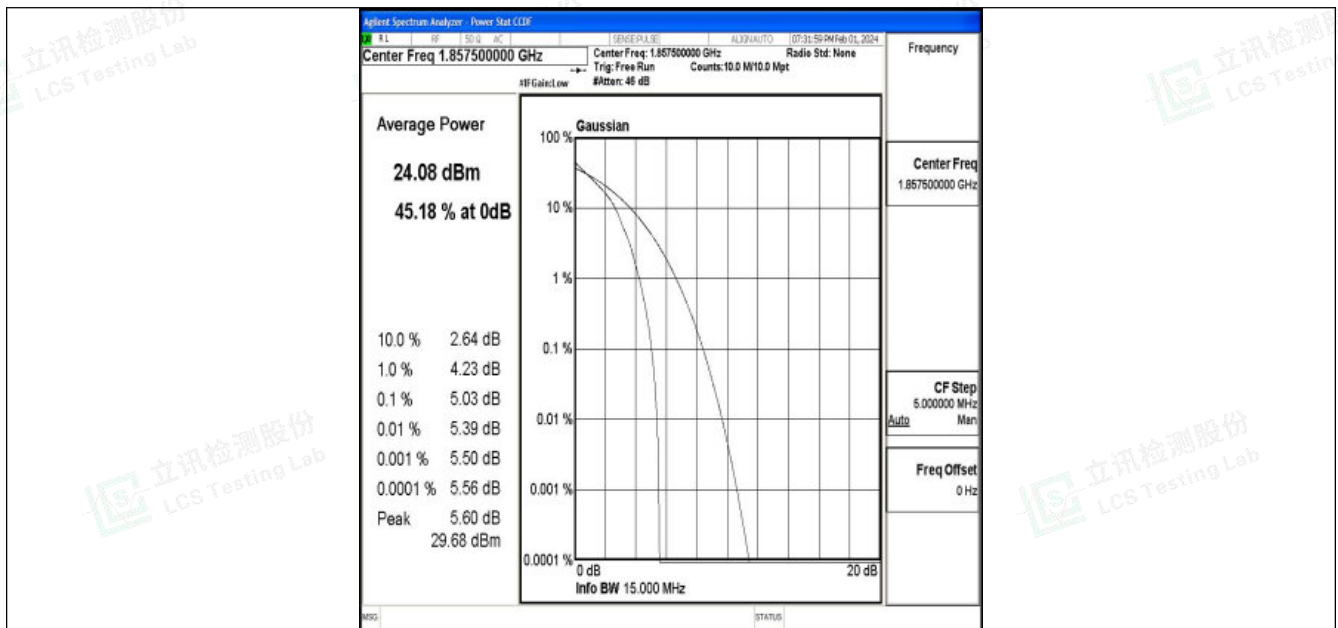
Band25-15MHz-QPSK-26115-1RB#0-PASS
