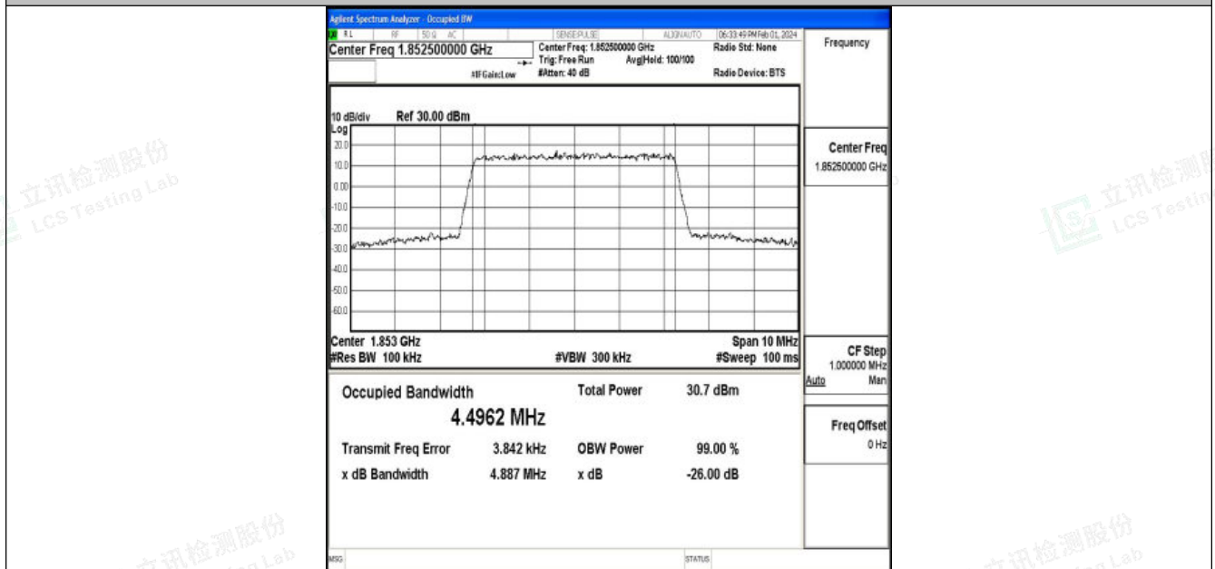
Band25-5MHz-16QAM-26065-25RB#0-PASS
