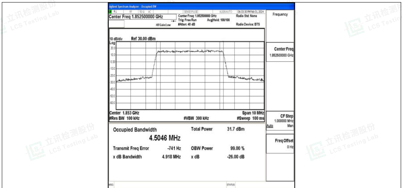
Band25-5MHz-QPSK-26065-25RB#0-PASS
