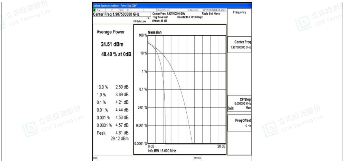
Band25-15MHz-QPSK-26615-1RB#0-PASS
