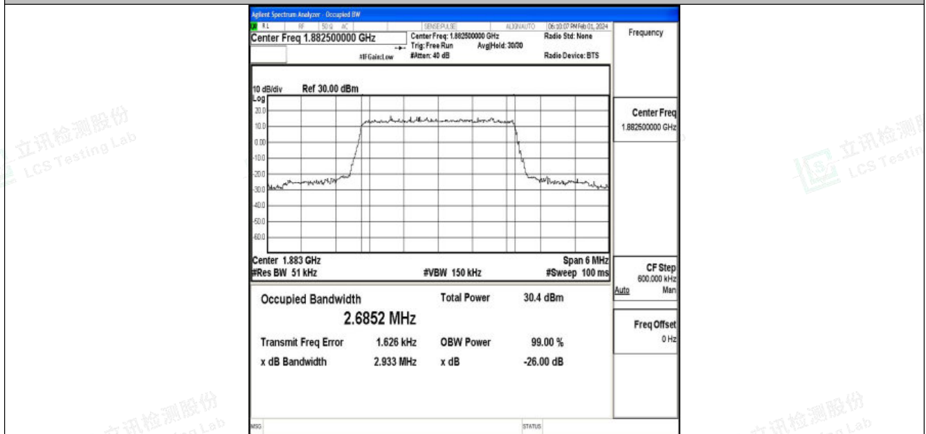
Band25-3MHz-16QAM-26365-15RB#0-PASS
