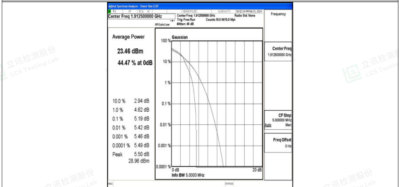
Band25-5MHz-16QAM-26665-1RB#0-PASS
