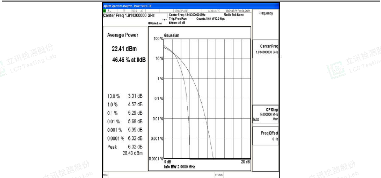
Band25-1.4MHz-16QAM-26683-6RB#0-PASS
