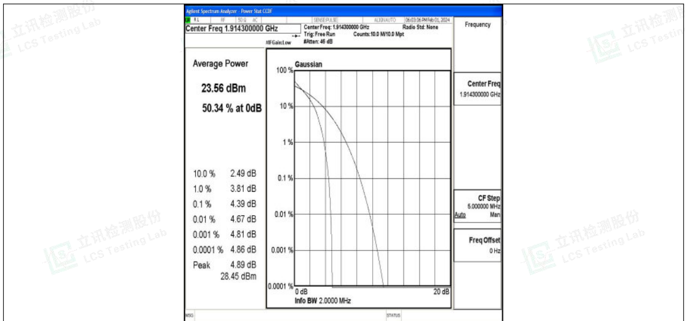
Band25-1.4MHz-QPSK-26683-6RB#0-PASS
