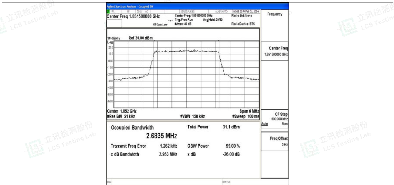
Band25-3MHz-QPSK-26055-15RB#0-PASS
