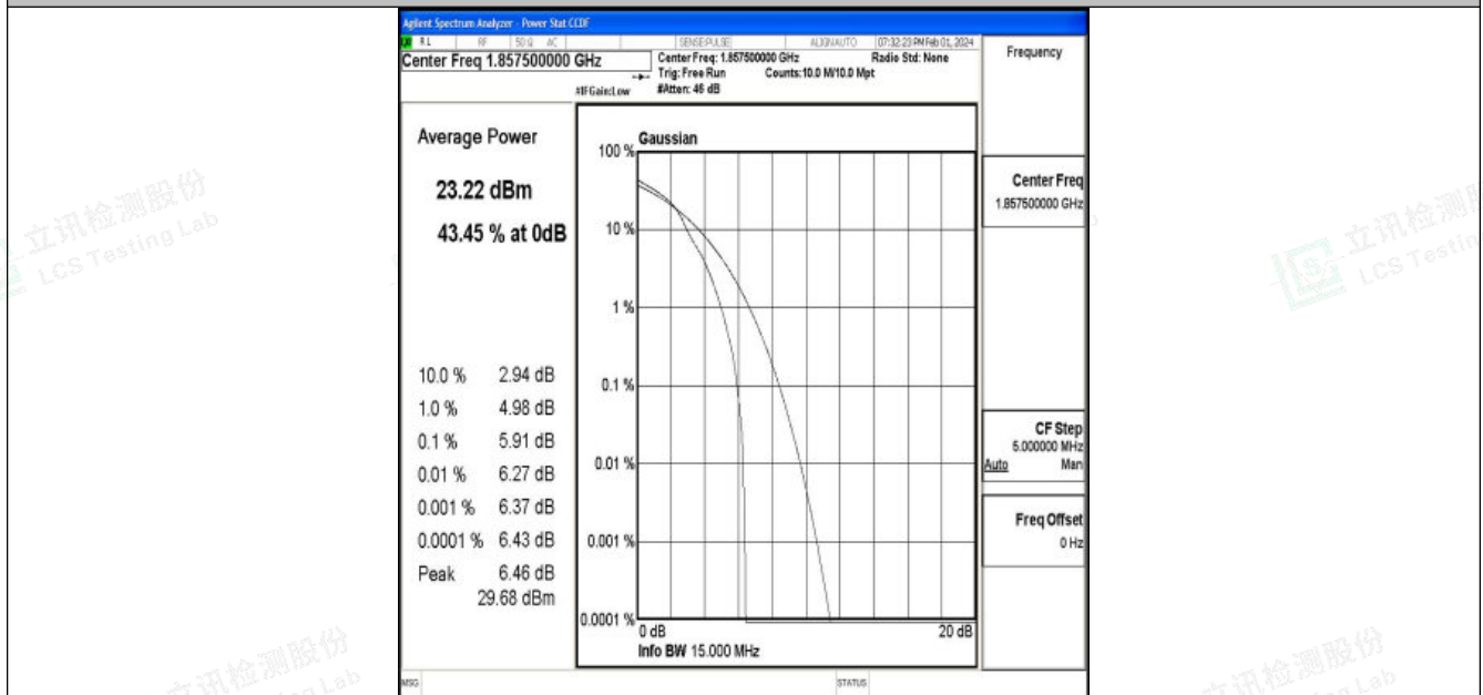
Band25-15MHz-16QAM-26115-1RB#0-PASS
