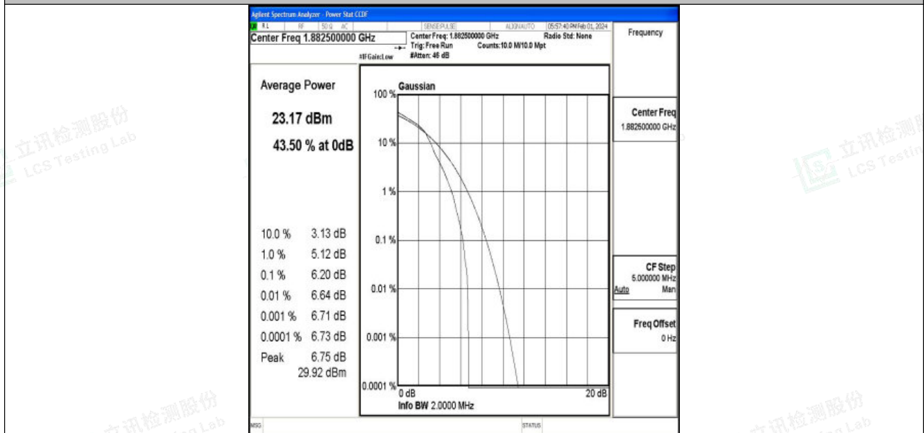
Band25-1.4MHz-16QAM-26365-1RB#0-PASS
