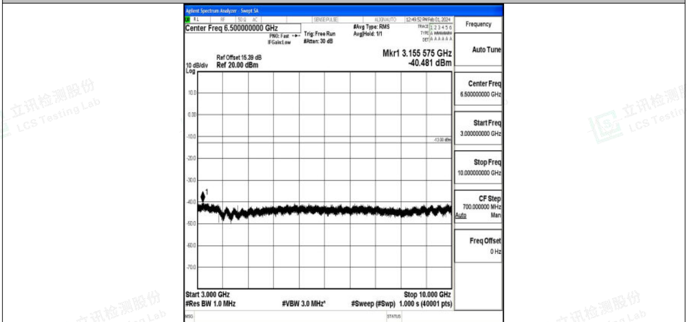
Band5_1.4MHz_16QAM_20407_1RB#0_3000~10000_3000~10000
