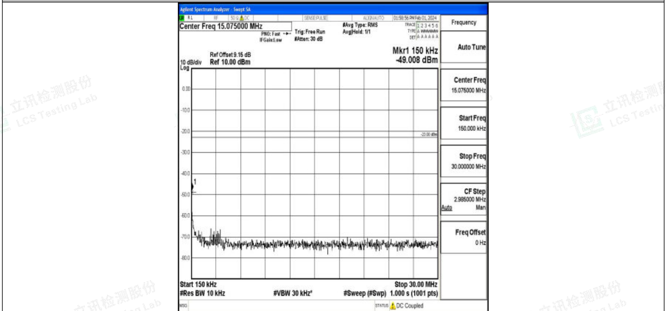
Band5_10MHz_QPSK_20525_1RB#0_0.15~30_0.15~30
