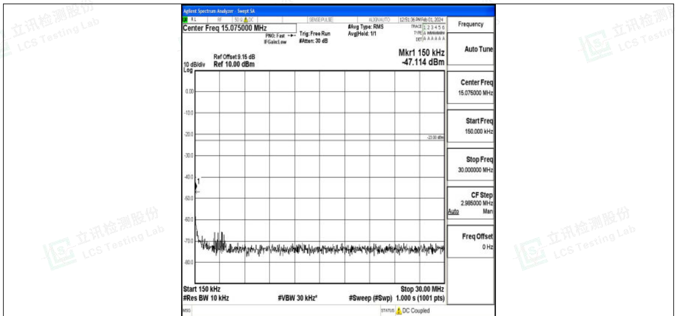
Band5_1.4MHz_16QAM_20643_1RB#0_0.15~30_0.15~30
