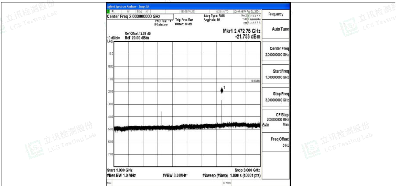
Band5_1.4MHz_16QAM_20407_1RB#0_1000~3000_1000~3000
