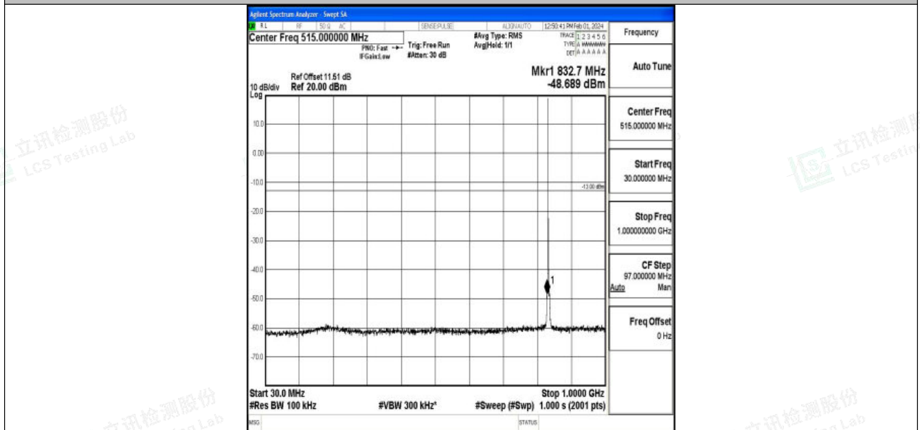
Band5_1.4MHz_16QAM_20525_1RB#0_30~1000_30~1000
