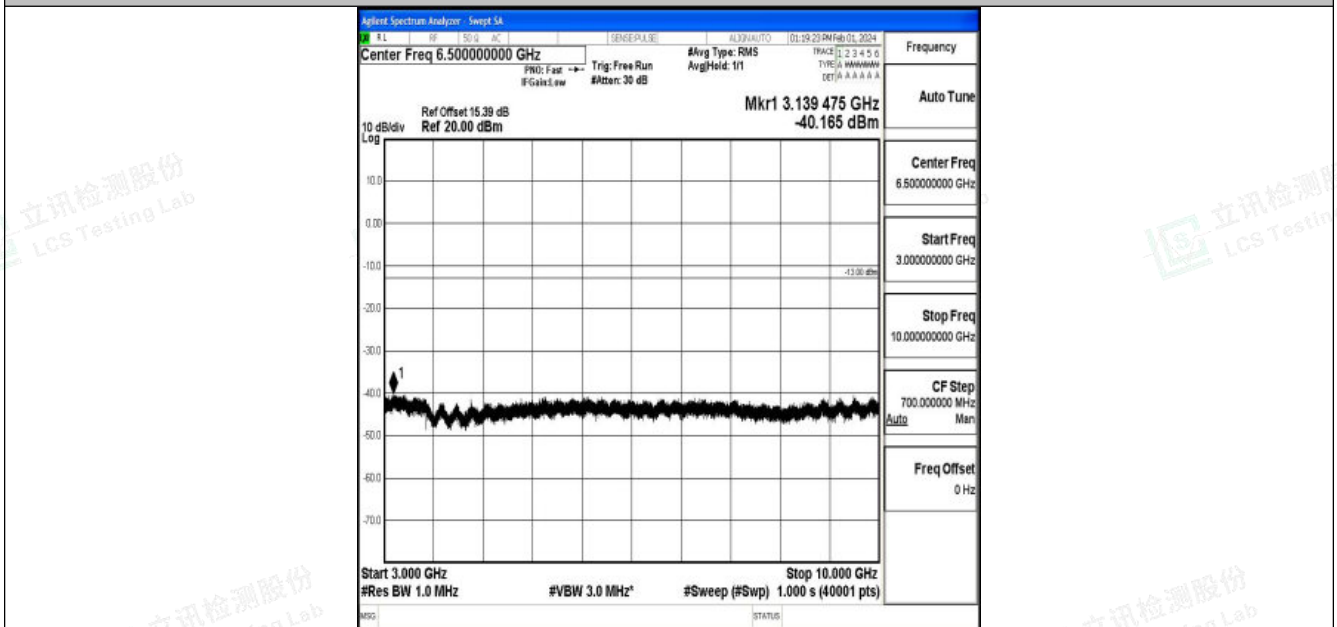
Band5_3MHz_16QAM_20635_1RB#0_3000~10000_3000~10000
