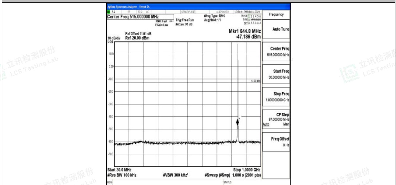
Band5_1.4MHz_16QAM_20643_1RB#0_30~1000_30~1000
