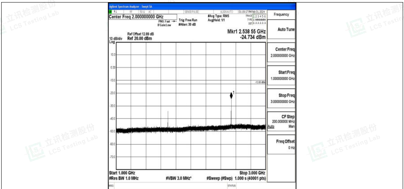
Band5_3MHz_16QAM_20635_1RB#0_1000~3000_1000~3000
