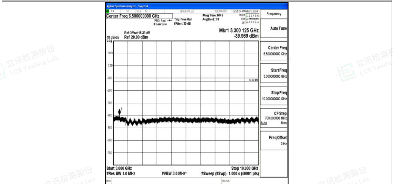
Band5_1.4MHz_16QAM_20643_1RB#0_3000~10000_3000~10000
