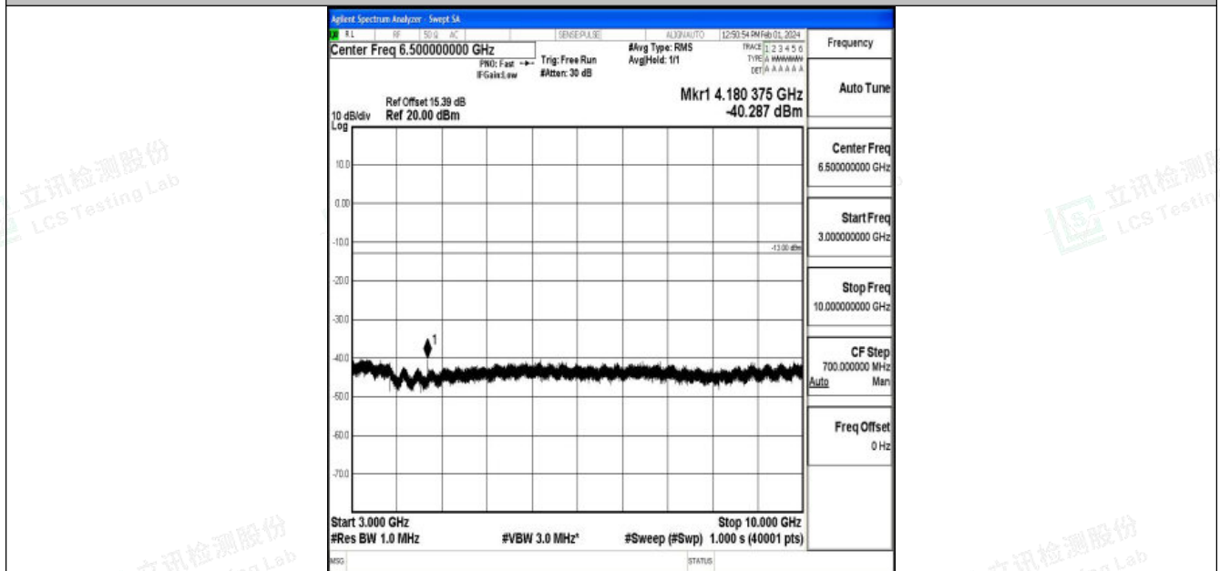
Band5_1.4MHz_16QAM_20525_1RB#0_3000~10000_3000~10000
