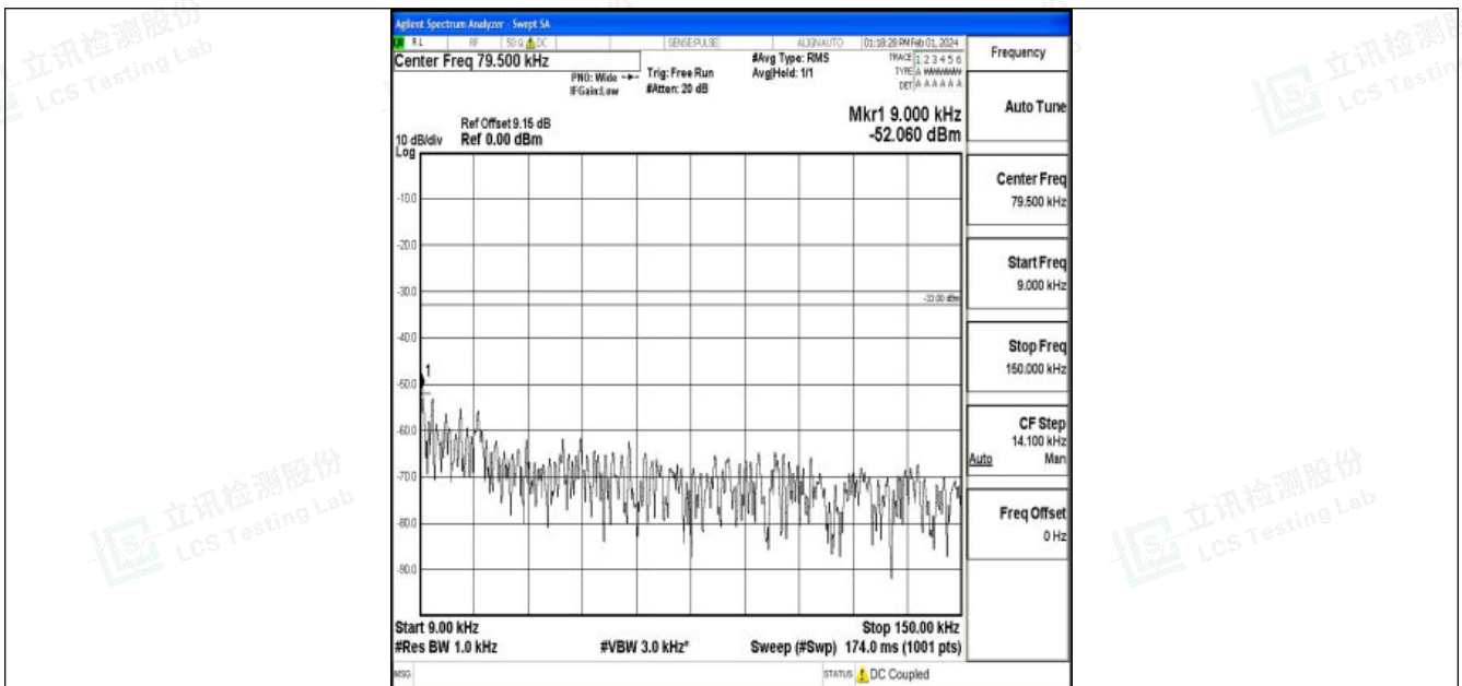
Band5_3MHz_QPSK_20635_1RB#0_0.009~0.15_0.009~0.15
