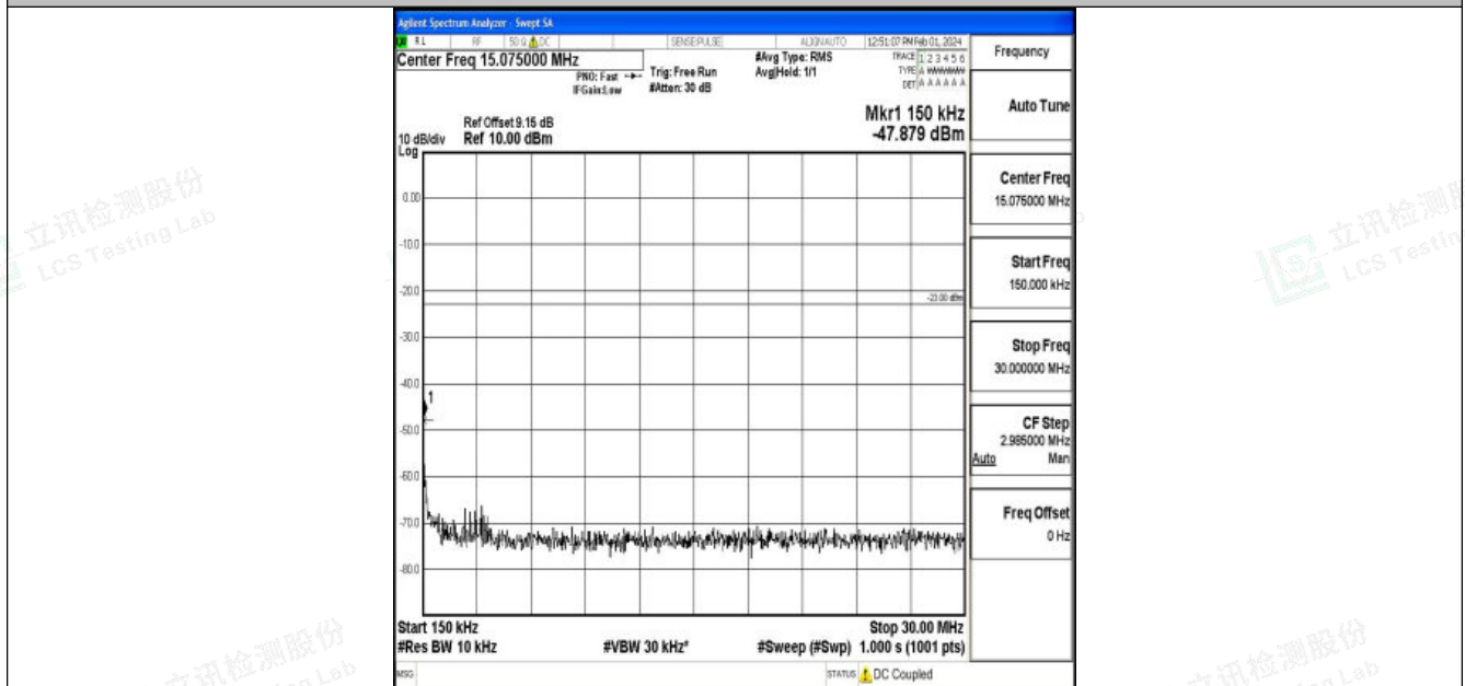
Band5_1.4MHz_QPSK_20643_1RB#0_0.15~30_0.15~30
