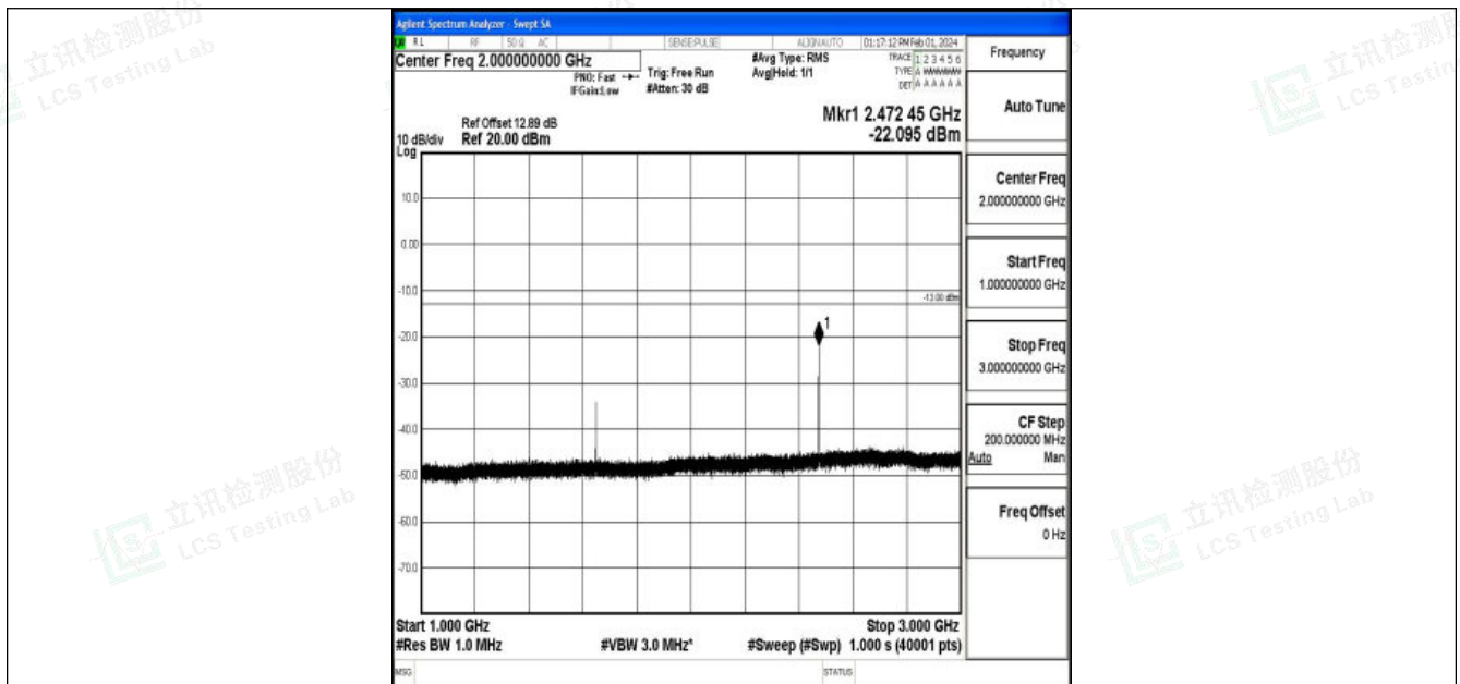
Band5_3MHz_16QAM_20415_1RB#0_1000~3000_1000~3000
