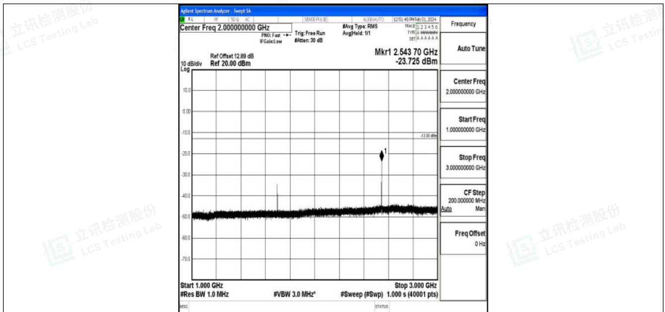
Band5_1.4MHz_16QAM_20643_1RB#0_1000~3000_1000~3000
