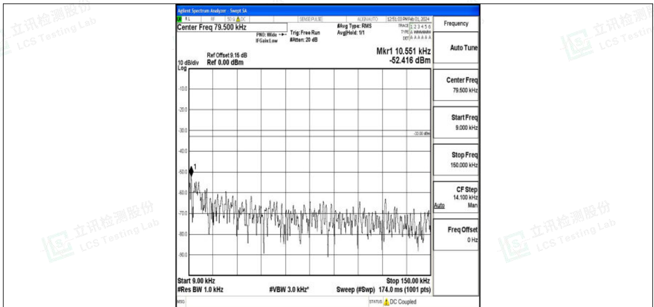
Band5_1.4MHz_QPSK_20643_1RB#0_0.009~0.15_0.009~0.15
