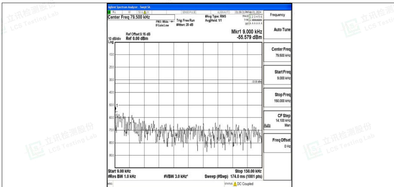
Band5_5MHz_QPSK_20625_1RB#0_0.009~0.15_0.009~0.15
