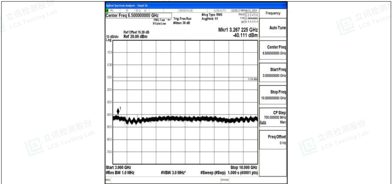
Band5_10MHz_QPSK_20600_1RB#0_3000~10000_3000~10000
