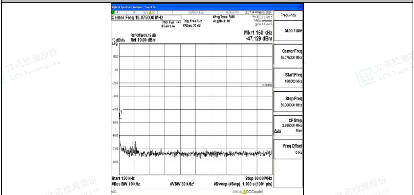
Band5_5MHz_QPSK_20425_1RB#0_0.15~30_0.15~30
