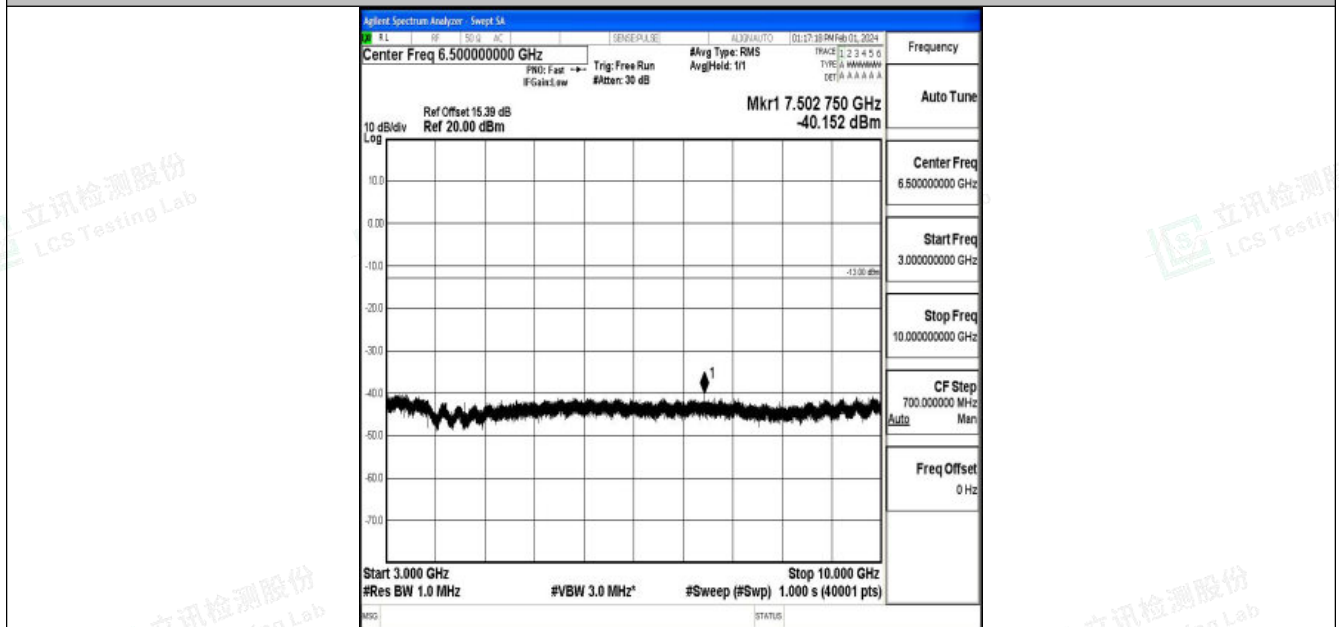
Band5_3MHz_16QAM_20415_1RB#0_3000~10000_3000~10000
