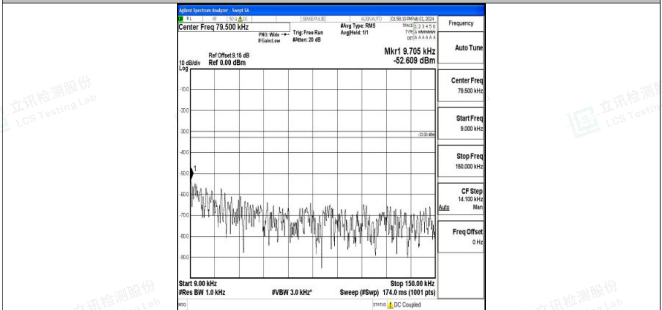
Band5_10MHz_16QAM_20450_1RB#0_0.009~0.15_0.009~0.15
