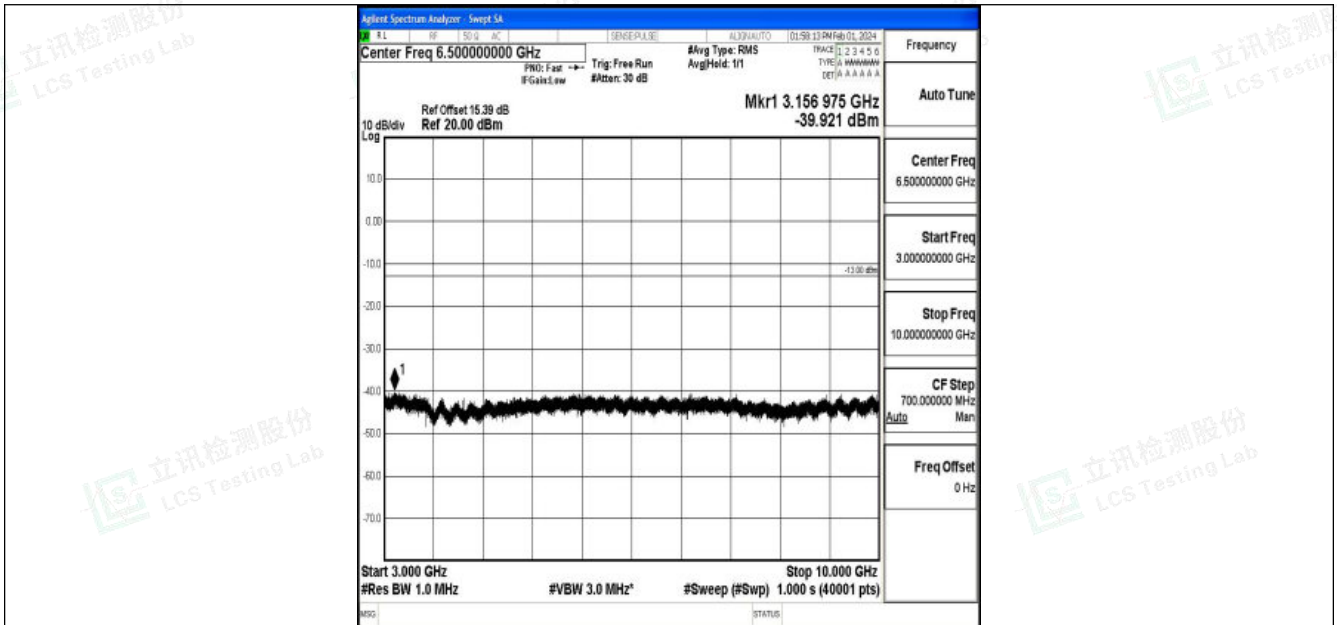
Band5_10MHz_QPSK_20450_1RB#0_3000~10000_3000~10000
