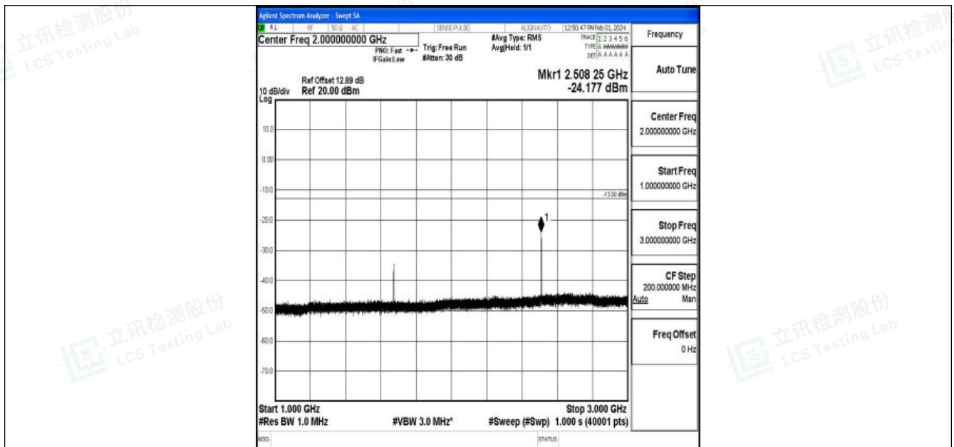
Band5_1.4MHz_16QAM_20525_1RB#0_1000~3000_1000~3000
