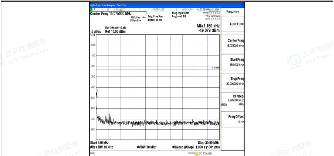
Band5_10MHz_QPSK_20450_1RB#0_0.15~30_0.15~30
