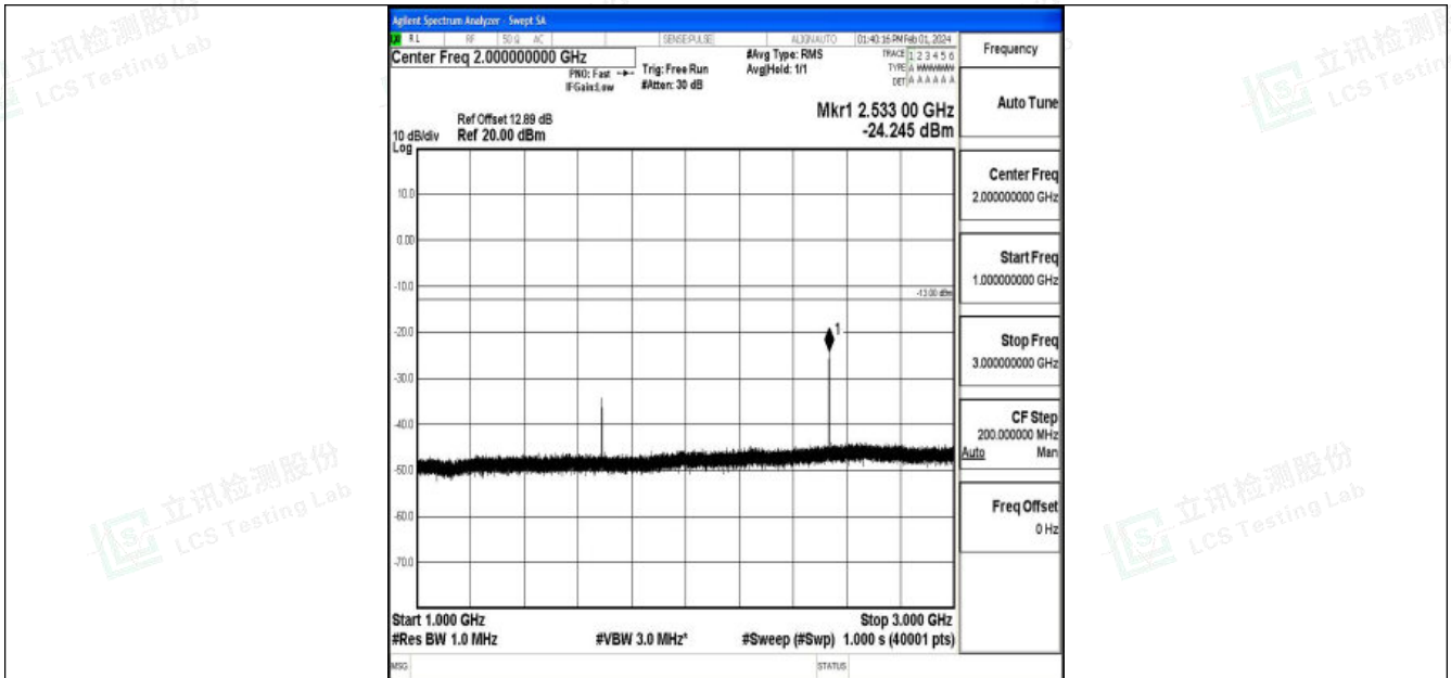
Band5_5MHz_16QAM_20625_1RB#0_1000~3000_1000~3000
