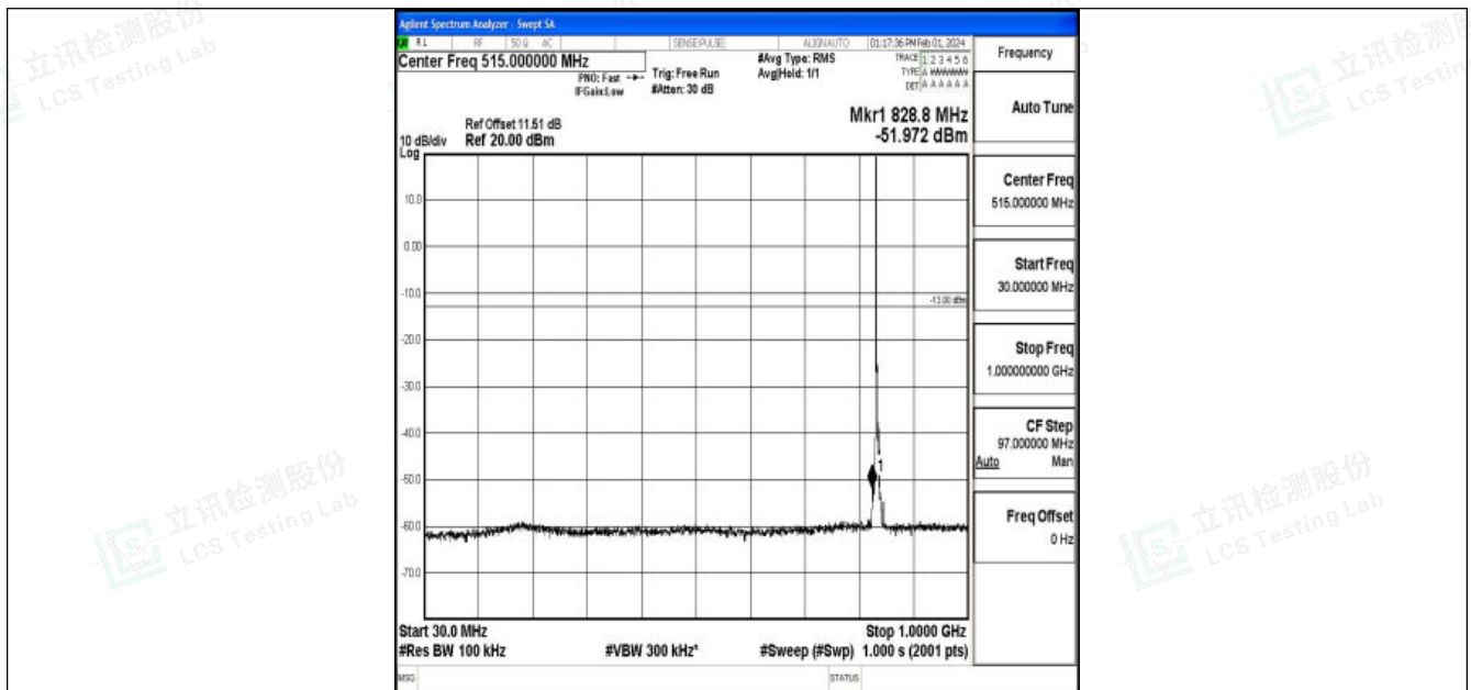
Band5_3MHz_QPSK_20525_1RB#0_30~1000_30~1000
