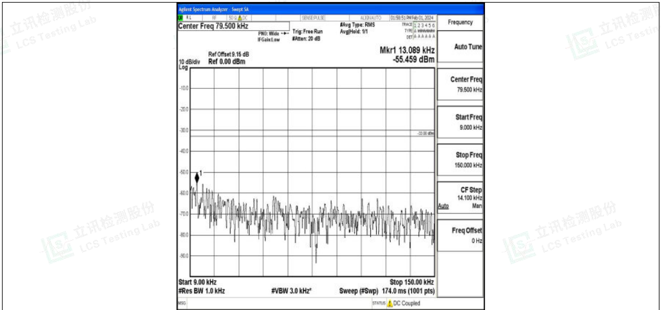
Band5_10MHz_QPSK_20525_1RB#0_0.009~0.15_0.009~0.15
