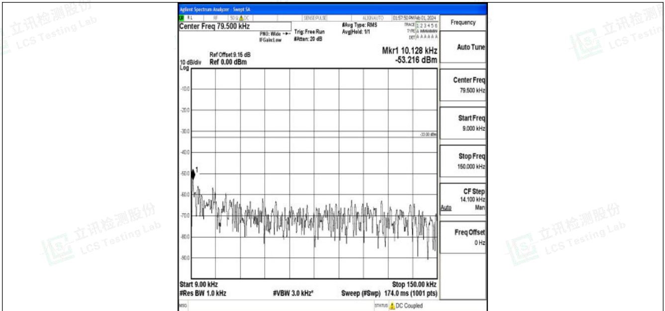
Band5_10MHz_QPSK_20450_1RB#0_0.009~0.15_0.009~0.15
