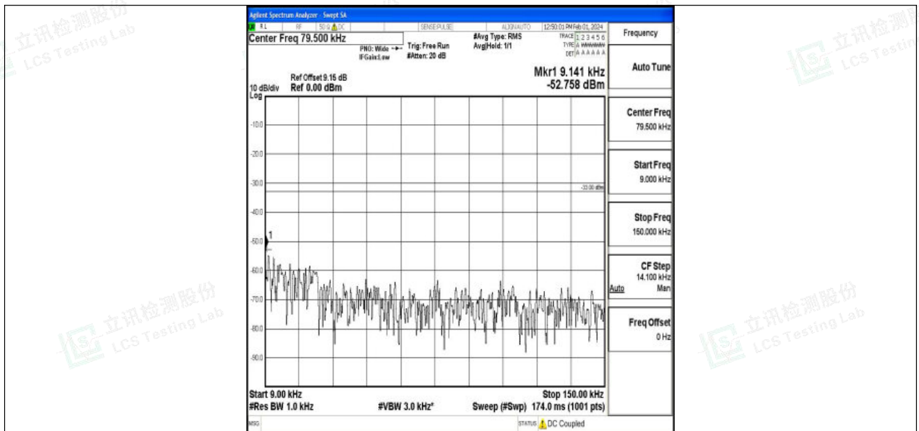
Band5_1.4MHz_QPSK_20525_1RB#0_0.009~0.15_0.009~0.15
