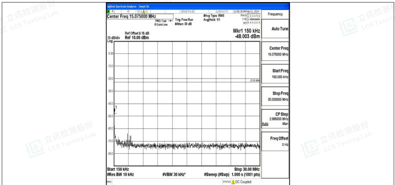
Band5_1.4MHz_16QAM_20525_1RB#0_0.15~30_0.15~30
