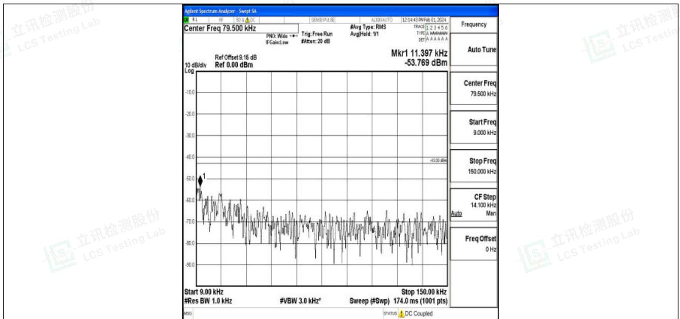
Band4_15MHz_QPSK_20175_1RB#0_0.009~0.15_0.009~0.15
