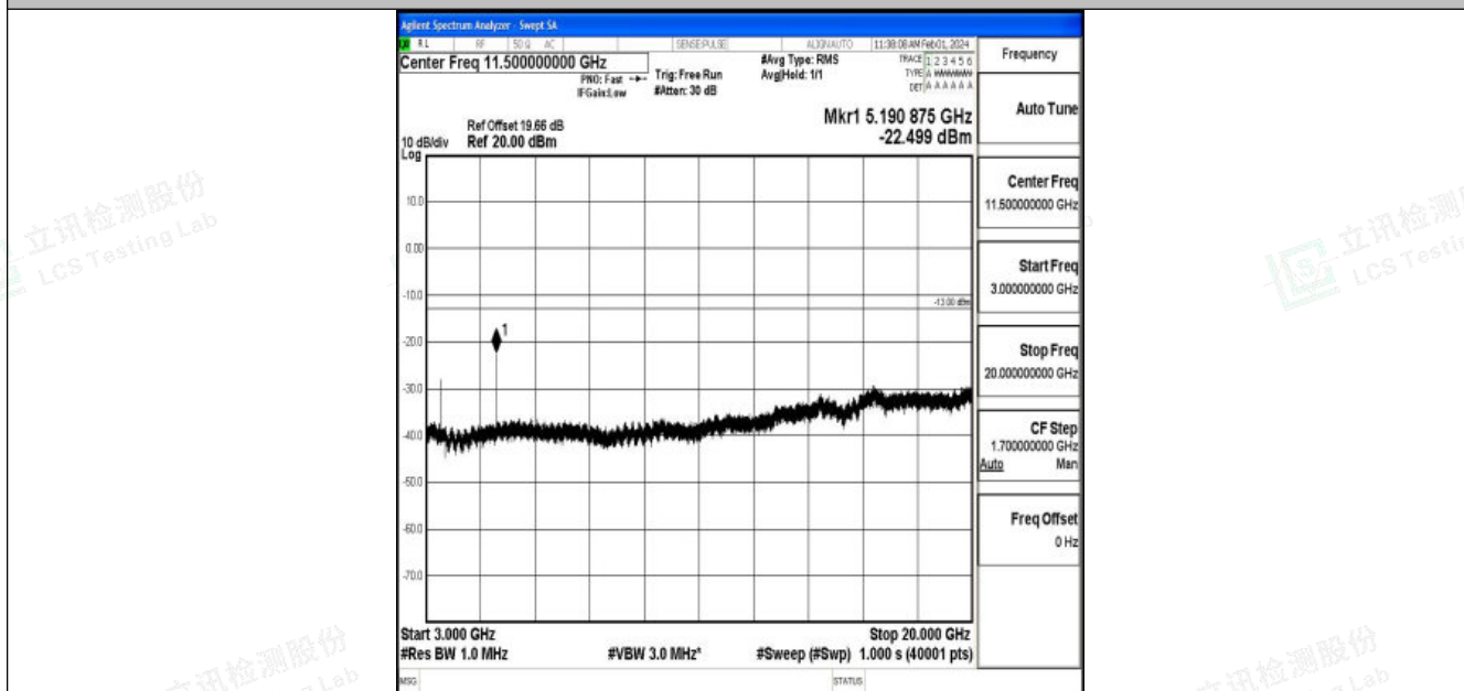
Band4_5MHz_16QAM_20175_1RB#0_3000~20000_3000~20000
