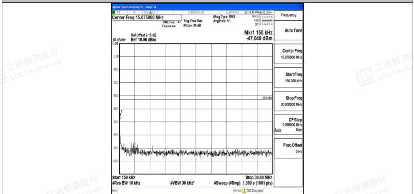
Band4_15MHz_QPSK_20175_1RB#0_0.15~30_0.15~30
