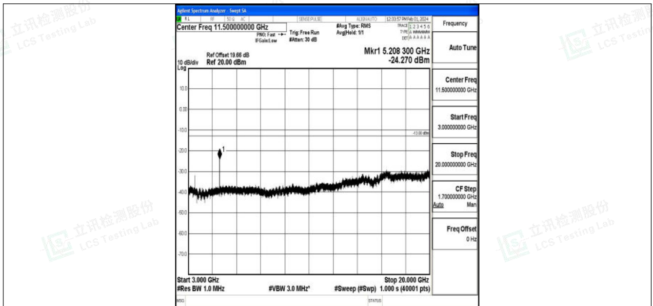
Band4_20MHz_QPSK_20300_1RB#0_3000~20000_3000~20000
