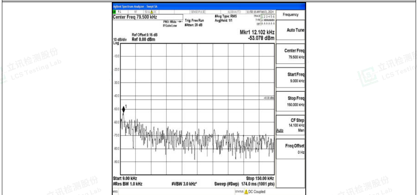
Band4_10MHz_16QAM_20350_1RB#0_0.009~0.15_0.009~0.15
