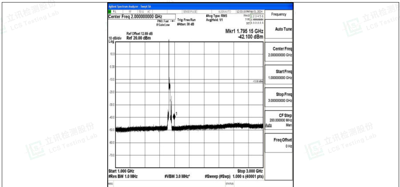
Band4_20MHz_16QAM_20175_1RB#0_1000~3000_1000~3000
