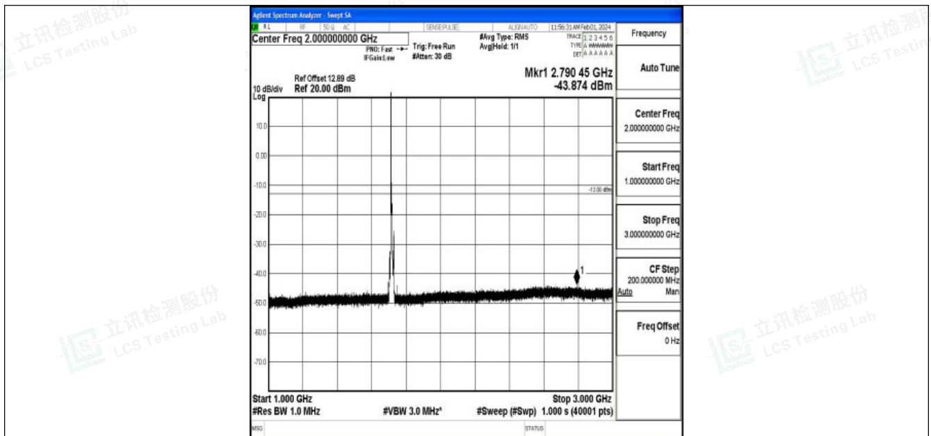
Band4_10MHz_16QAM_20000_1RB#0_1000~3000_1000~3000
