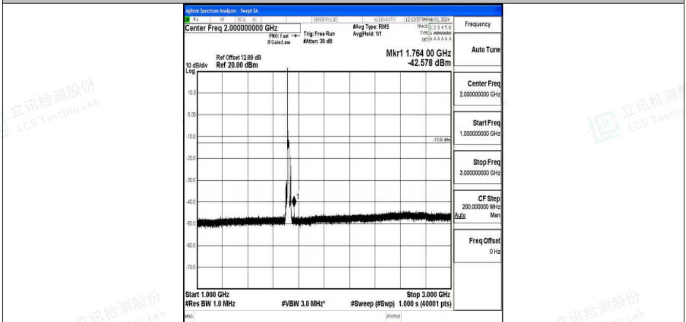
Band4_15MHz_QPSK_20025_1RB#0_1000~3000_1000~3000
