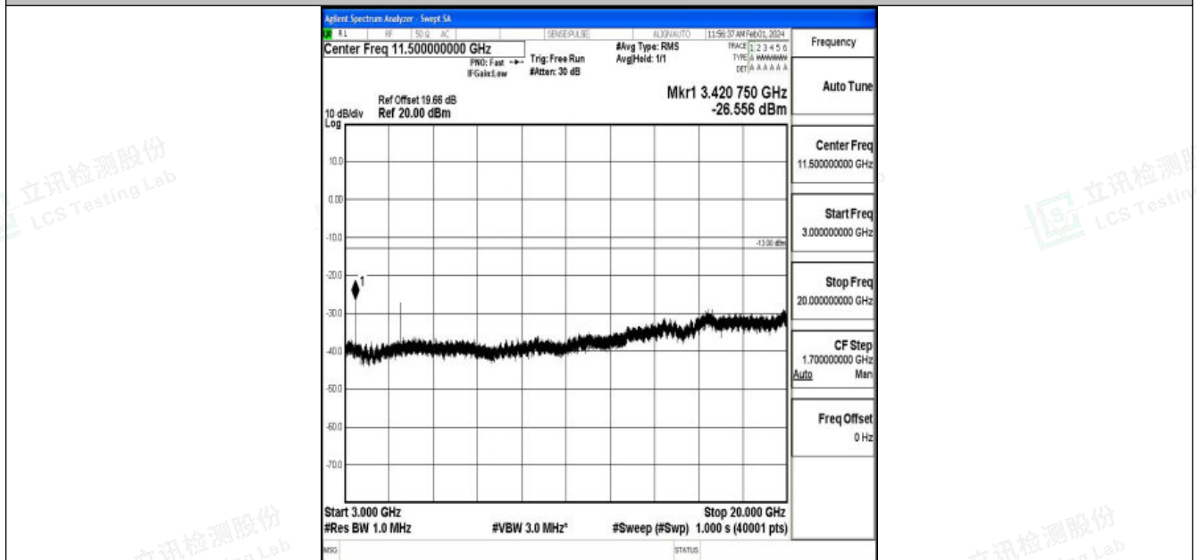
Band4_10MHz_16QAM_20000_1RB#0_3000~20000_3000~20000
