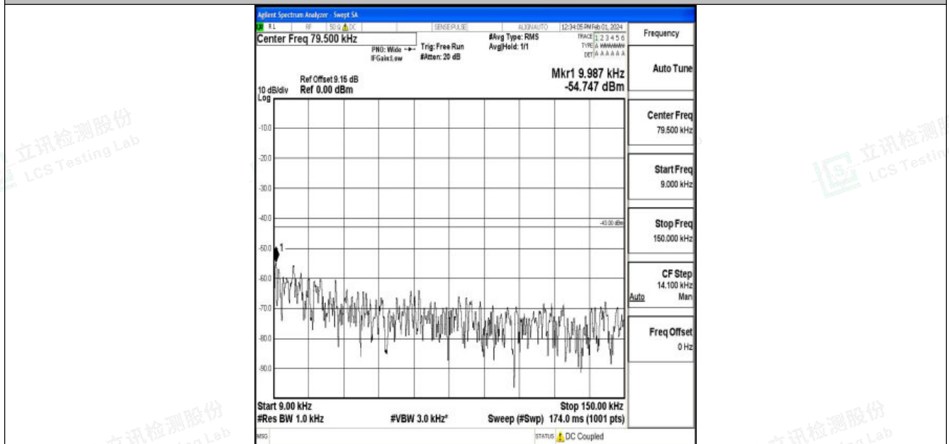
Band4_20MHz_16QAM_20300_1RB#0_0.009~0.15_0.009~0.15
