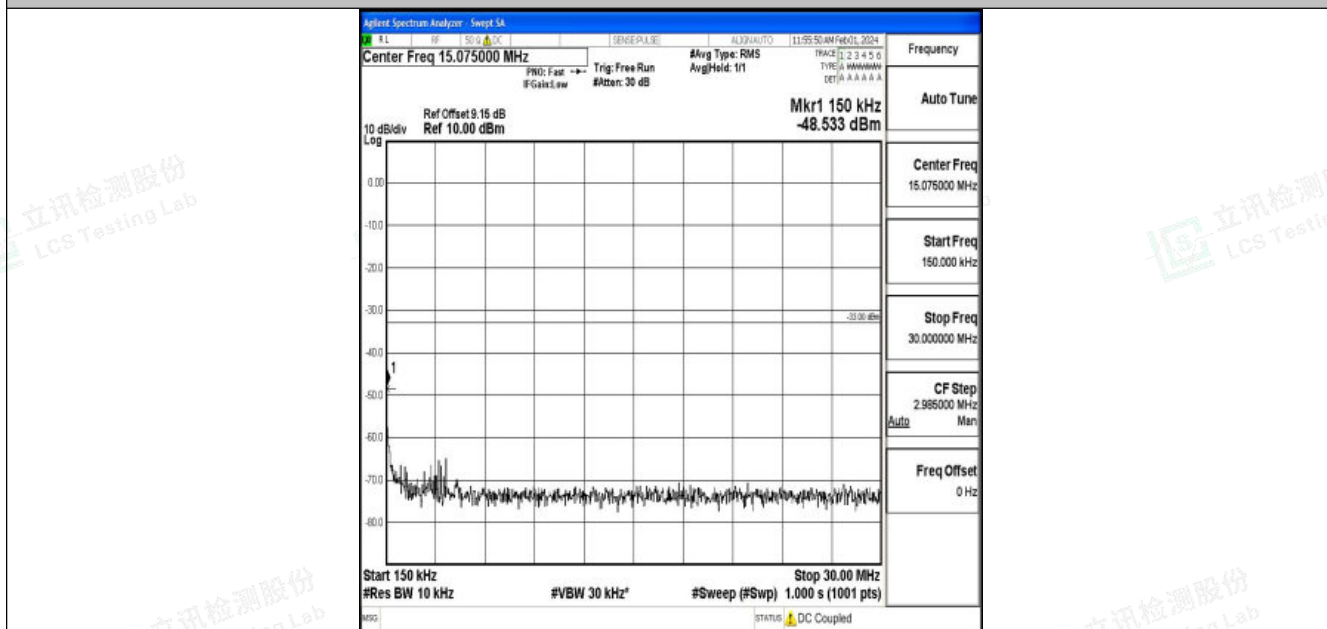
Band4_10MHz_QPSK_20000_1RB#0_0.15~30_0.15~30
