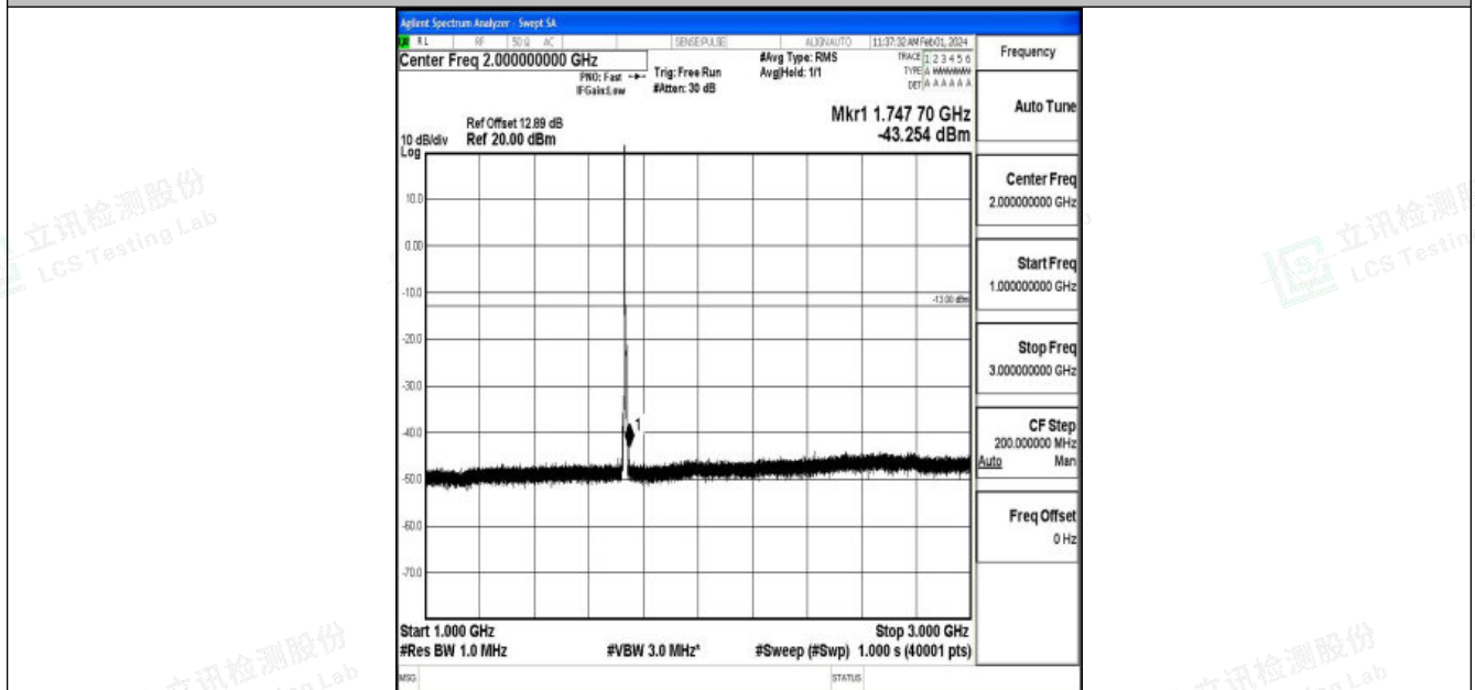
Band4_5MHz_QPSK_20175_1RB#0_1000~3000_1000~3000
