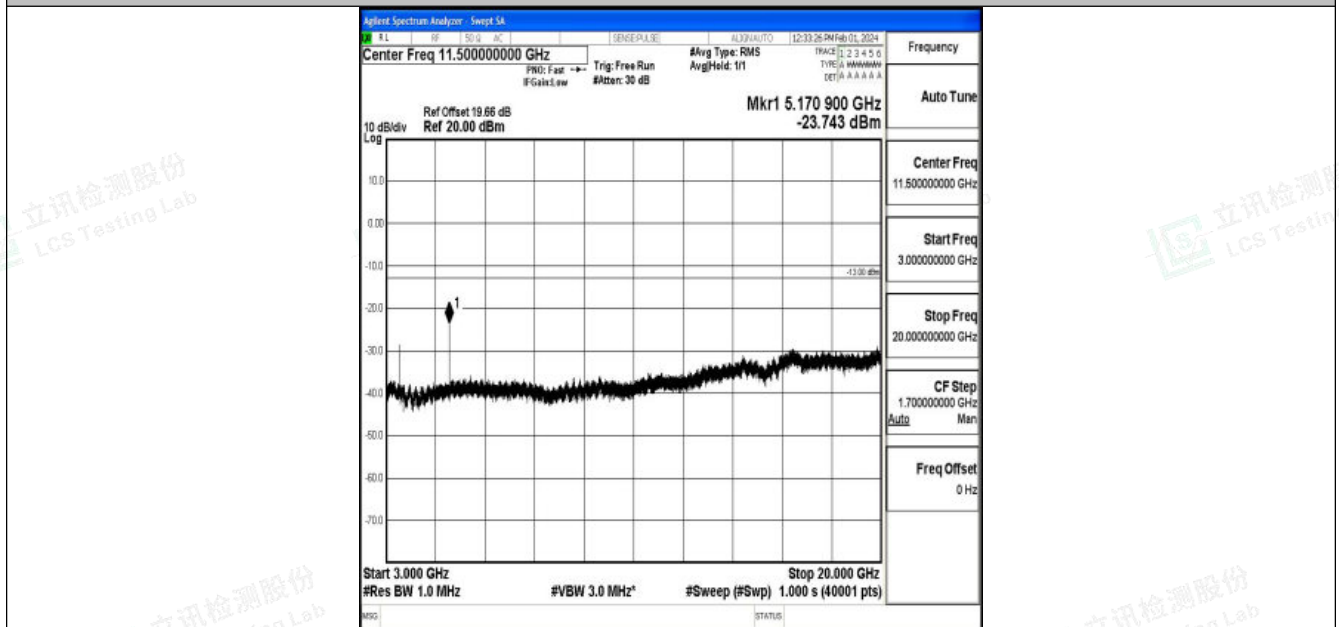
Band4_20MHz_16QAM_20175_1RB#0_3000~20000_3000~20000
