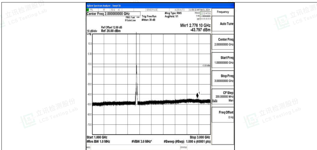
Band4_10MHz_16QAM_20350_1RB#0_1000~3000_1000~3000
