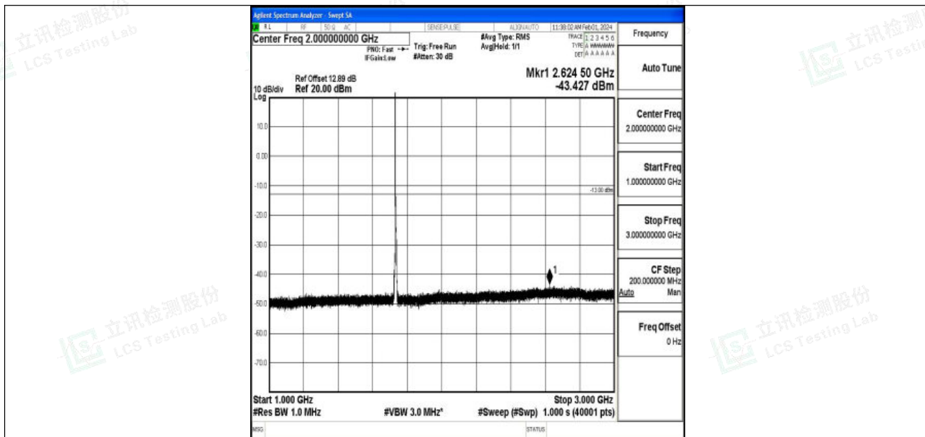
Band4_5MHz_16QAM_20175_1RB#0_1000~3000_1000~3000
