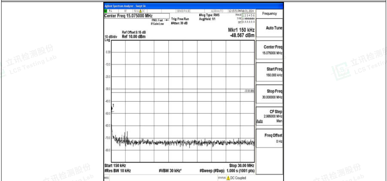
Band4_15MHz_QPSK_20325_1RB#0_0.15~30_0.15~30
