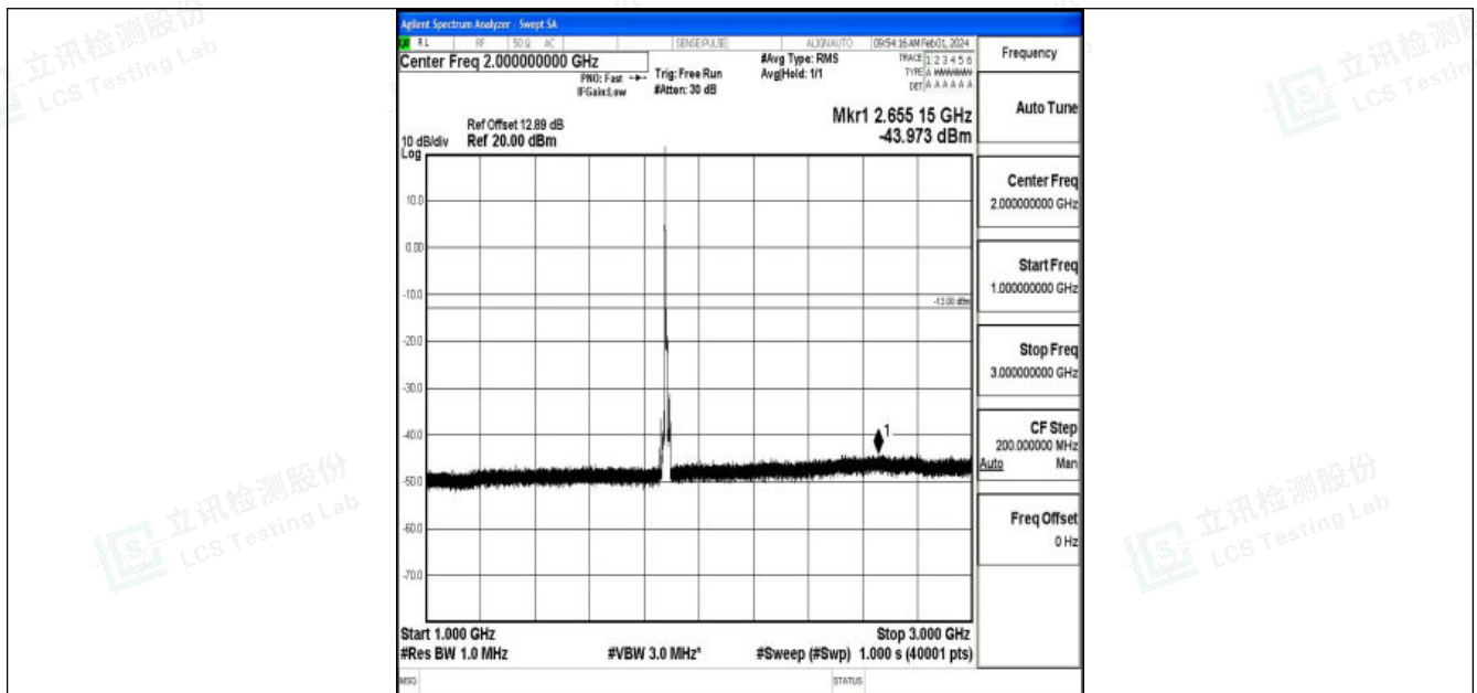
Band2_10MHz_16QAM_18900_1RB#0_1000~3000_1000~3000
