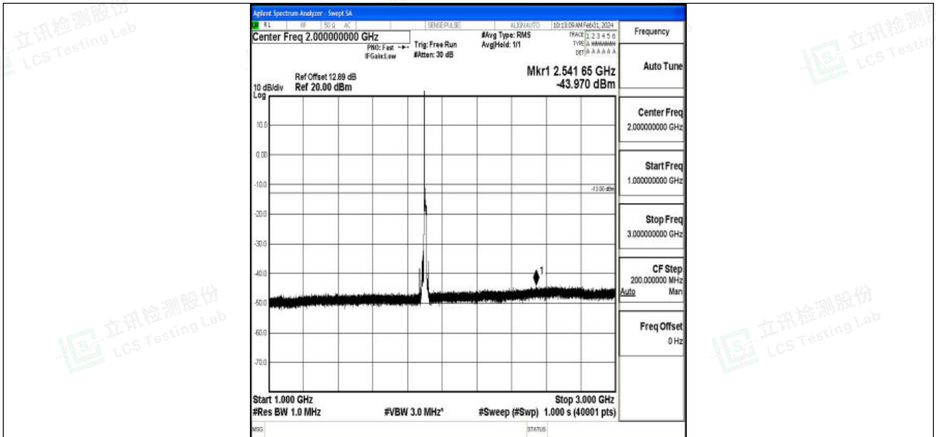
Band2_15MHz_16QAM_19125_1RB#0_1000~3000_1000~3000
