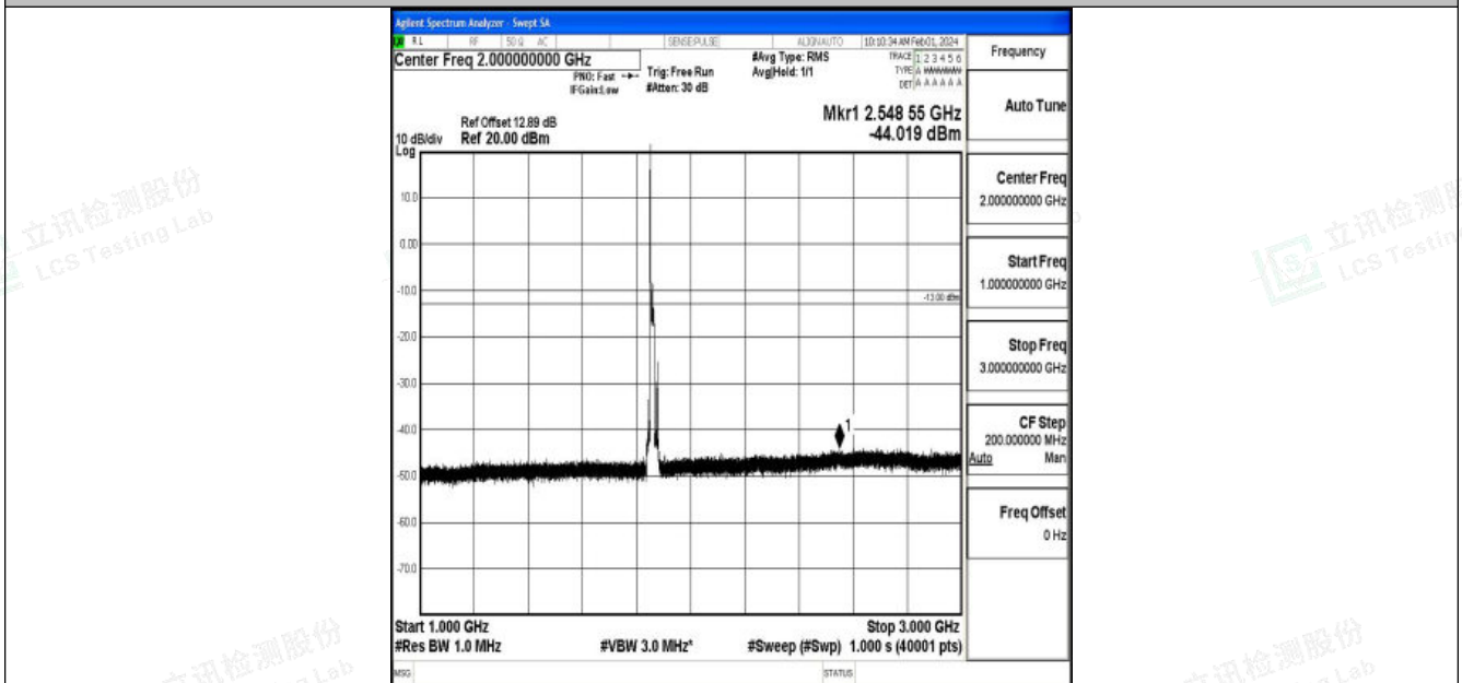
Band2_15MHz_QPSK_18675_1RB#0_1000~3000_1000~3000
