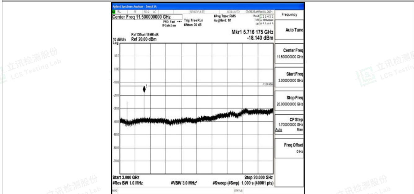
Band2_5MHz_16QAM_19175_1RB#0_3000~20000_3000~20000
