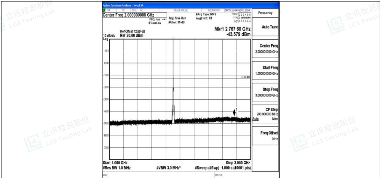
Band2_10MHz_16QAM_19150_1RB#0_1000~3000_1000~3000
