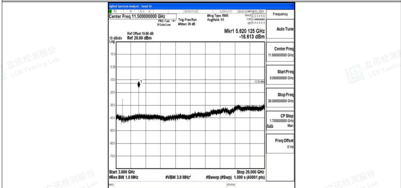
Band2_15MHz_16QAM_18900_1RB#0_3000~20000_3000~20000
