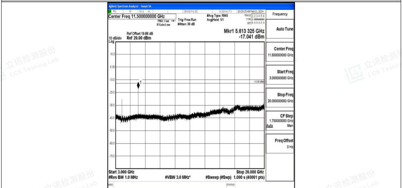
Band2_20MHz_16QAM_18900_1RB#0_3000~20000_3000~20000
