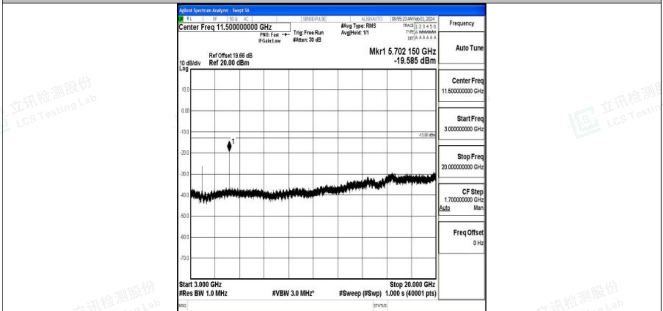
Band2_10MHz_16QAM_19150_1RB#0_3000~20000_3000~20000
