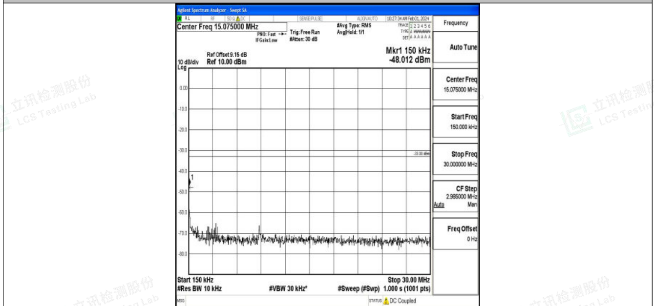
Band2_20MHz_QPSK_18700_1RB#0_0.15~30_0.15~30
