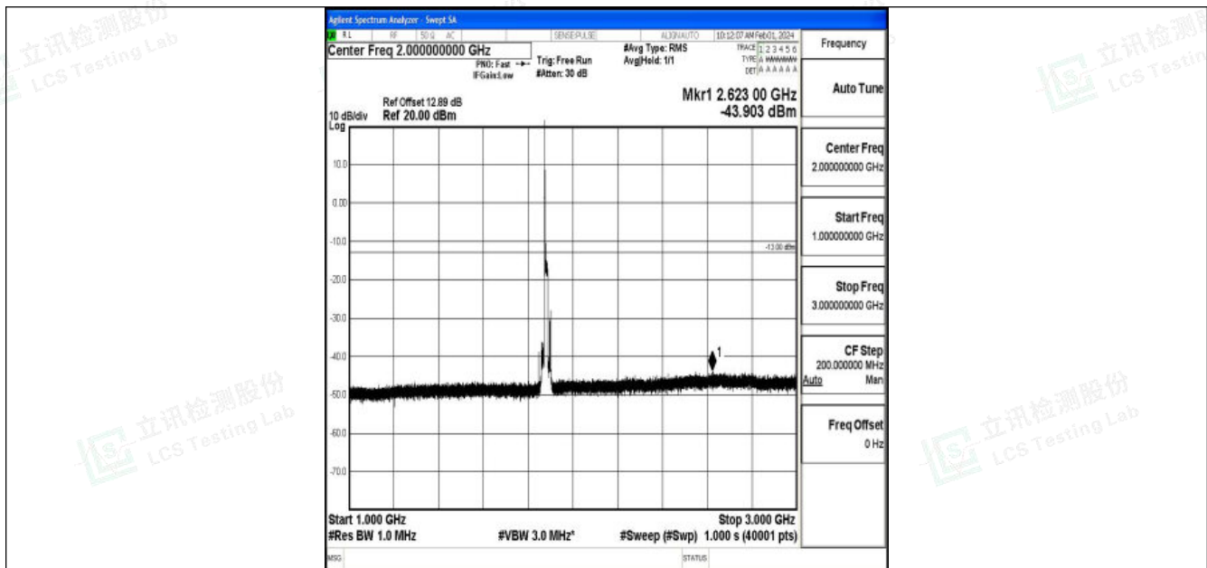
Band2_15MHz_16QAM_18900_1RB#0_1000~3000_1000~3000
