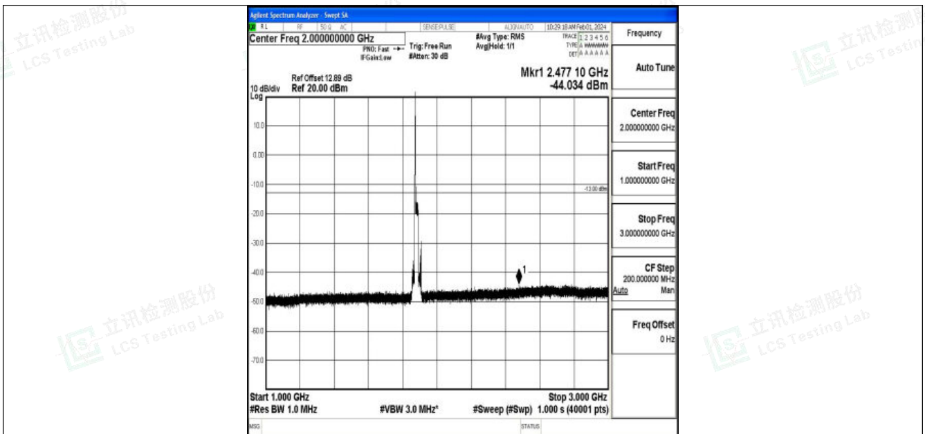
Band2_20MHz_16QAM_18900_1RB#0_1000~3000_1000~3000
