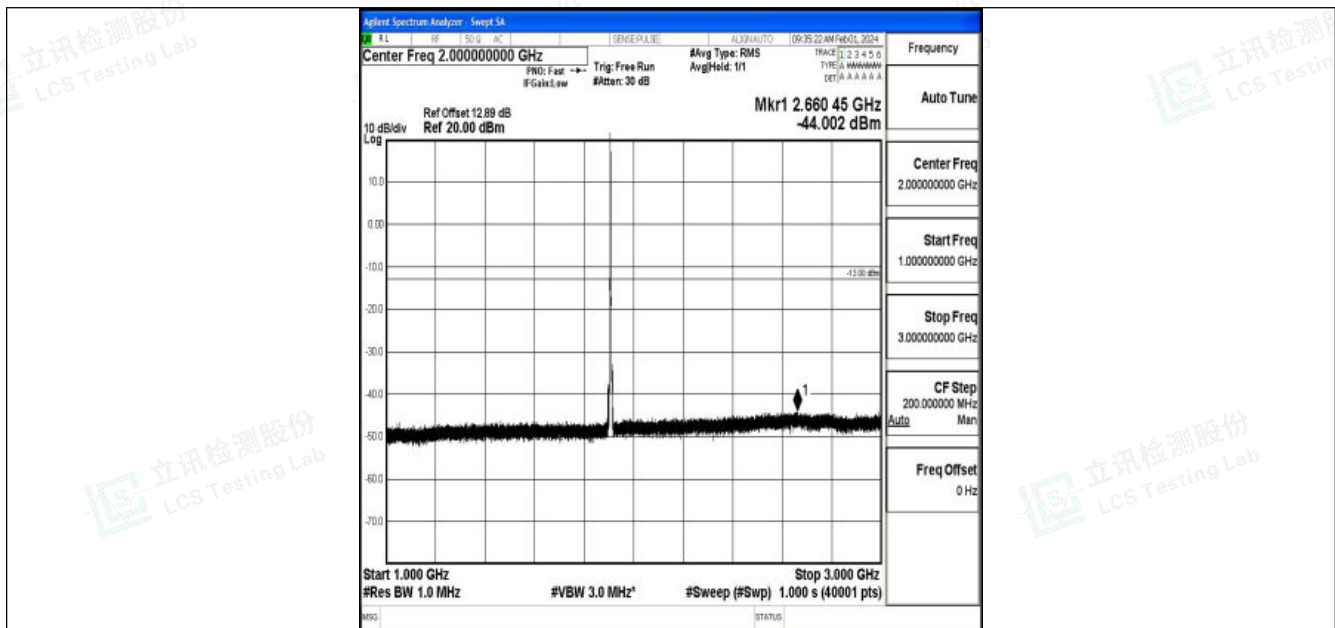
Band2_5MHz_16QAM_19175_1RB#0_1000~3000_1000~3000
