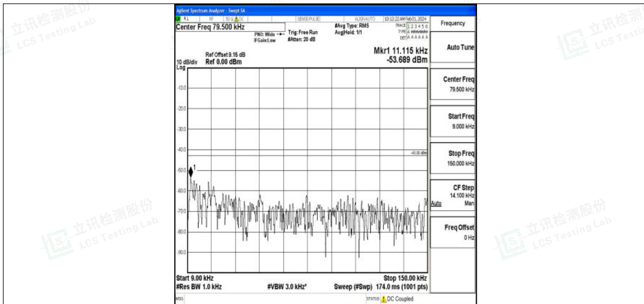
Band2_15MHz_QPSK_19125_1RB#0_0.009~0.15_0.009~0.15
