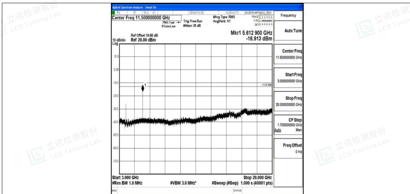
Band2_20MHz_QPSK_18900_1RB#0_3000~20000_3000~20000
